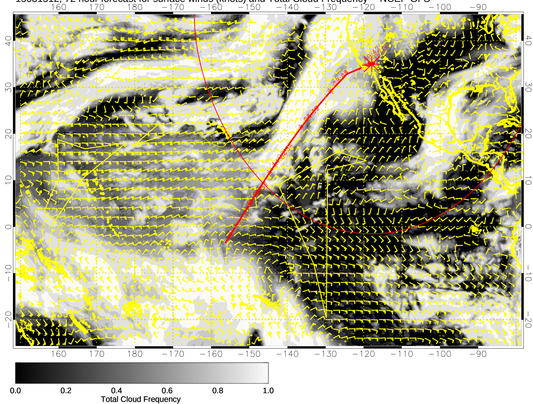
15031512, 72 hour forecast for surface winds (knots) and Total Cloud Frequency -- NCEP GFS
