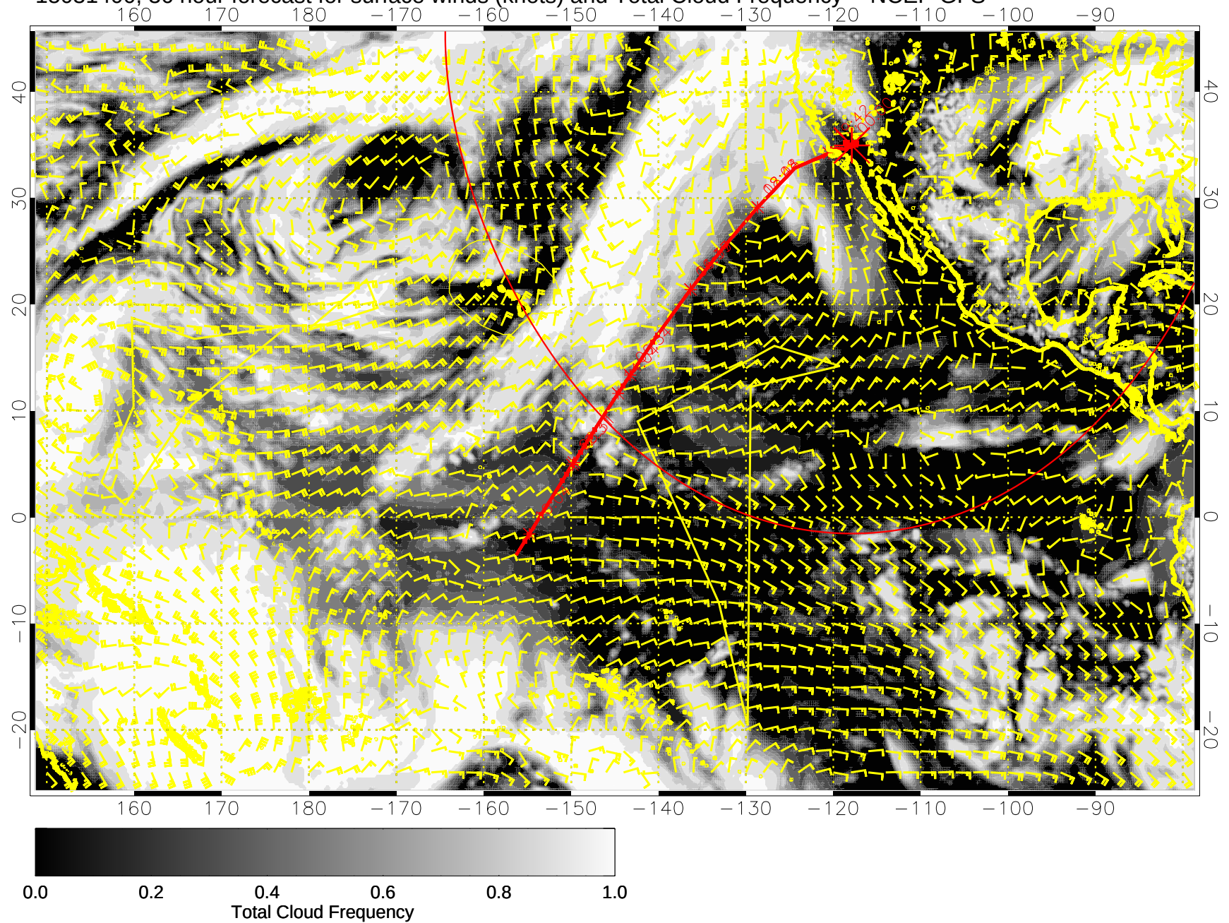
15031400, 36 hour forecast for surface winds (knots) and Total Cloud Frequency -- NCEP GFS
