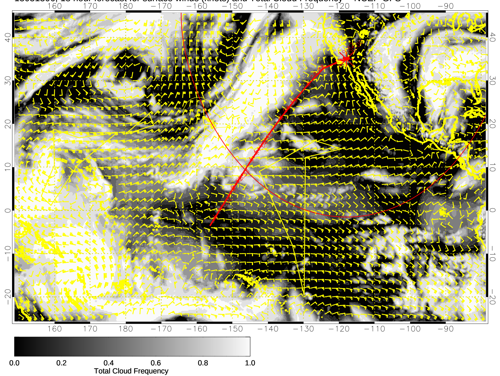
15031306, 18 hour forecast for surface winds (knots) and Total Cloud Frequency -- NCEP GFS
