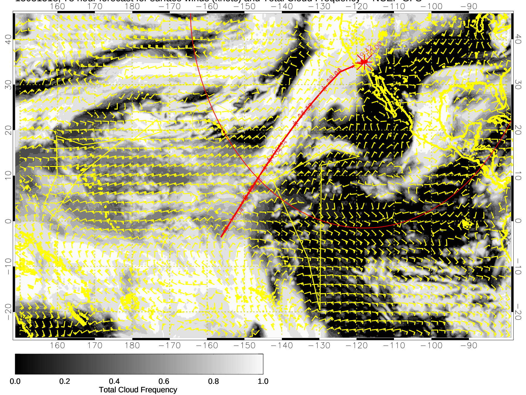
15031518, 78 hour forecast for surface winds (knots) and Total Cloud Frequency -- NCEP GFS
