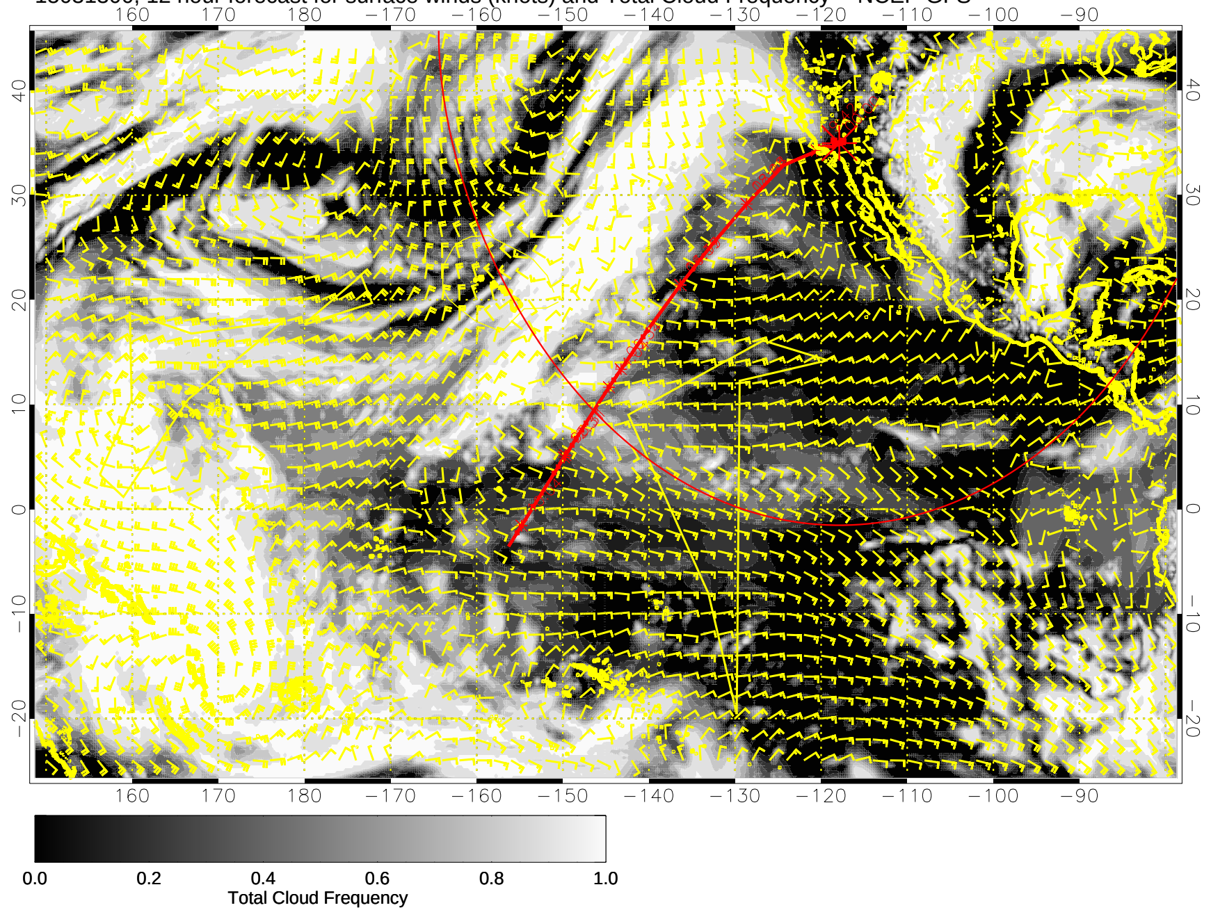
15031300, 12 hour forecast for surface winds (knots) and Total Cloud Frequency -- NCEP GFS
