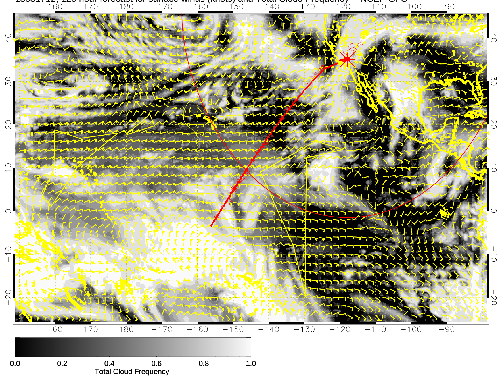
15031712, 120 hour forecast for surface winds (knots) and Total Cloud Frequency -- NCEP GFS
