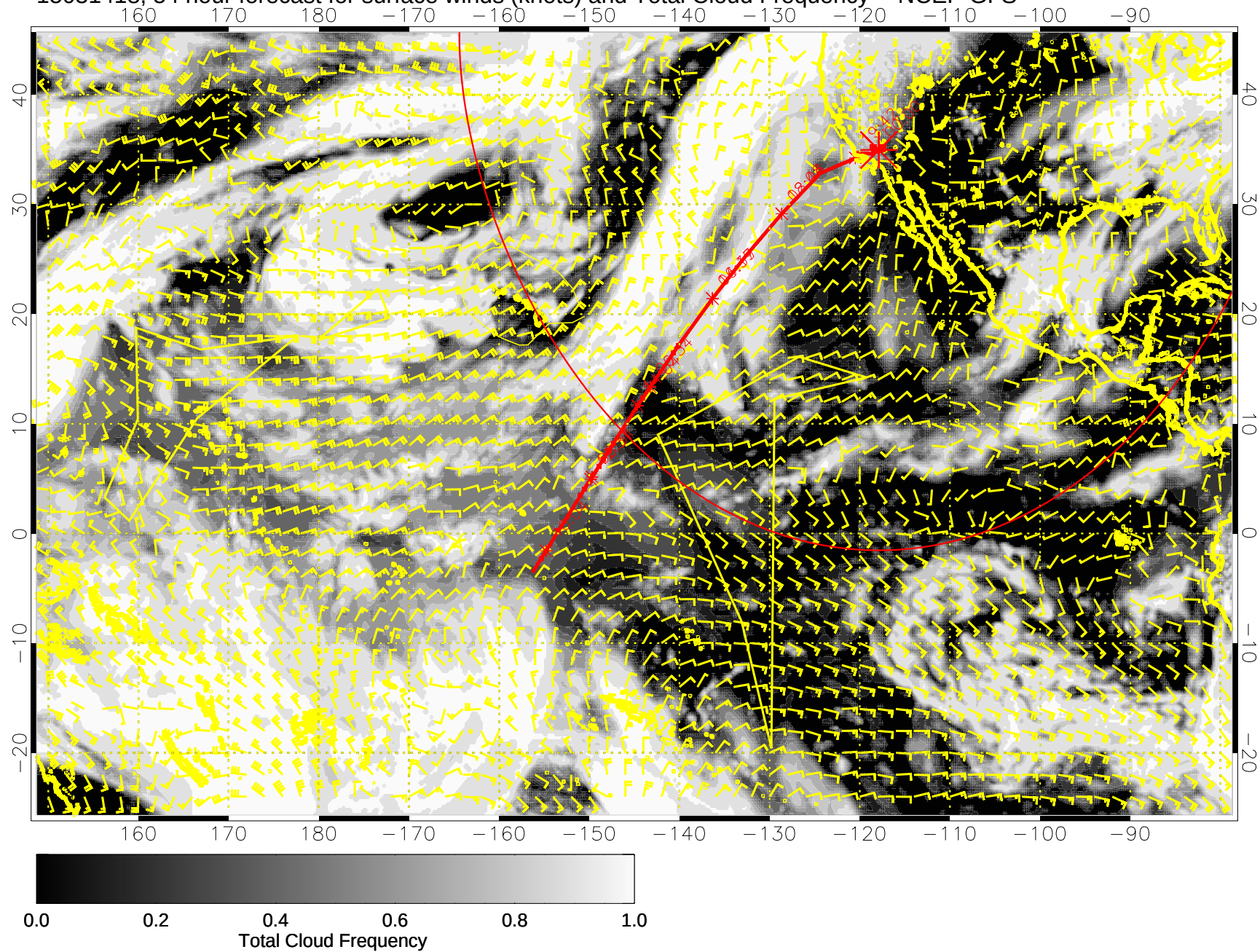
15031418, 54 hour forecast for surface winds (knots) and Total Cloud Frequency -- NCEP GFS
