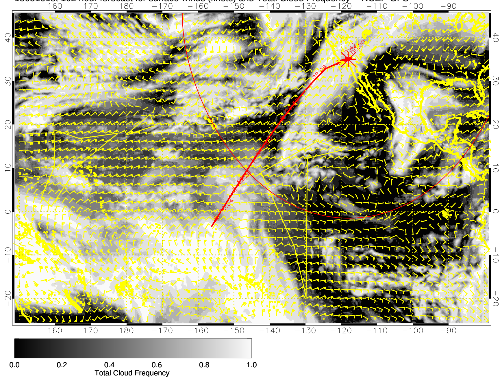
15031618, 102 hour forecast for surface winds (knots) and Total Cloud Frequency -- NCEP GFS
