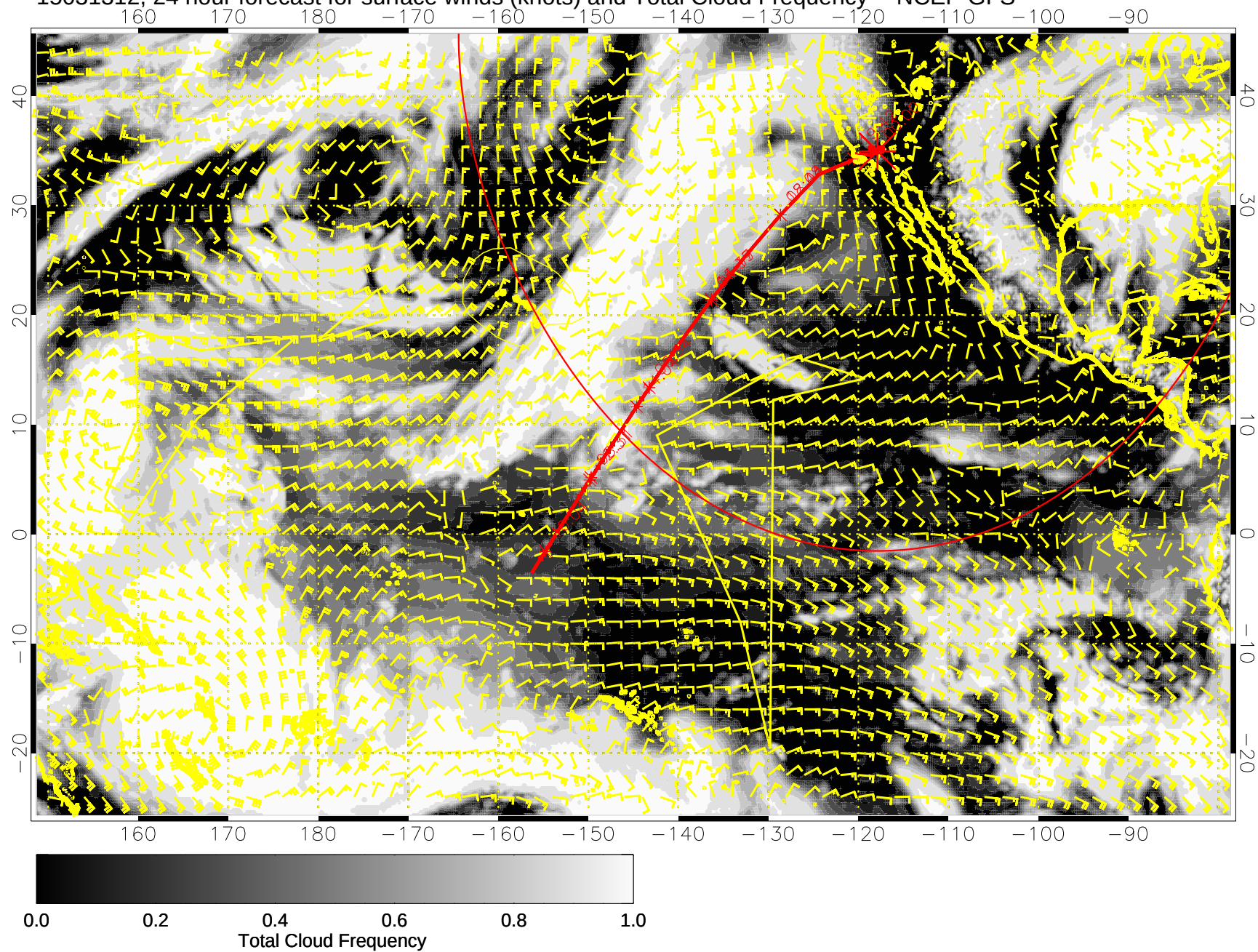
15031312, 24 hour forecast for surface winds (knots) and Total Cloud Frequency -- NCEP GFS
