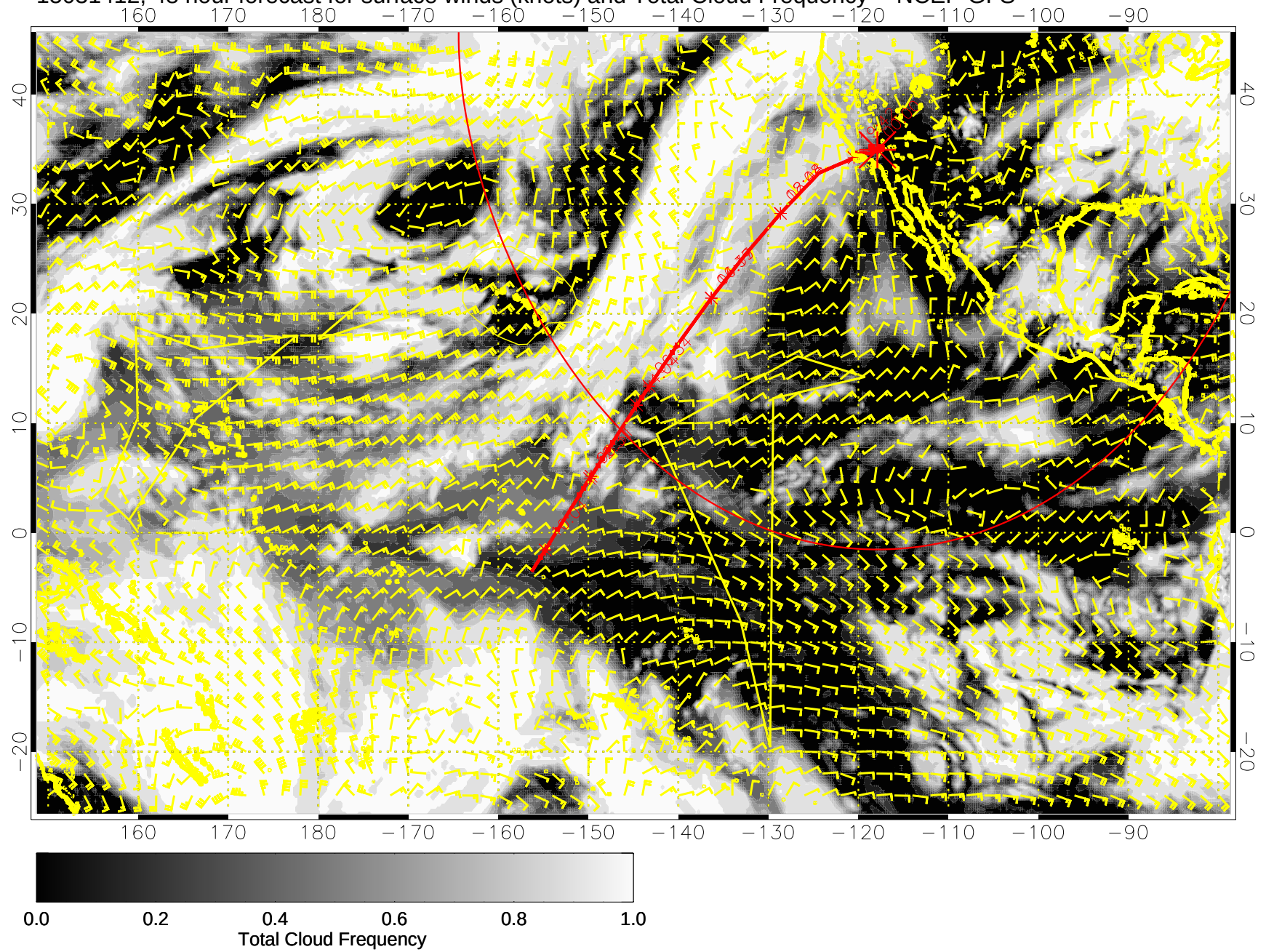
15031412, 48 hour forecast for surface winds (knots) and Total Cloud Frequency -- NCEP GFS
