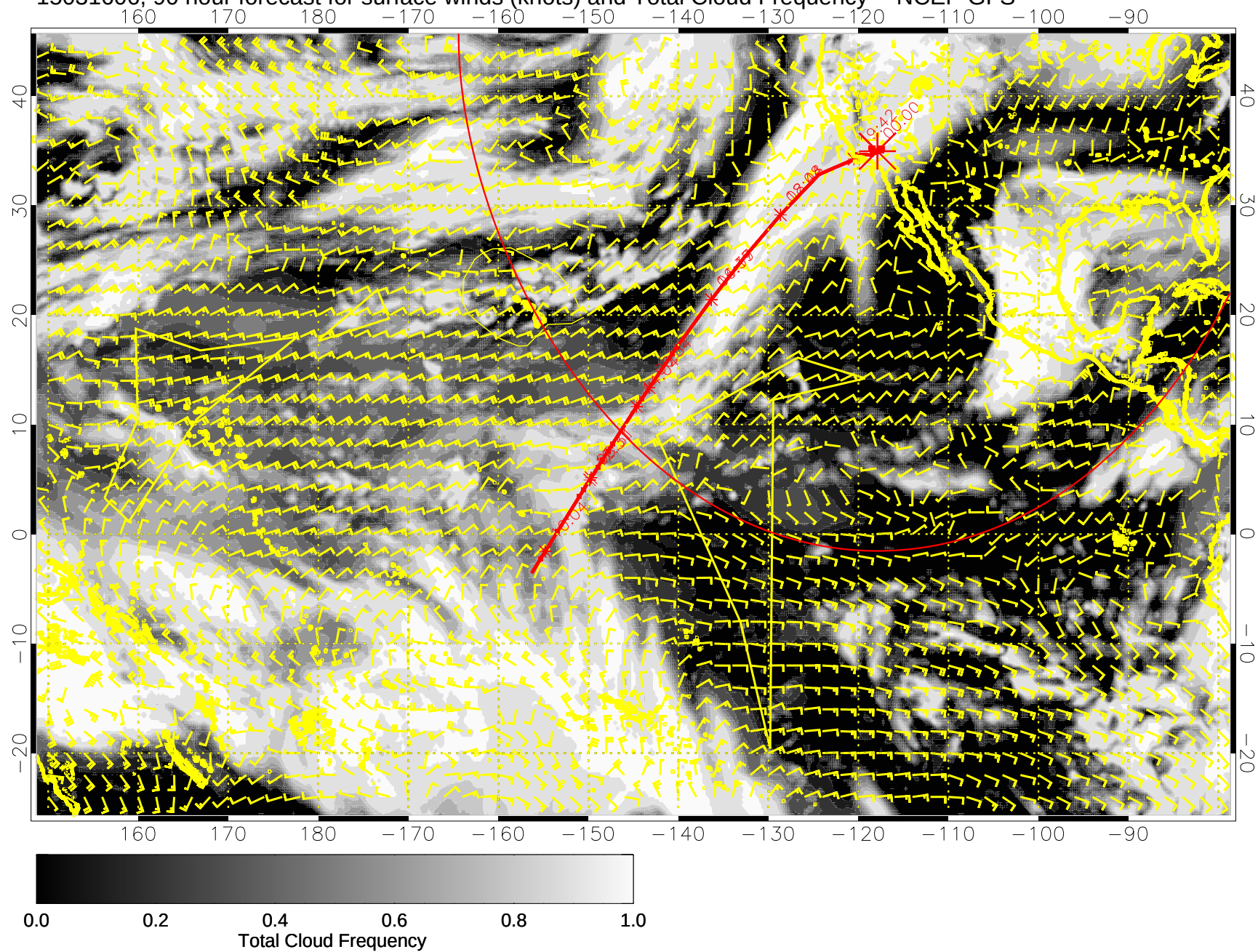
15031606, 90 hour forecast for surface winds (knots) and Total Cloud Frequency -- NCEP GFS
