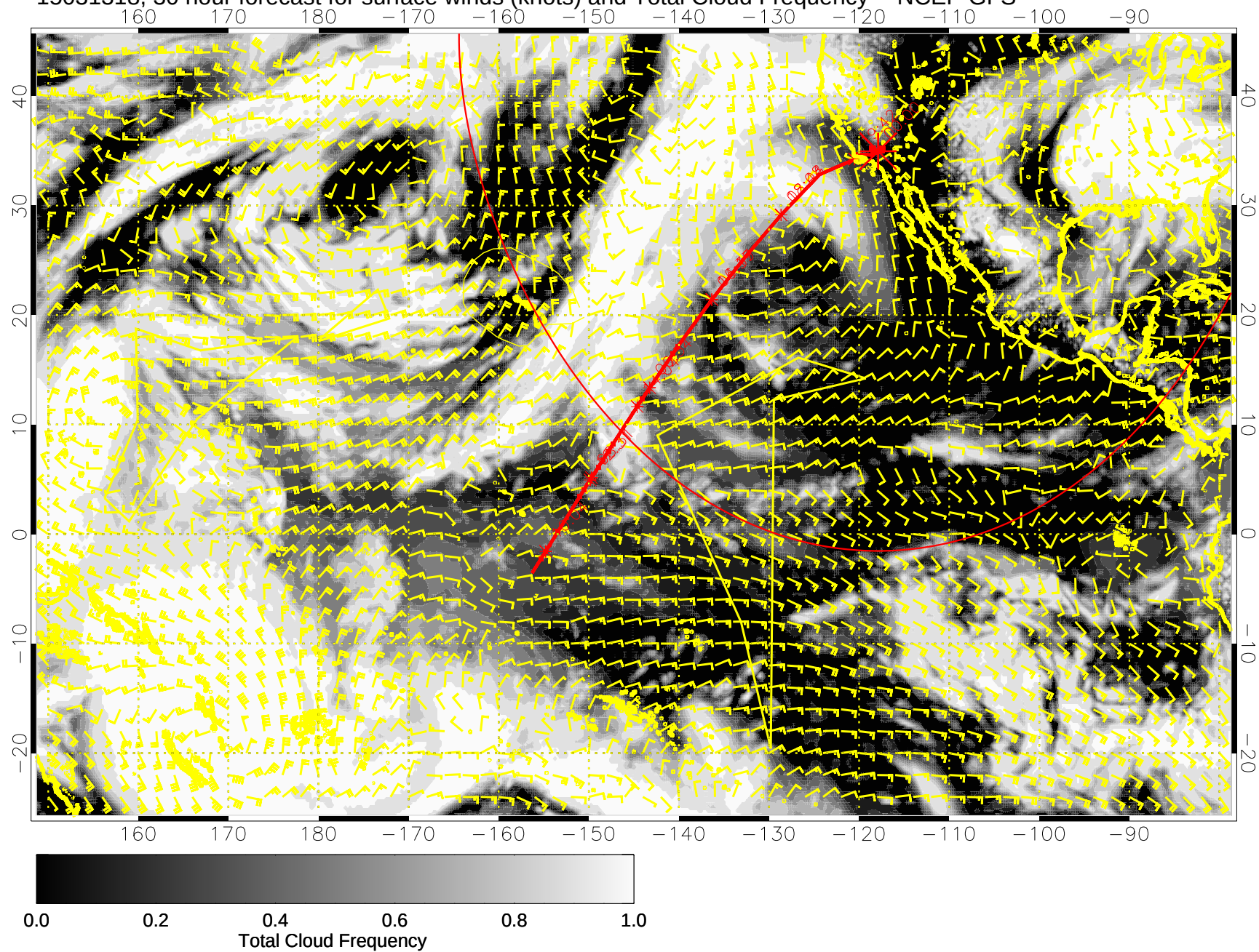
15031318, 30 hour forecast for surface winds (knots) and Total Cloud Frequency -- NCEP GFS
