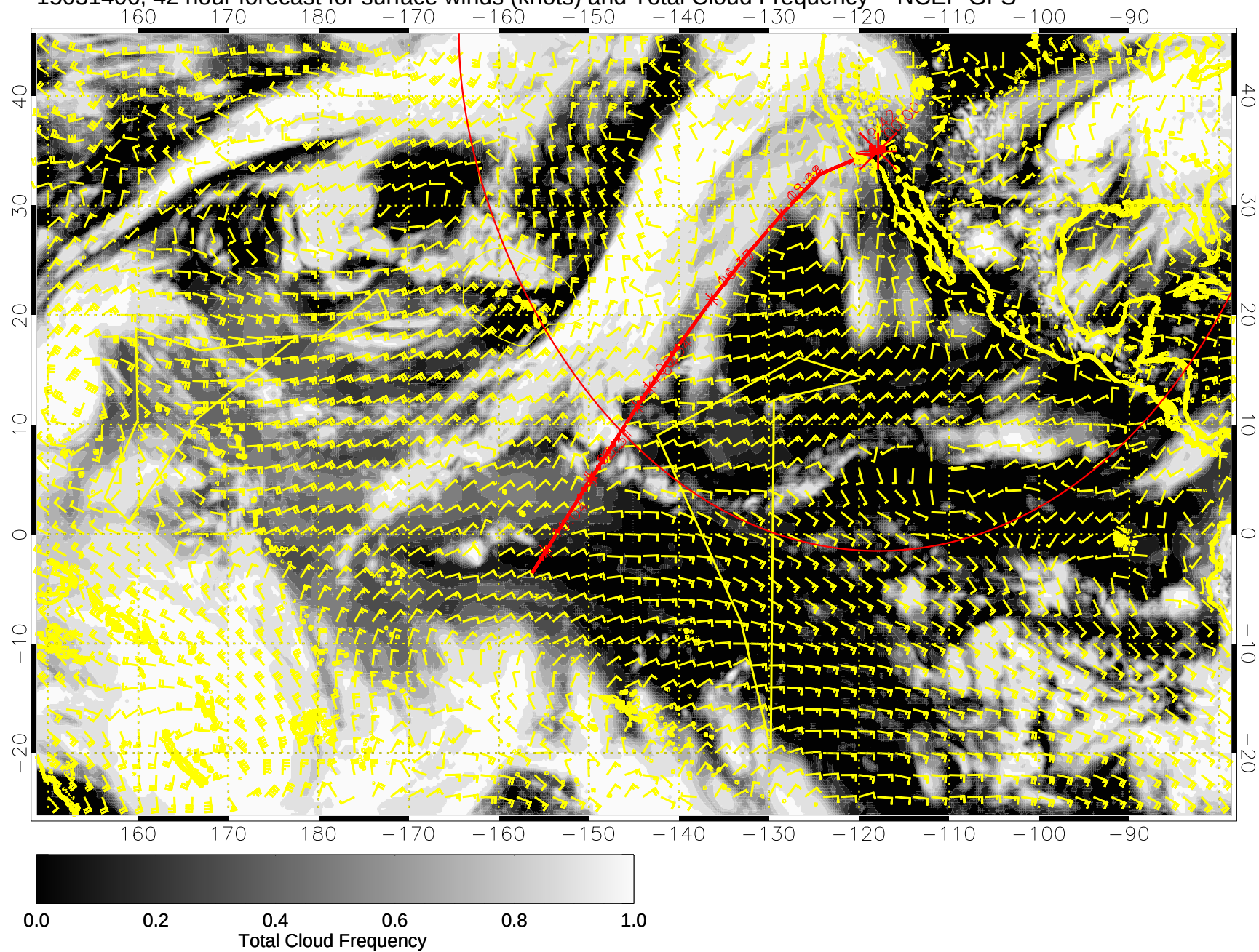
15031406, 42 hour forecast for surface winds (knots) and Total Cloud Frequency -- NCEP GFS
