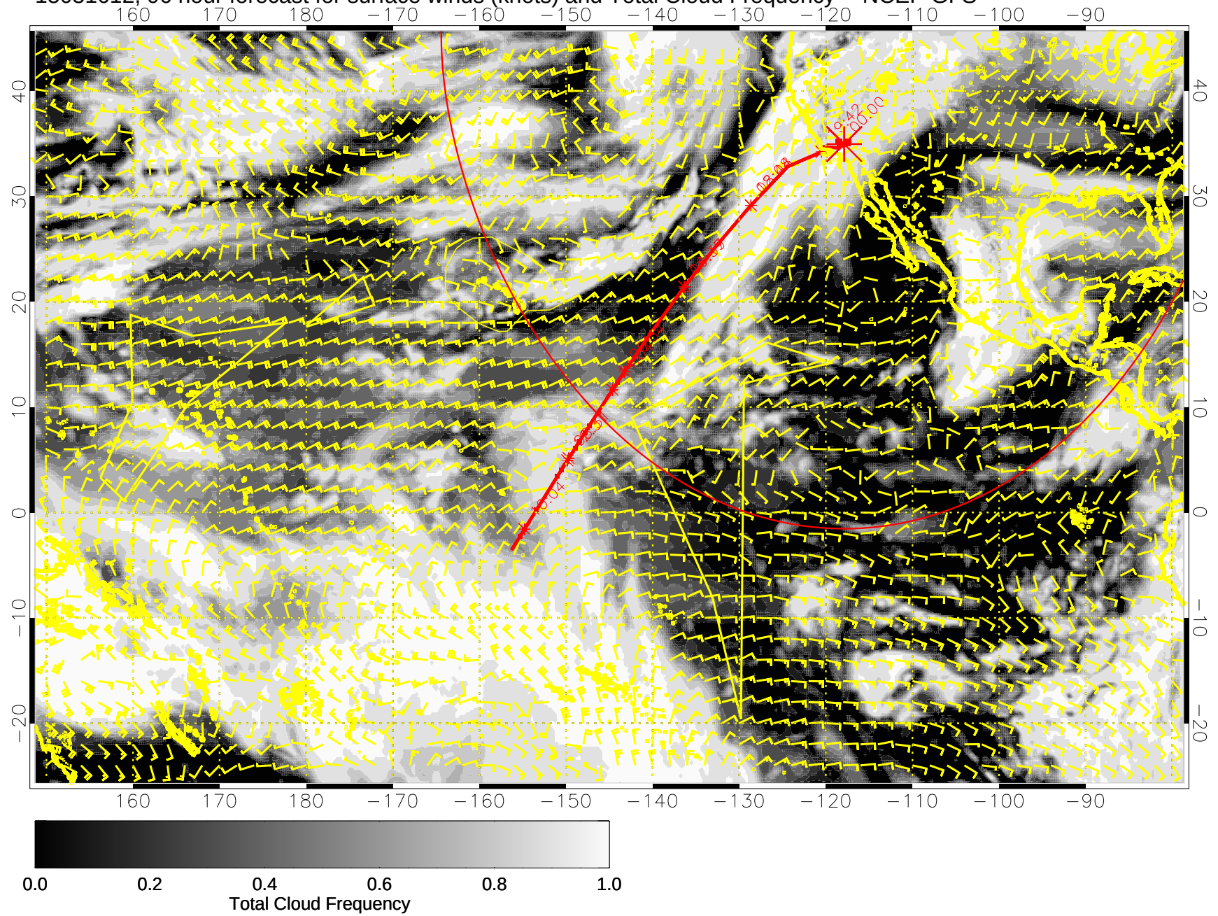
15031612, 96 hour forecast for surface winds (knots) and Total Cloud Frequency -- NCEP GFS
