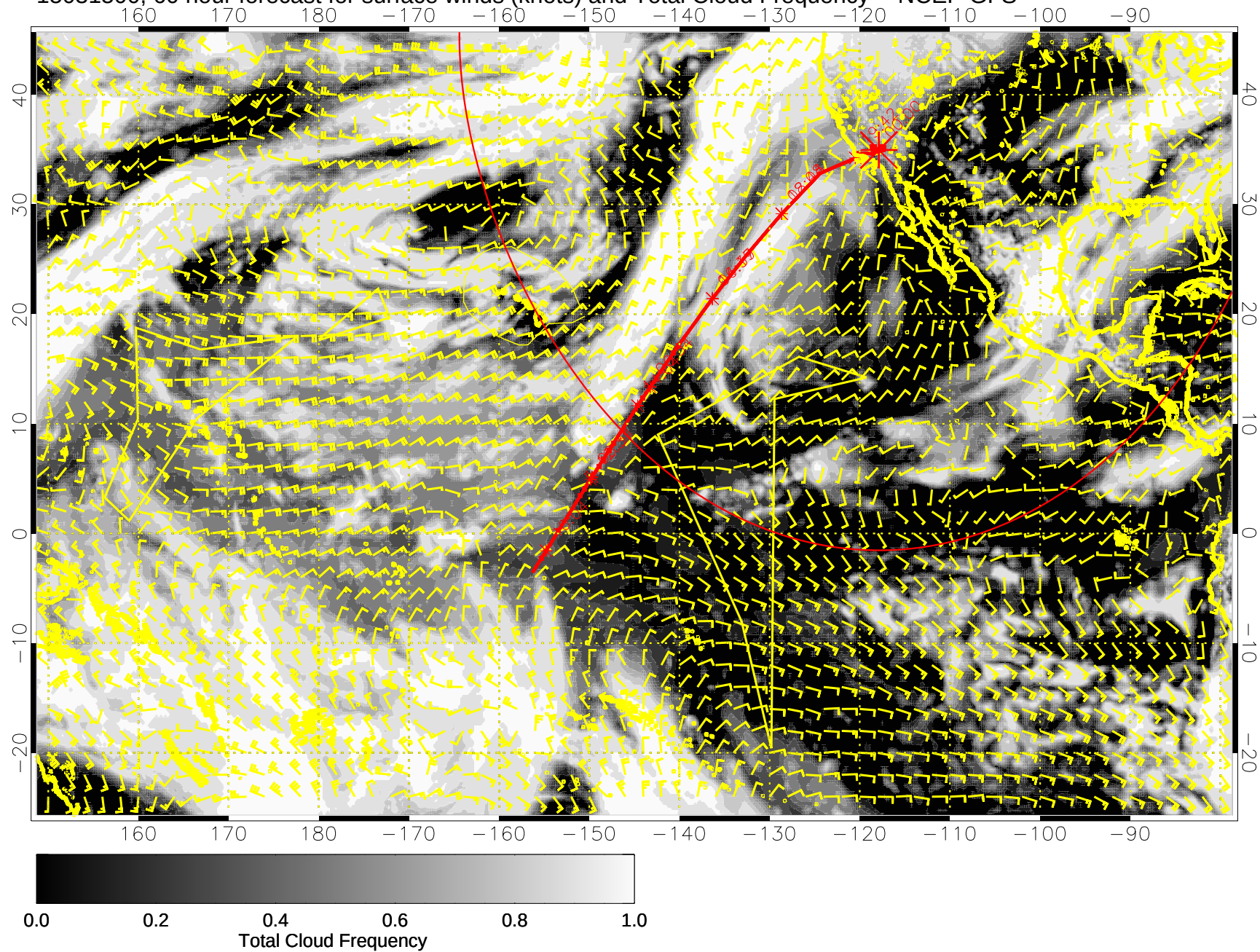
15031500, 60 hour forecast for surface winds (knots) and Total Cloud Frequency -- NCEP GFS
