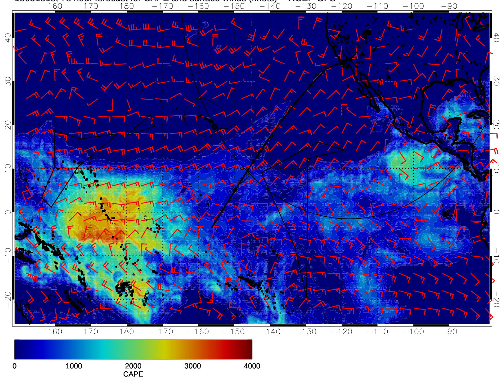
15031518, 78 hour forecast for CAPE and surface winds (knots) -- NCEP GFS
