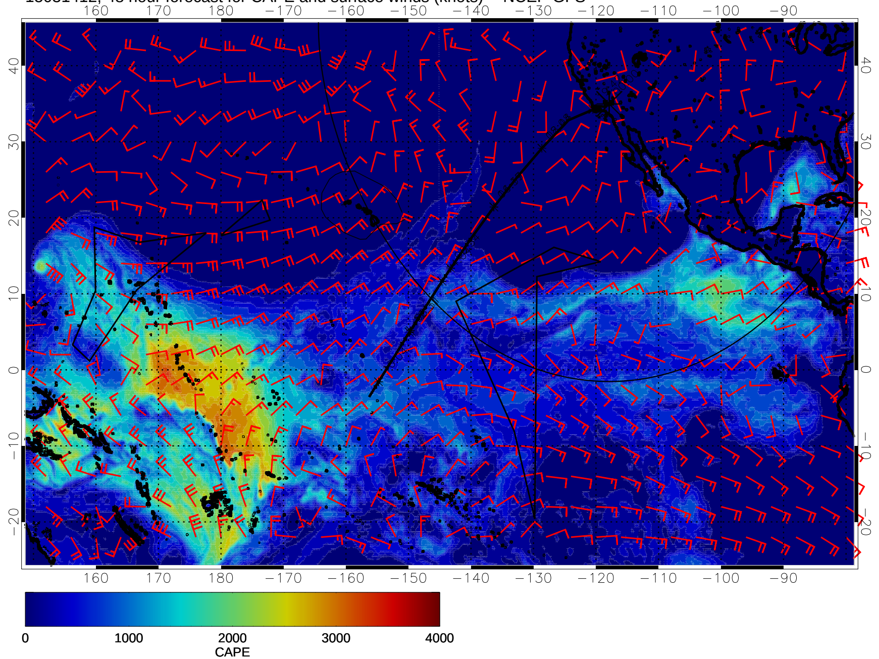
15031412, 48 hour forecast for CAPE and surface winds (knots) -- NCEP GFS
