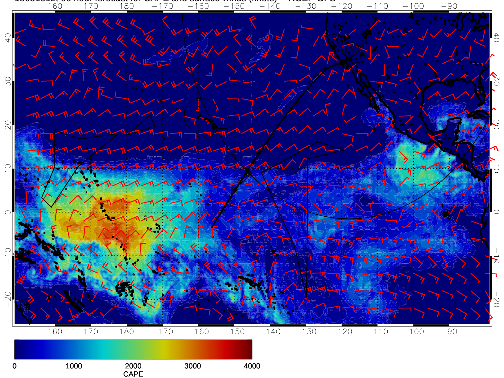
15031612, 96 hour forecast for CAPE and surface winds (knots) -- NCEP GFS
