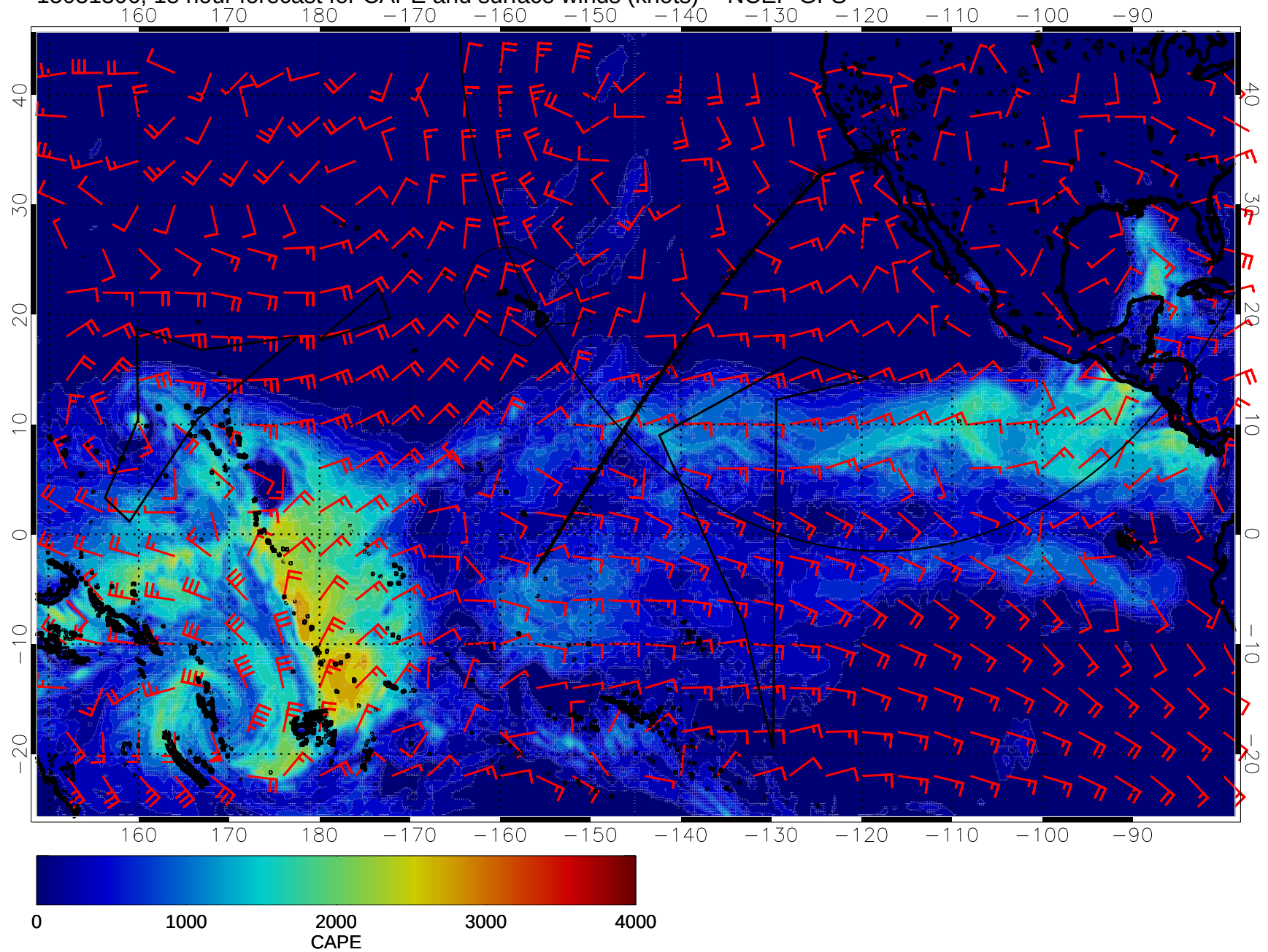
15031306, 18 hour forecast for CAPE and surface winds (knots) -- NCEP GFS
