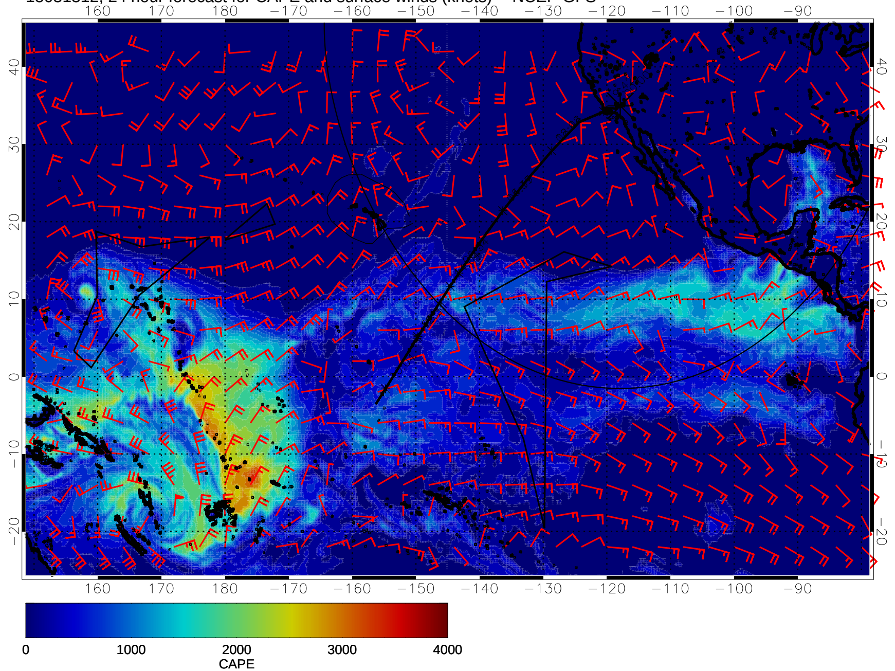
15031312, 24 hour forecast for CAPE and surface winds (knots) -- NCEP GFS
