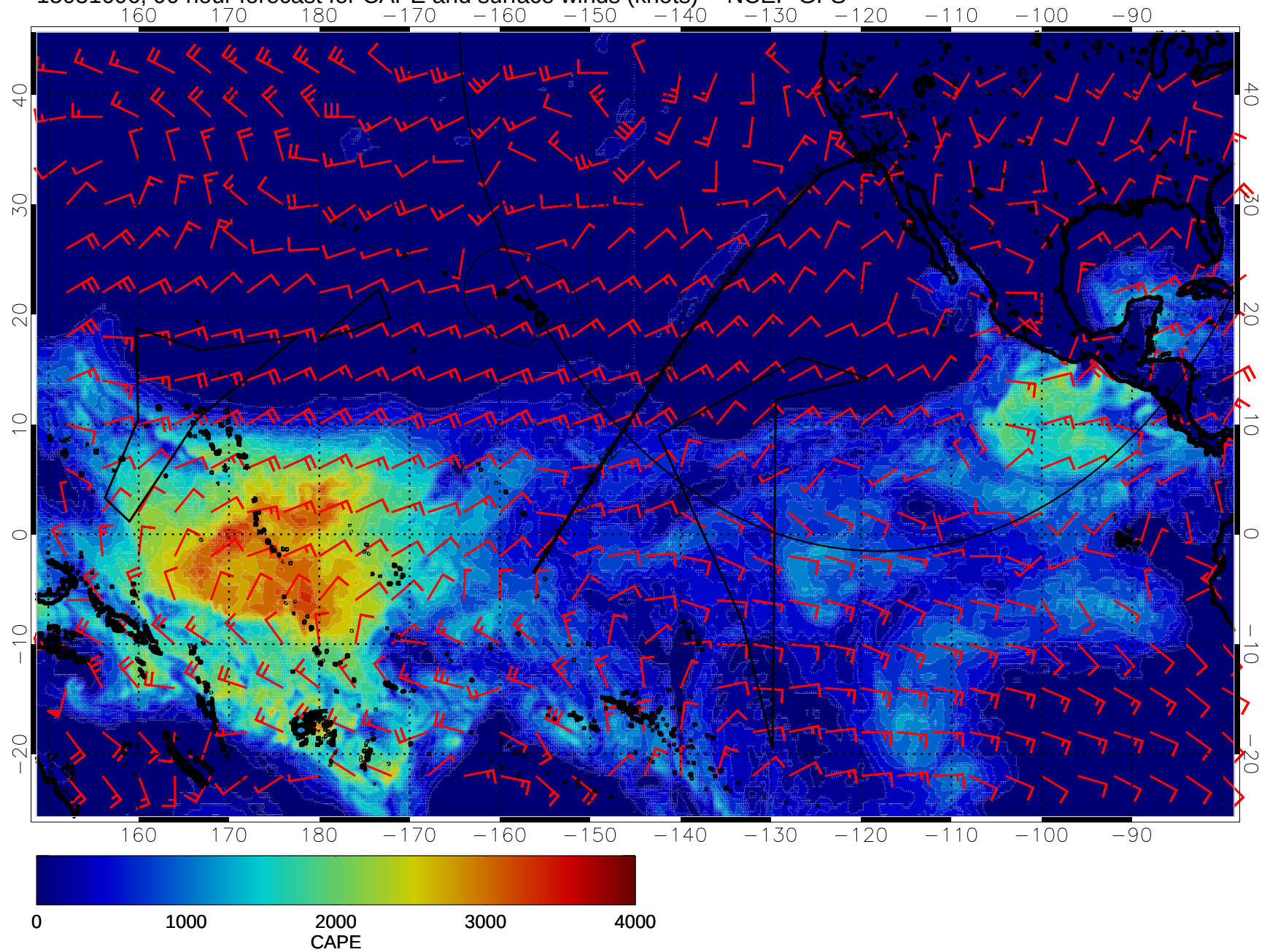
15031606, 90 hour forecast for CAPE and surface winds (knots) -- NCEP GFS
