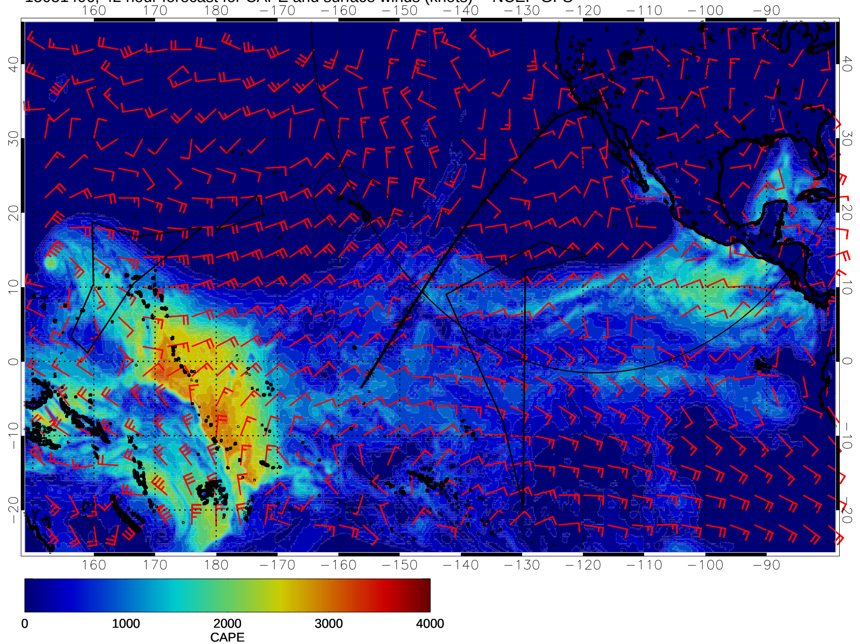
15031406, 42 hour forecast for CAPE and surface winds (knots) -- NCEP GFS
