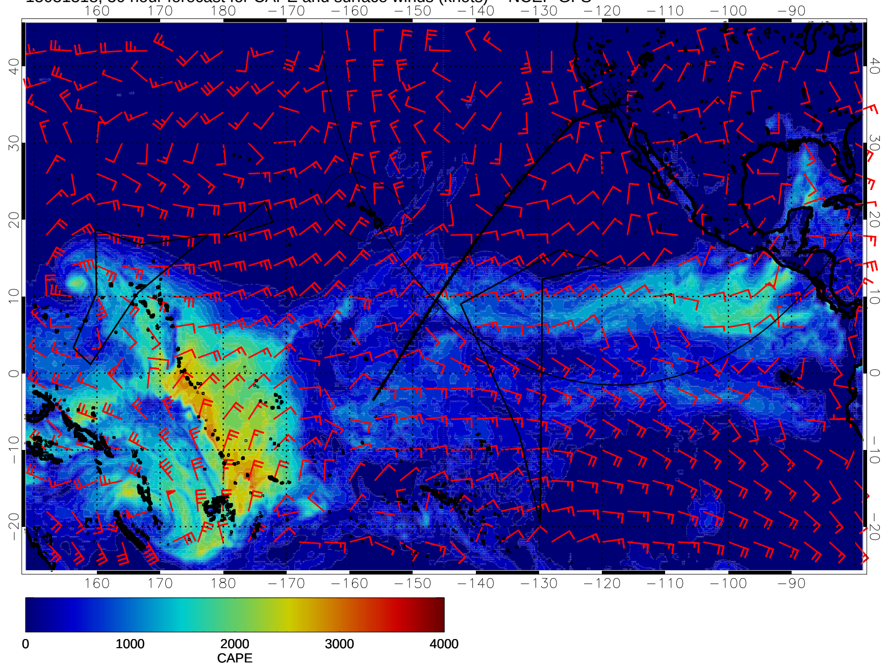
15031318, 30 hour forecast for CAPE and surface winds (knots) -- NCEP GFS
