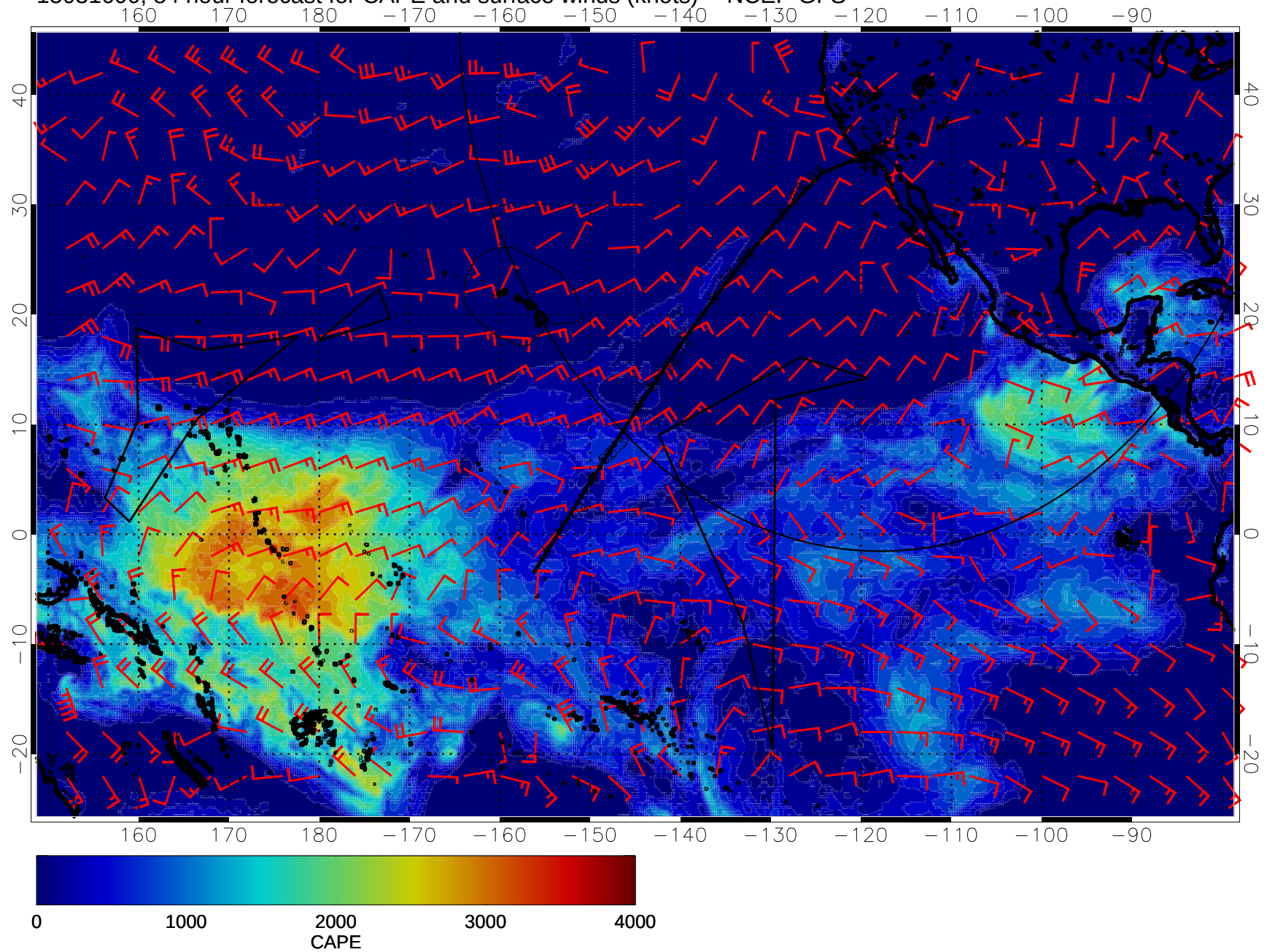
15031600, 84 hour forecast for CAPE and surface winds (knots) -- NCEP GFS
