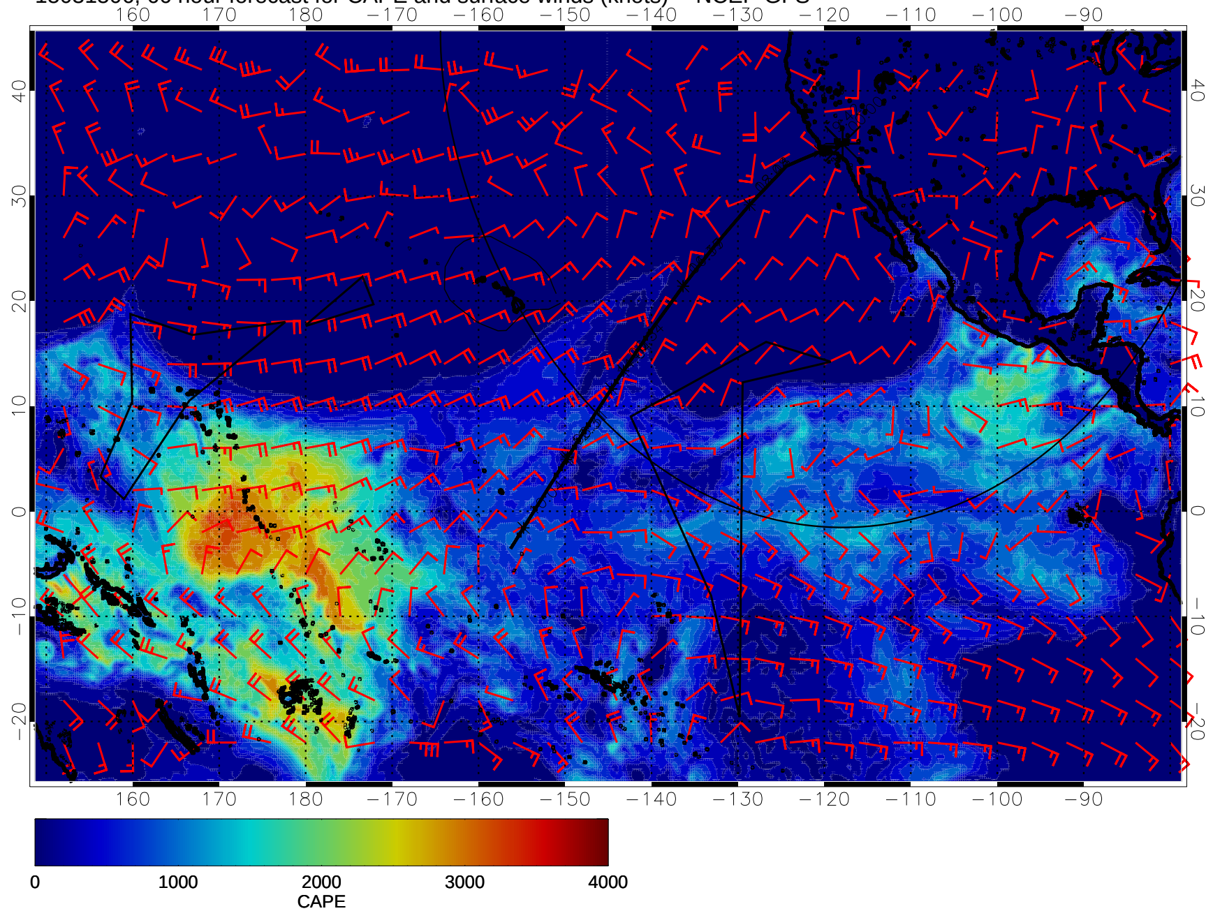
15031506, 66 hour forecast for CAPE and surface winds (knots) -- NCEP GFS
