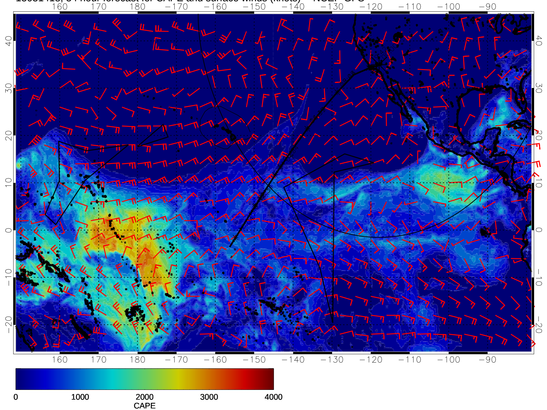
15031418, 54 hour forecast for CAPE and surface winds (knots) -- NCEP GFS
