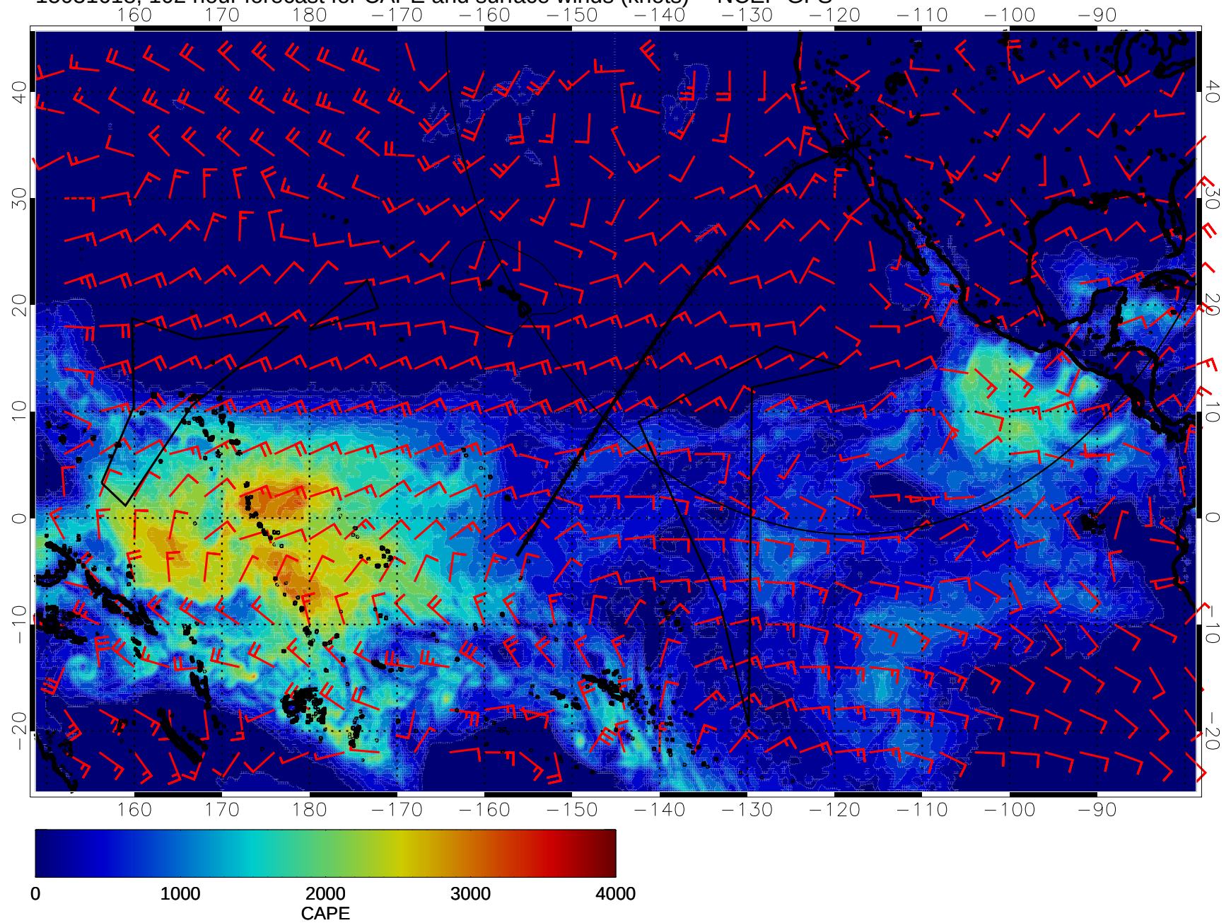
15031618, 102 hour forecast for CAPE and surface winds (knots) -- NCEP GFS
