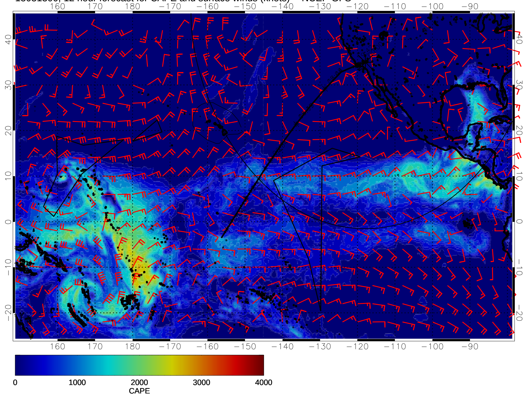
15031300, 12 hour forecast for CAPE and surface winds (knots) -- NCEP GFS
