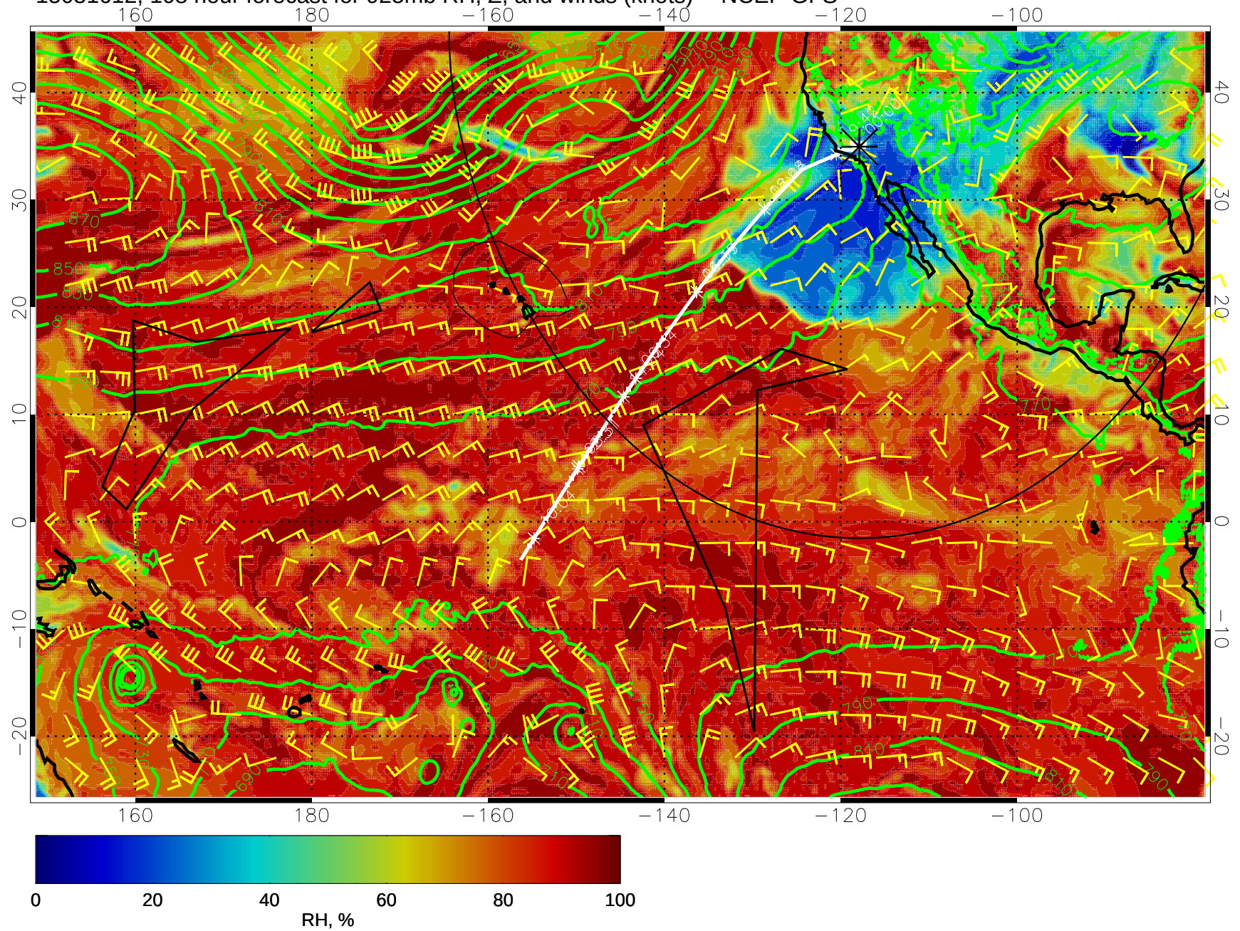
15031612, 108 hour forecast for 925mb RH, Z, and winds (knots) -- NCEP GFS
