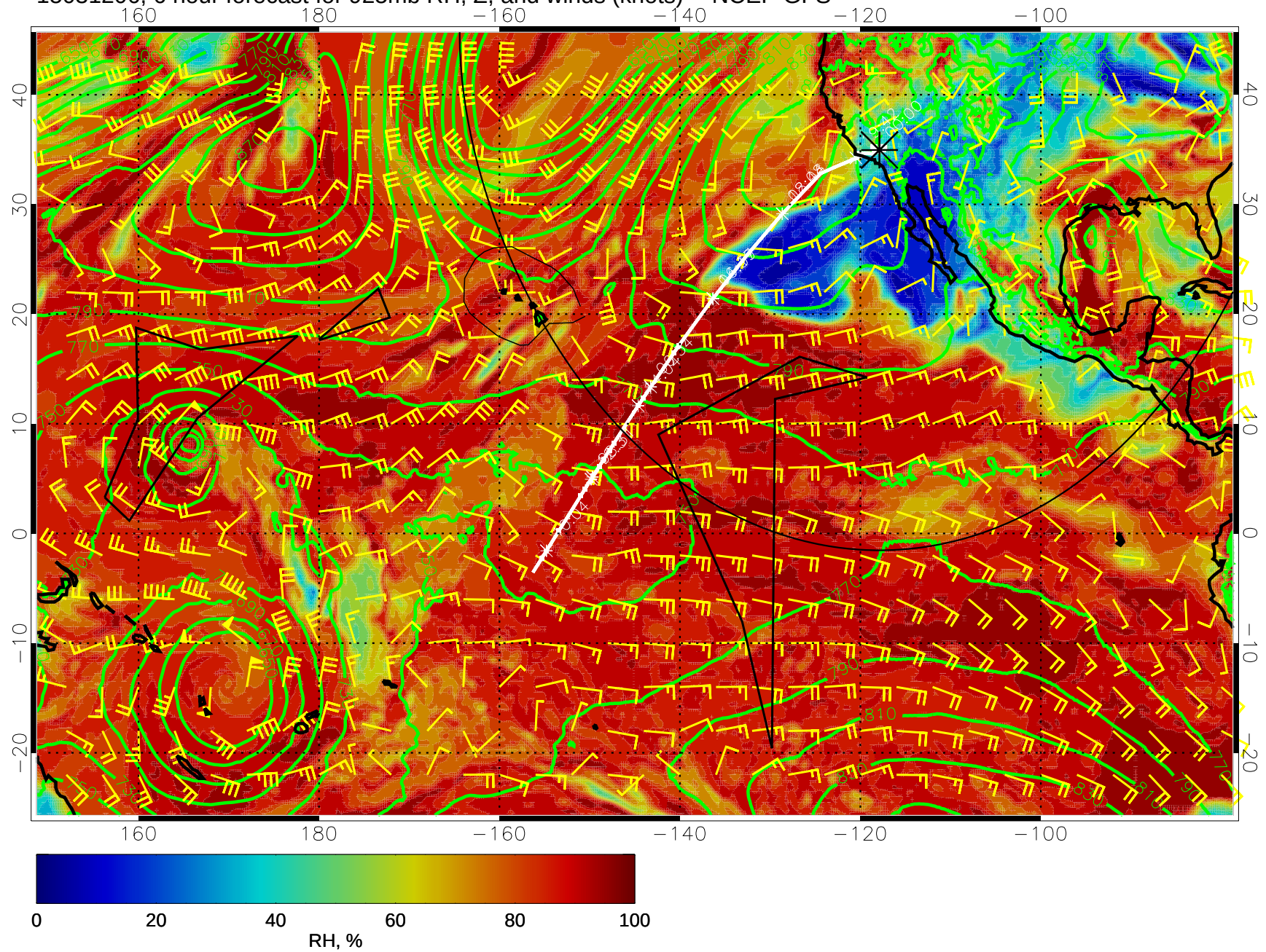
15031206, 6 hour forecast for 925mb RH, Z, and winds (knots) -- NCEP GFS
