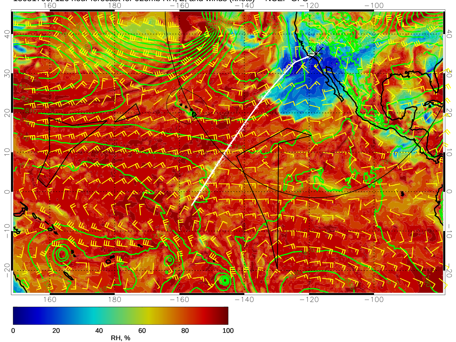
15031706, 126 hour forecast for 925mb RH, Z, and winds (knots) -- NCEP GFS
