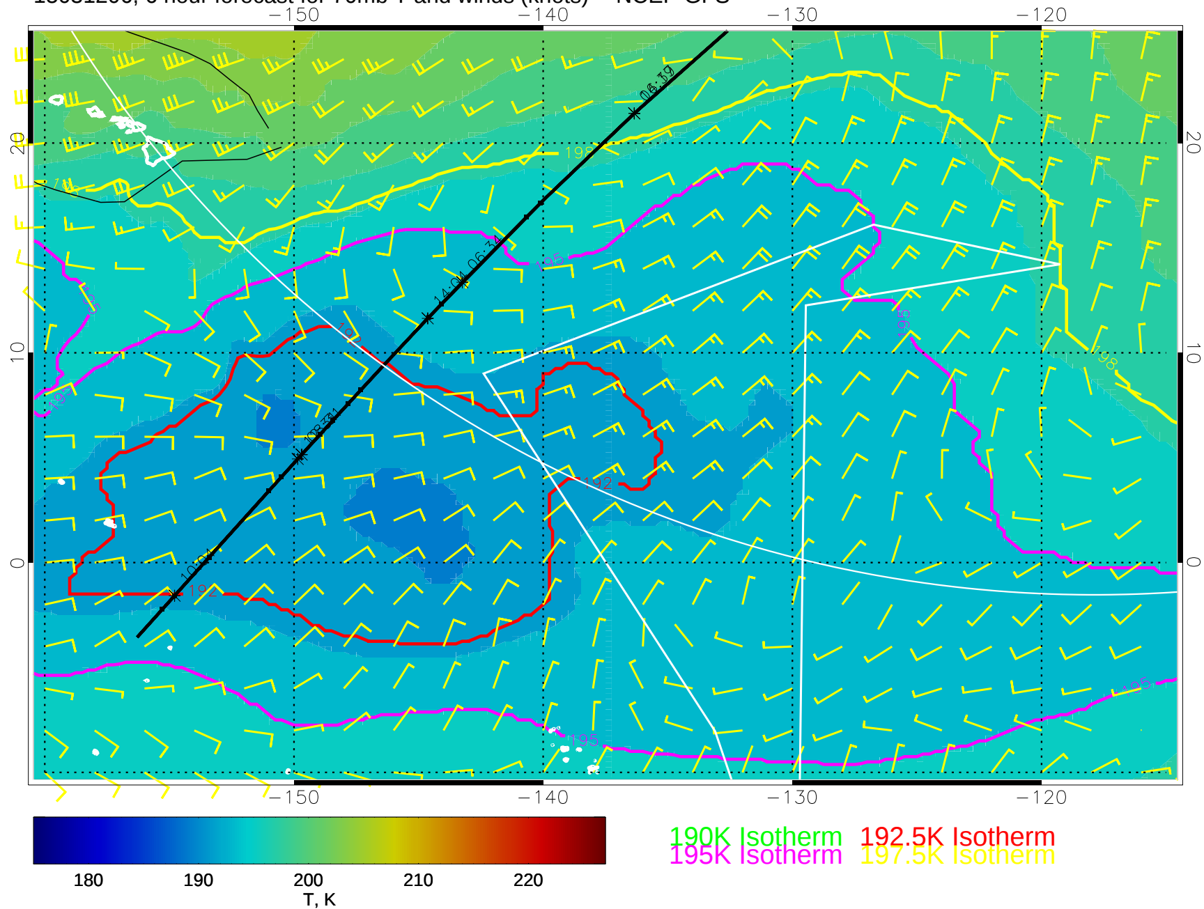
15031206, 6 hour forecast for 70mb T and winds (knots) -- NCEP GFS
