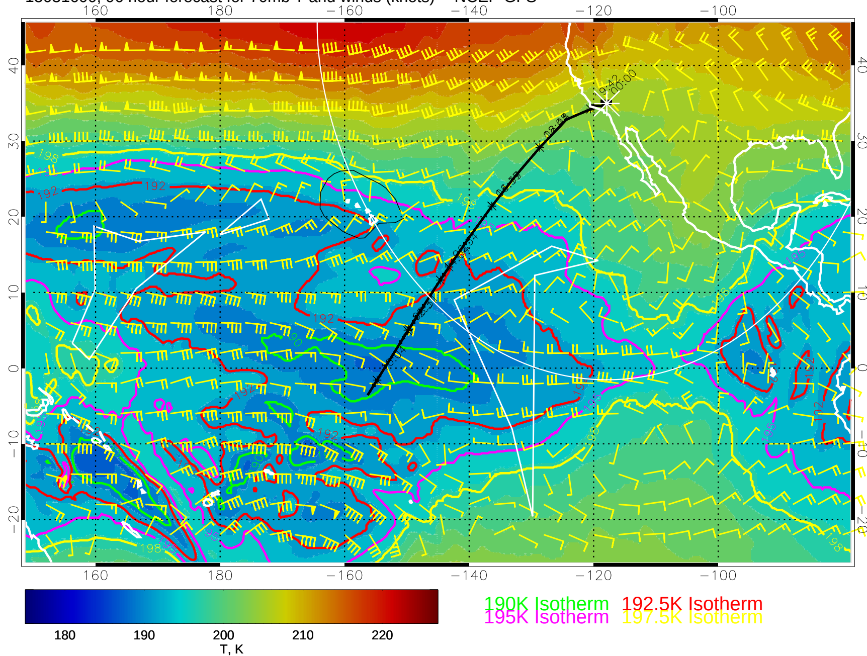
15031600, 96 hour forecast for 70mb T and winds (knots) -- NCEP GFS
