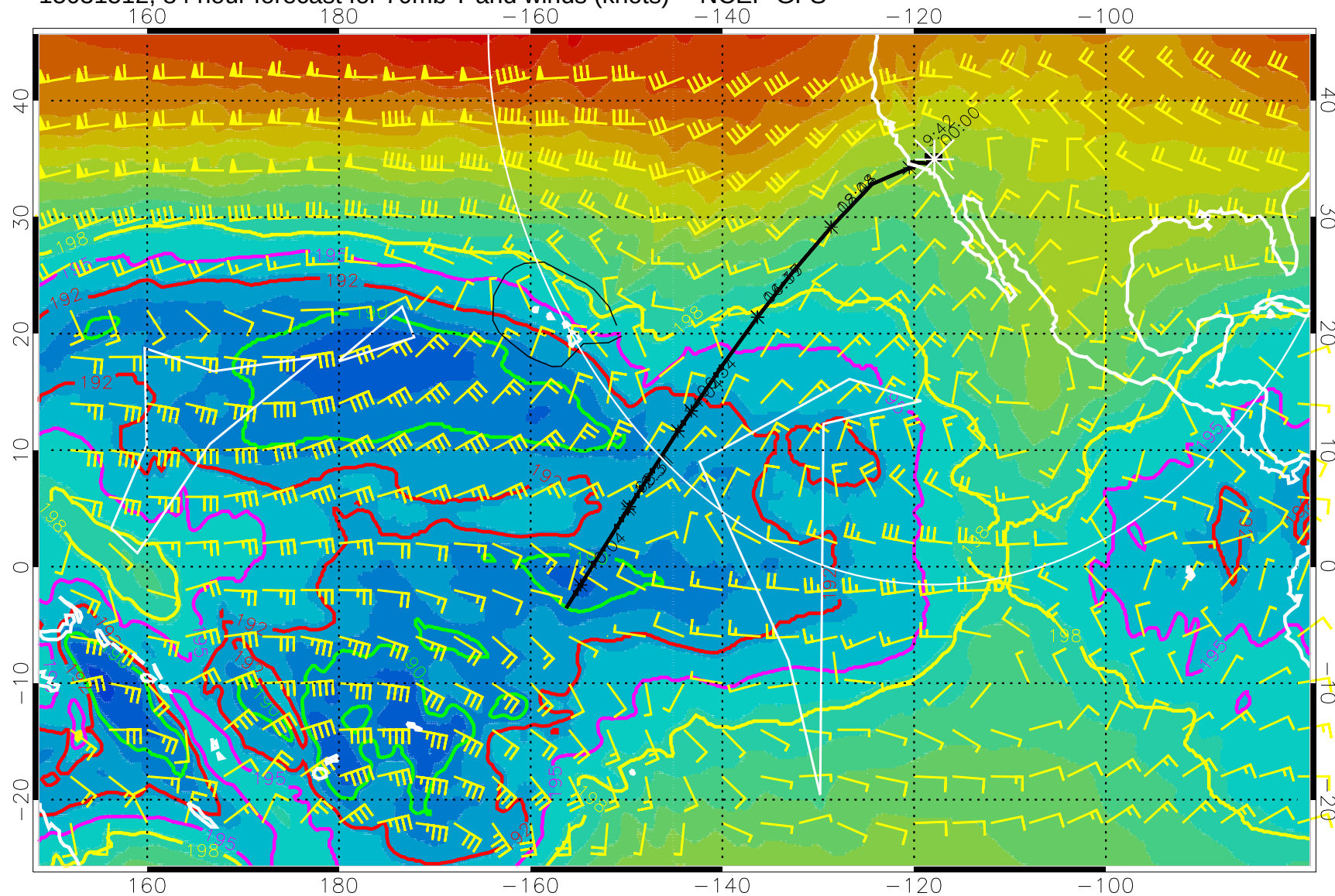
15031512, 84 hour forecast for 70mb T and winds (knots) -- NCEP GFS
