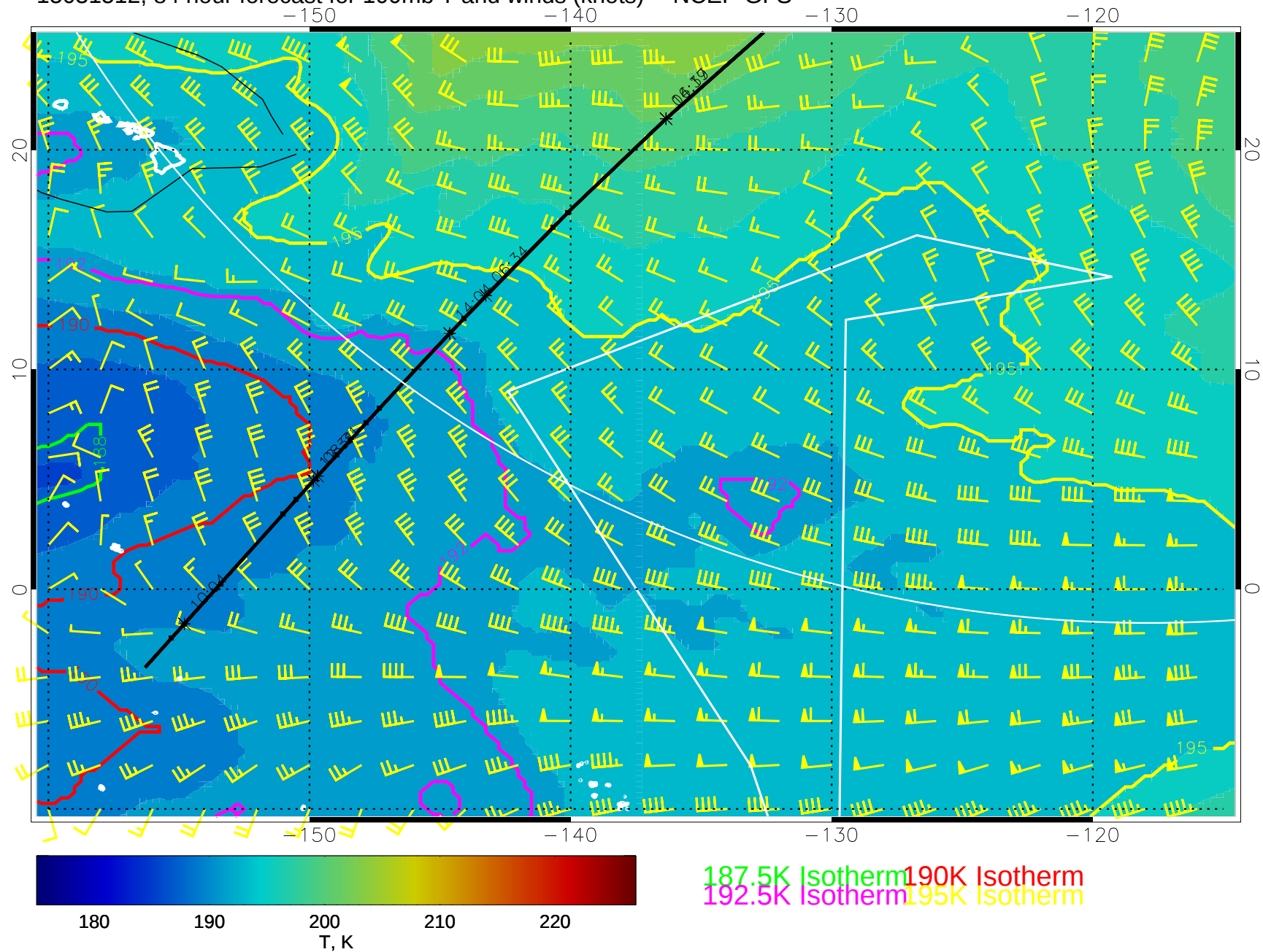
15031512, 84 hour forecast for 100mb T and winds (knots) -- NCEP GFS
