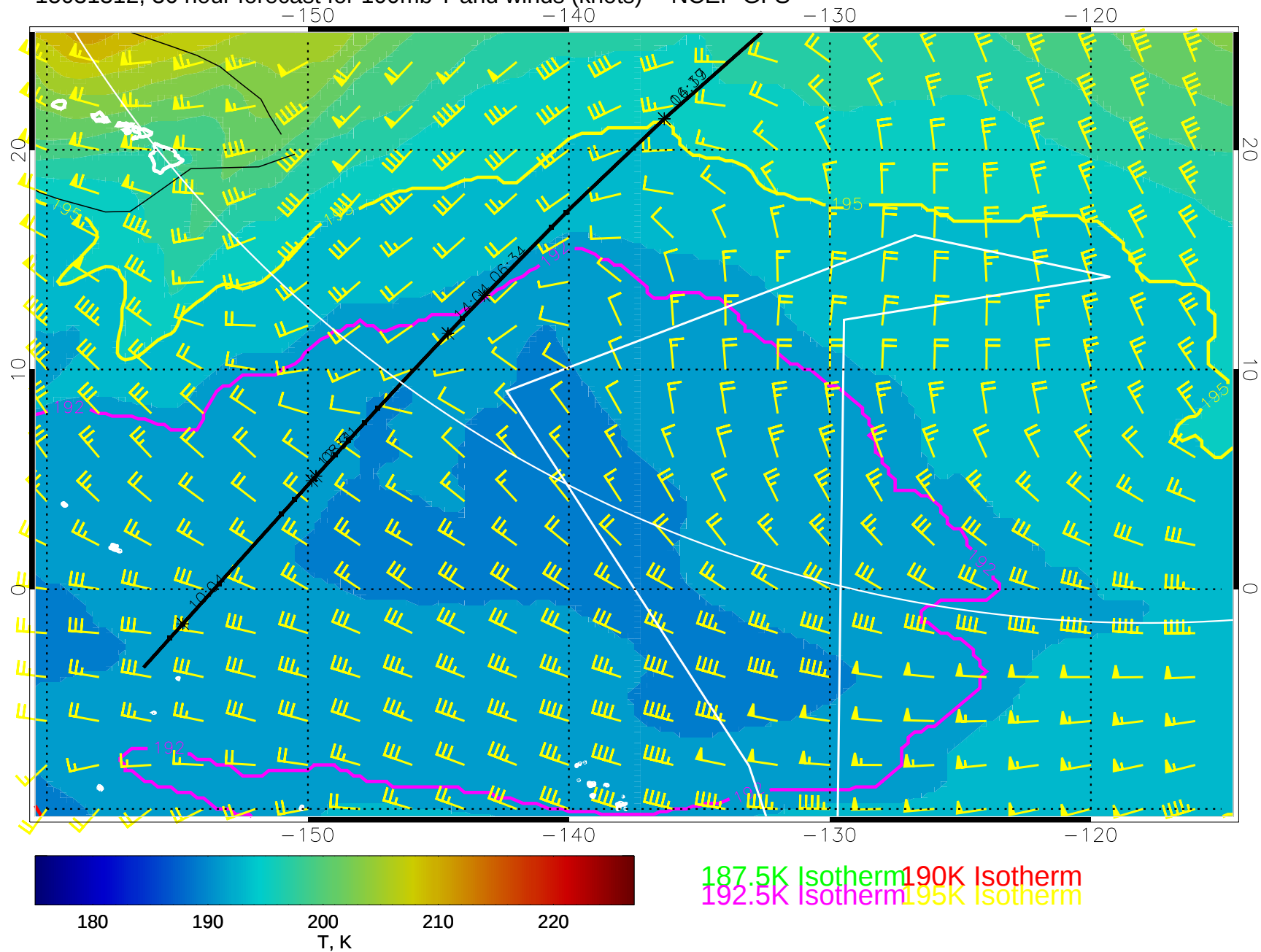
15031312, 36 hour forecast for 100mb T and winds (knots) -- NCEP GFS
