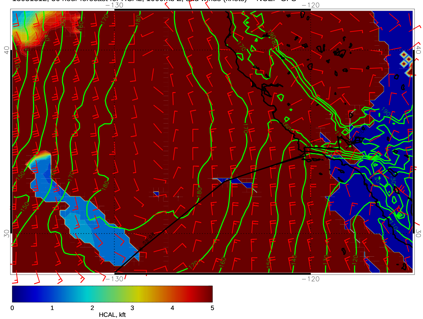
15031312, 36 hour forecast for HCAL, 1000mb Z, and winds (knots) -- NCEP GFS
