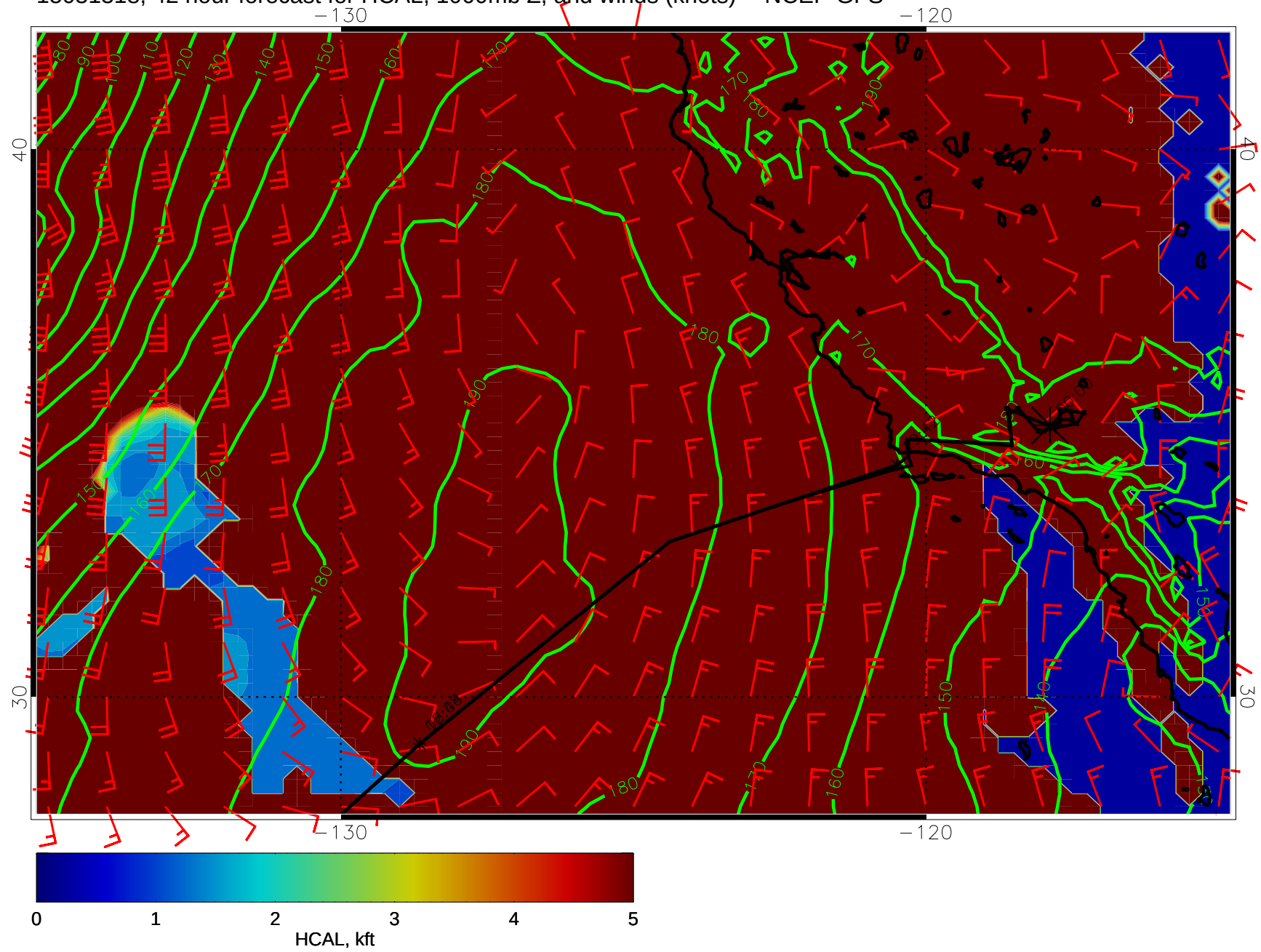
15031318, 42 hour forecast for HCAL, 1000mb Z, and winds (knots) -- NCEP GFS
