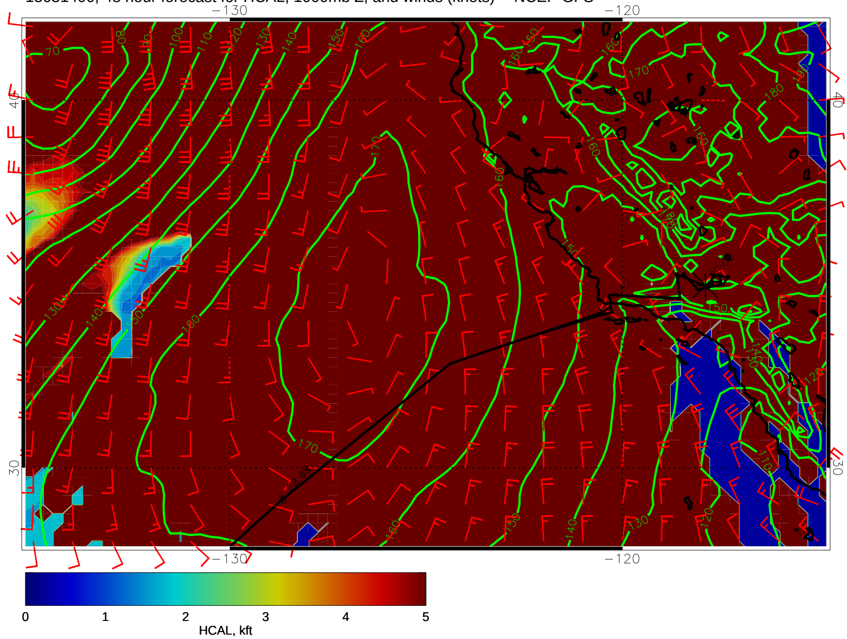
15031400, 48 hour forecast for HCAL, 1000mb Z, and winds (knots) -- NCEP GFS
