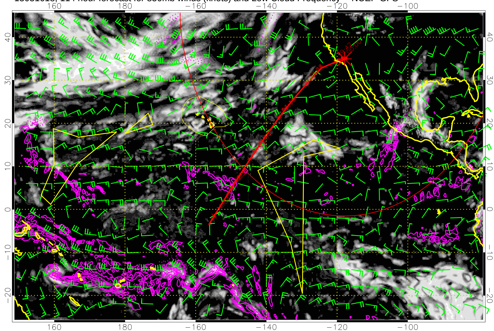
15031618, 114 hour forecast for 850mb winds (knots) and Low Cloud Frequency -- NCEP GFS
