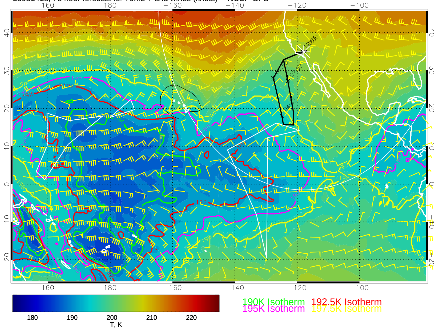
15031418, 78 hour forecast for 70mb T and winds (knots) -- NCEP GFS
