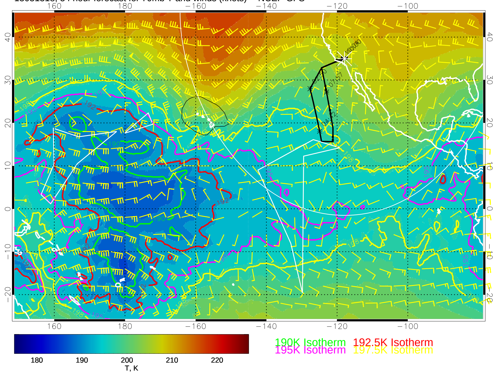
15031318, 54 hour forecast for 70mb T and winds (knots) -- NCEP GFS
