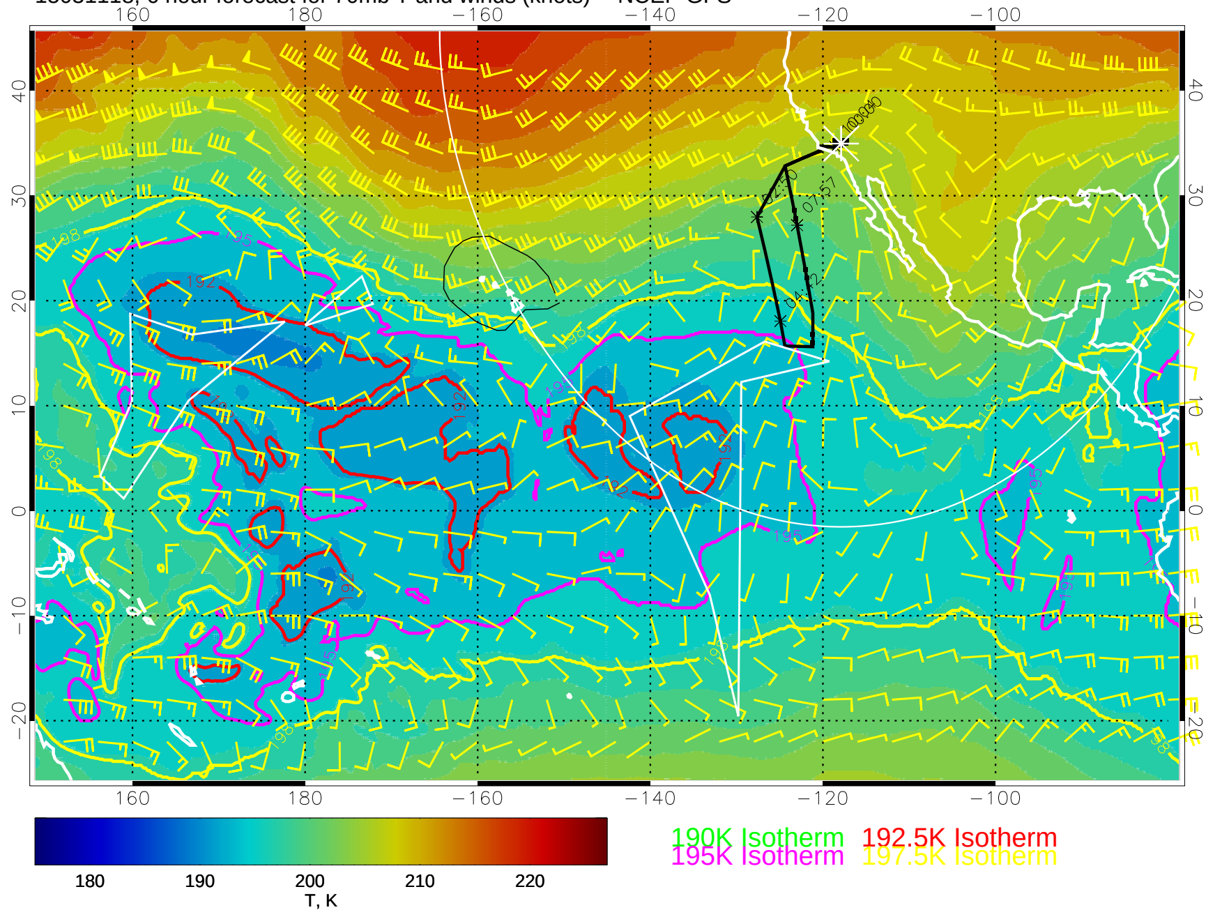
15031118, 6 hour forecast for 70mb T and winds (knots) -- NCEP GFS
