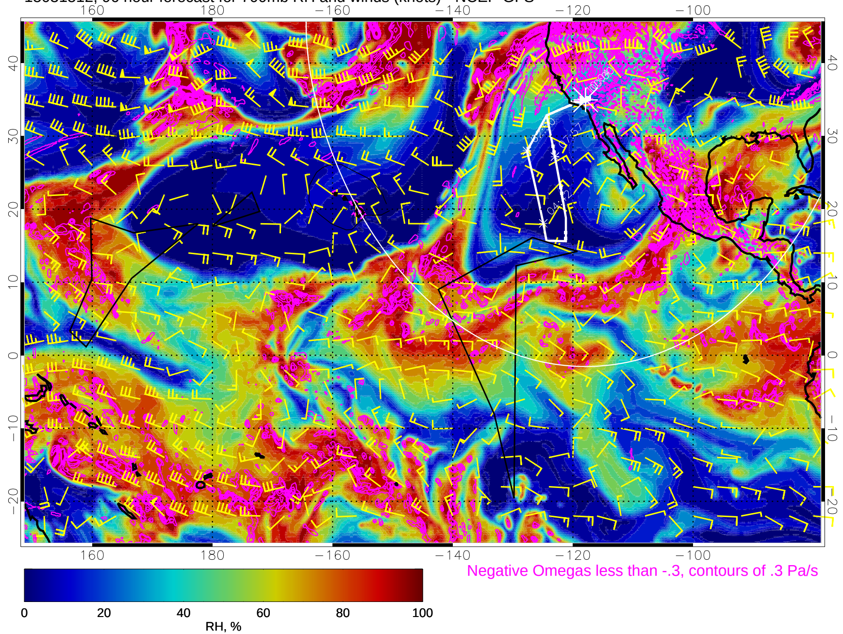
15031512, 96 hour forecast for 700mb RH and winds (knots) - NCEP GFS
