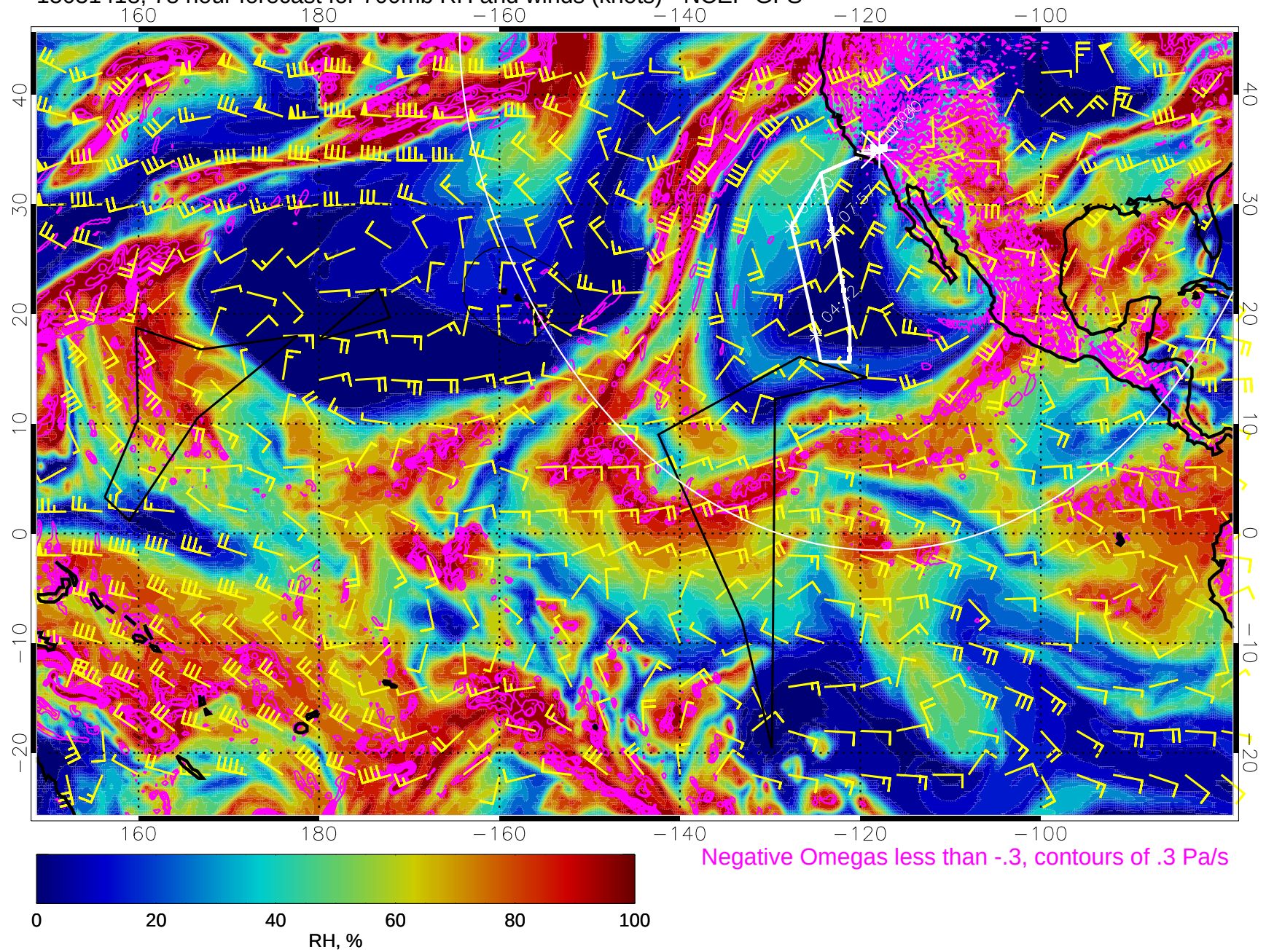
15031418, 78 hour forecast for 700mb RH and winds (knots) - NCEP GFS
