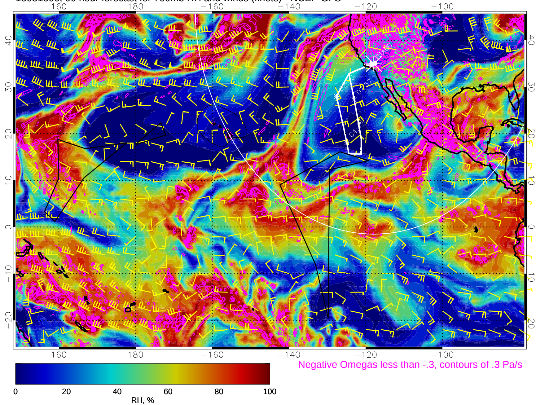
15031506, 90 hour forecast for 700mb RH and winds (knots) - NCEP GFS
