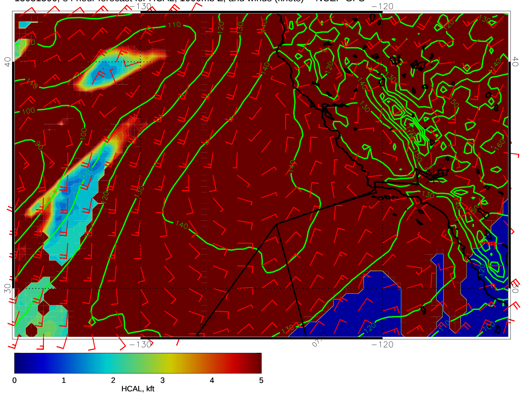
15031500, 84 hour forecast for HCAL, 1000mb Z, and winds (knots) -- NCEP GFS
