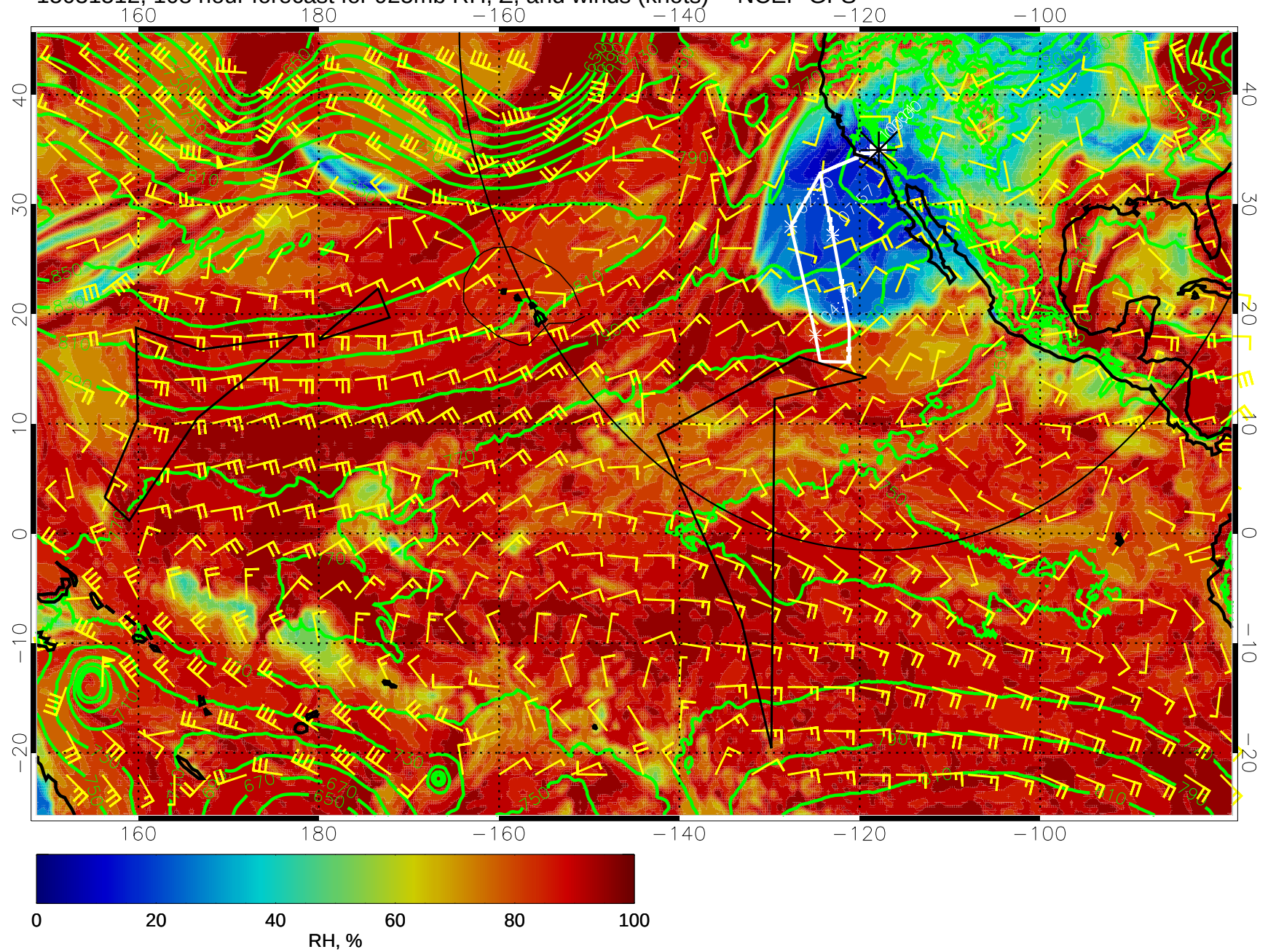
15031512, 108 hour forecast for 925mb RH, Z, and winds (knots) -- NCEP GFS
