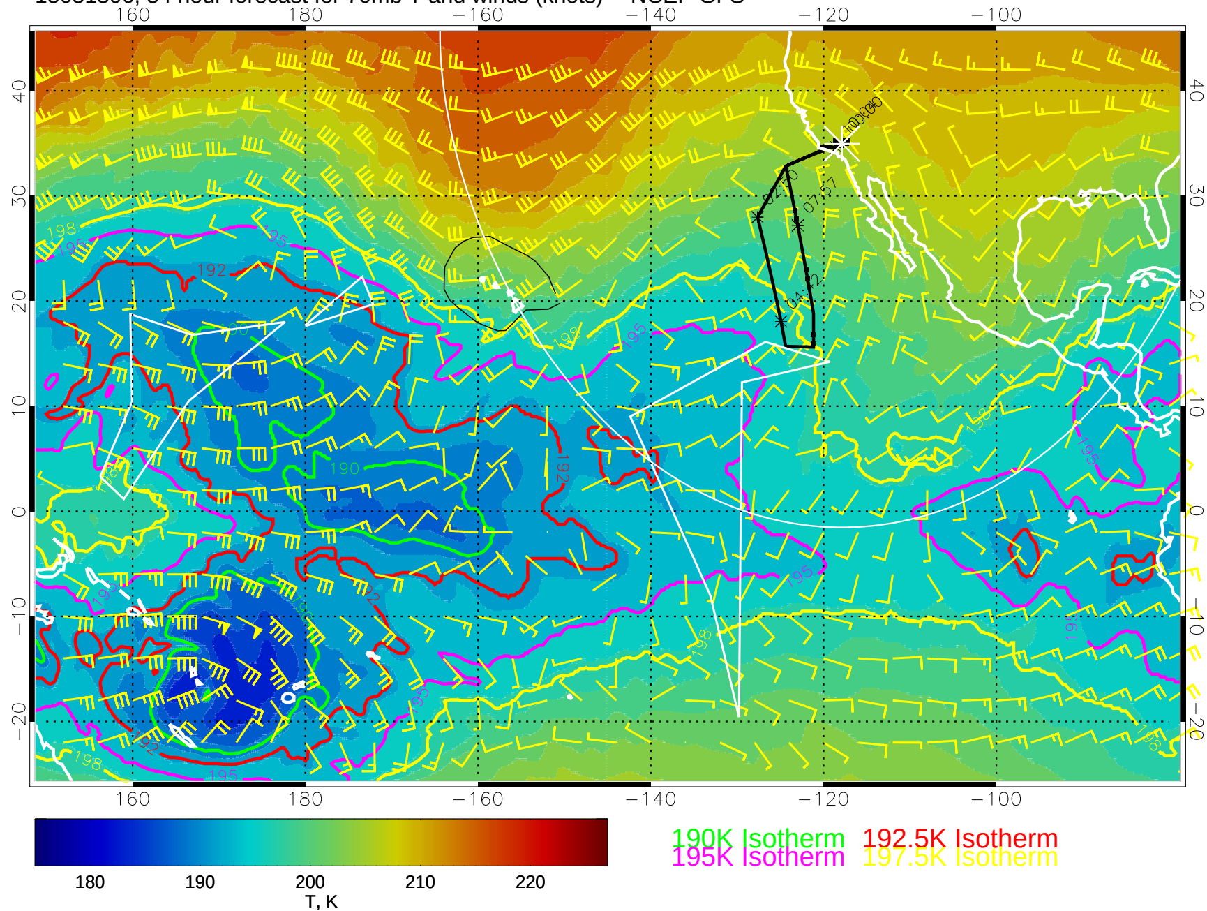
15031306, 54 hour forecast for 70mb T and winds (knots) -- NCEP GFS
