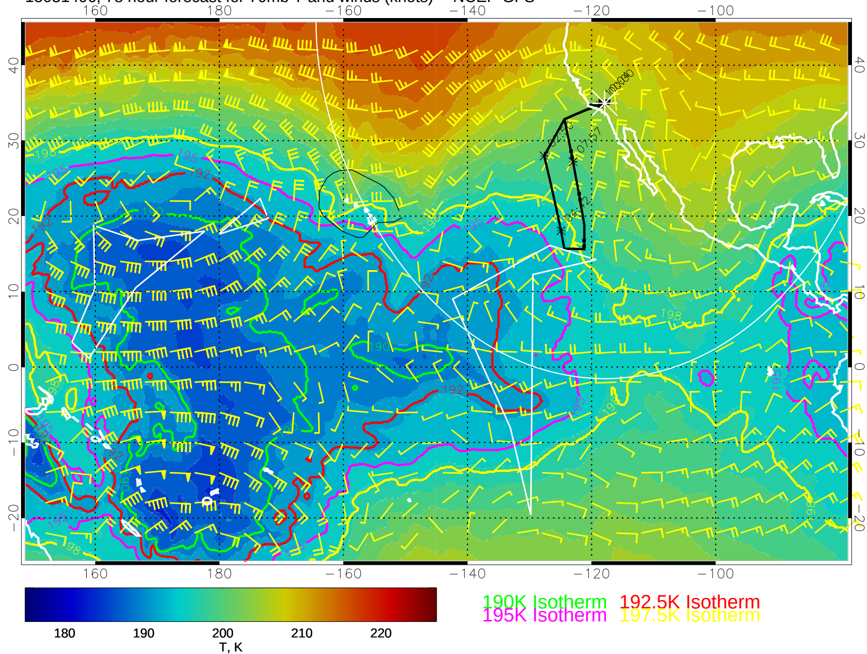
15031406, 78 hour forecast for 70mb T and winds (knots) -- NCEP GFS
