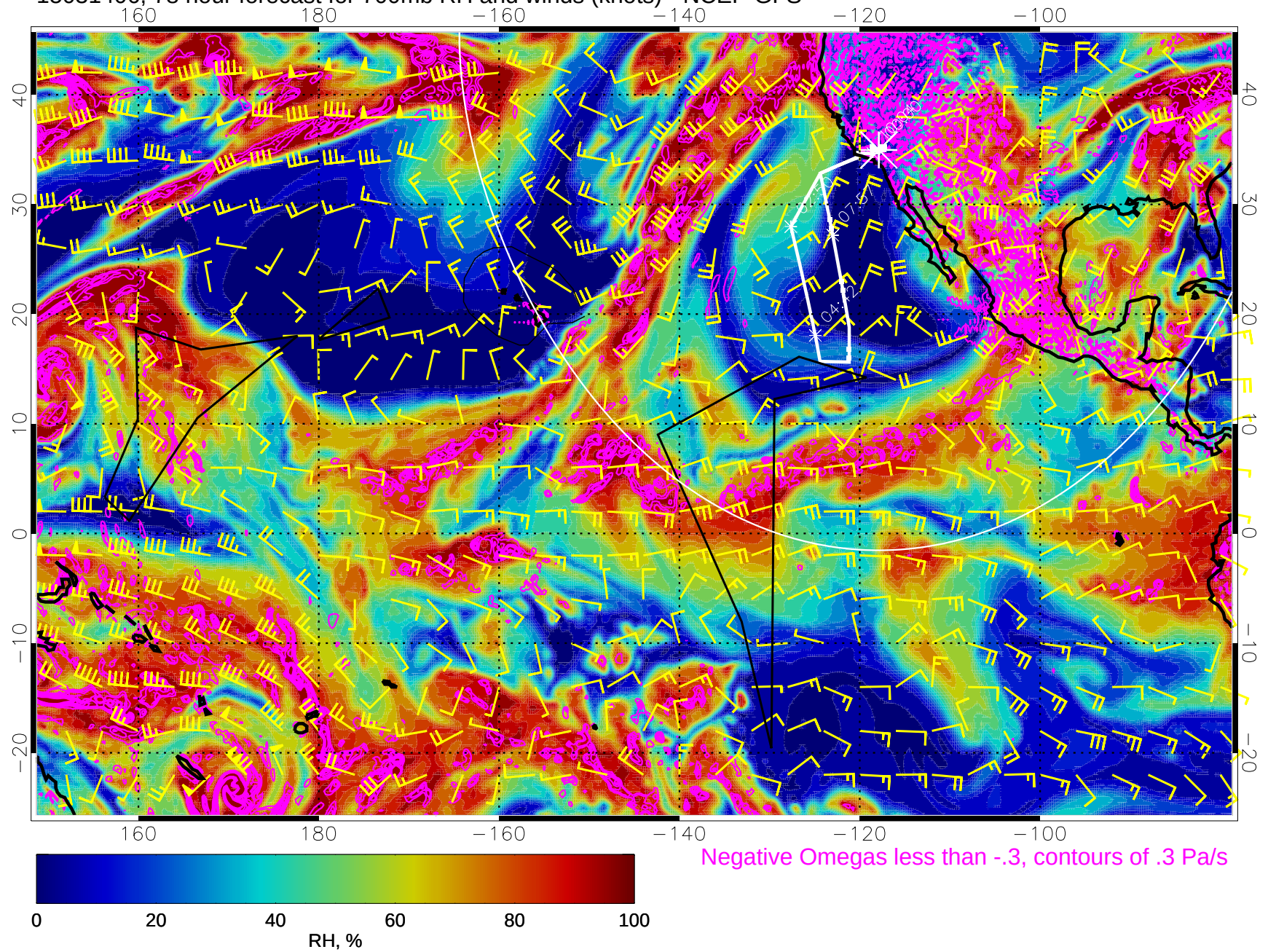
15031406, 78 hour forecast for 700mb RH and winds (knots) - NCEP GFS
