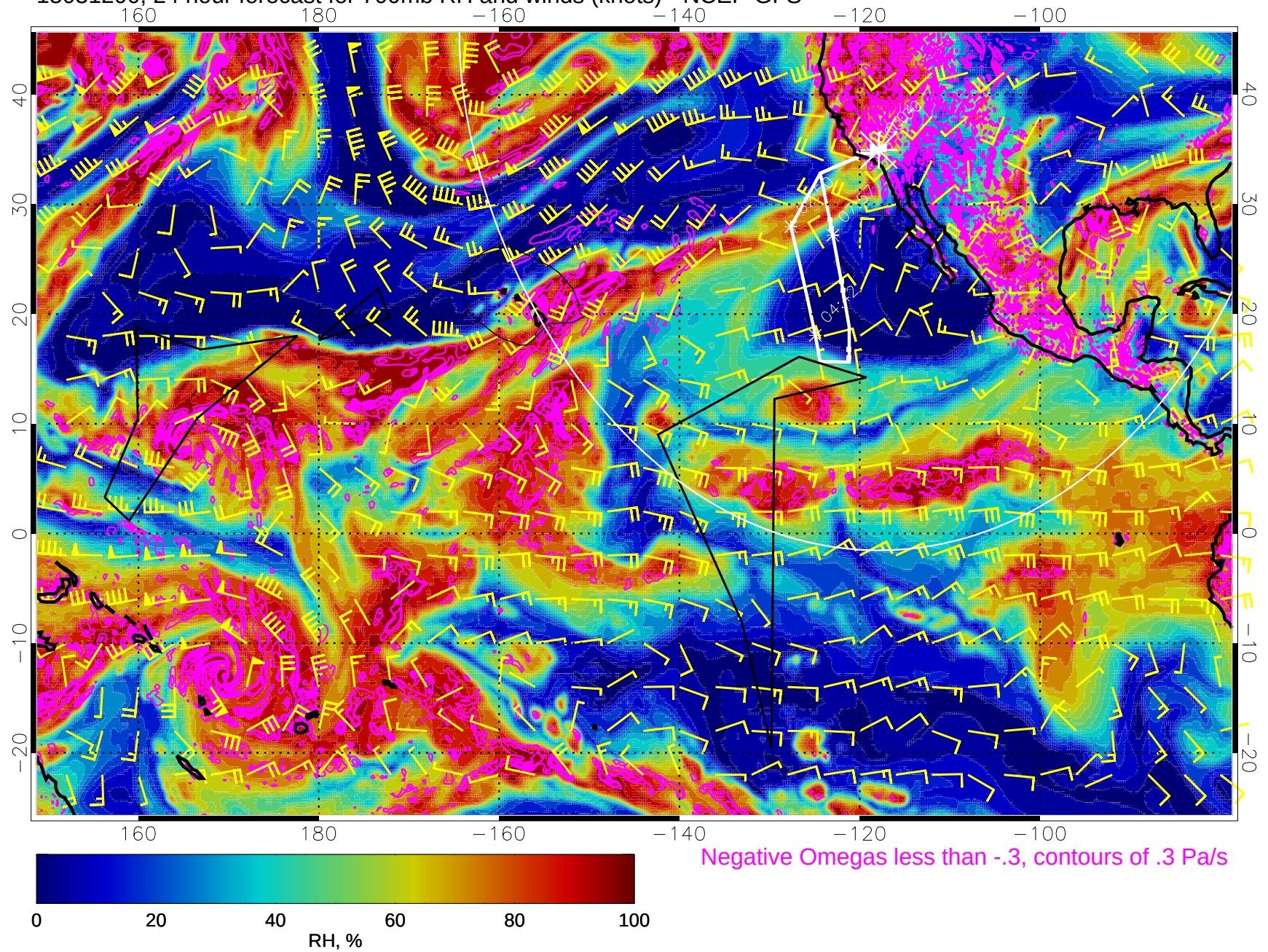
15031200, 24 hour forecast for 700mb RH and winds (knots) - NCEP GFS
