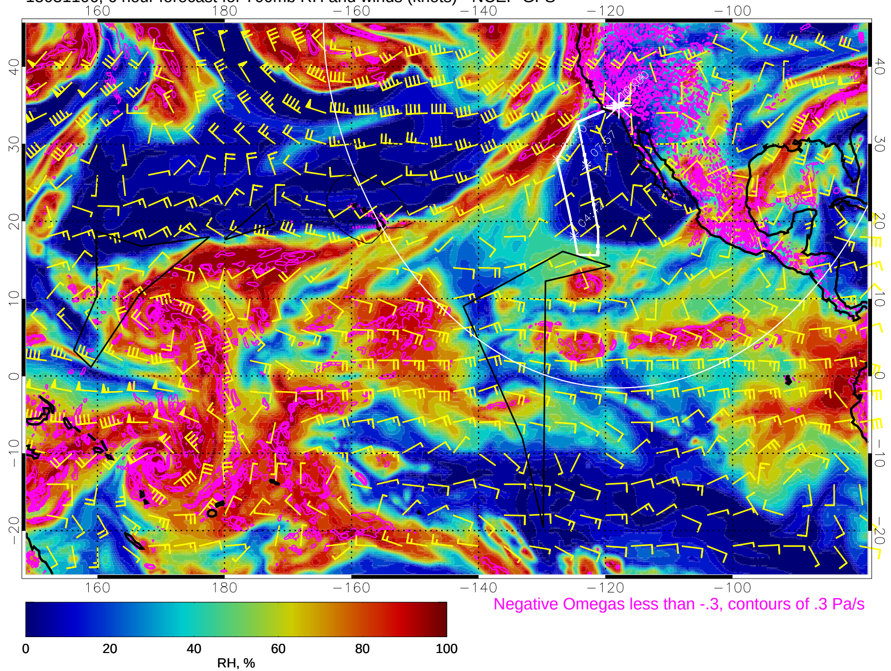
15031106, 6 hour forecast for 700mb RH and winds (knots) - NCEP GFS
