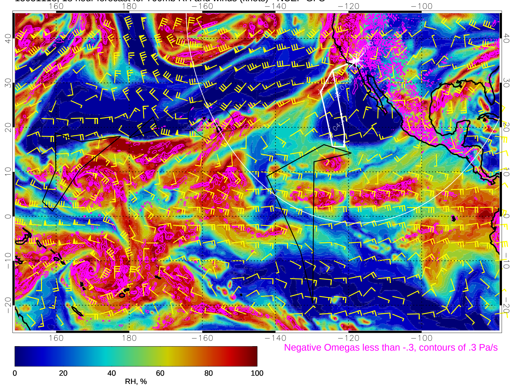
15031118, 18 hour forecast for 700mb RH and winds (knots) - NCEP GFS
