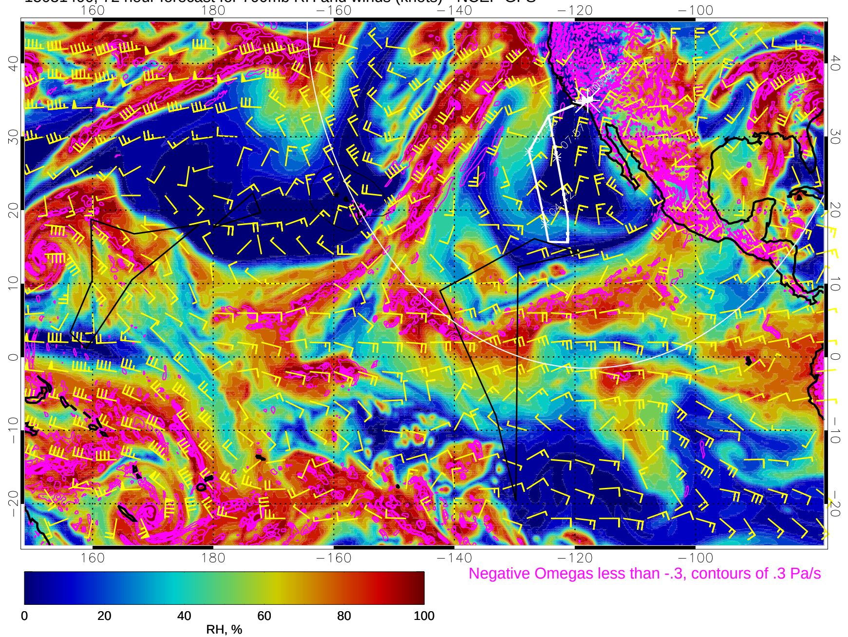
15031400, 72 hour forecast for 700mb RH and winds (knots) - NCEP GFS
