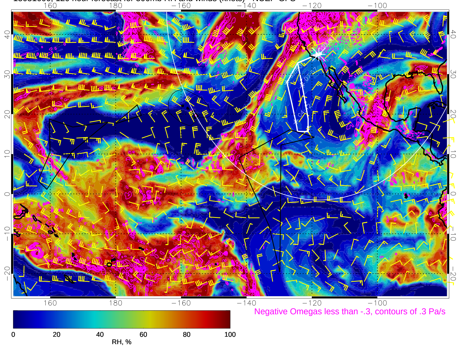
15031600, 120 hour forecast for 500mb RH and winds (knots) - NCEP GFS
