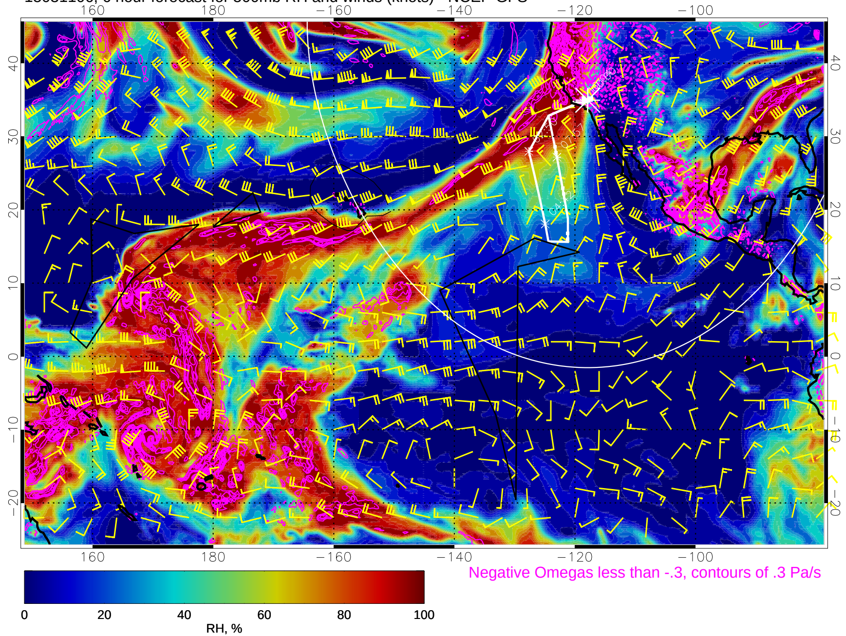
15031106, 6 hour forecast for 500mb RH and winds (knots) - NCEP GFS
