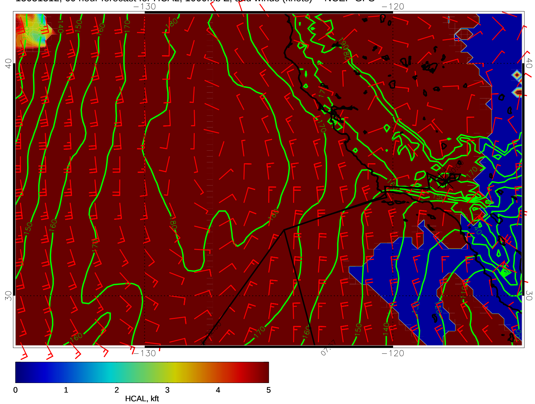
15031312, 60 hour forecast for HCAL, 1000mb Z, and winds (knots) -- NCEP GFS
