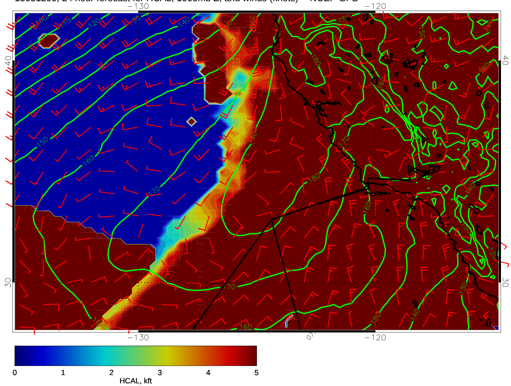
15031200, 24 hour forecast for HCAL, 1000mb Z, and winds (knots) -- NCEP GFS
