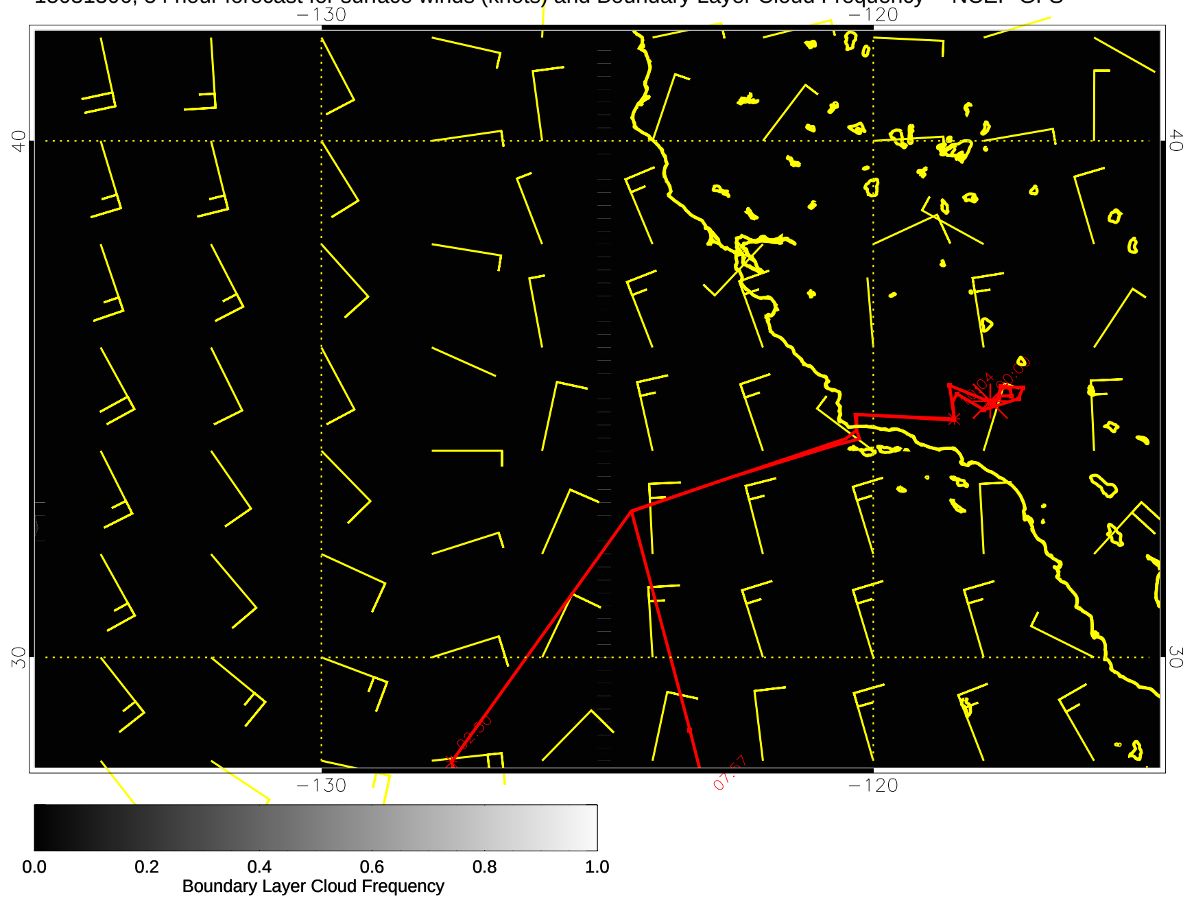
15031306, 54 hour forecast for surface winds (knots) and Boundary Layer Cloud Frequency -- NCEP GFS
