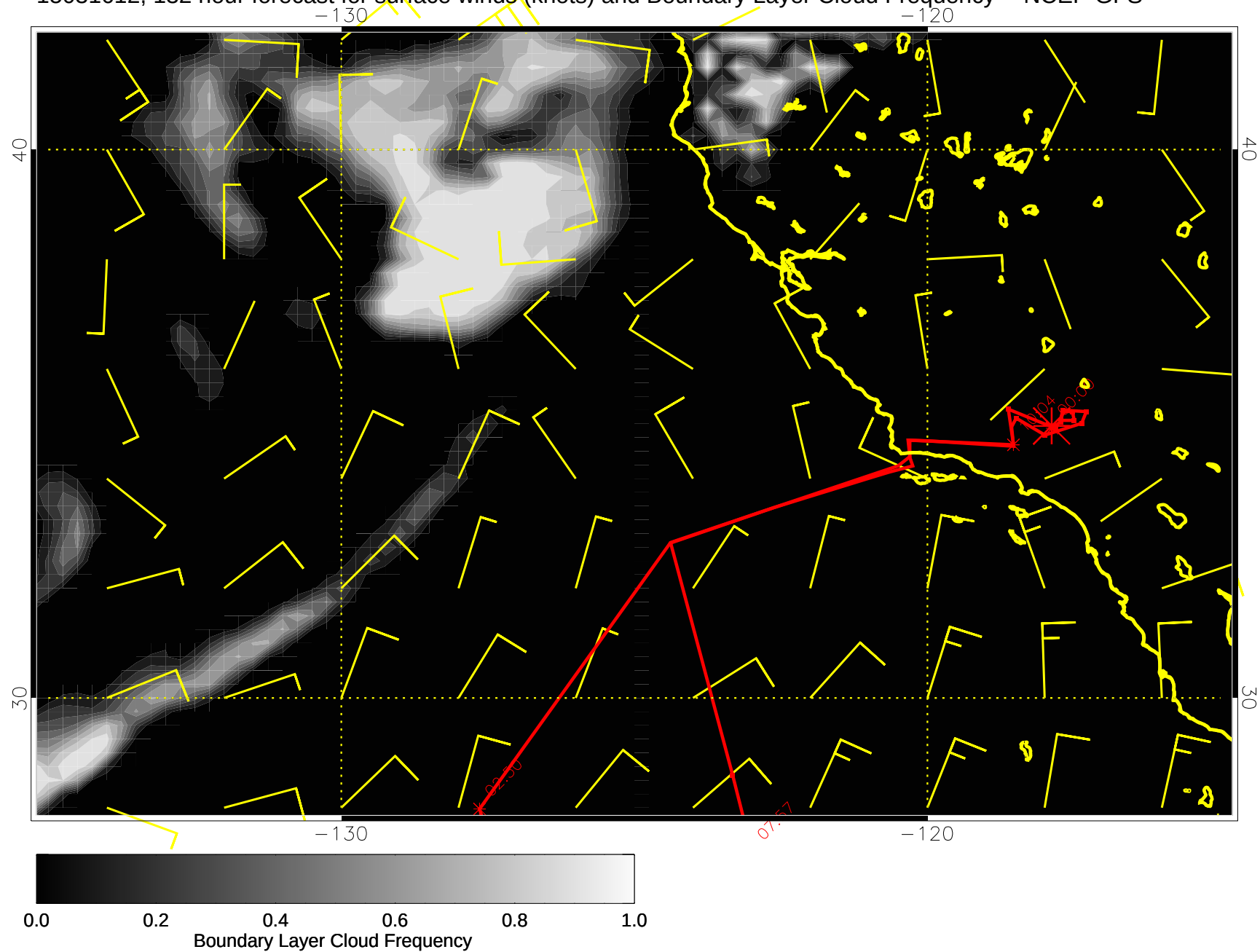
15031612, 132 hour forecast for surface winds (knots) and Boundary Layer Cloud Frequency -- NCEP GFS
