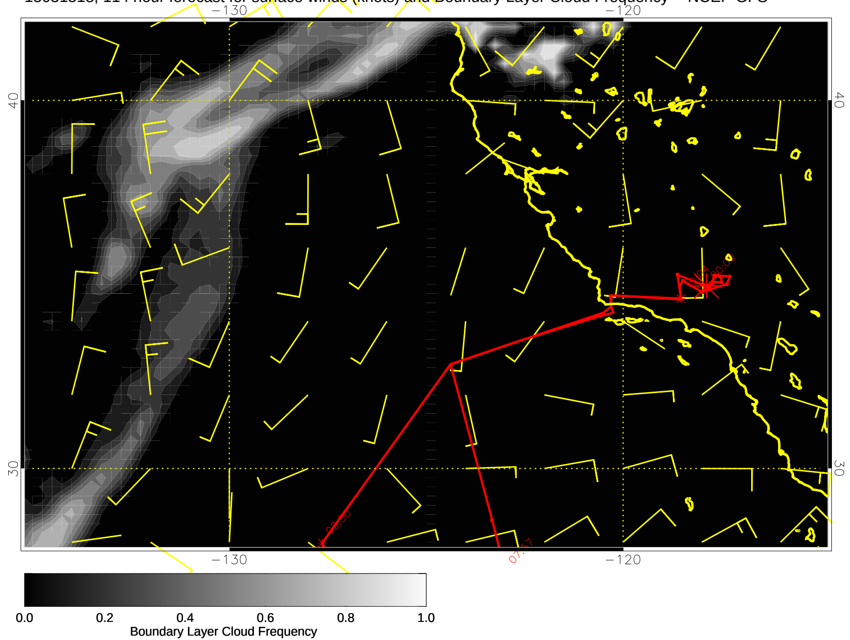
15031518, 114 hour forecast for surface winds (knots) and Boundary Layer Cloud Frequency -- NCEP GFS
