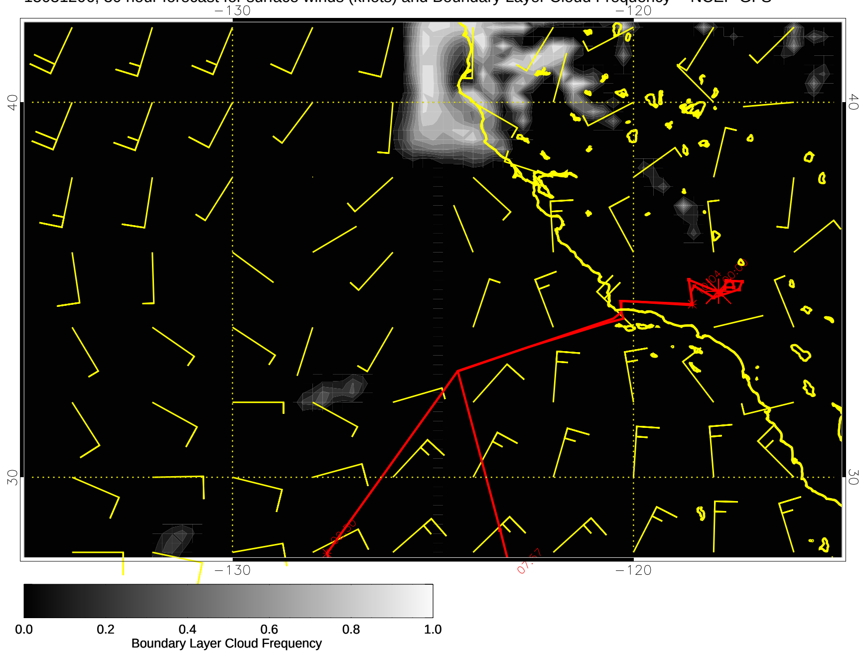
15031206, 30 hour forecast for surface winds (knots) and Boundary Layer Cloud Frequency -- NCEP GFS
