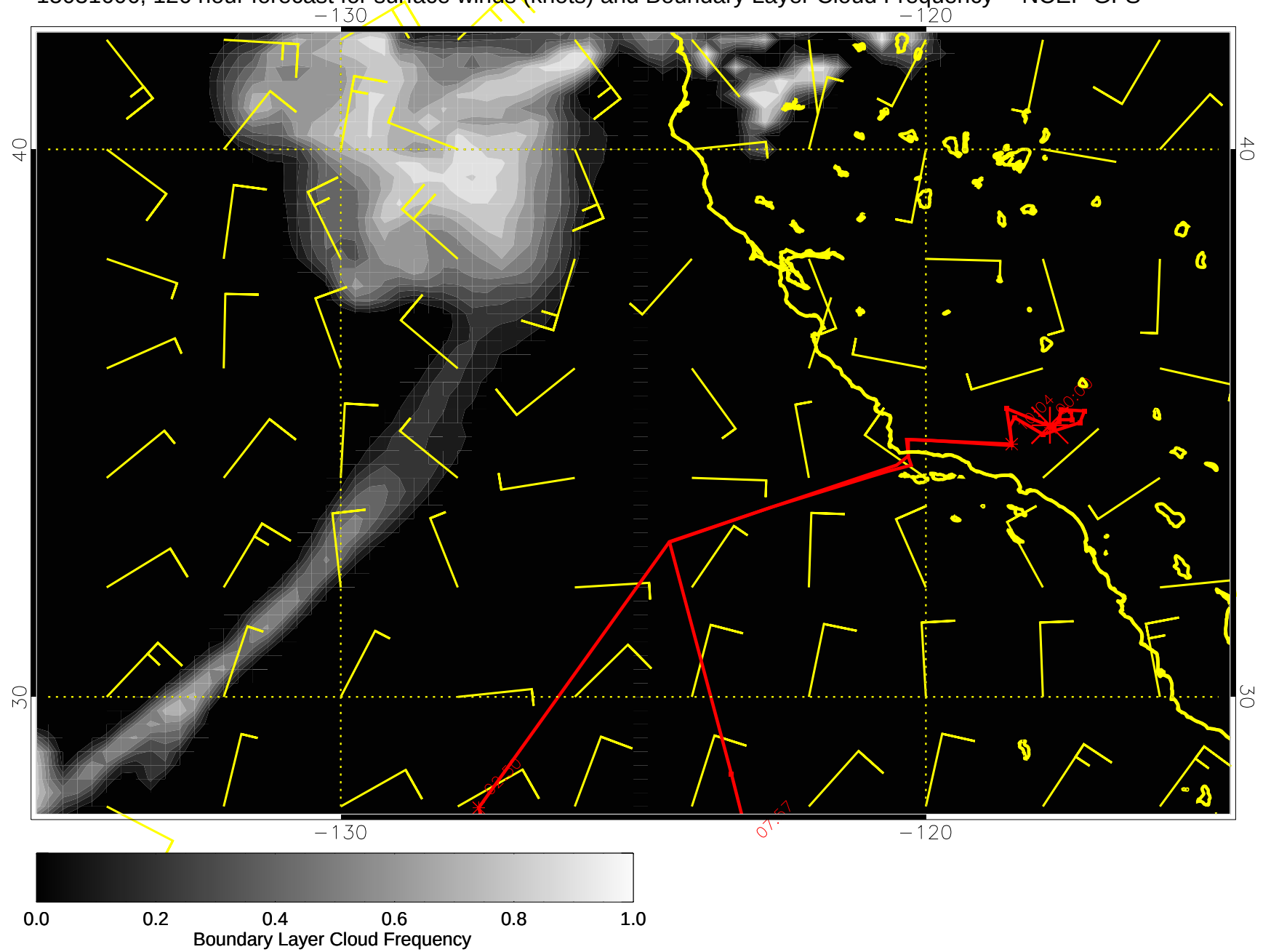
15031606, 126 hour forecast for surface winds (knots) and Boundary Layer Cloud Frequency -- NCEP GFS
