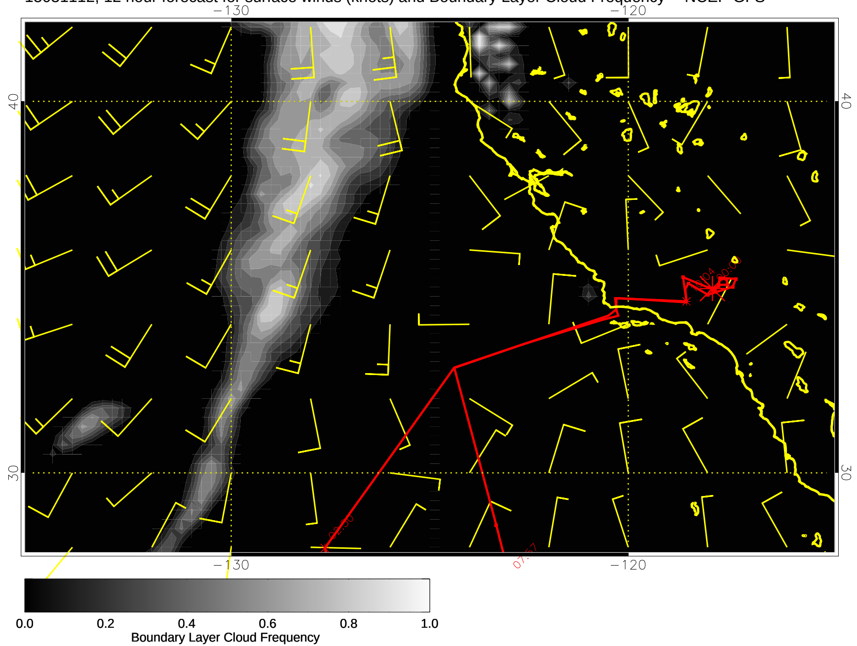
15031112, 12 hour forecast for surface winds (knots) and Boundary Layer Cloud Frequency -- NCEP GFS
