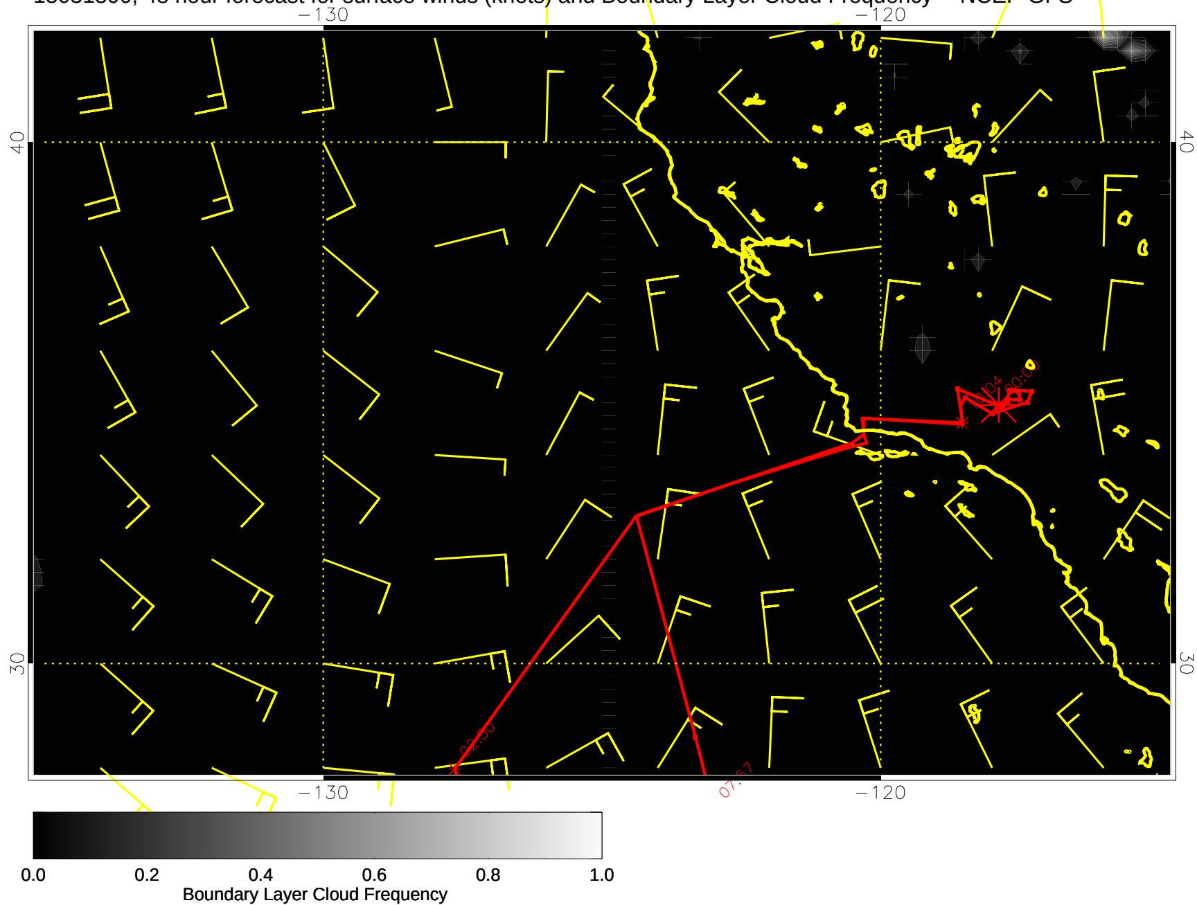
15031300, 48 hour forecast for surface winds (knots) and Boundary Layer Cloud Frequency -- NCEP GFS
