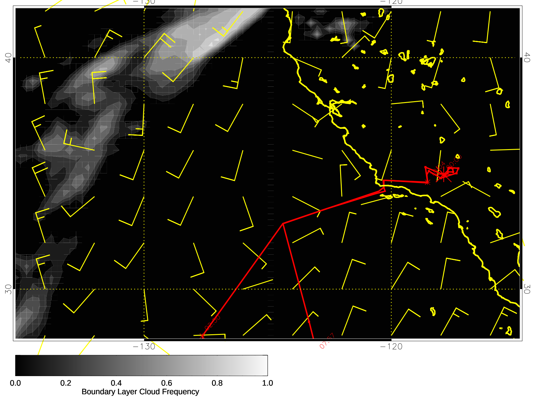
15031512, 108 hour forecast for surface winds (knots) and Boundary Layer Cloud Frequency -- NCEP GFS
