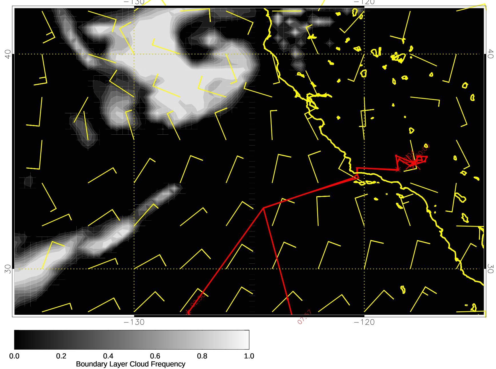
15031618, 138 hour forecast for surface winds (knots) and Boundary Layer Cloud Frequency -- NCEP GFS
