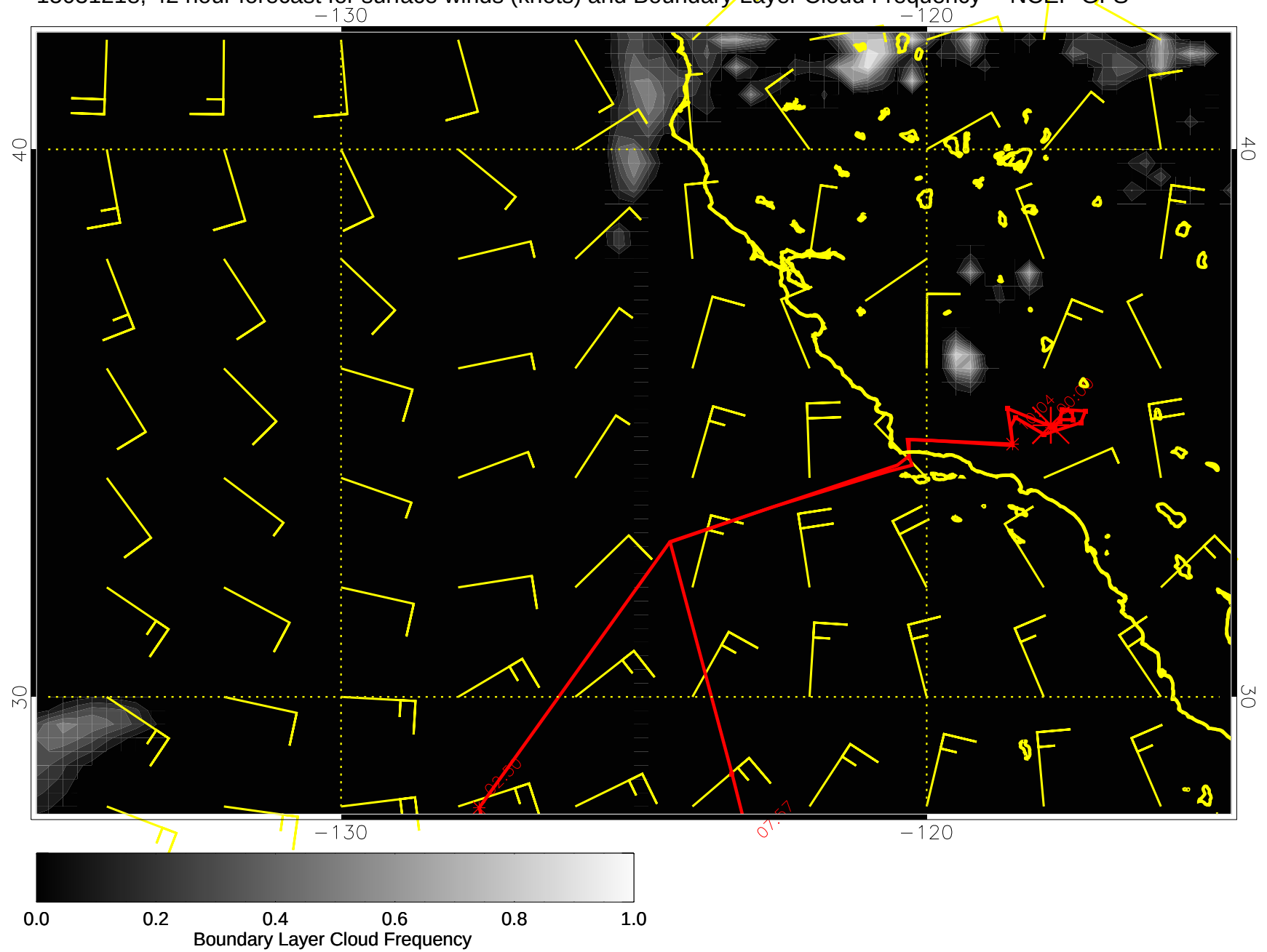
15031218, 42 hour forecast for surface winds (knots) and Boundary Layer Cloud Frequency -- NCEP GFS
