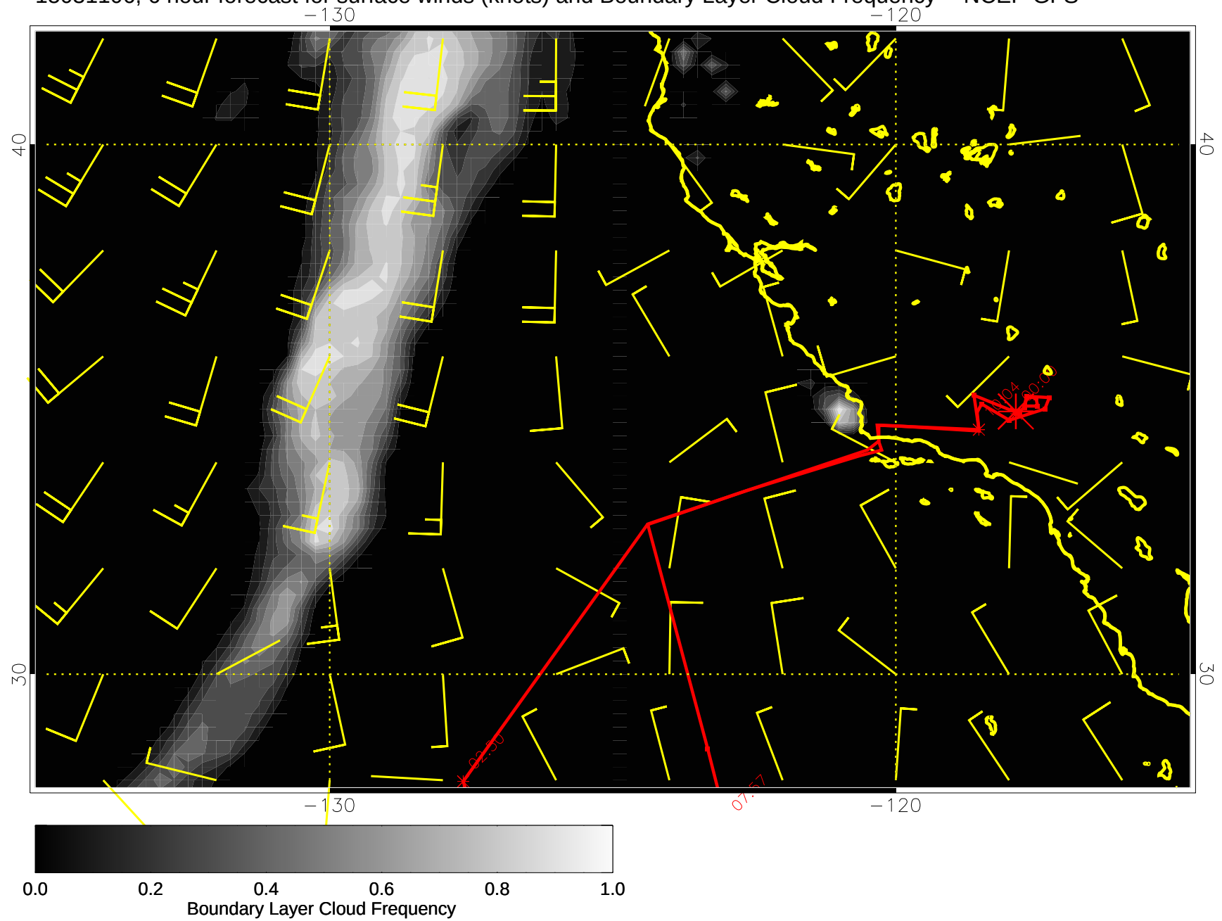
15031106, 6 hour forecast for surface winds (knots) and Boundary Layer Cloud Frequency -- NCEP GFS
