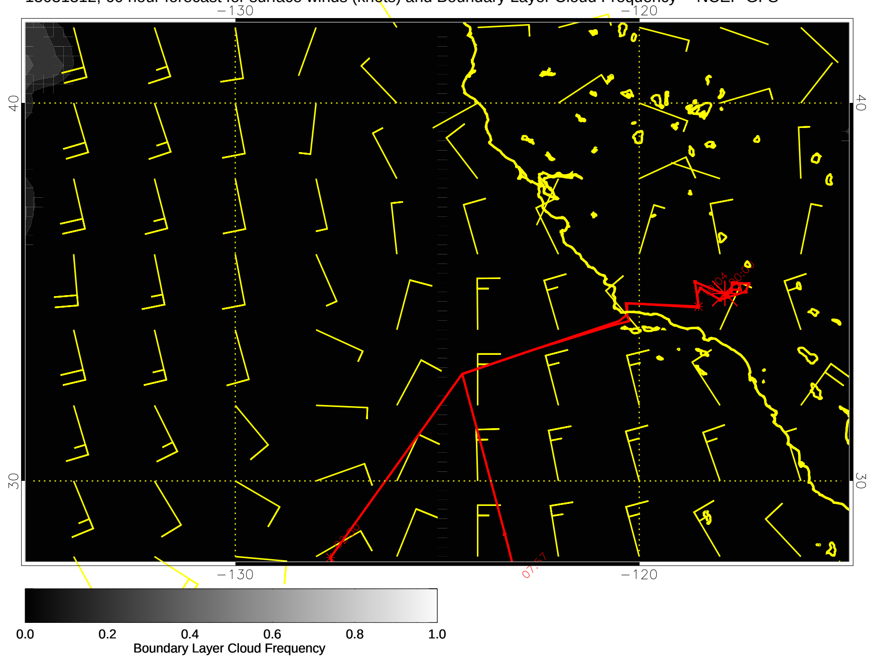
15031312, 60 hour forecast for surface winds (knots) and Boundary Layer Cloud Frequency -- NCEP GFS
