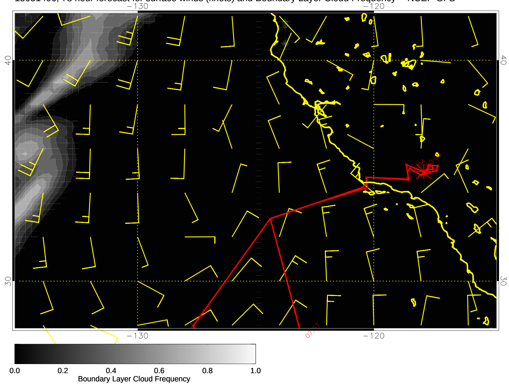
15031406, 78 hour forecast for surface winds (knots) and Boundary Layer Cloud Frequency -- NCEP GFS
