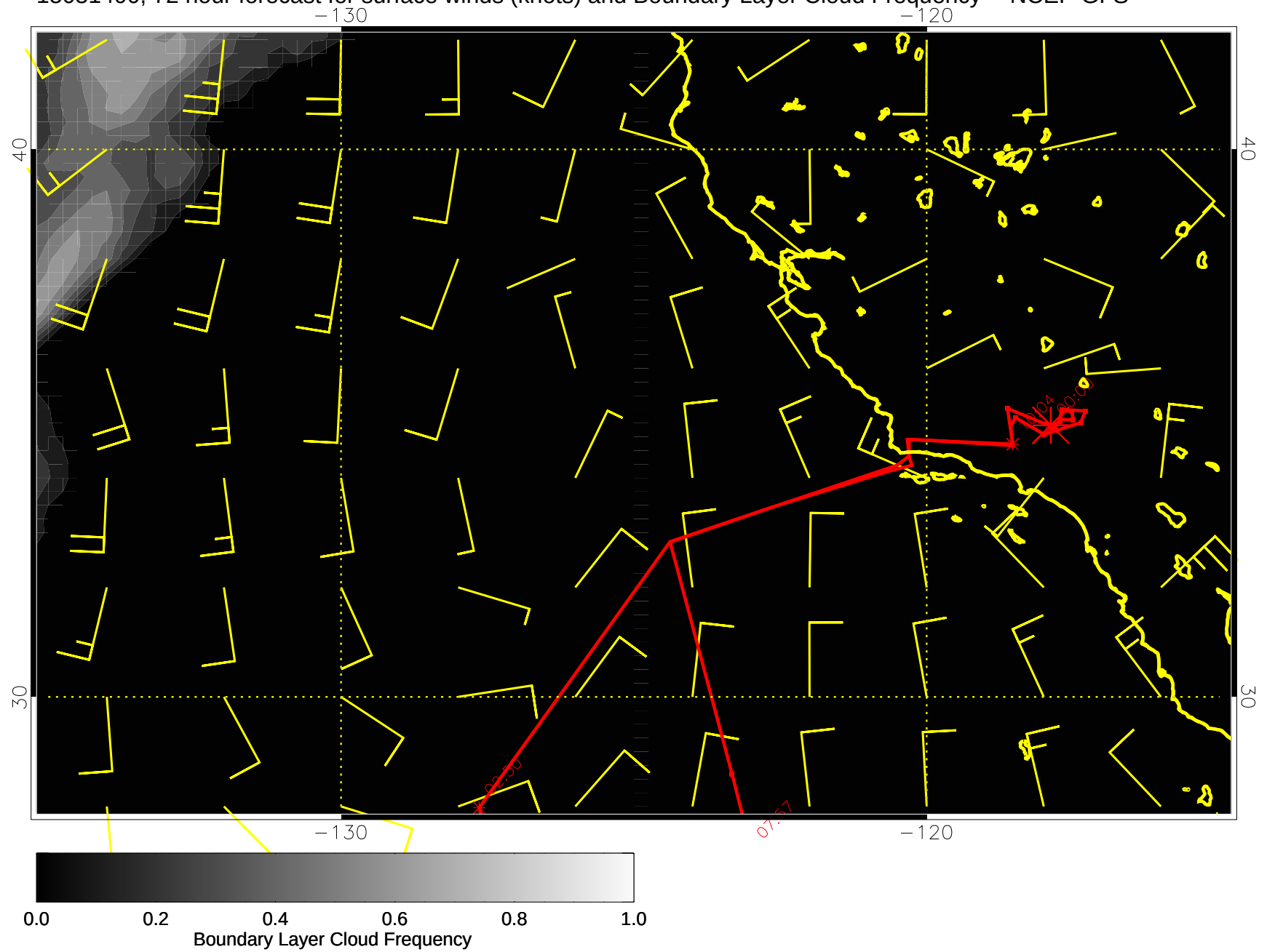
15031400, 72 hour forecast for surface winds (knots) and Boundary Layer Cloud Frequency -- NCEP GFS
