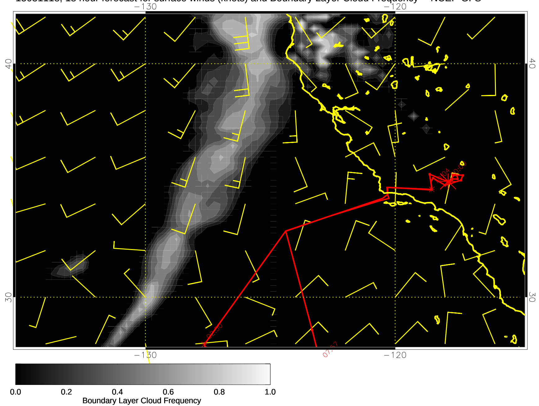
15031118, 18 hour forecast for surface winds (knots) and Boundary Layer Cloud Frequency -- NCEP GFS
