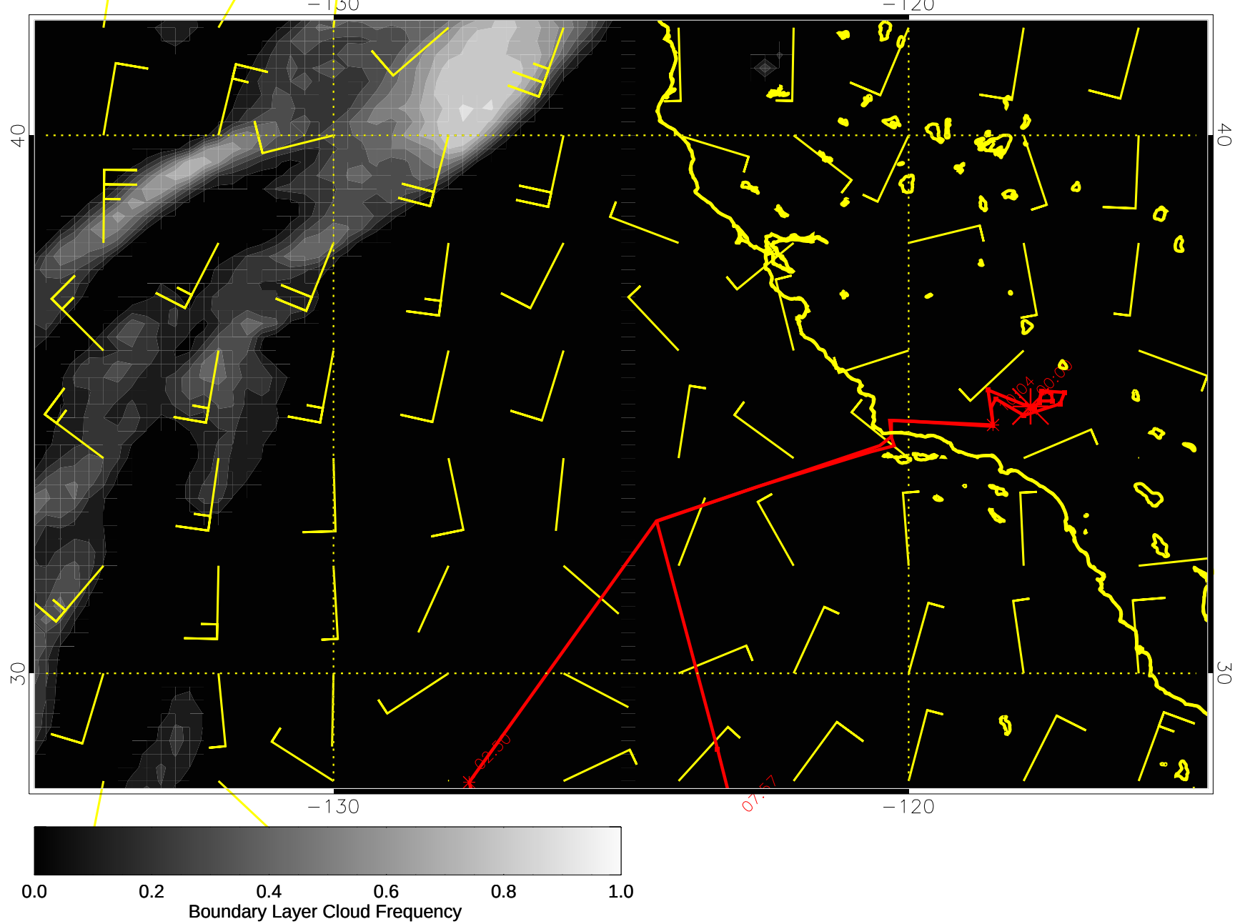
15031506, 102 hour forecast for surface winds (knots) and Boundary Layer Cloud Frequency -- NCEP GFS
