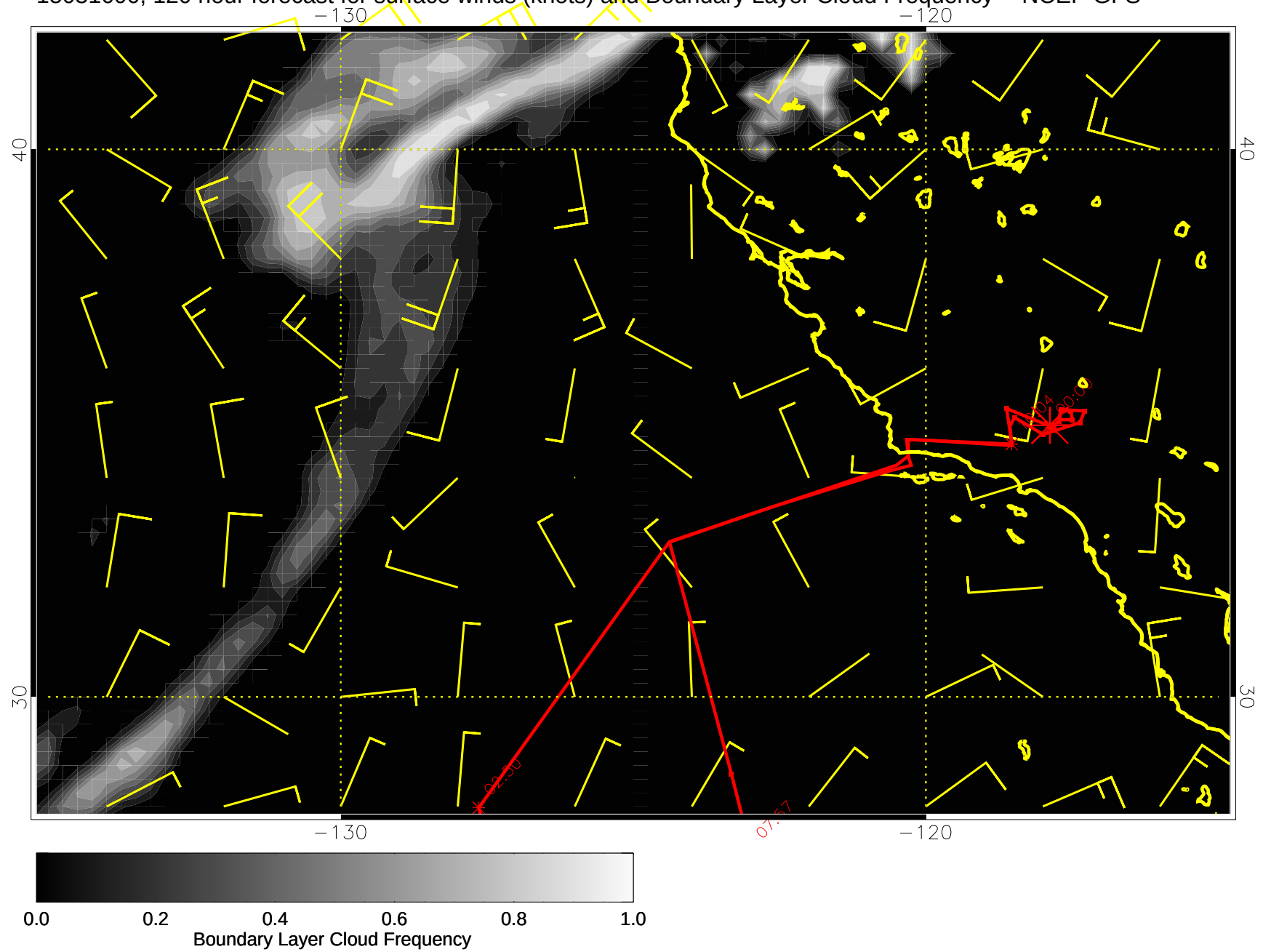
15031600, 120 hour forecast for surface winds (knots) and Boundary Layer Cloud Frequency -- NCEP GFS
