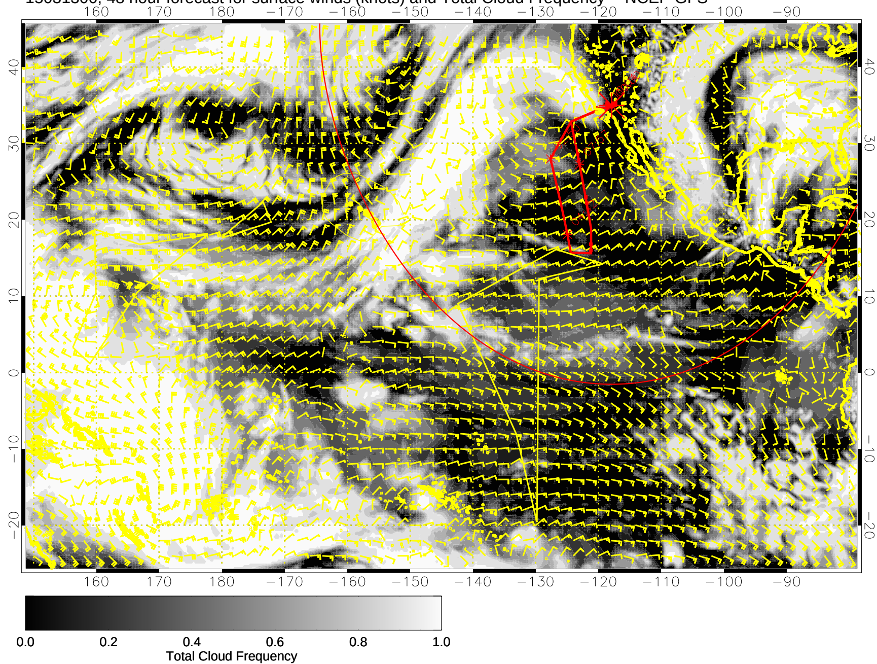
15031300, 48 hour forecast for surface winds (knots) and Total Cloud Frequency -- NCEP GFS
