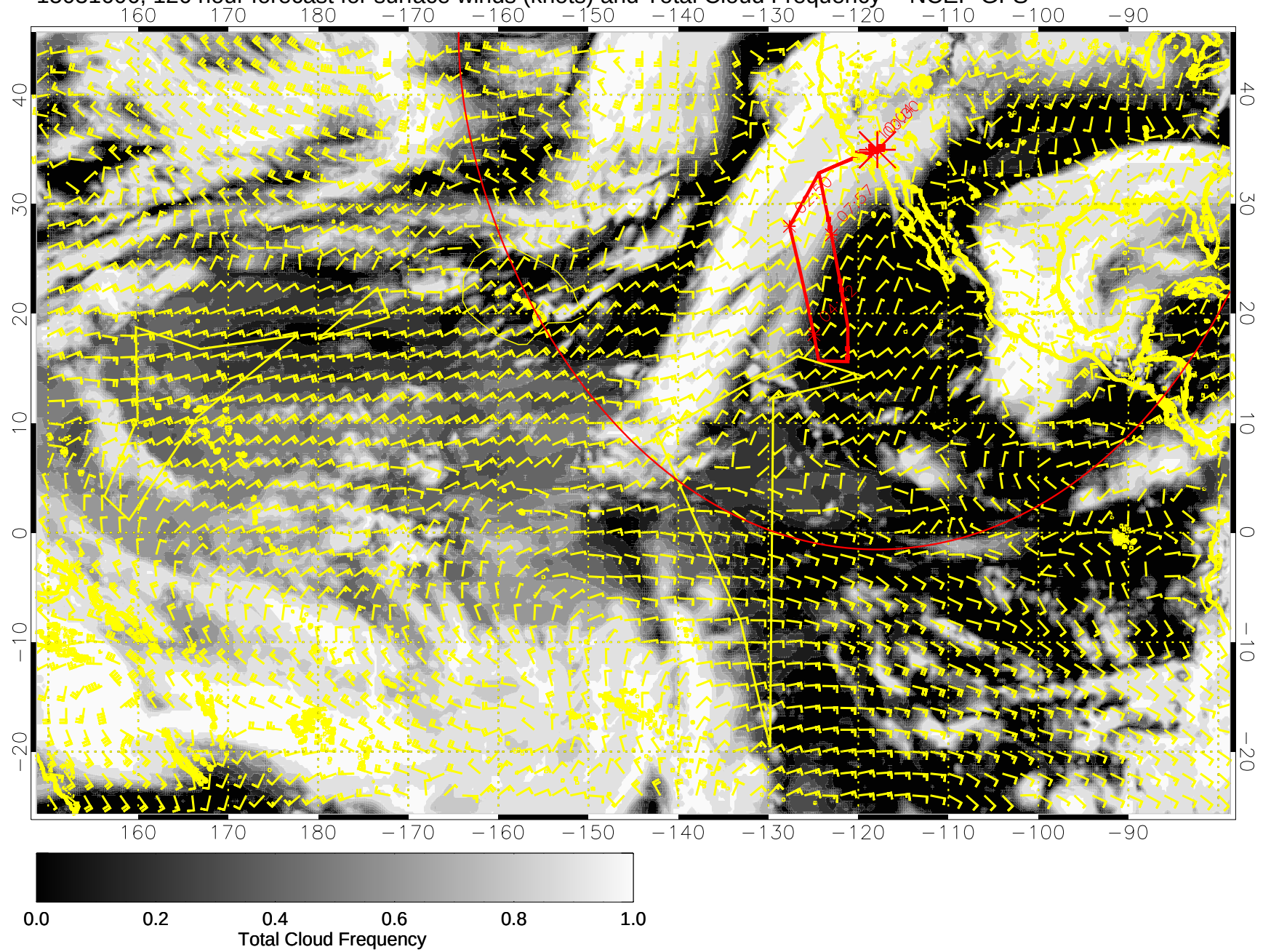
15031606, 126 hour forecast for surface winds (knots) and Total Cloud Frequency -- NCEP GFS
