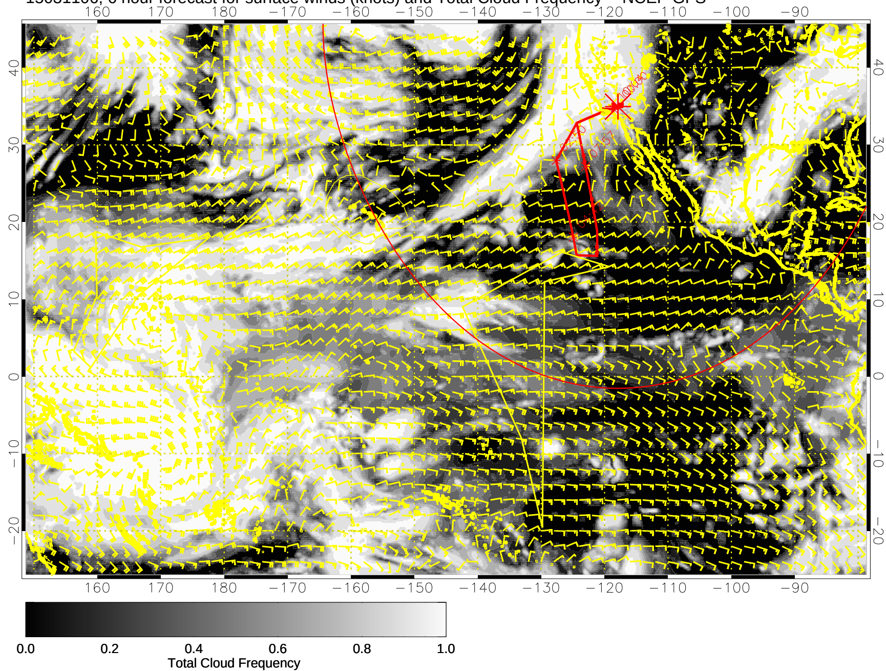
15031106, 6 hour forecast for surface winds (knots) and Total Cloud Frequency -- NCEP GFS
