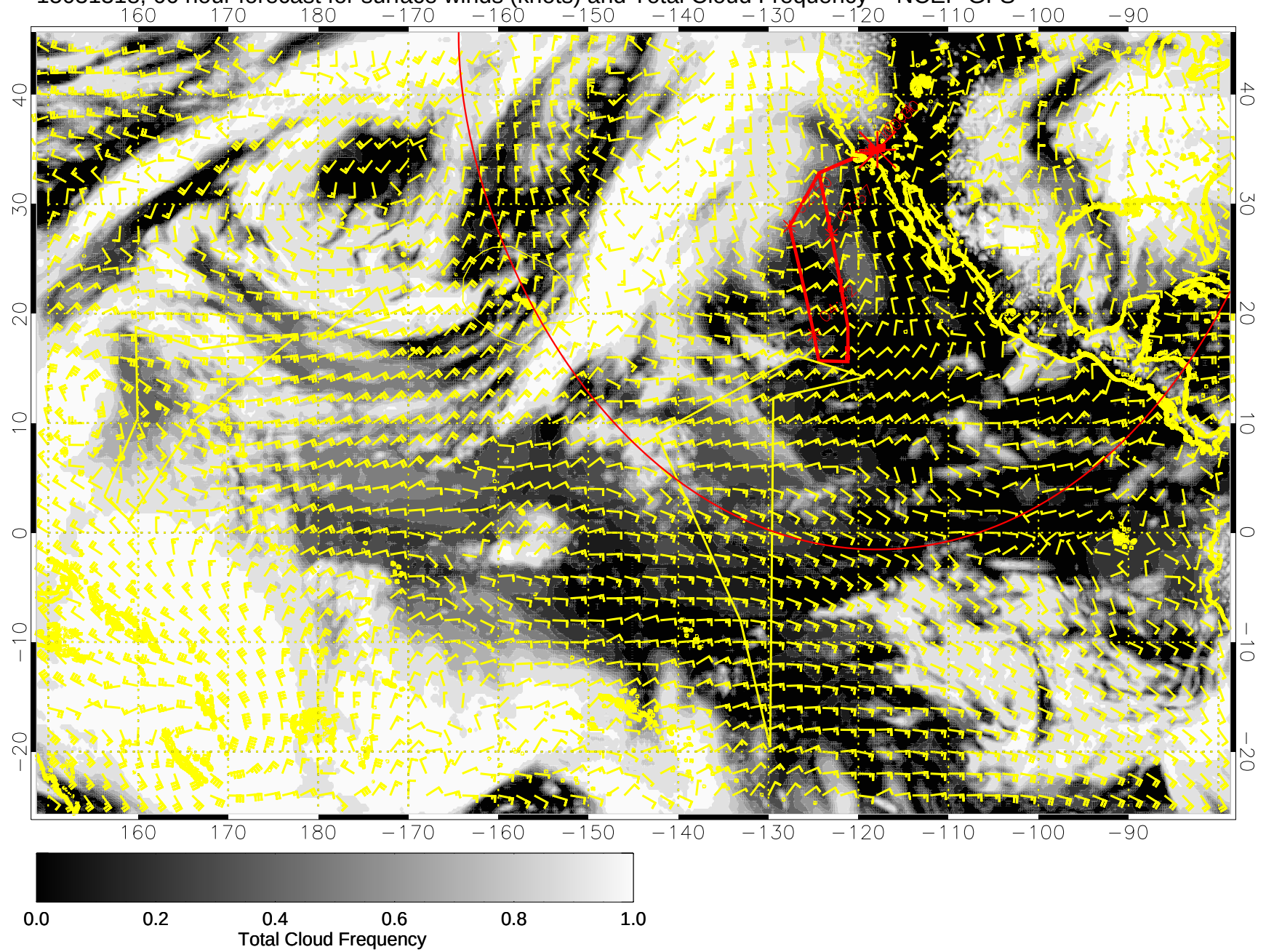
15031318, 66 hour forecast for surface winds (knots) and Total Cloud Frequency -- NCEP GFS
