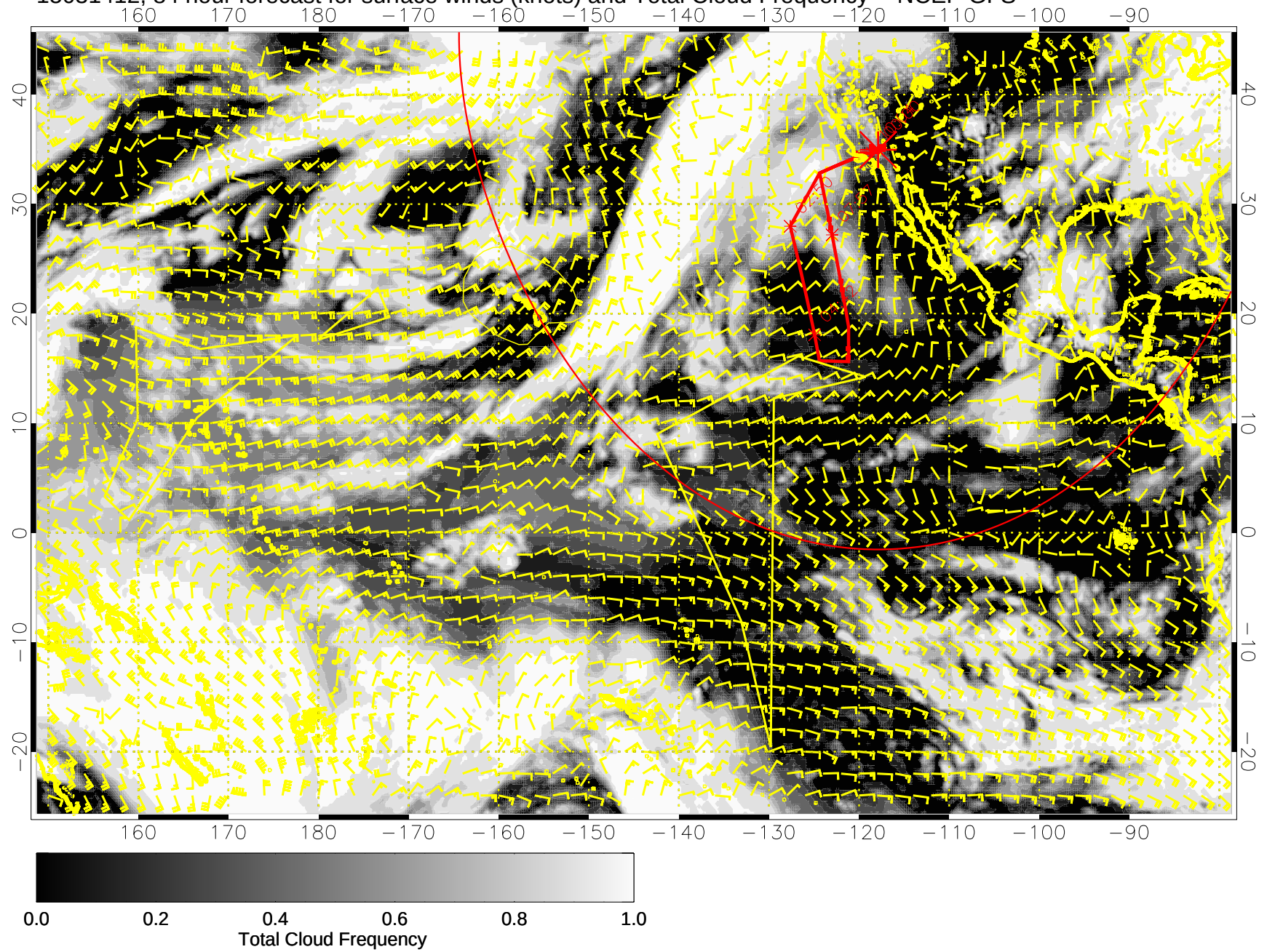
15031412, 84 hour forecast for surface winds (knots) and Total Cloud Frequency -- NCEP GFS
