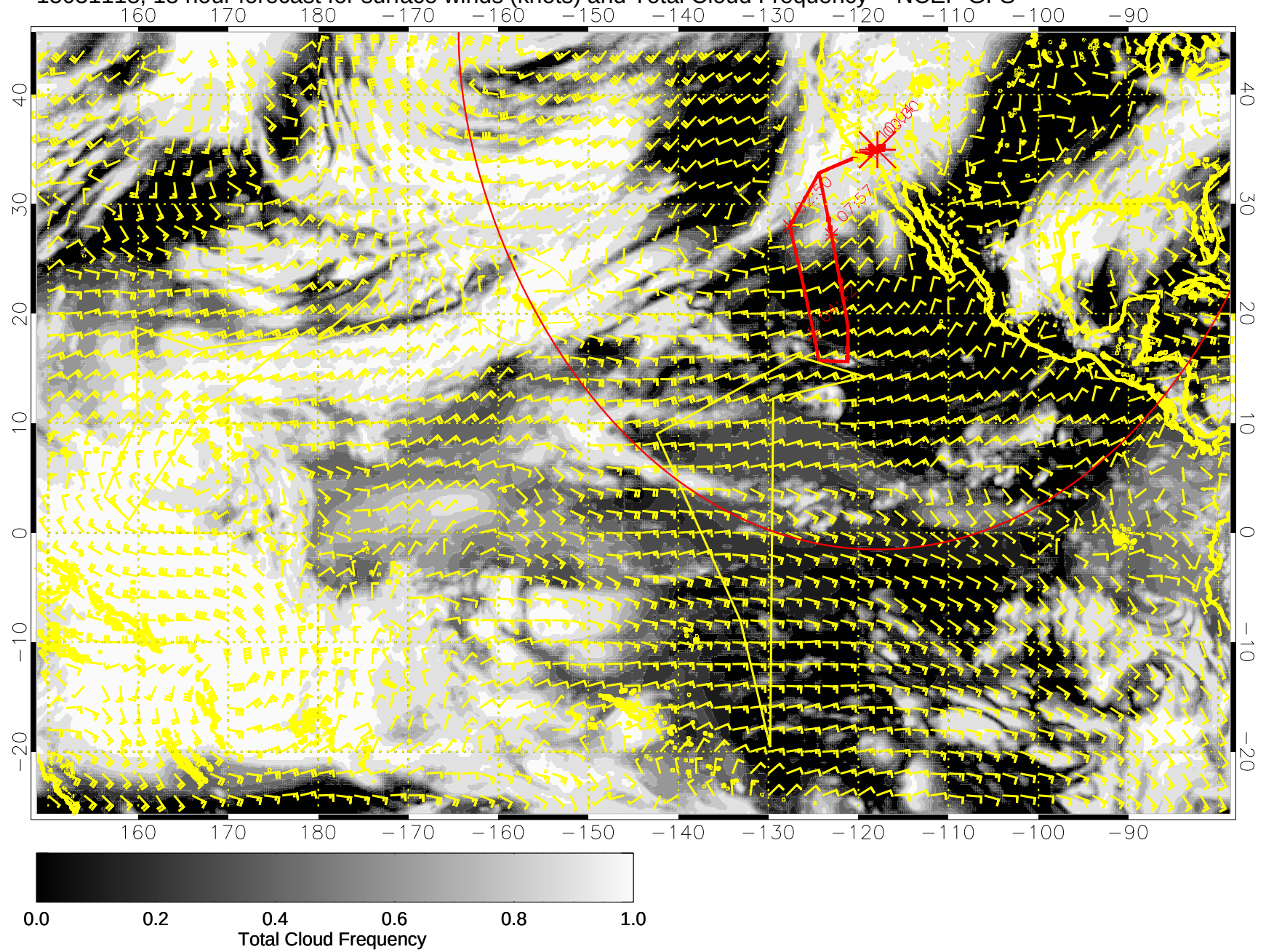
15031118, 18 hour forecast for surface winds (knots) and Total Cloud Frequency -- NCEP GFS
