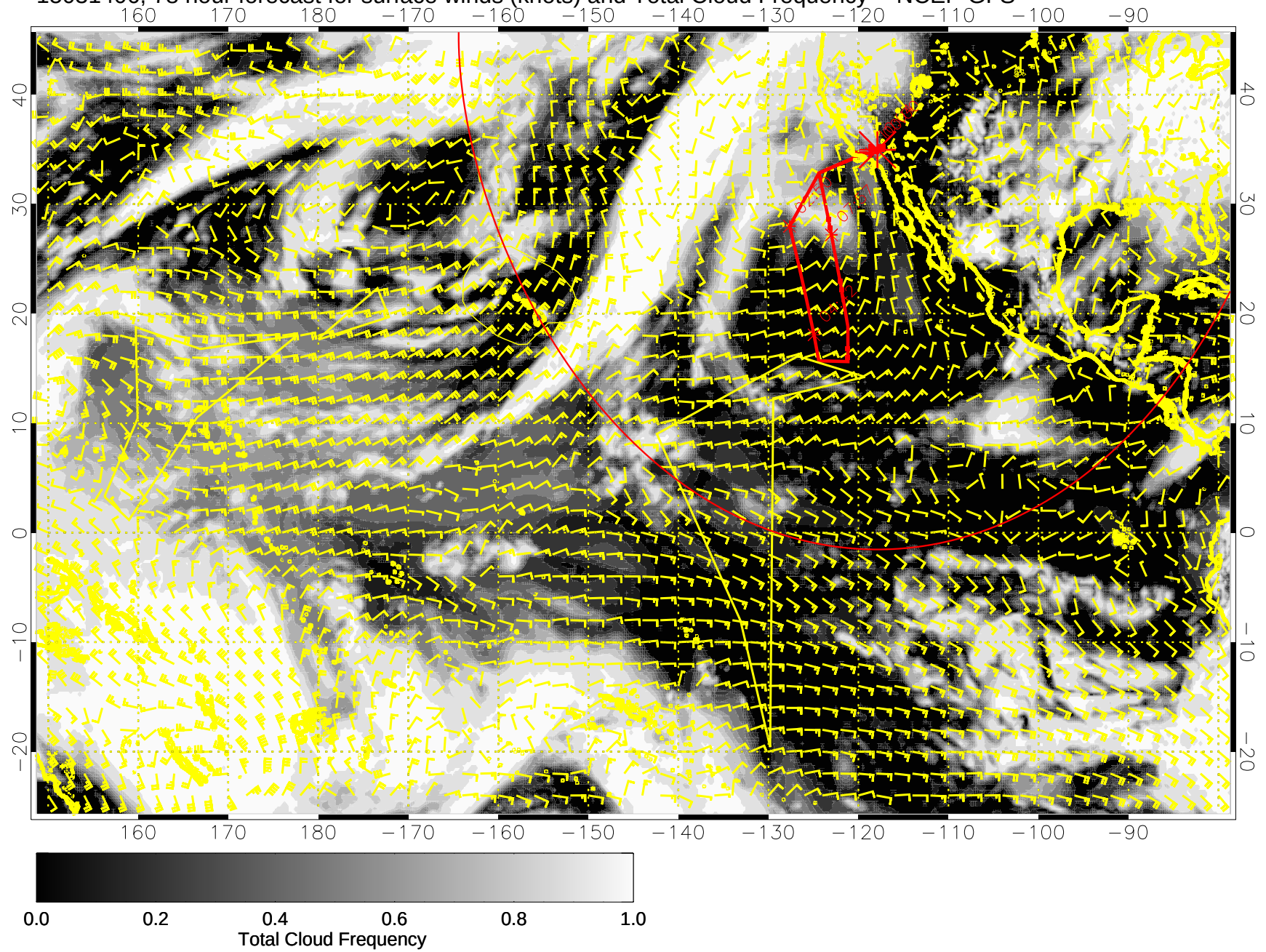
15031406, 78 hour forecast for surface winds (knots) and Total Cloud Frequency -- NCEP GFS
