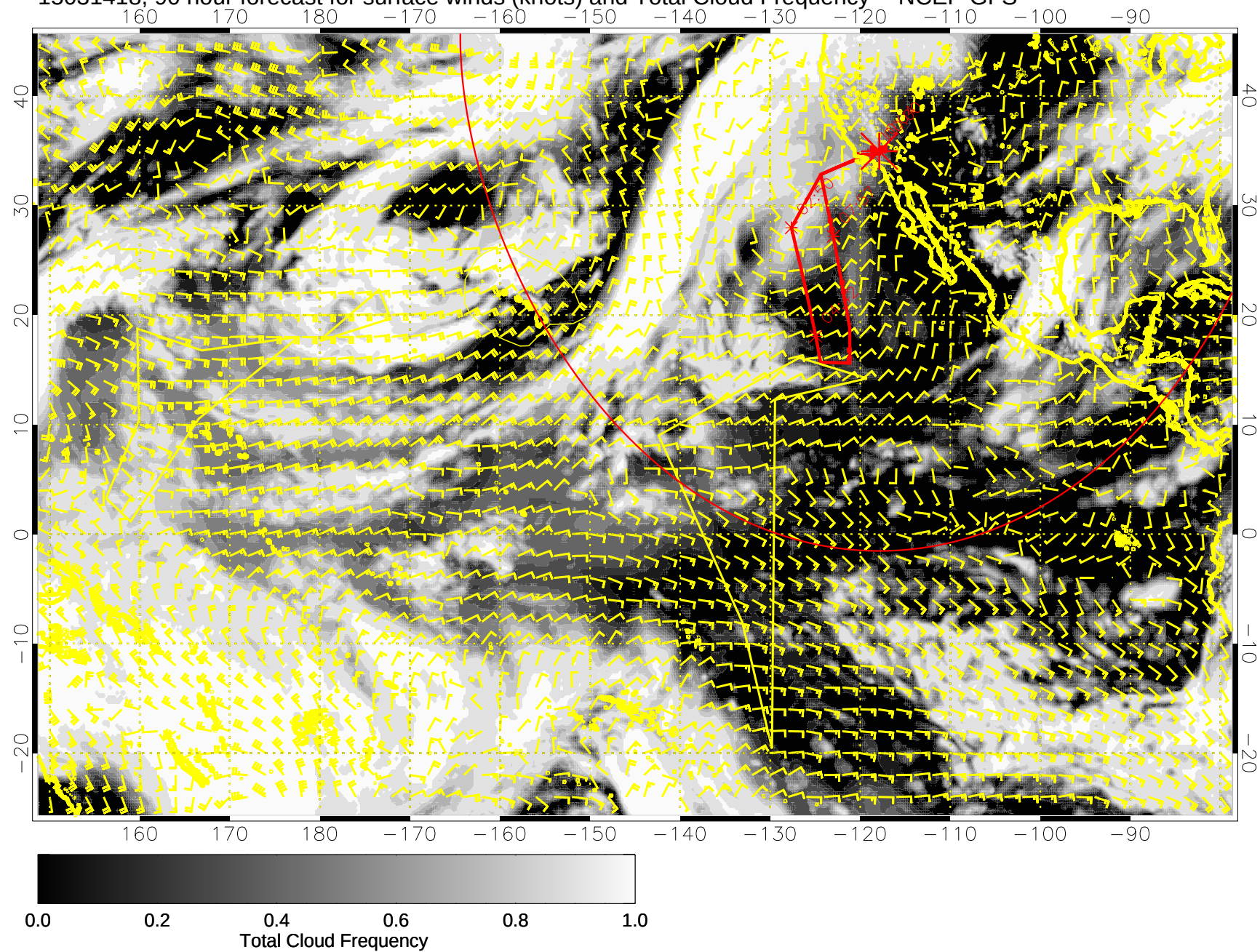
15031418, 90 hour forecast for surface winds (knots) and Total Cloud Frequency -- NCEP GFS
