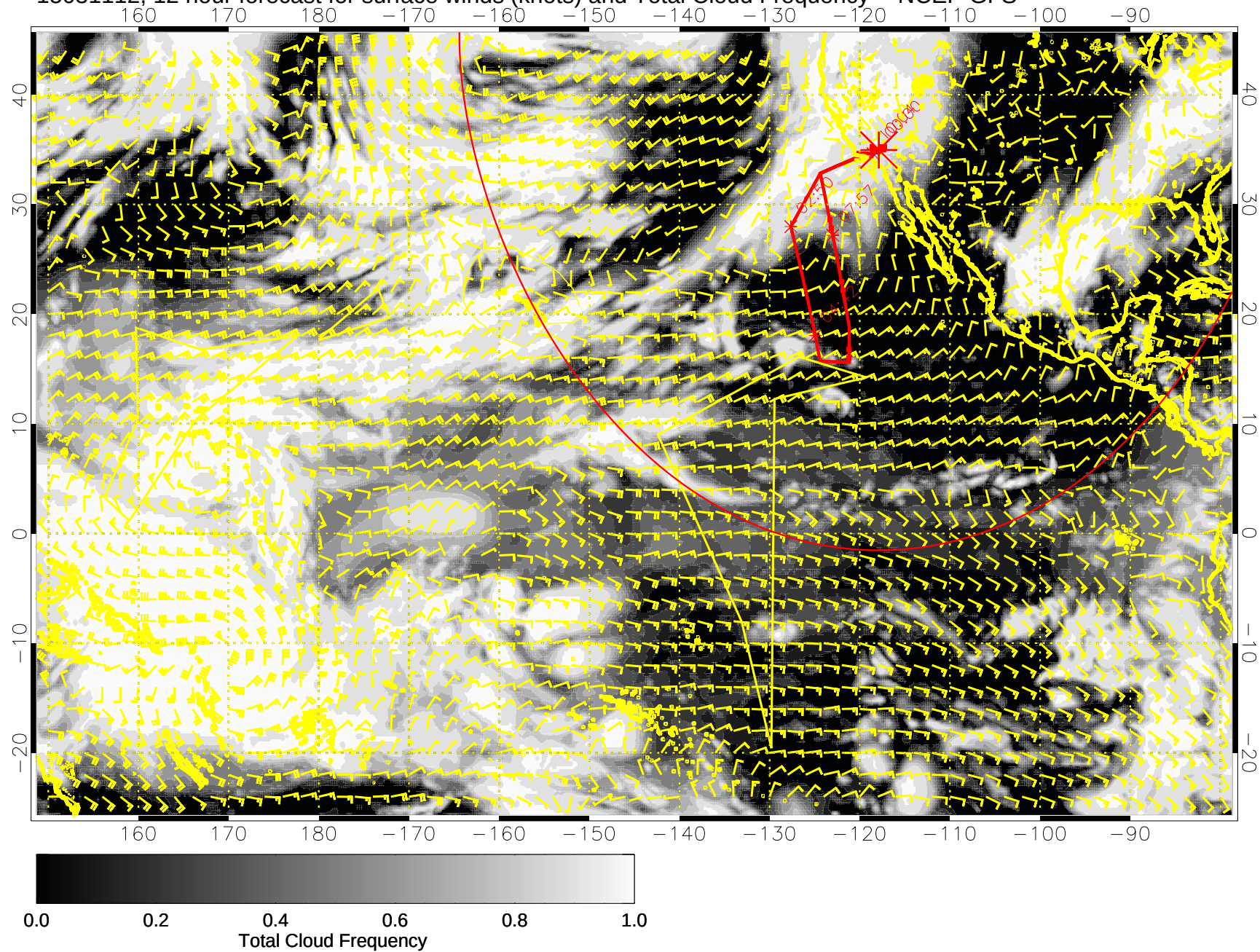
15031112, 12 hour forecast for surface winds (knots) and Total Cloud Frequency -- NCEP GFS
