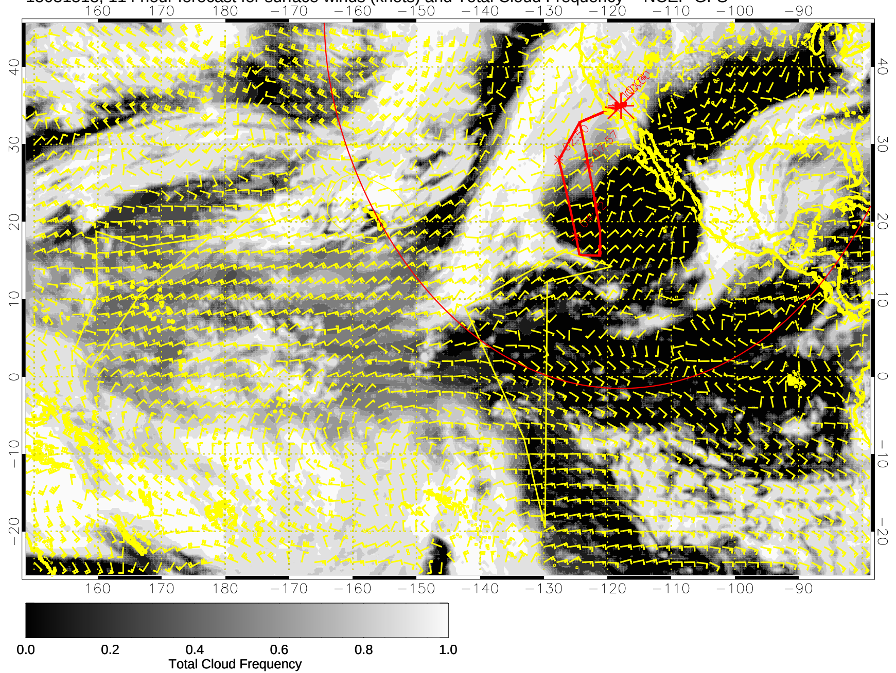
15031518, 114 hour forecast for surface winds (knots) and Total Cloud Frequency -- NCEP GFS
