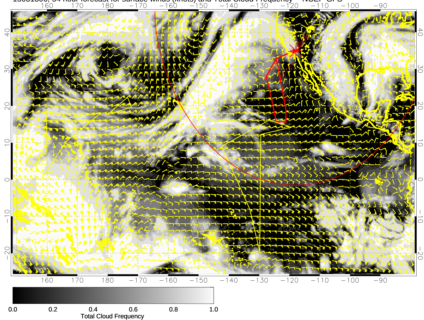
15031306, 54 hour forecast for surface winds (knots) and Total Cloud Frequency -- NCEP GFS
