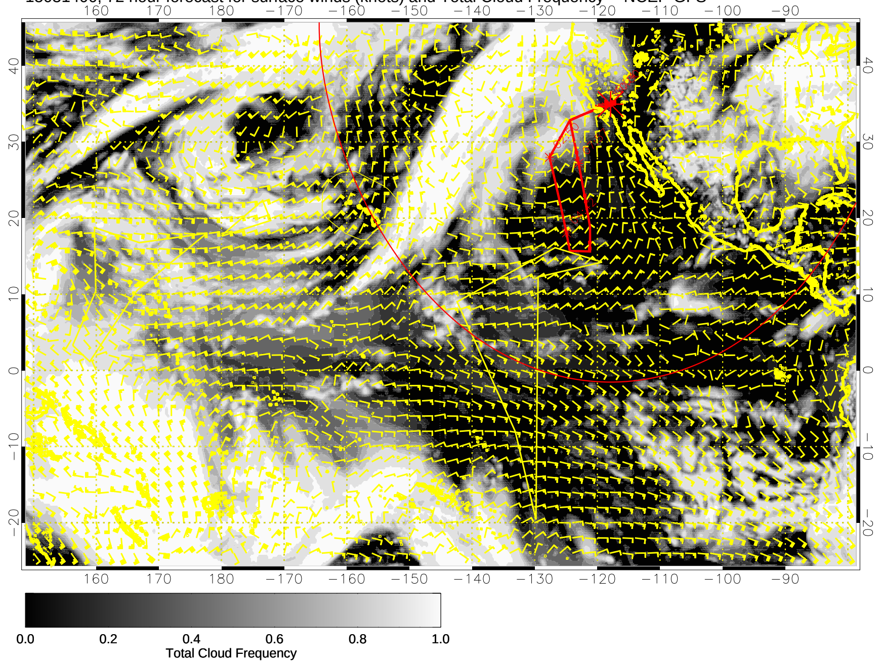
15031400, 72 hour forecast for surface winds (knots) and Total Cloud Frequency -- NCEP GFS
