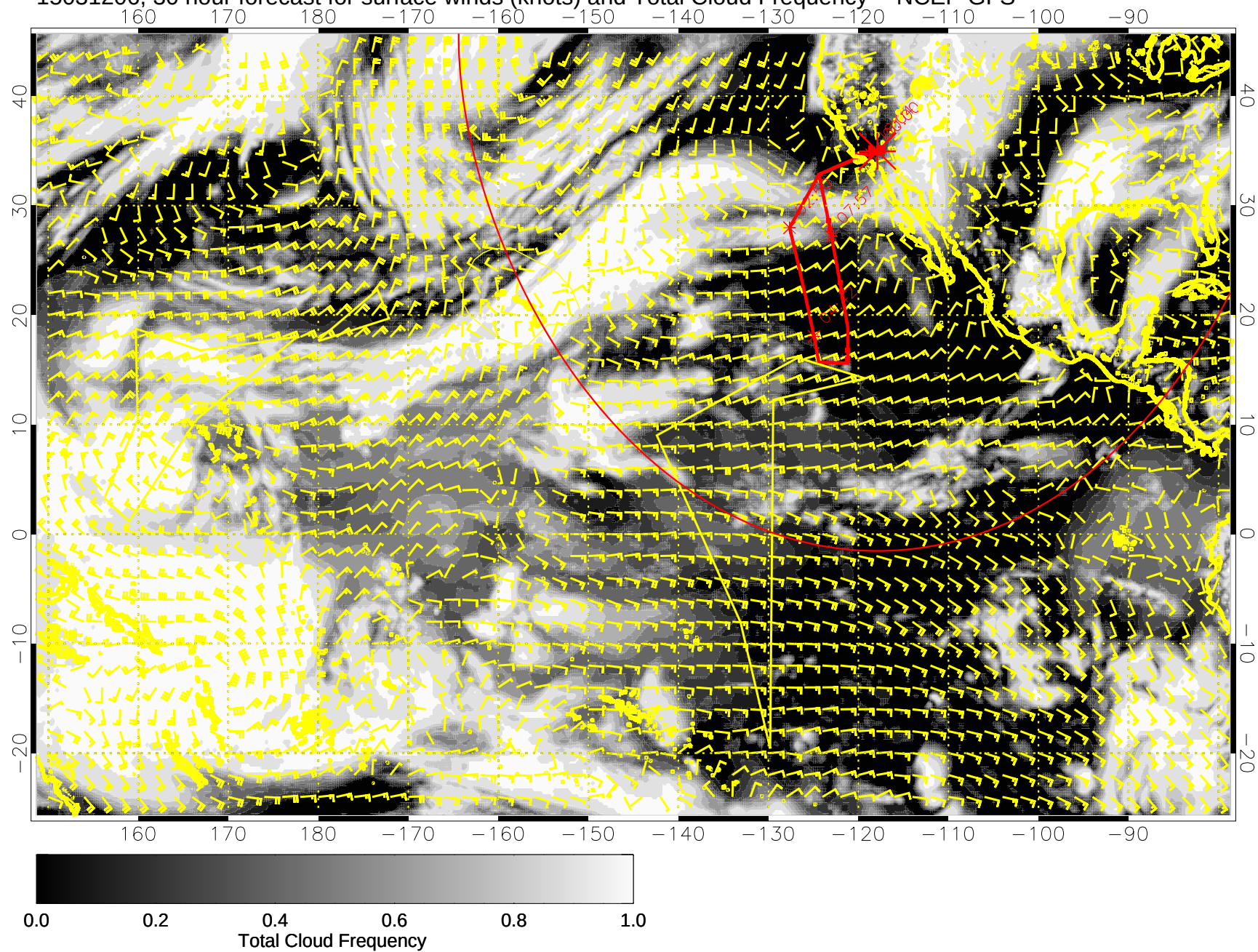
15031206, 30 hour forecast for surface winds (knots) and Total Cloud Frequency -- NCEP GFS
