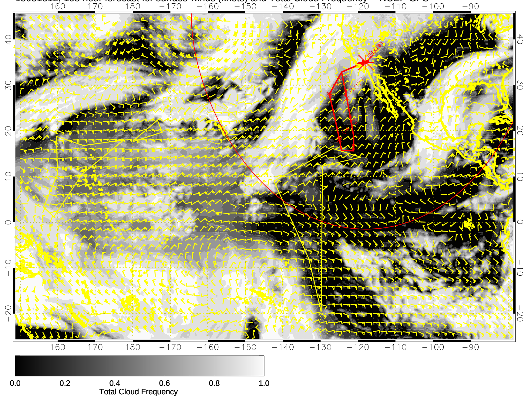
15031512, 108 hour forecast for surface winds (knots) and Total Cloud Frequency -- NCEP GFS
