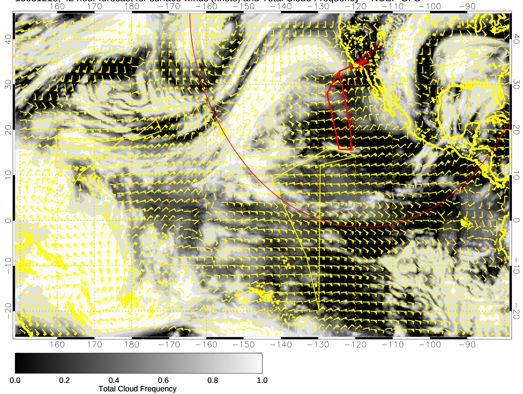
15031218, 42 hour forecast for surface winds (knots) and Total Cloud Frequency -- NCEP GFS
