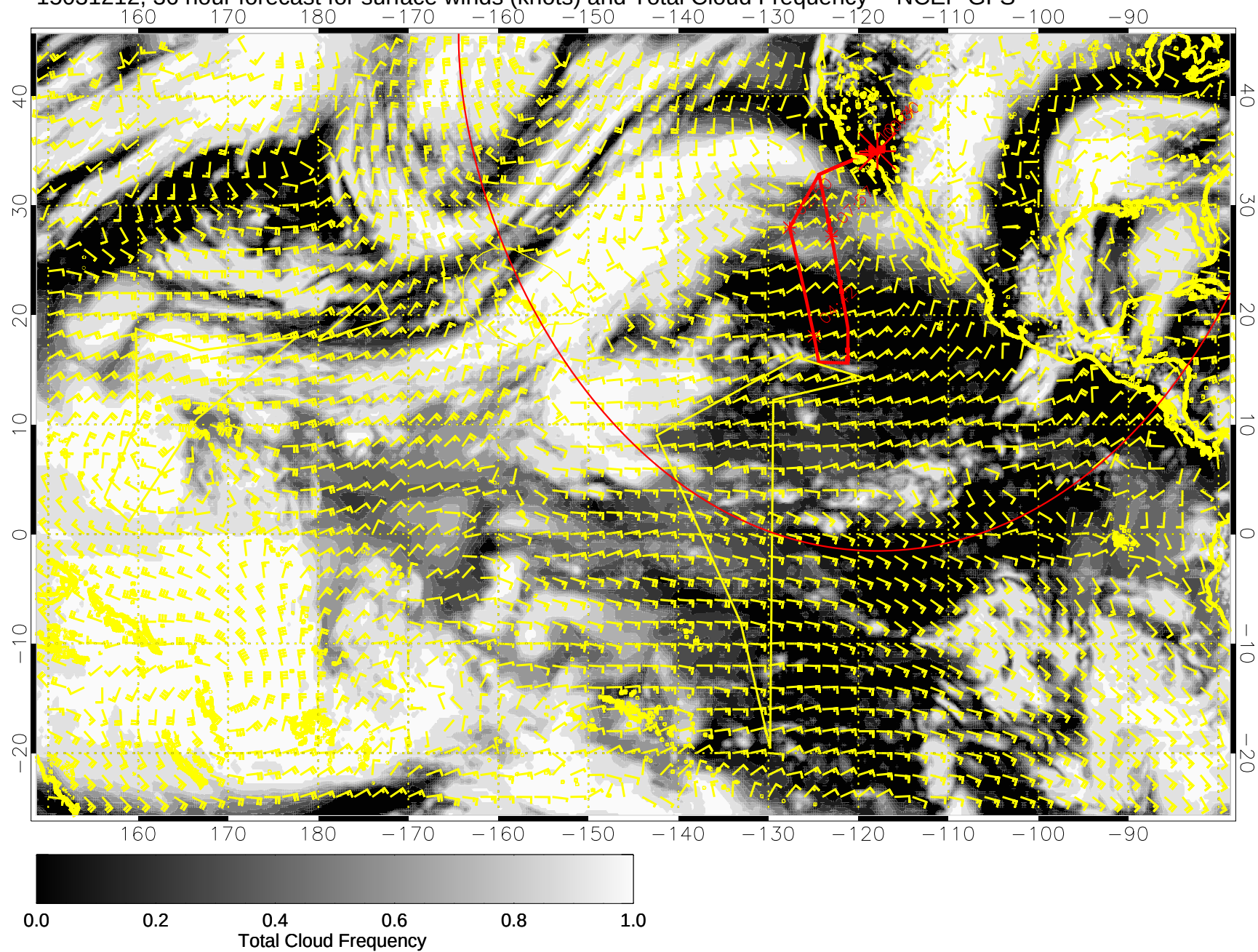
15031212, 36 hour forecast for surface winds (knots) and Total Cloud Frequency -- NCEP GFS
