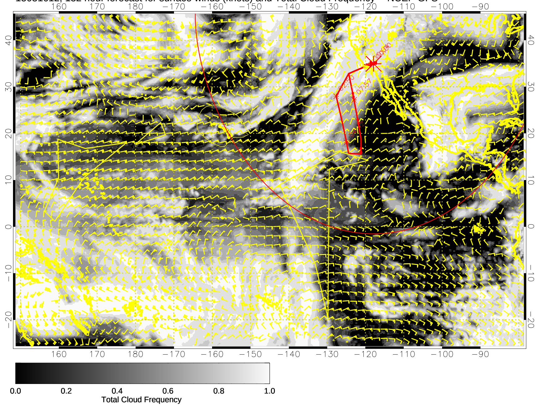
15031612, 132 hour forecast for surface winds (knots) and Total Cloud Frequency -- NCEP GFS
