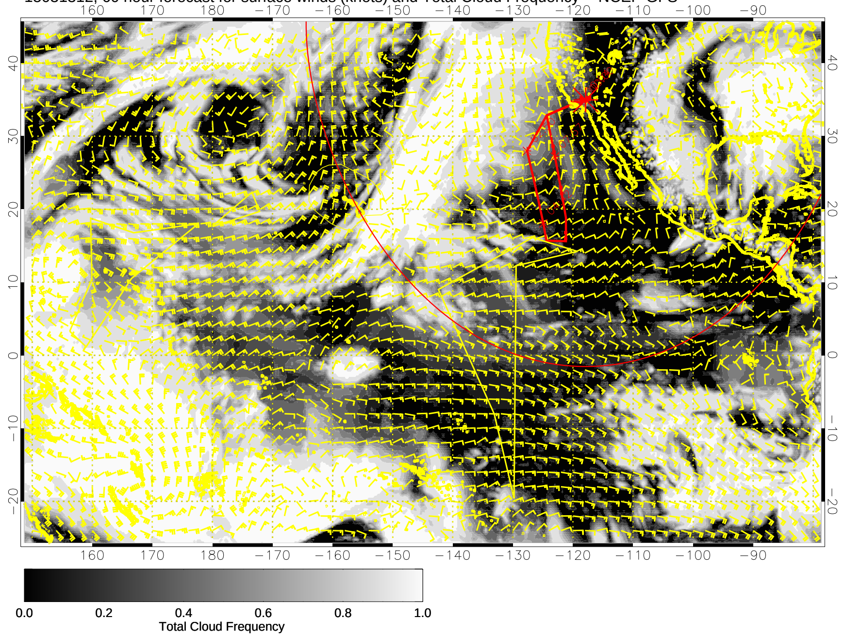
15031312, 60 hour forecast for surface winds (knots) and Total Cloud Frequency -- NCEP GFS
