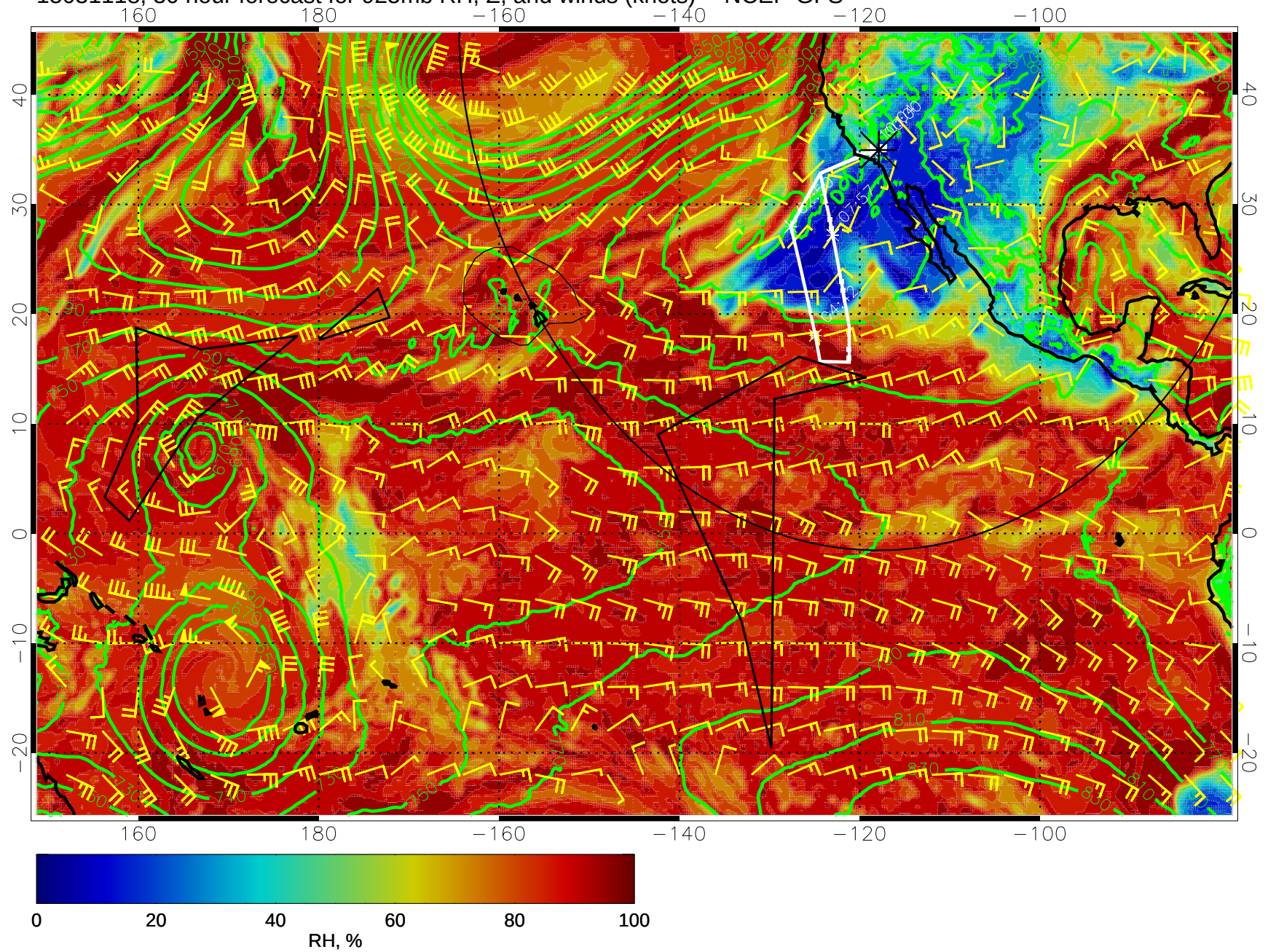
15031118, 30 hour forecast for 925mb RH, Z, and winds (knots) -- NCEP GFS
