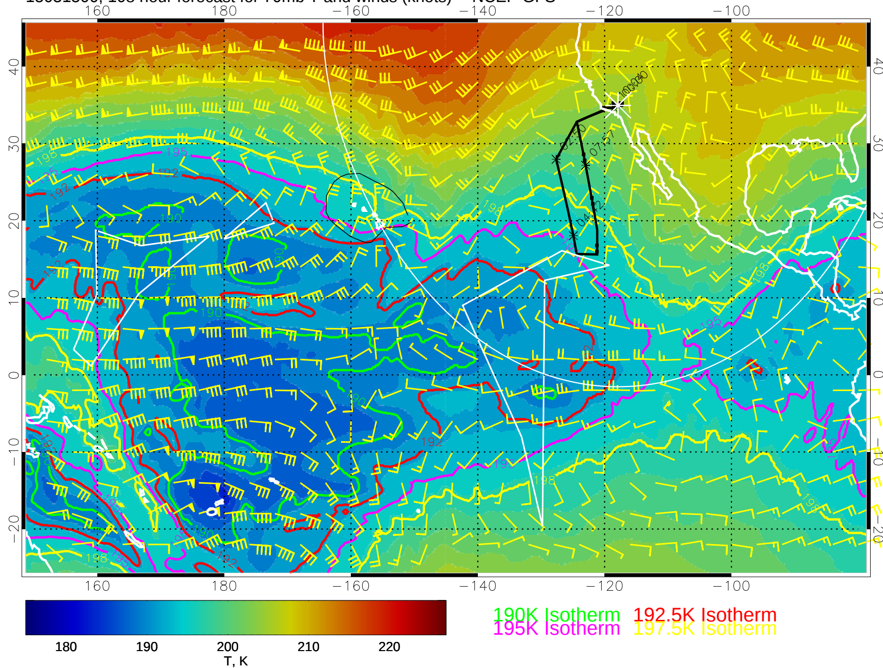
15031500, 108 hour forecast for 70mb T and winds (knots) -- NCEP GFS
