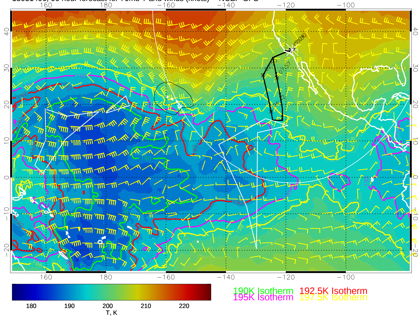
15031406, 90 hour forecast for 70mb T and winds (knots) -- NCEP GFS
