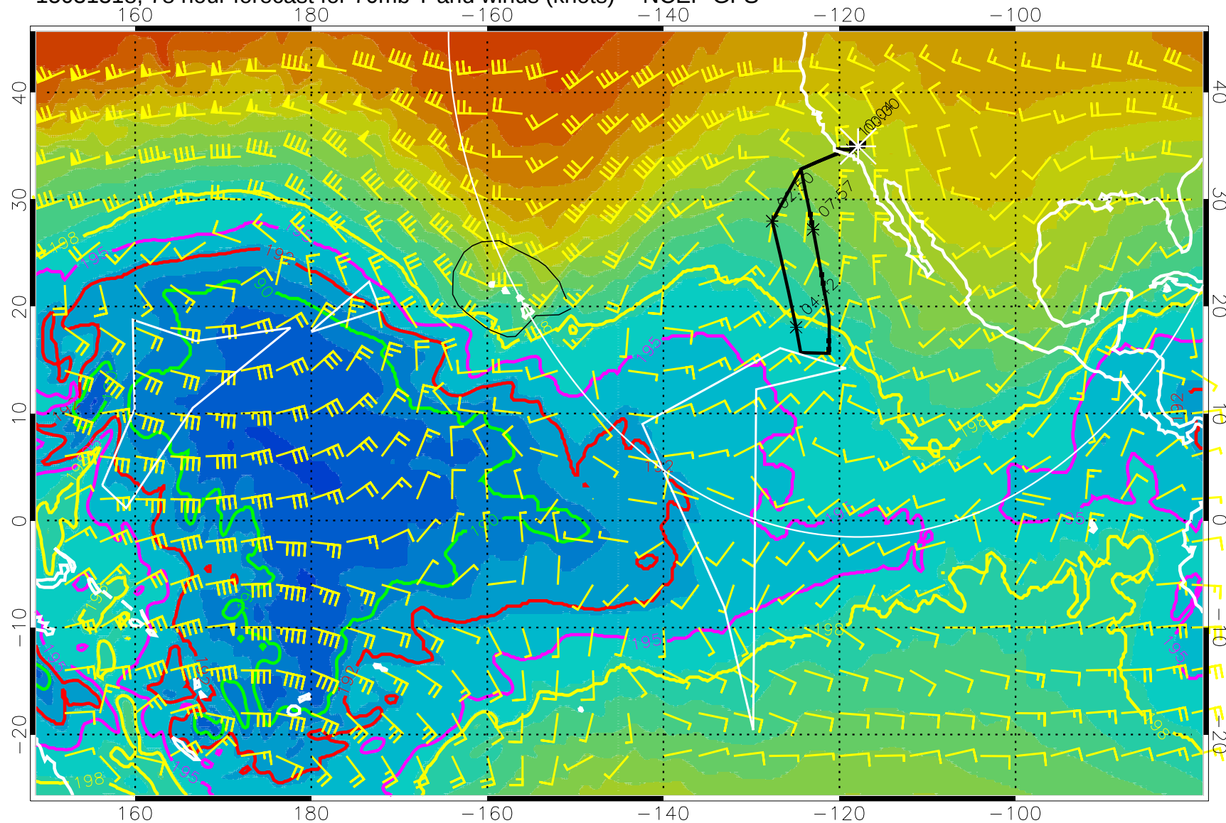
15031318, 78 hour forecast for 70mb T and winds (knots) -- NCEP GFS
