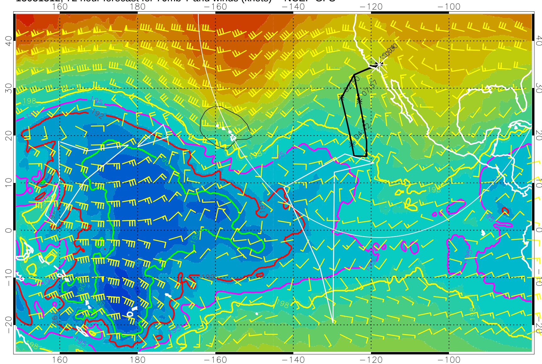
15031312, 72 hour forecast for 70mb T and winds (knots) -- NCEP GFS
