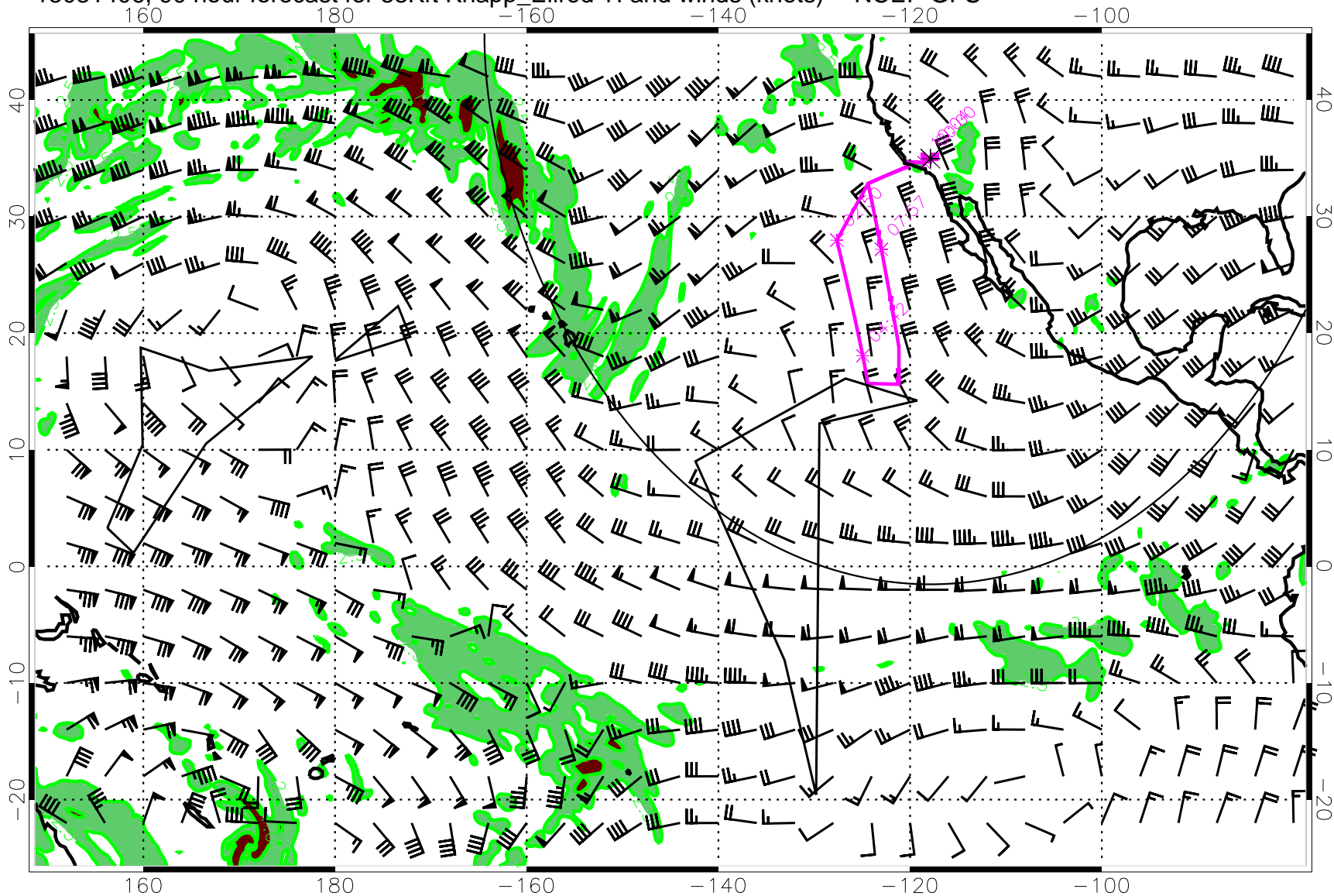
15031406, 90 hour forecast for 53Kft Knapp_Ellrod TI and winds (knots) -- NCEP GFS
