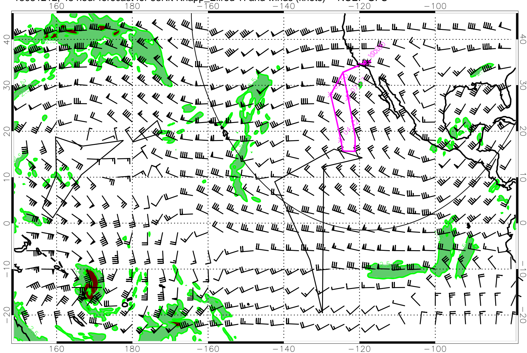
15031212, 48 hour forecast for 53Kft Knapp_Ellrod TI and winds (knots) -- NCEP GFS
