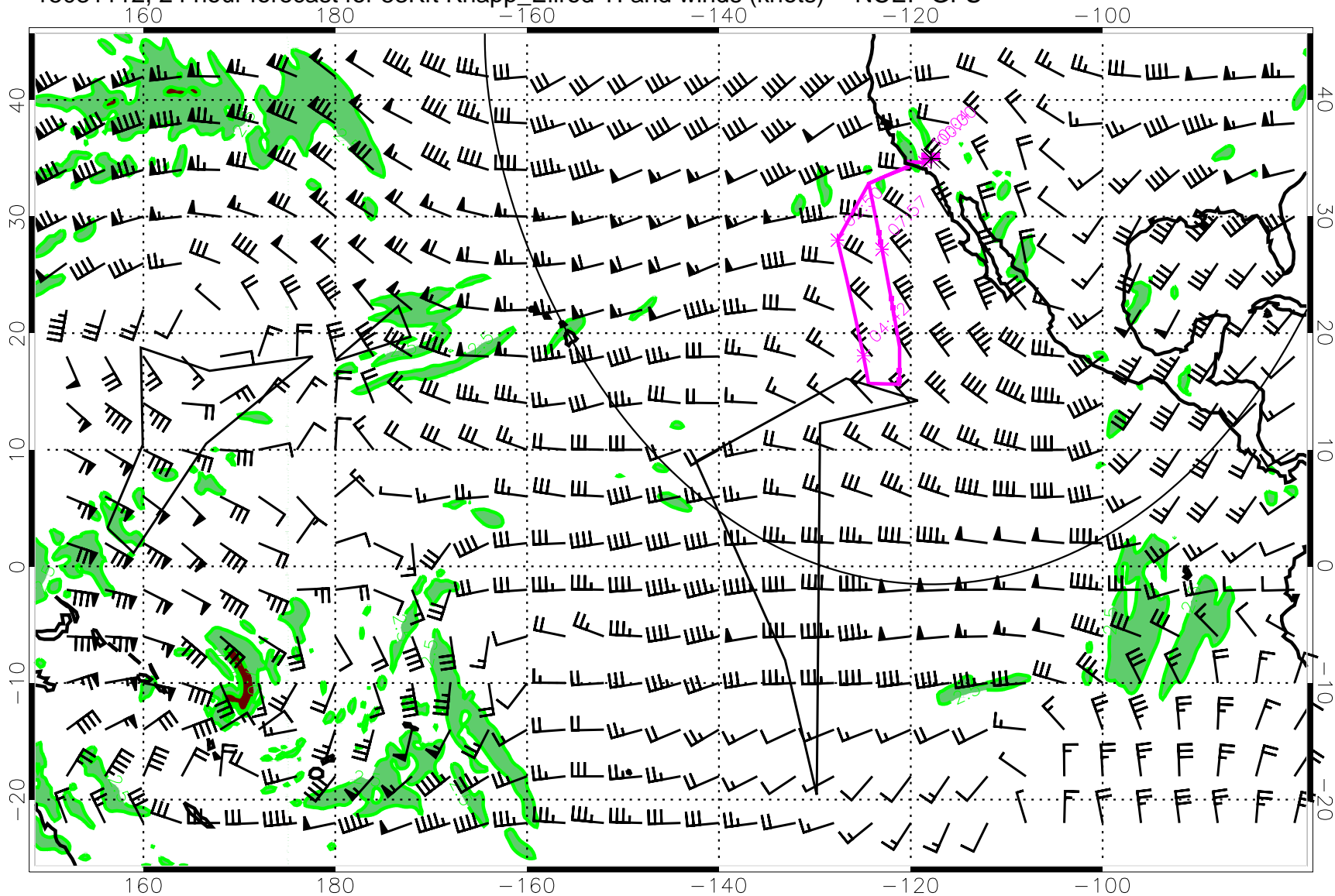
15031112, 24 hour forecast for 53Kft Knapp_Ellrod TI and winds (knots) -- NCEP GFS
