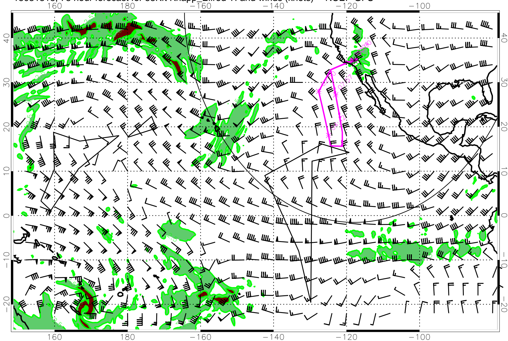
15031318, 78 hour forecast for 53Kft Knapp_Ellrod TI and winds (knots) -- NCEP GFS
