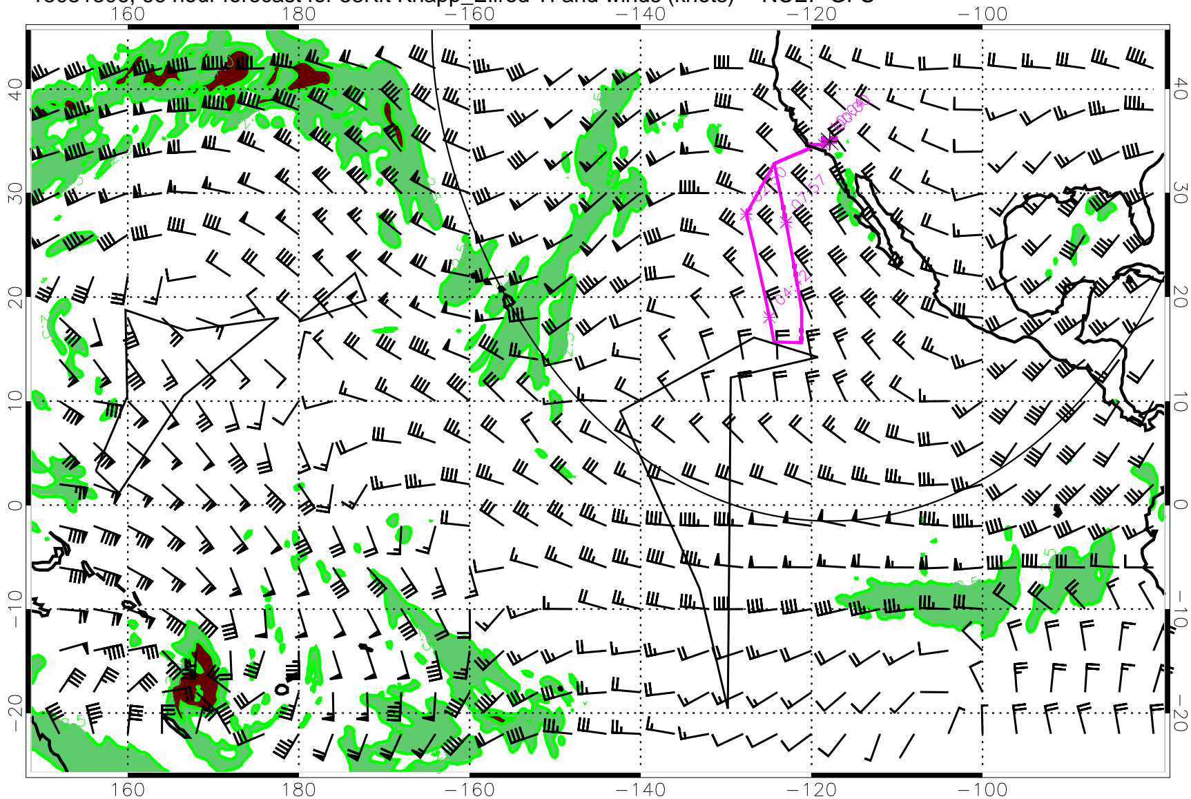
15031306, 66 hour forecast for 53Kft Knapp_Ellrod TI and winds (knots) -- NCEP GFS
