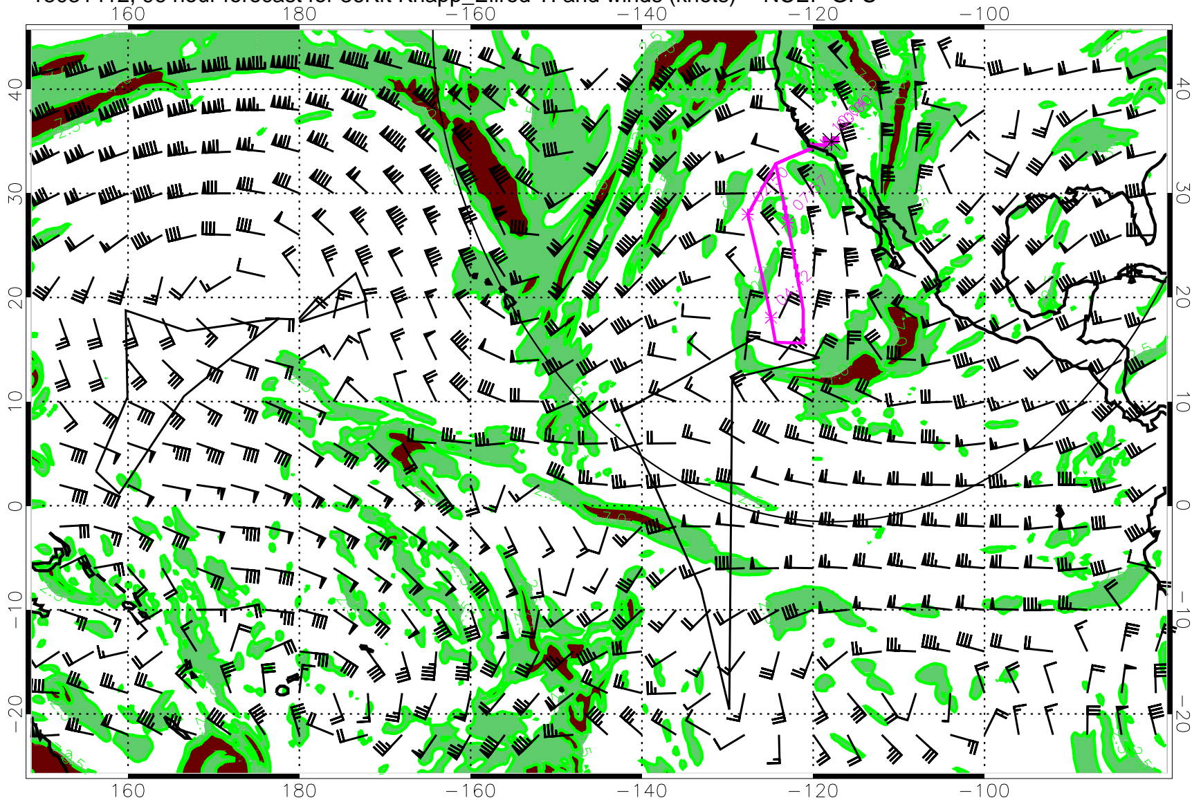
15031412, 96 hour forecast for 36Kft Knapp_Ellrod TI and winds (knots) -- NCEP GFS
