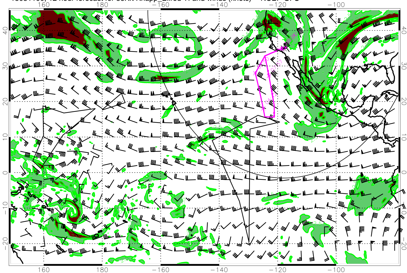
15031100, 12 hour forecast for 36Kft Knapp_Ellrod TI and winds (knots) -- NCEP GFS
