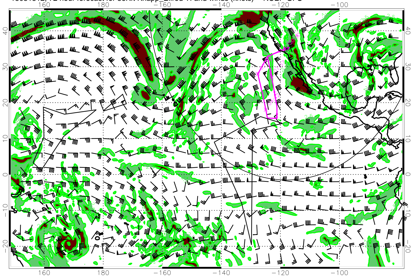
15031312, 72 hour forecast for 36Kft Knapp_Ellrod TI and winds (knots) -- NCEP GFS
