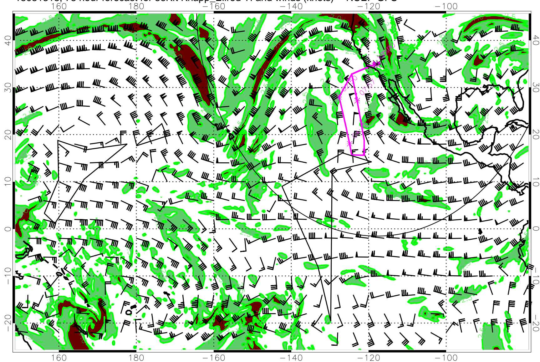
15031318, 78 hour forecast for 36Kft Knapp_Ellrod TI and winds (knots) -- NCEP GFS
