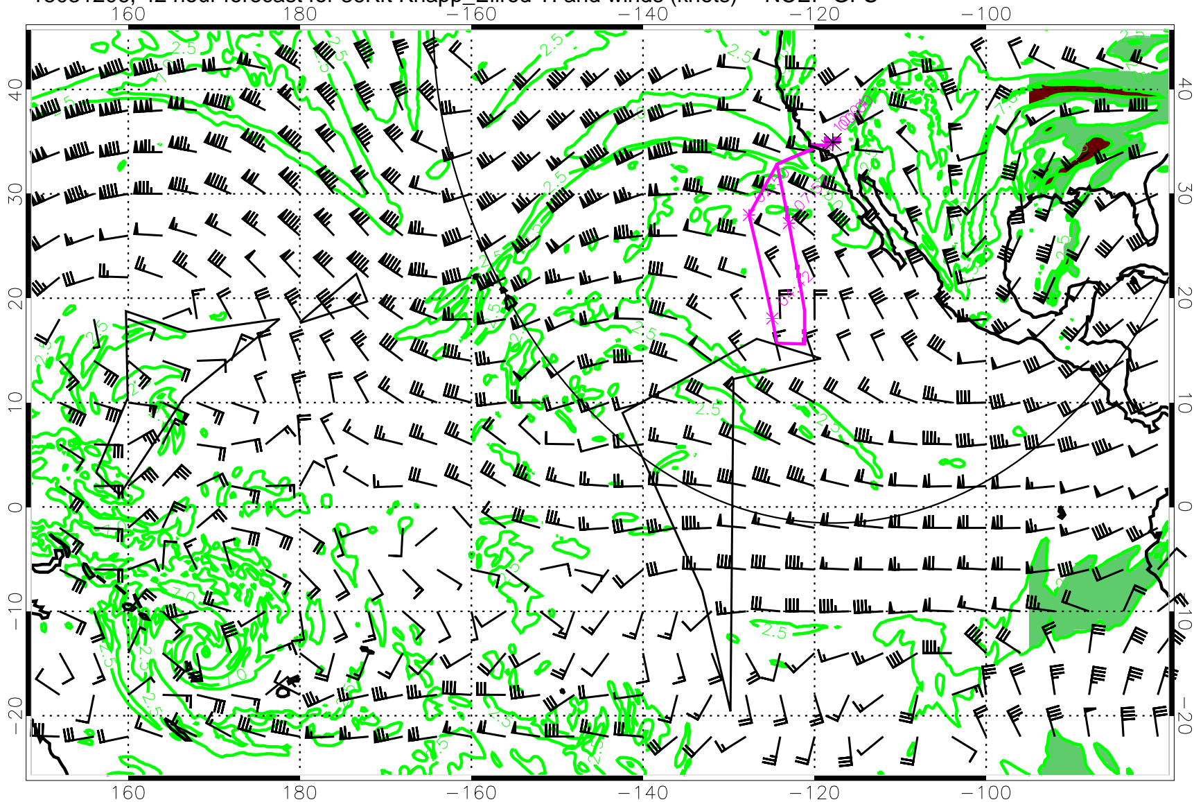
15031206, 42 hour forecast for 36Kft Knapp_Ellrod TI and winds (knots) -- NCEP GFS
