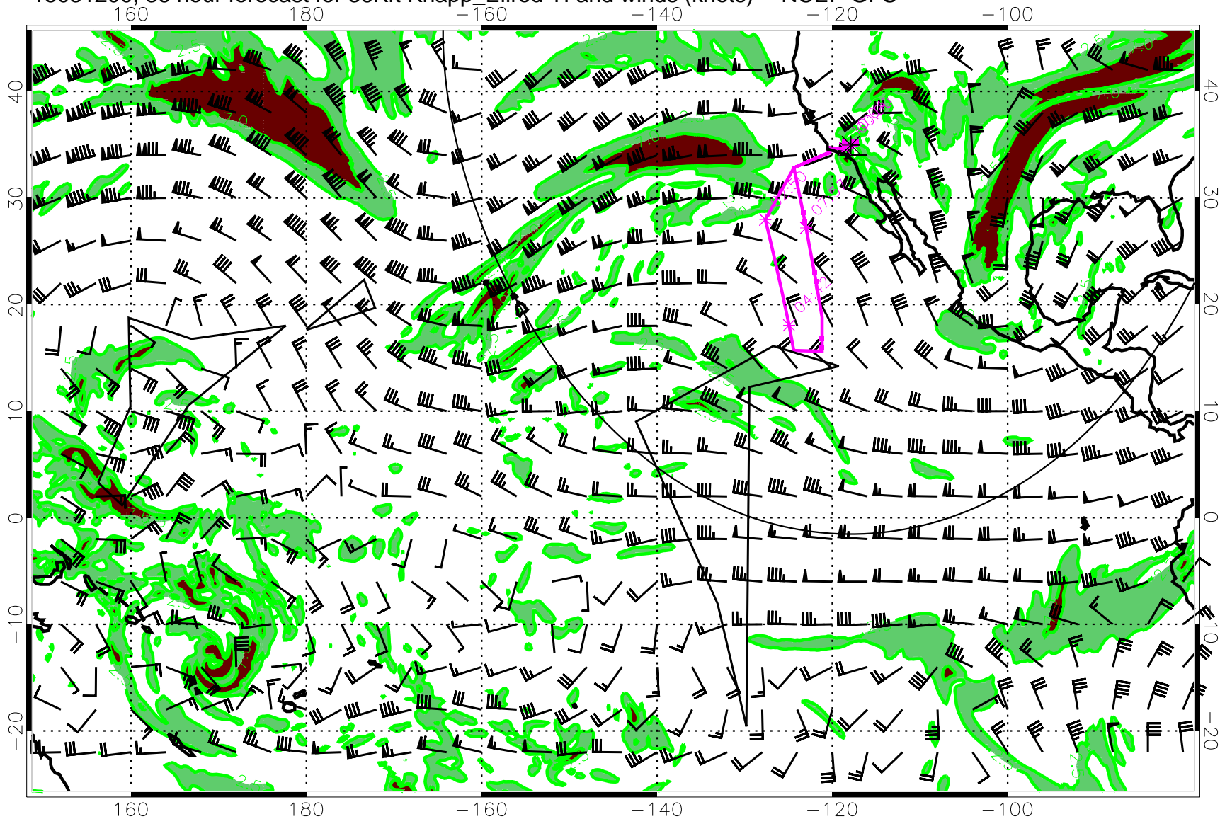
15031200, 36 hour forecast for 36Kft Knapp_Ellrod TI and winds (knots) -- NCEP GFS
