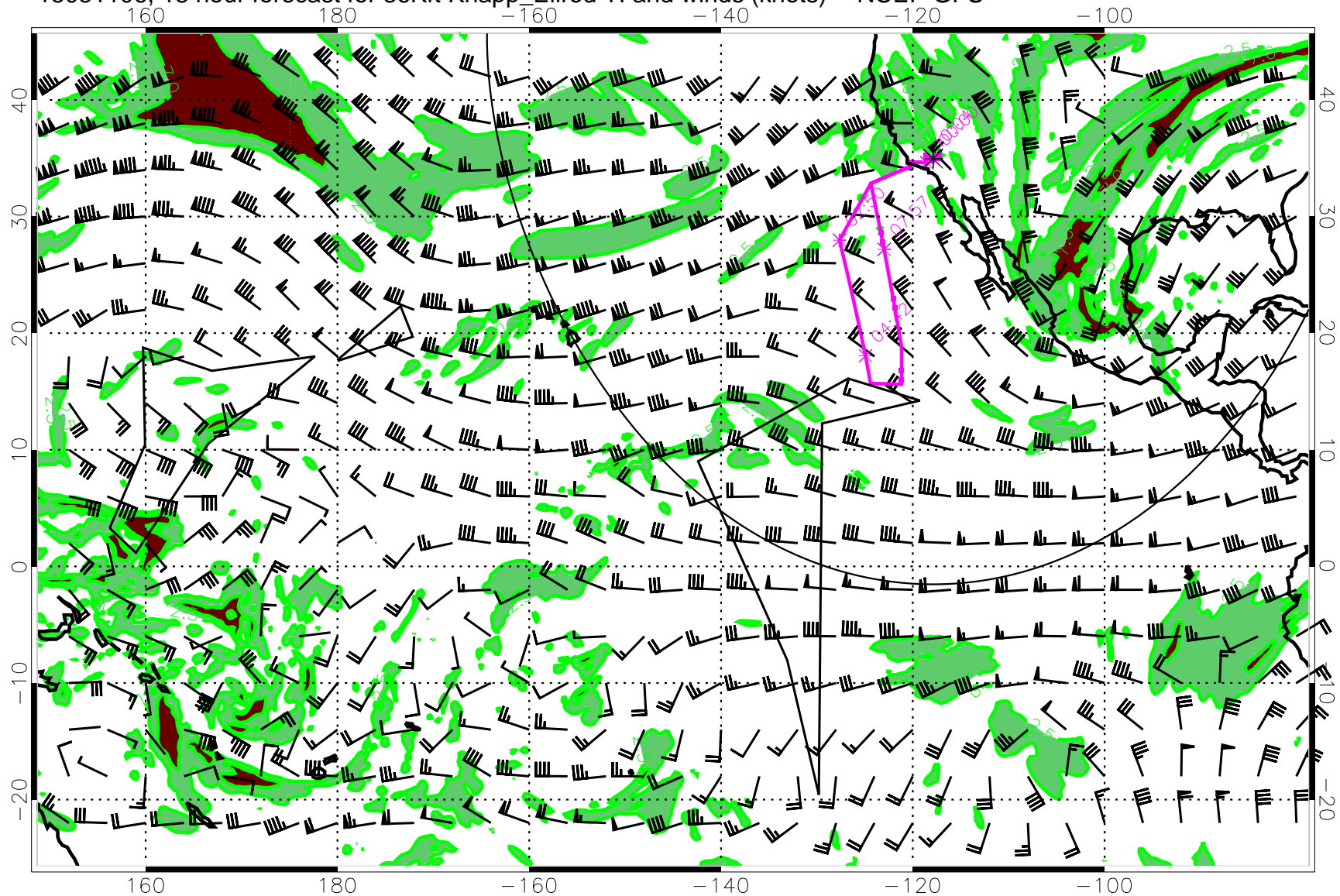
15031106, 18 hour forecast for 36Kft Knapp_Ellrod TI and winds (knots) -- NCEP GFS
