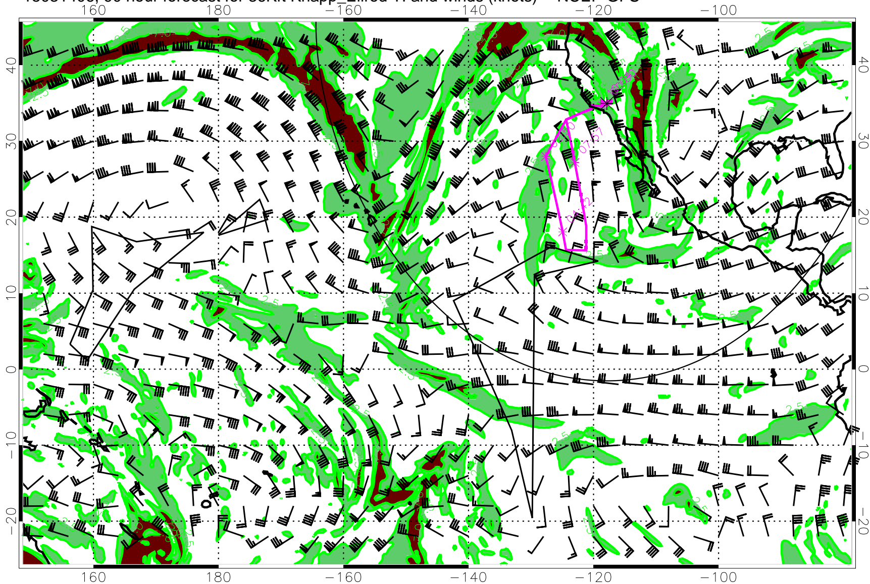
15031406, 90 hour forecast for 36Kft Knapp_Ellrod TI and winds (knots) -- NCEP GFS
