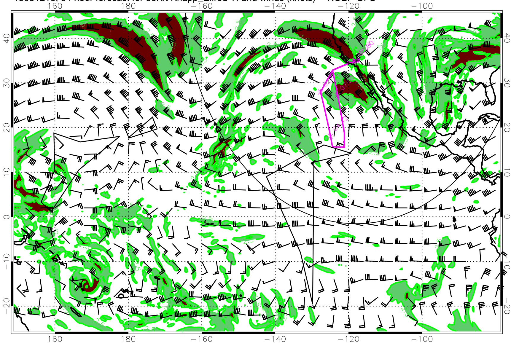
15031218, 54 hour forecast for 36Kft Knapp_Ellrod TI and winds (knots) -- NCEP GFS
