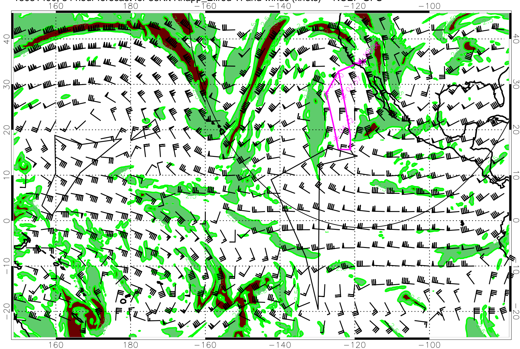
15031400, 84 hour forecast for 36Kft Knapp_Ellrod TI and winds (knots) -- NCEP GFS
