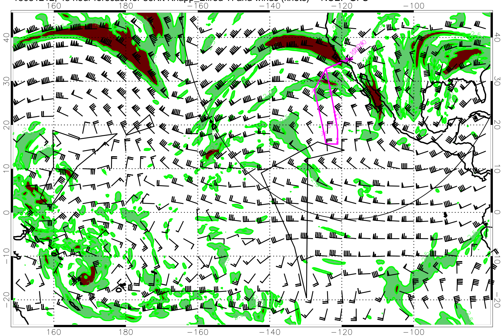
15031212, 48 hour forecast for 36Kft Knapp_Ellrod TI and winds (knots) -- NCEP GFS
