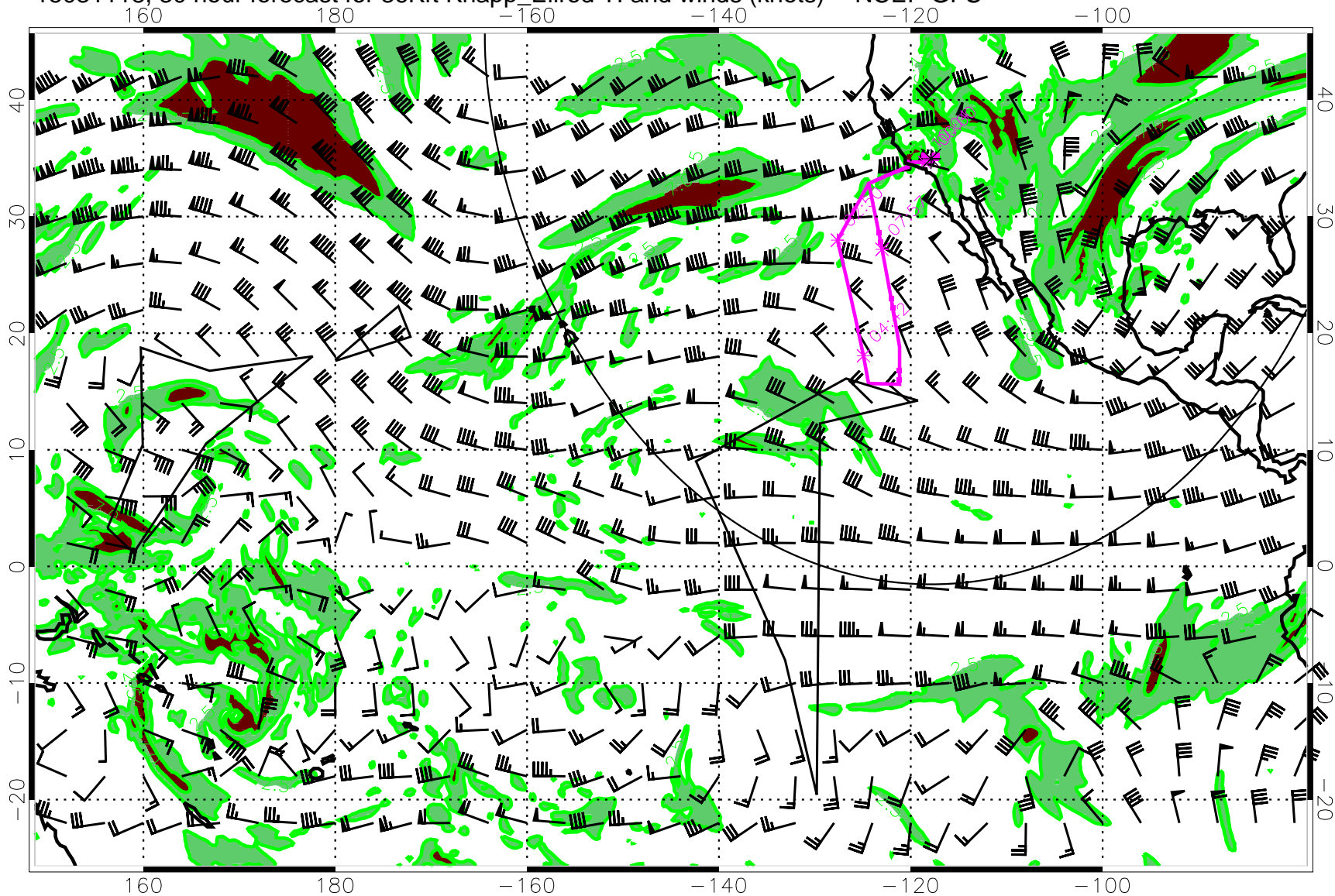
15031118, 30 hour forecast for 36Kft Knapp_Ellrod TI and winds (knots) -- NCEP GFS
