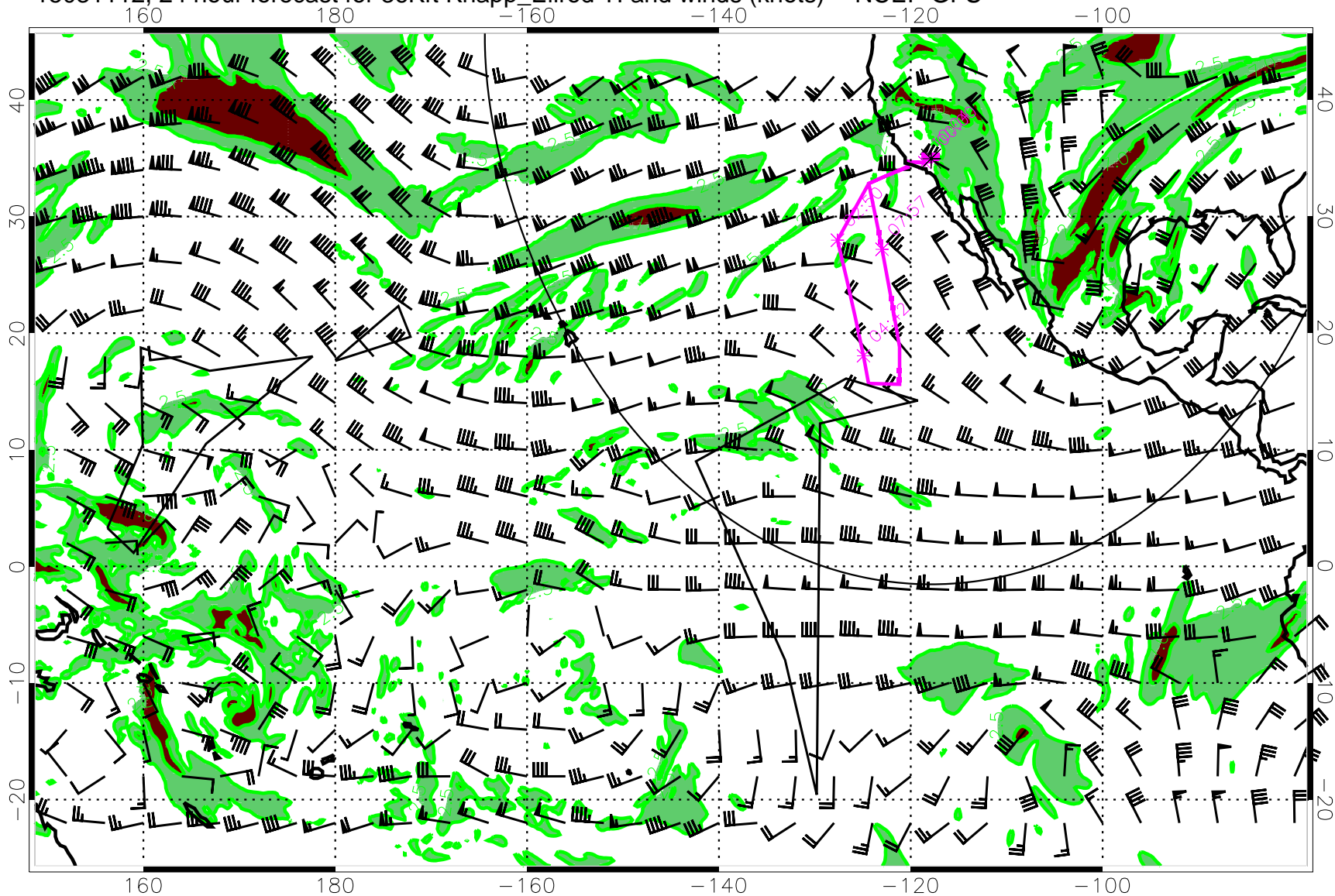
15031112, 24 hour forecast for 36Kft Knapp_Ellrod TI and winds (knots) -- NCEP GFS
