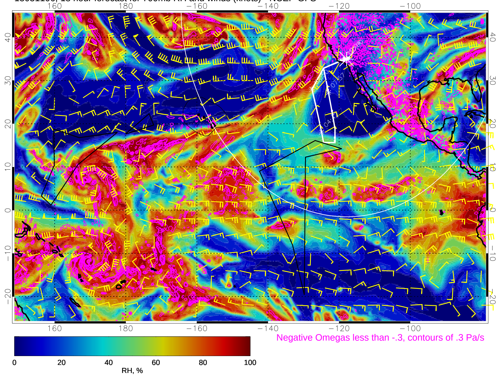
15031106, 18 hour forecast for 700mb RH and winds (knots) - NCEP GFS
