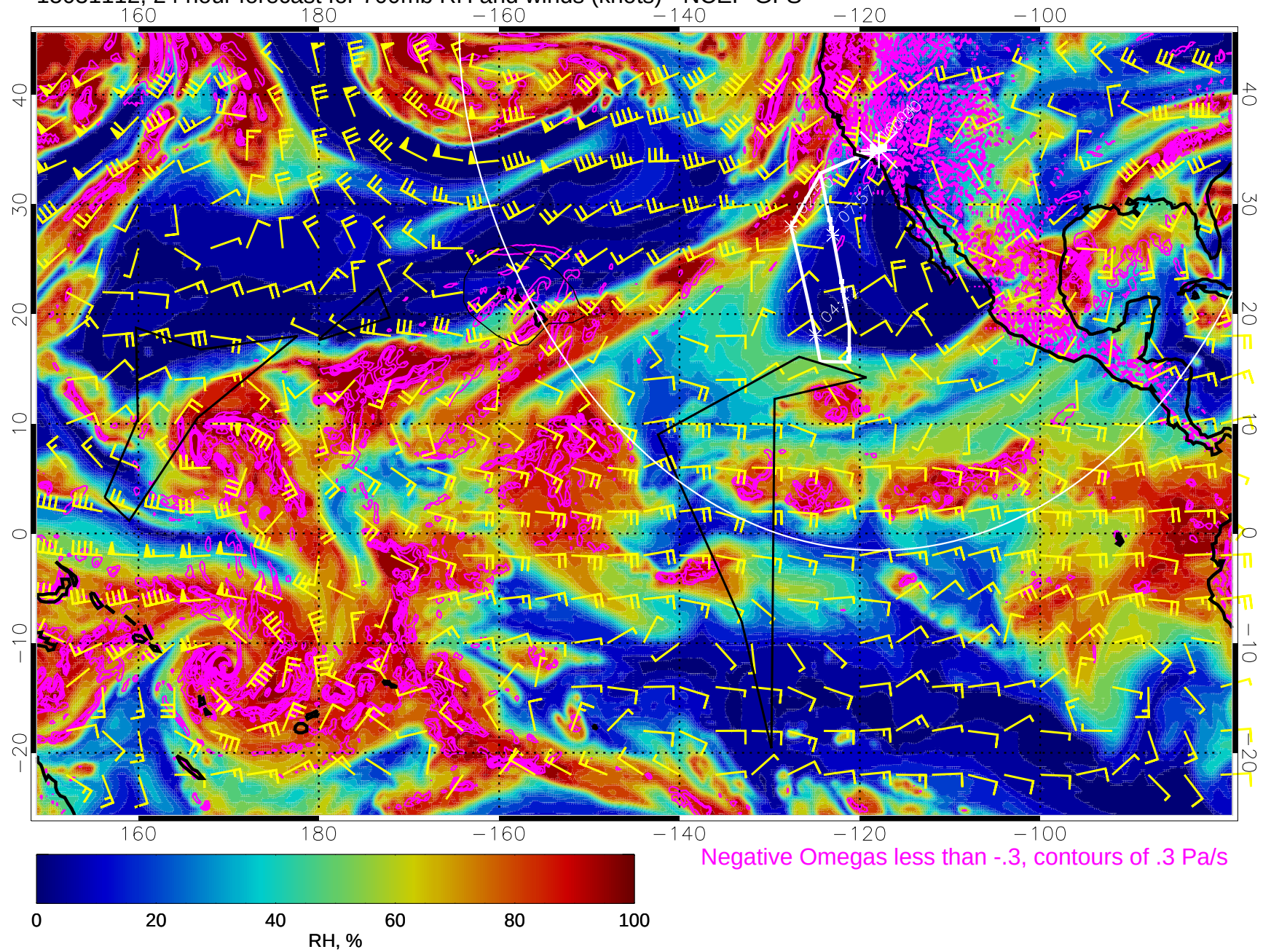
15031112, 24 hour forecast for 700mb RH and winds (knots) - NCEP GFS
