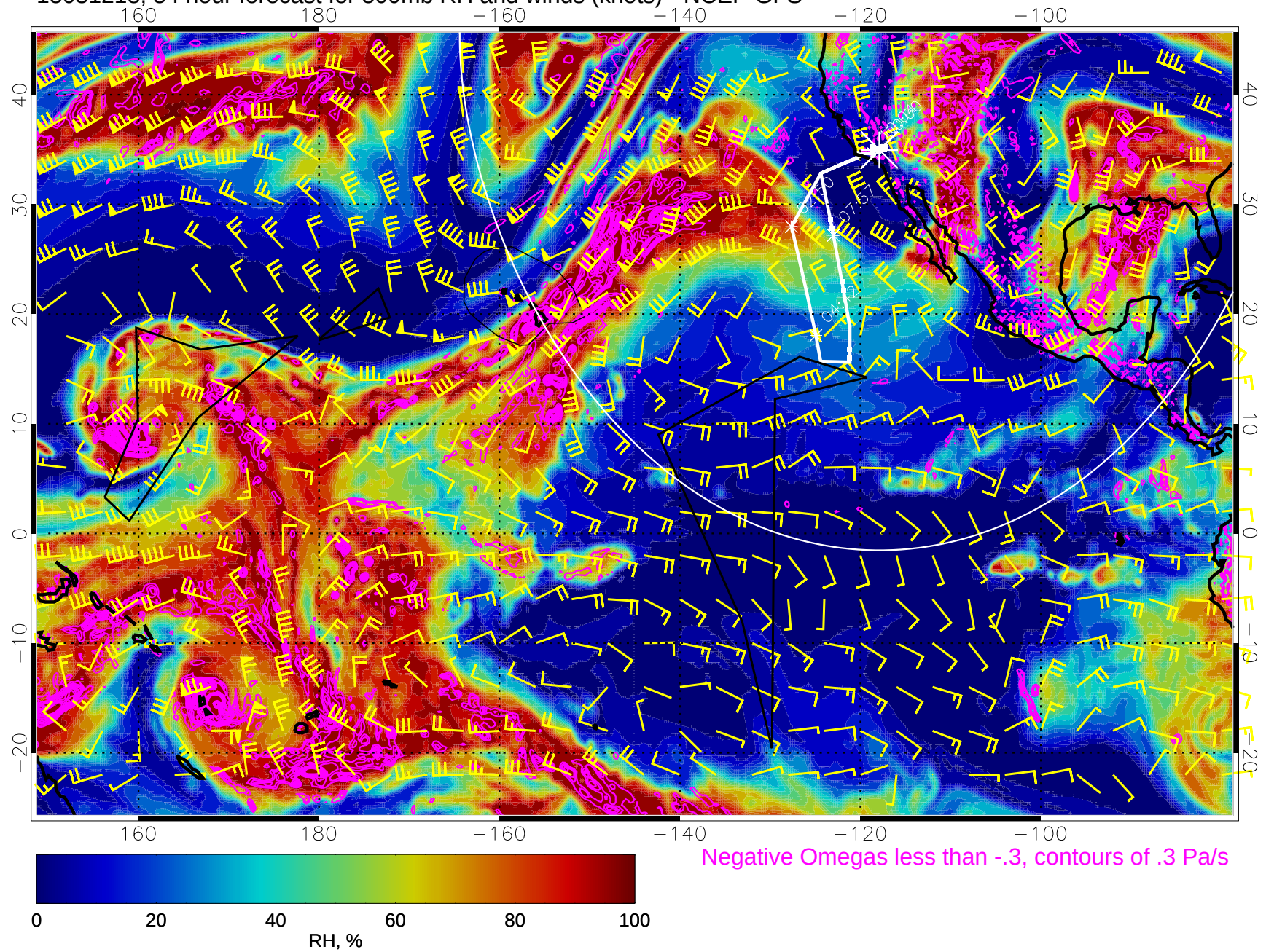
15031218, 54 hour forecast for 500mb RH and winds (knots) - NCEP GFS
