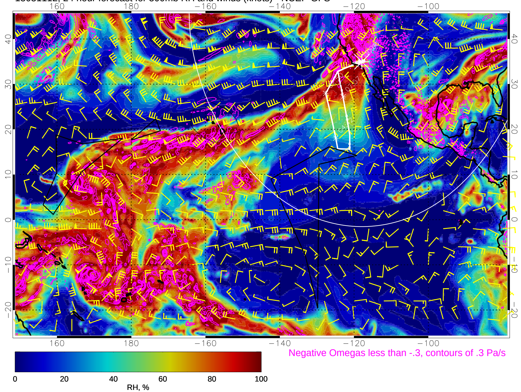
15031112, 24 hour forecast for 500mb RH and winds (knots) - NCEP GFS
