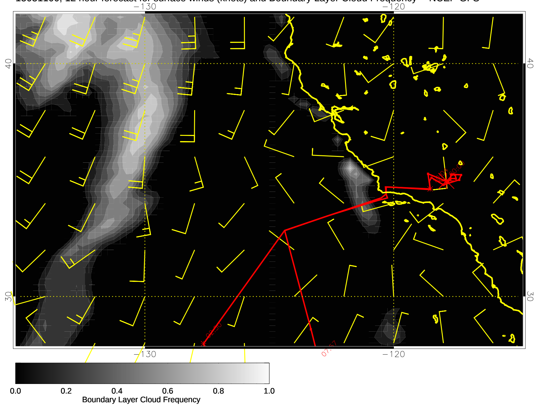
15031100, 12 hour forecast for surface winds (knots) and Boundary Layer Cloud Frequency -- NCEP GFS
