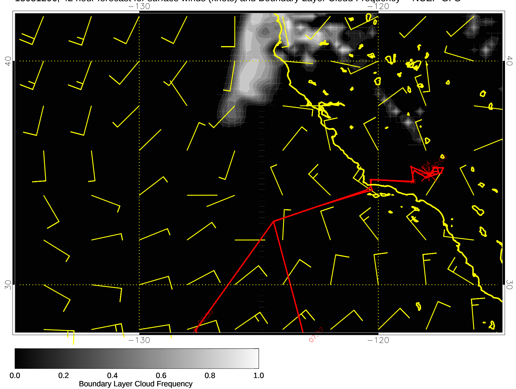
15031206, 42 hour forecast for surface winds (knots) and Boundary Layer Cloud Frequency -- NCEP GFS
