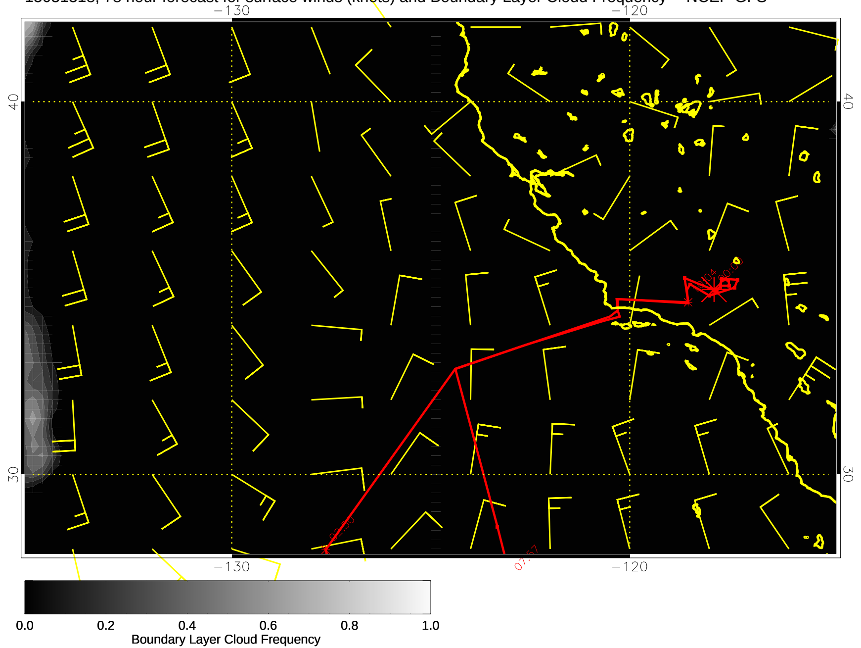
15031318, 78 hour forecast for surface winds (knots) and Boundary Layer Cloud Frequency -- NCEP GFS
