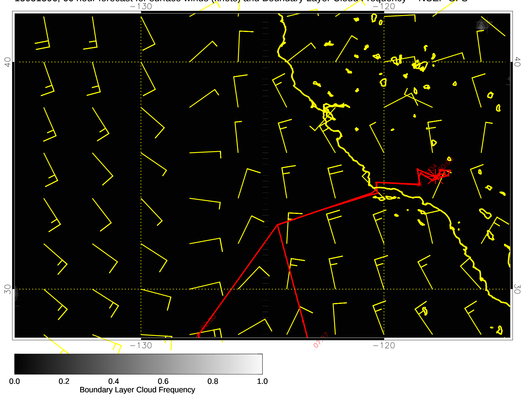
15031306, 66 hour forecast for surface winds (knots) and Boundary Layer Cloud Frequency -- NCEP GFS
