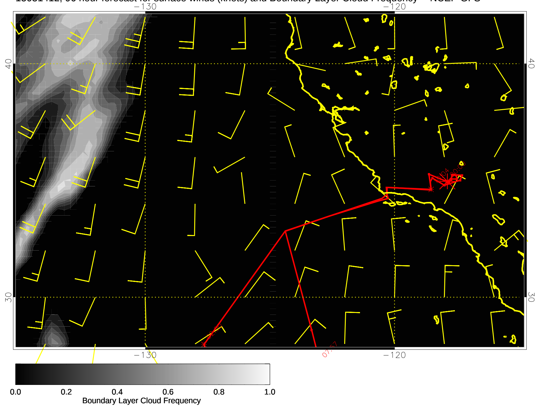
15031412, 96 hour forecast for surface winds (knots) and Boundary Layer Cloud Frequency -- NCEP GFS
