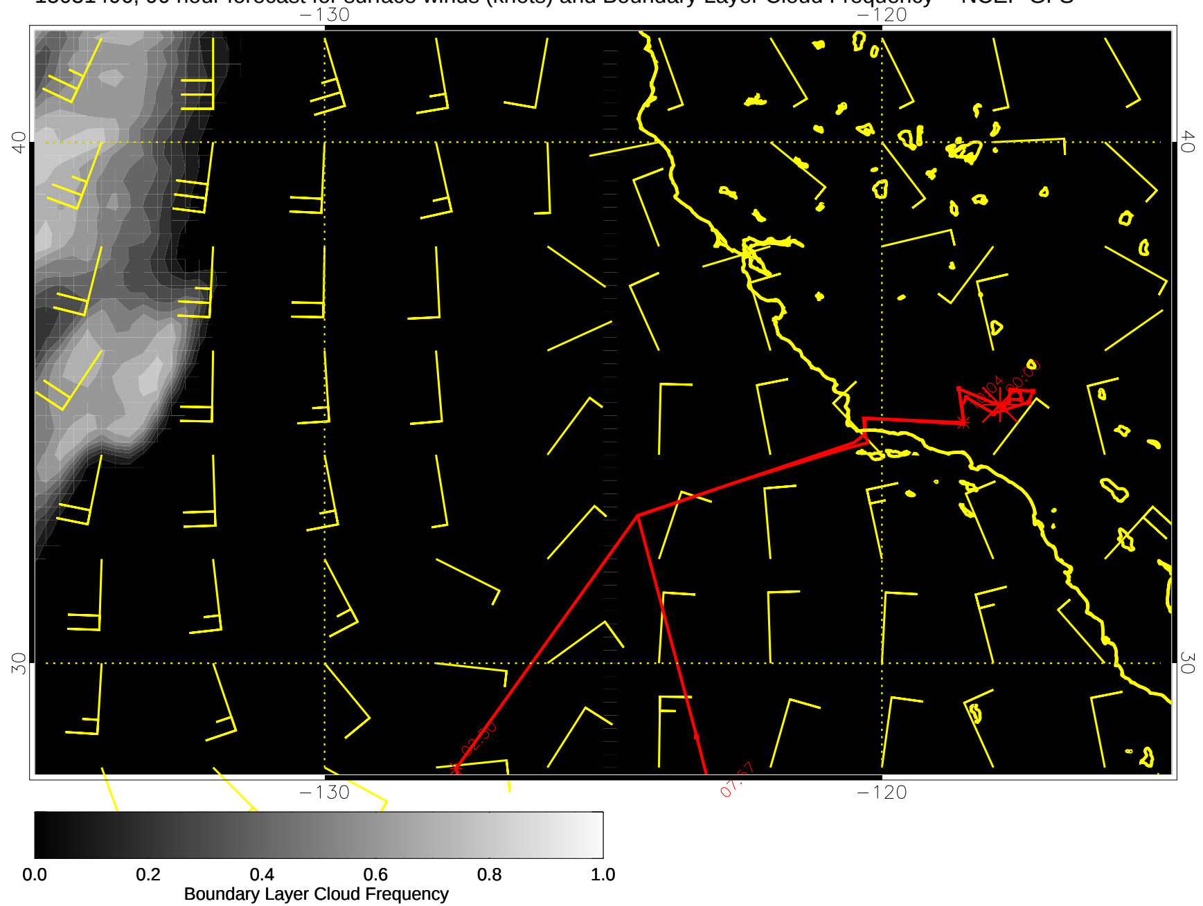
15031406, 90 hour forecast for surface winds (knots) and Boundary Layer Cloud Frequency -- NCEP GFS
