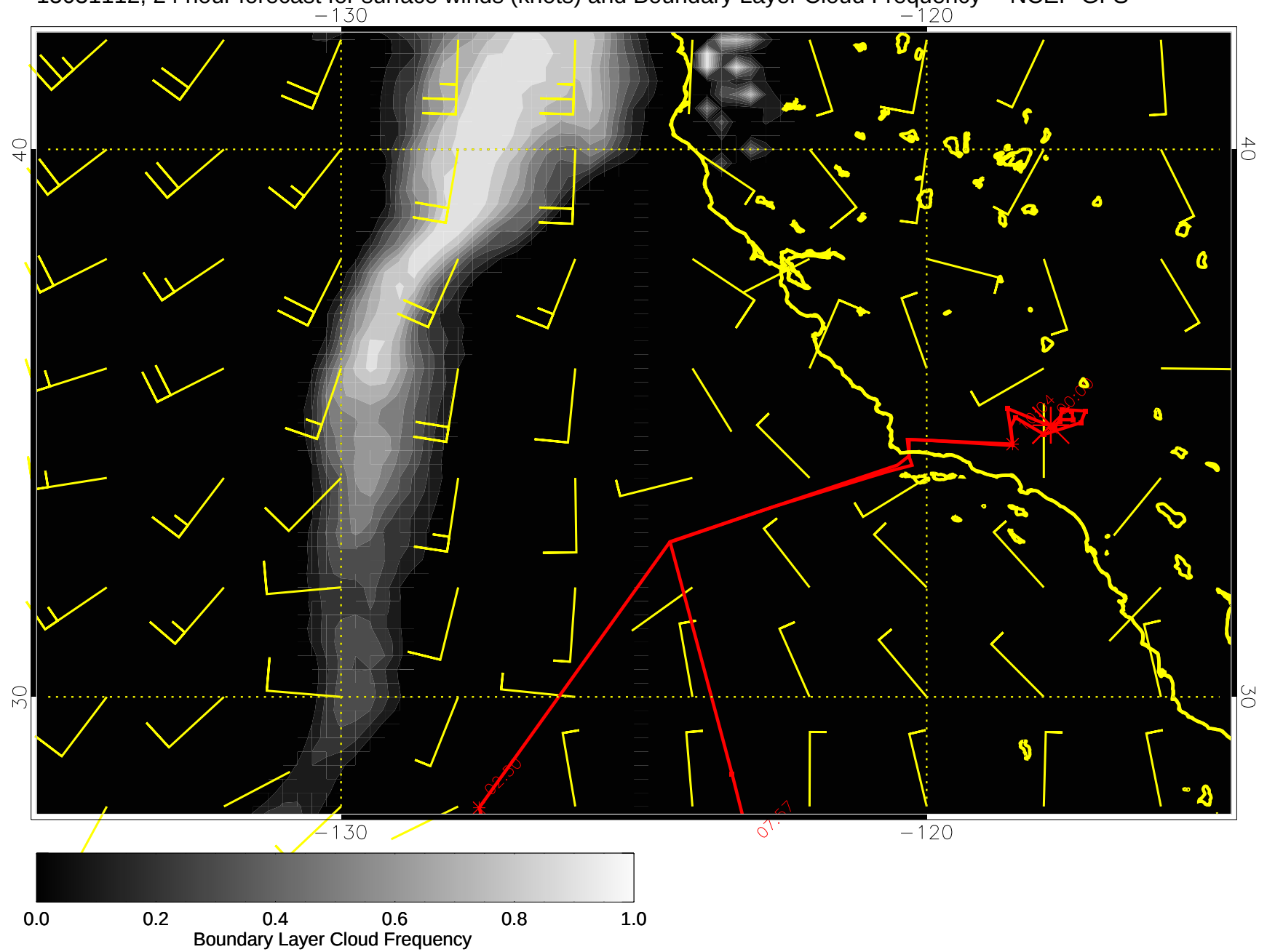
15031112, 24 hour forecast for surface winds (knots) and Boundary Layer Cloud Frequency -- NCEP GFS
