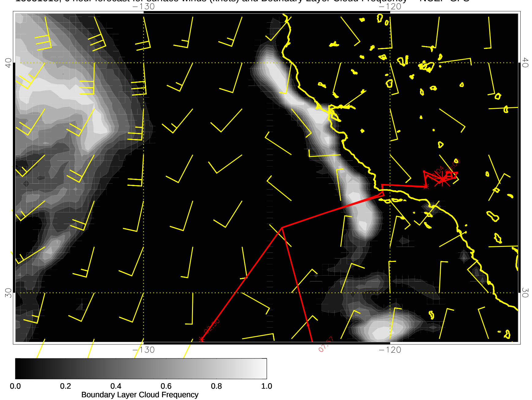
15031018, 6 hour forecast for surface winds (knots) and Boundary Layer Cloud Frequency -- NCEP GFS
