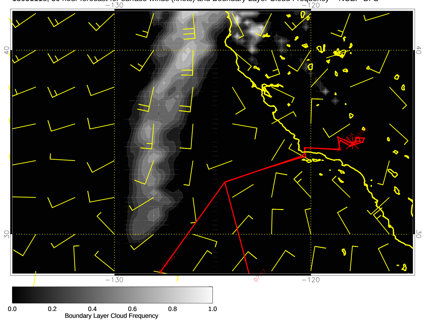
15031118, 30 hour forecast for surface winds (knots) and Boundary Layer Cloud Frequency -- NCEP GFS
