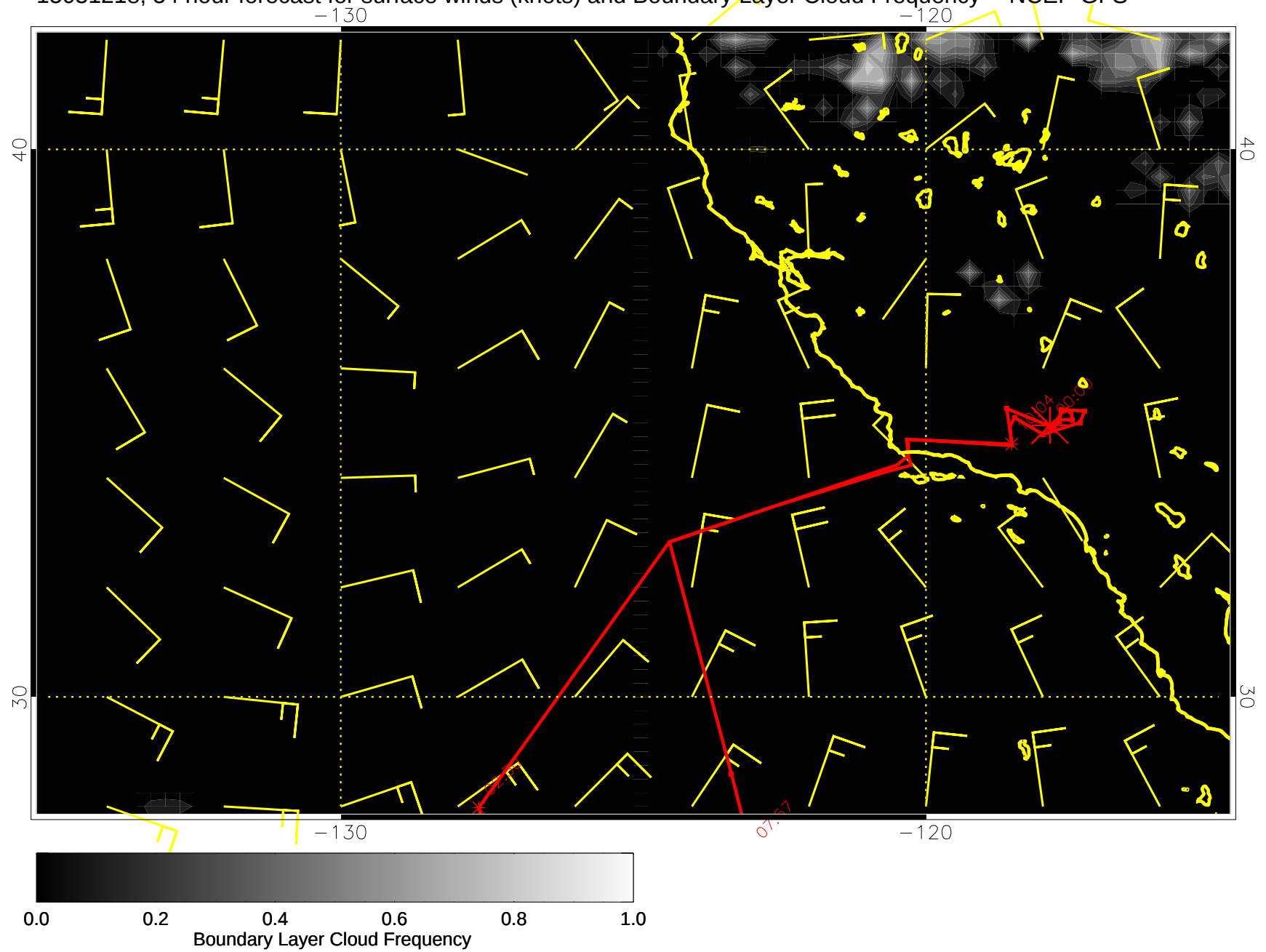
15031218, 54 hour forecast for surface winds (knots) and Boundary Layer Cloud Frequency -- NCEP GFS
