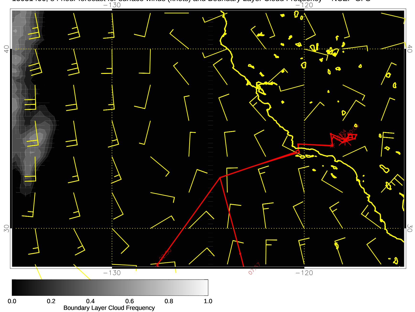
15031400, 84 hour forecast for surface winds (knots) and Boundary Layer Cloud Frequency -- NCEP GFS
