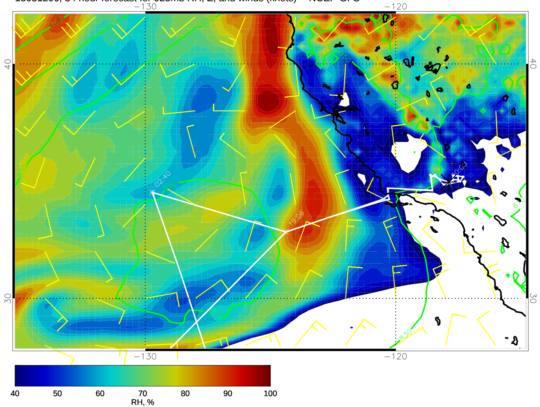
15031206, 54 hour forecast for 925mb RH, Z, and winds (knots) -- NCEP GFS
