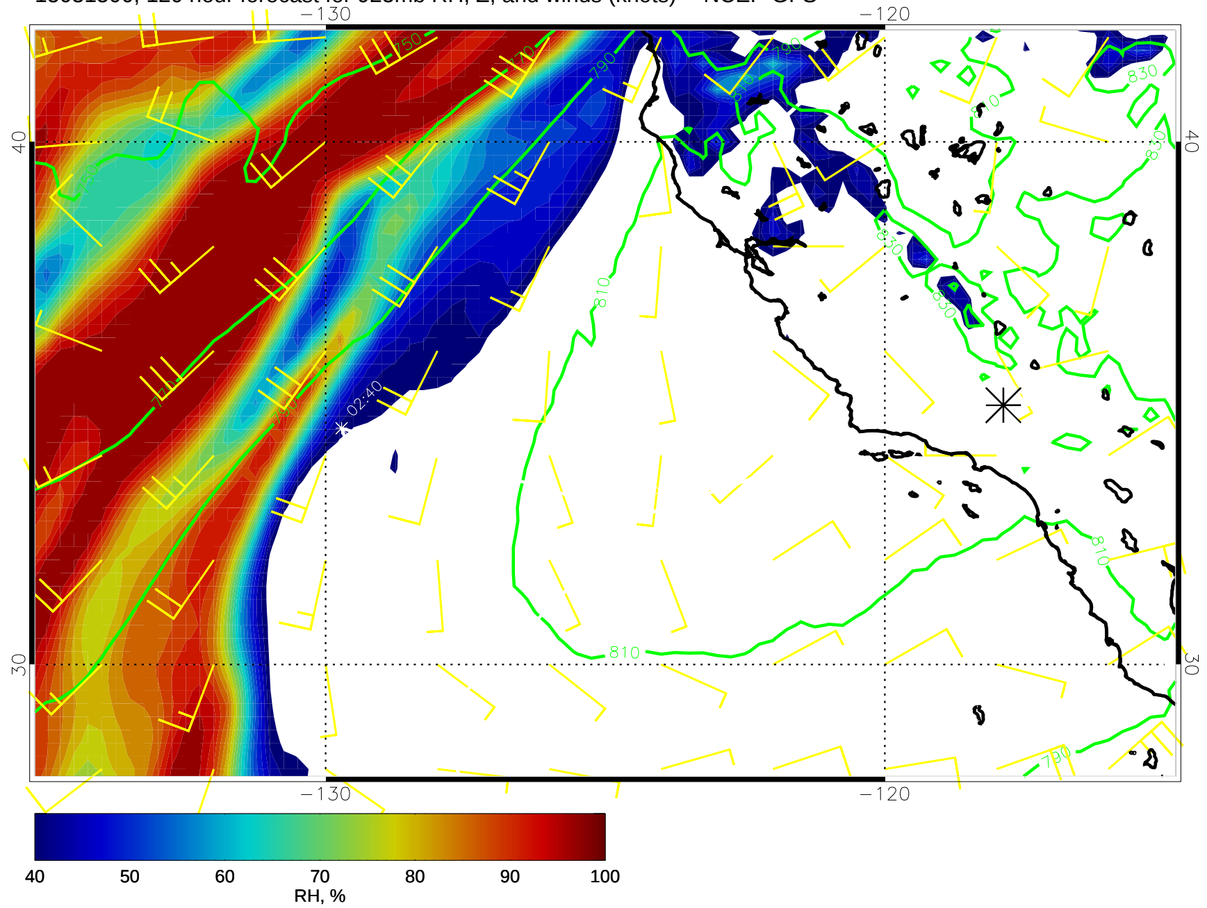
15031500, 120 hour forecast for 925mb RH, Z, and winds (knots) -- NCEP GFS
