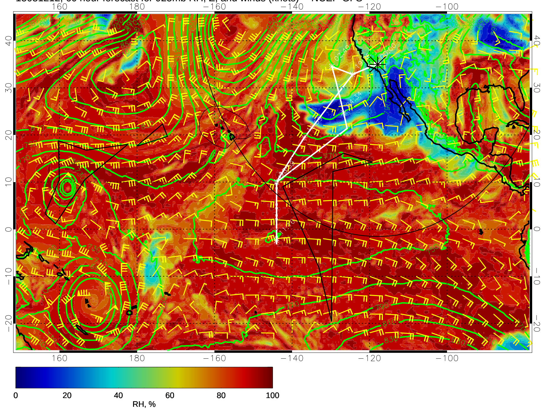
15031212, 60 hour forecast for 925mb RH, Z, and winds (knots) -- NCEP GFS
