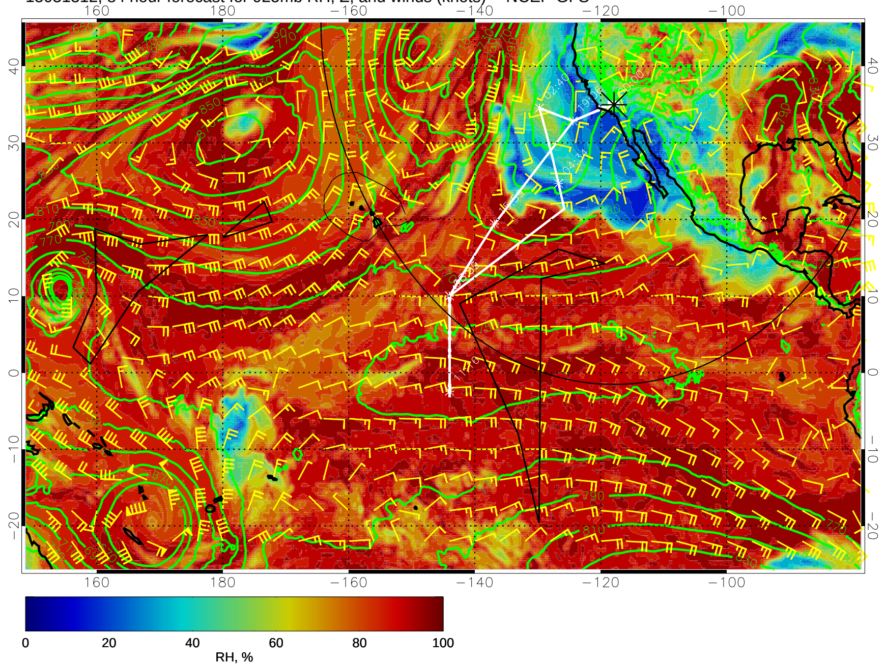
15031312, 84 hour forecast for 925mb RH, Z, and winds (knots) -- NCEP GFS
