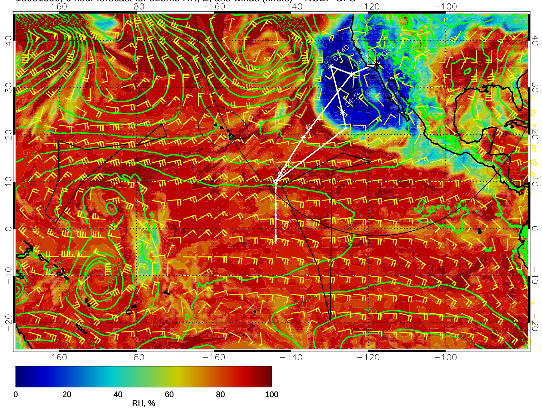
15031006, 6 hour forecast for 925mb RH, Z, and winds (knots) -- NCEP GFS
