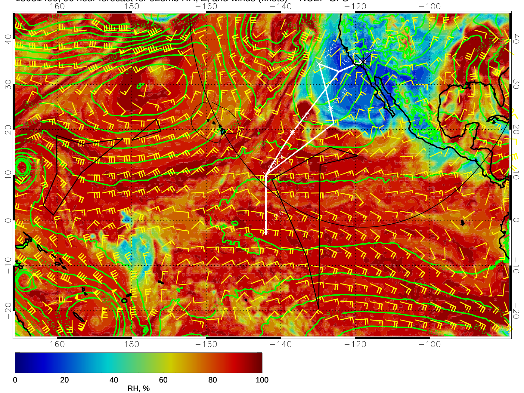
15031400, 96 hour forecast for 925mb RH, Z, and winds (knots) -- NCEP GFS
