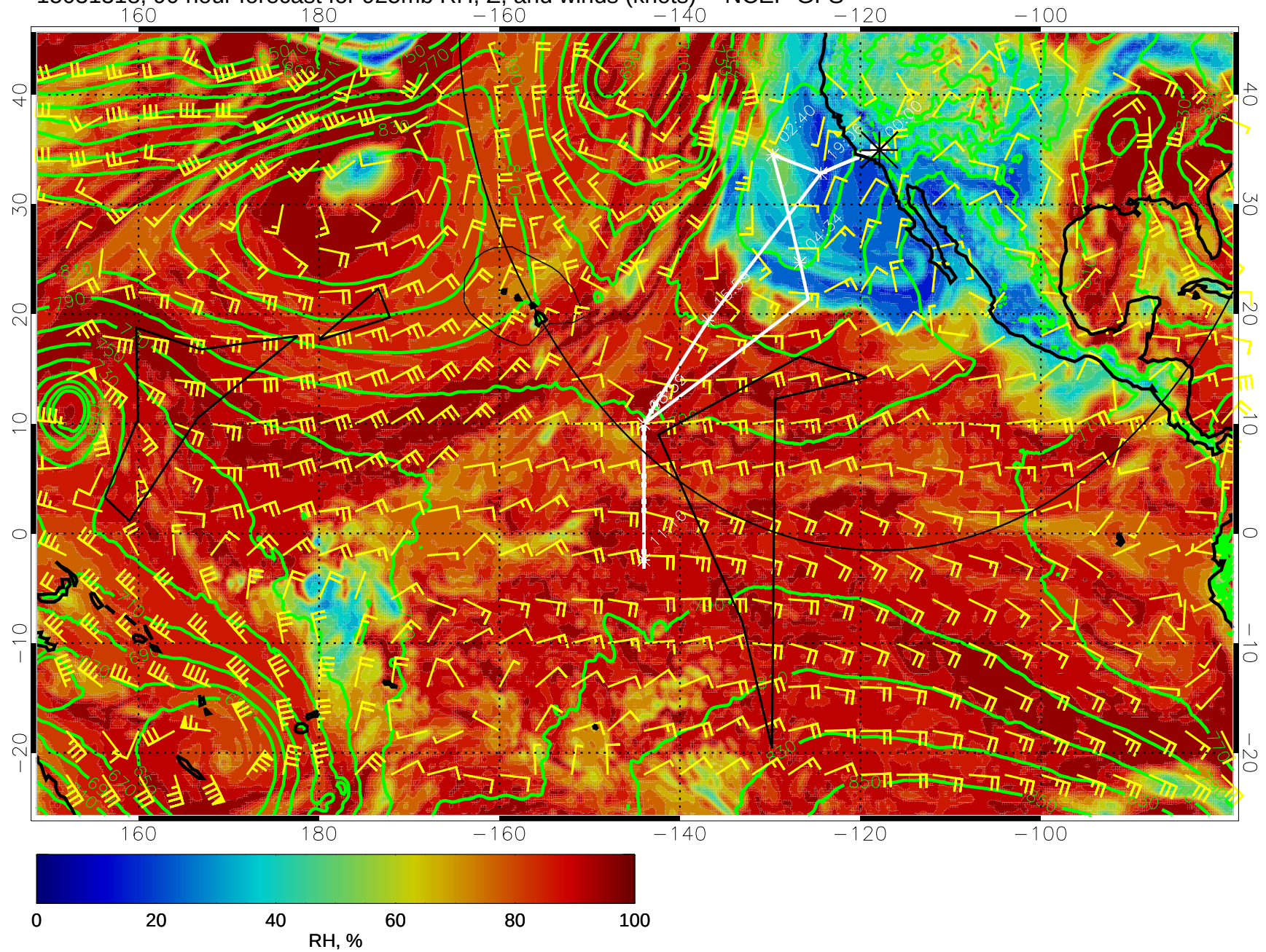
15031318, 90 hour forecast for 925mb RH, Z, and winds (knots) -- NCEP GFS
