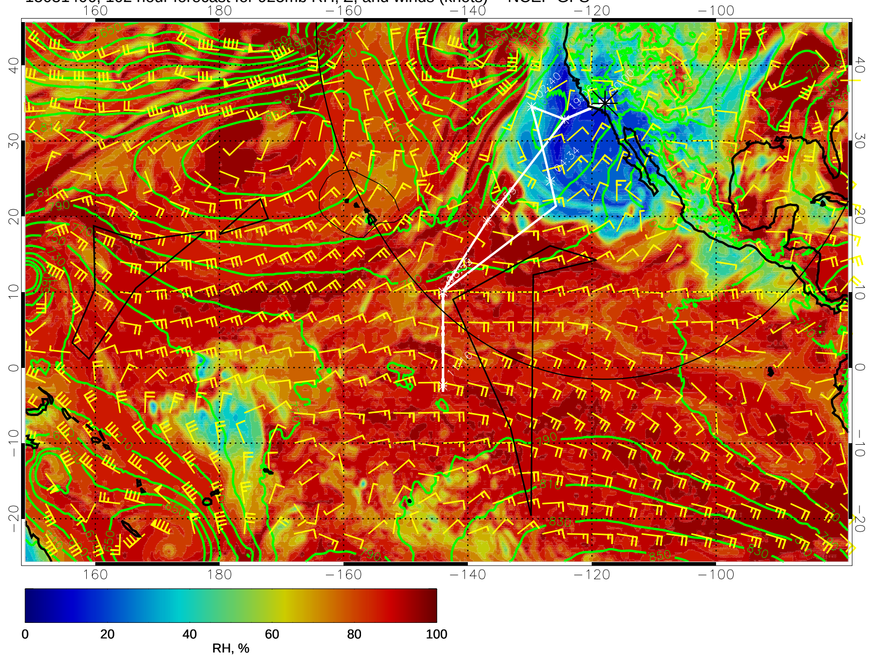
15031406, 102 hour forecast for 925mb RH, Z, and winds (knots) -- NCEP GFS
