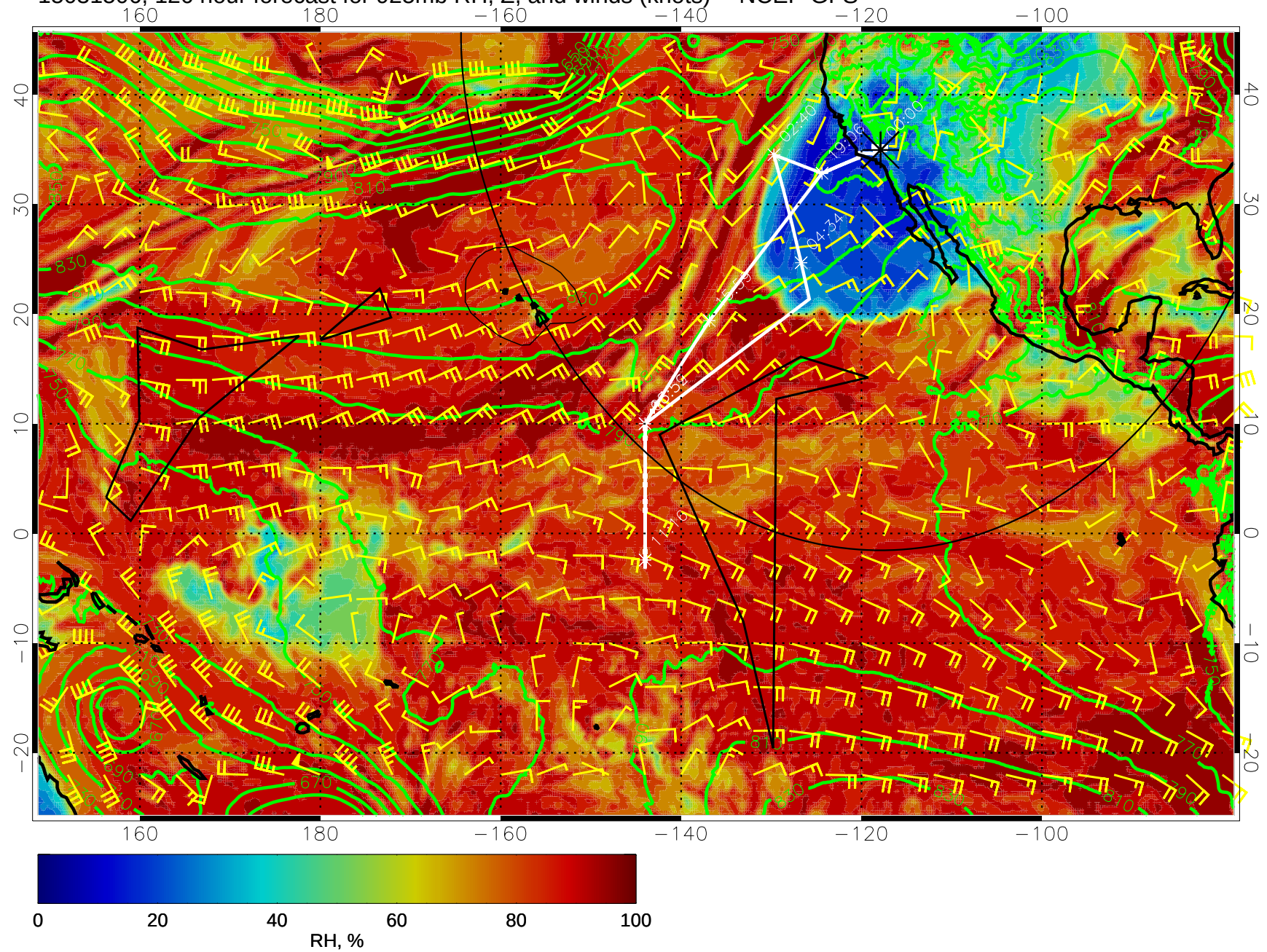
15031506, 126 hour forecast for 925mb RH, Z, and winds (knots) -- NCEP GFS
