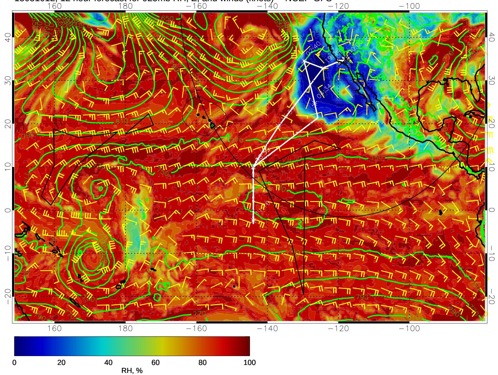
15031012, 12 hour forecast for 925mb RH, Z, and winds (knots) -- NCEP GFS
