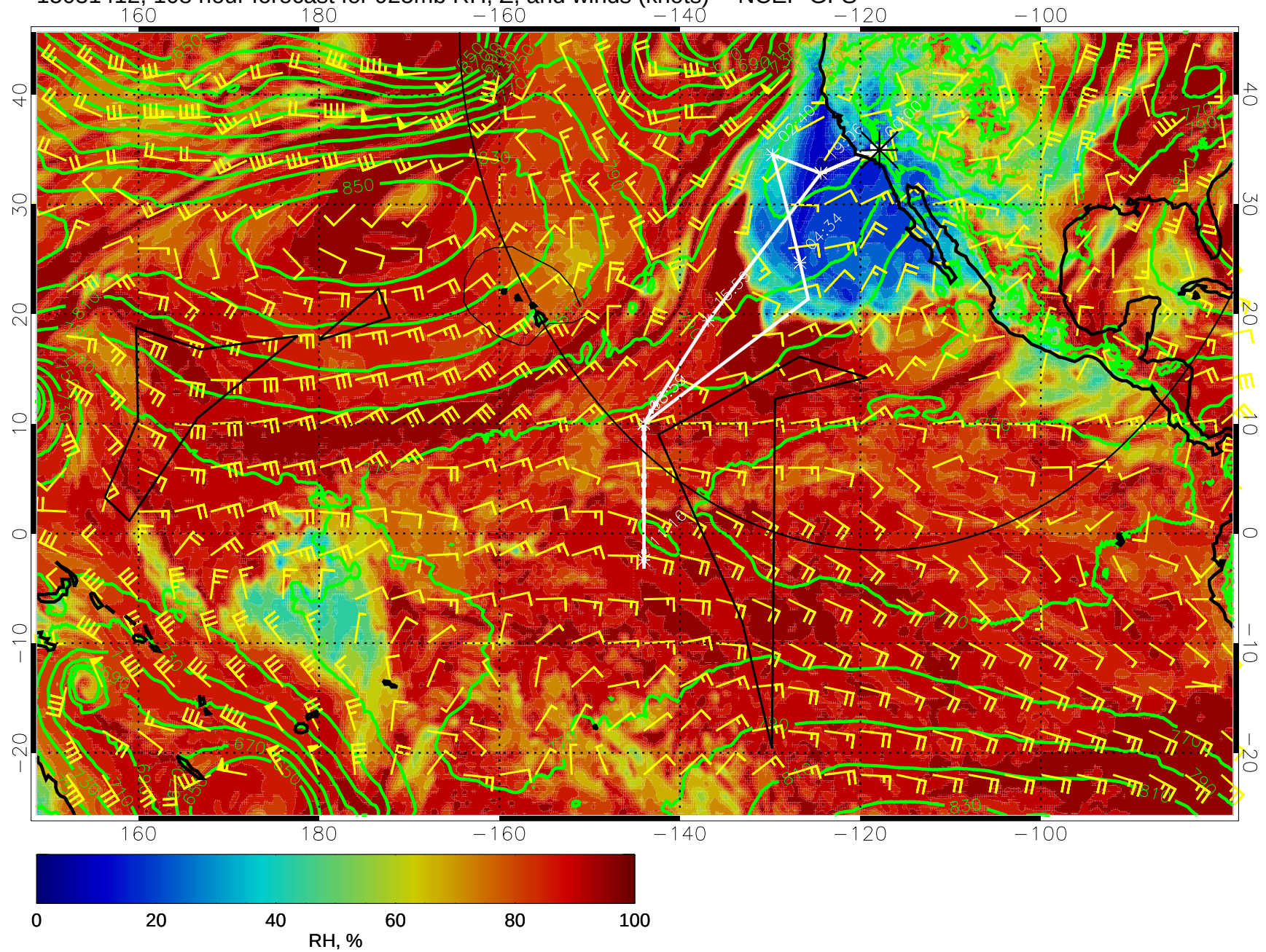
15031412, 108 hour forecast for 925mb RH, Z, and winds (knots) -- NCEP GFS
