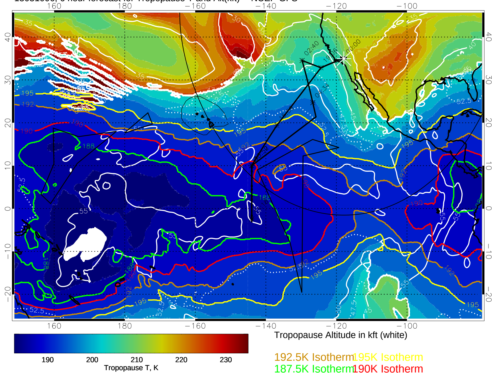
15031006, 6 hour forecast for Tropopause T and Alt(kft) -- NCEP GFS
