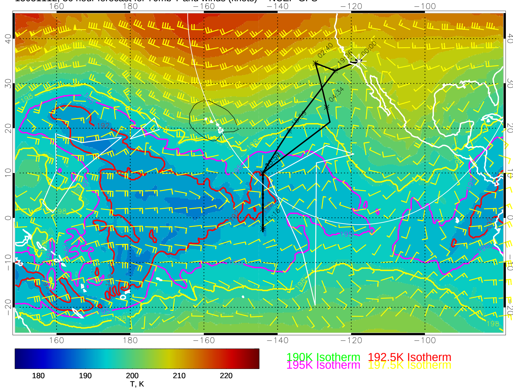
15031112, 36 hour forecast for 70mb T and winds (knots) -- NCEP GFS
