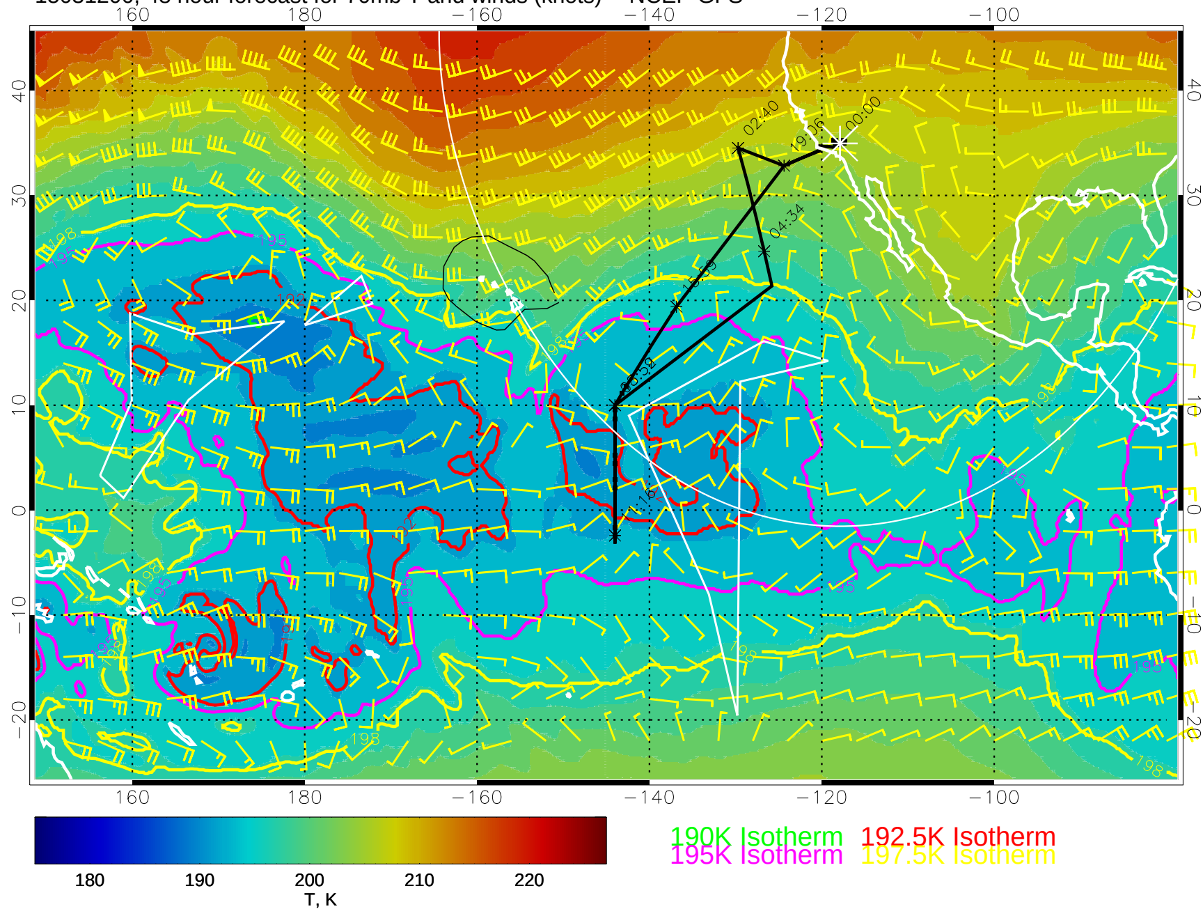
15031200, 48 hour forecast for 70mb T and winds (knots) -- NCEP GFS
