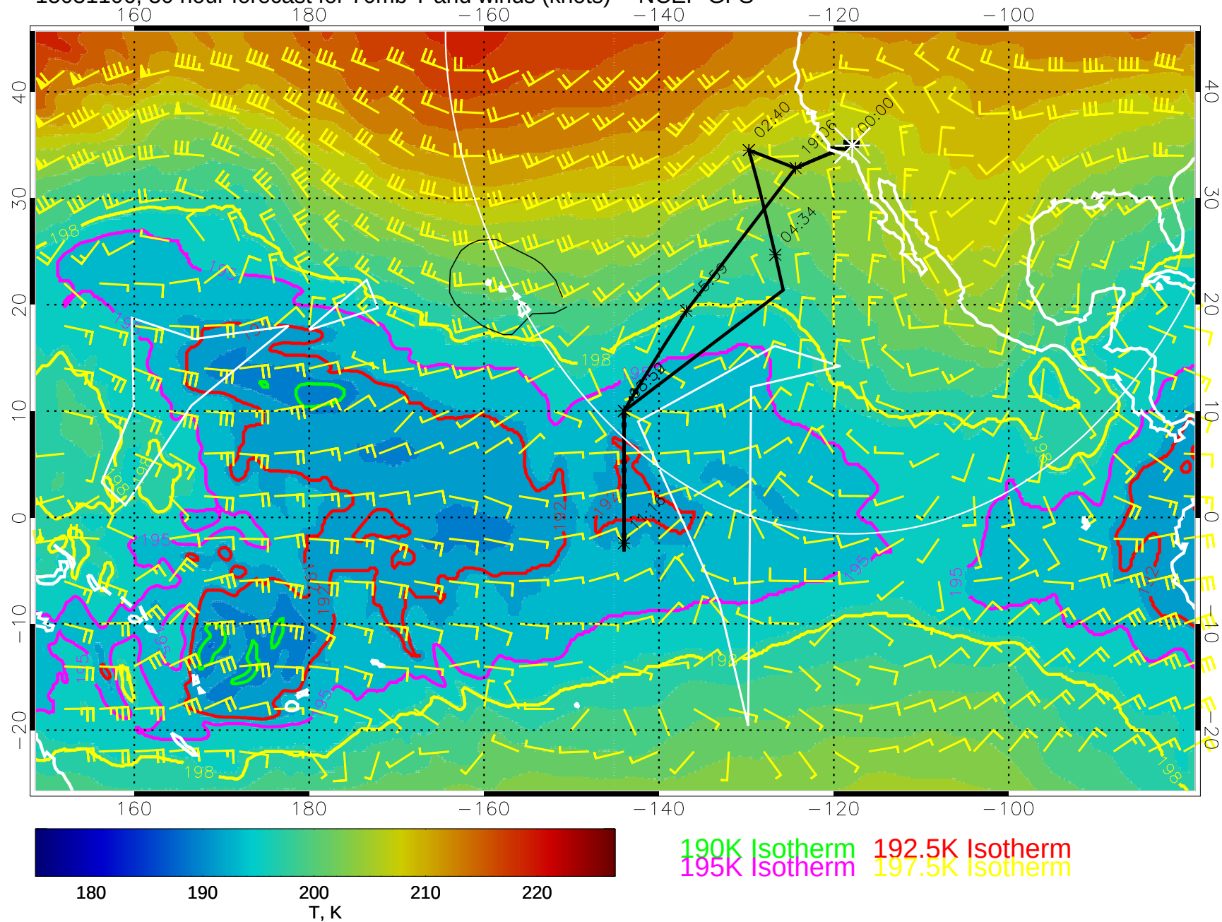
15031106, 30 hour forecast for 70mb T and winds (knots) -- NCEP GFS
