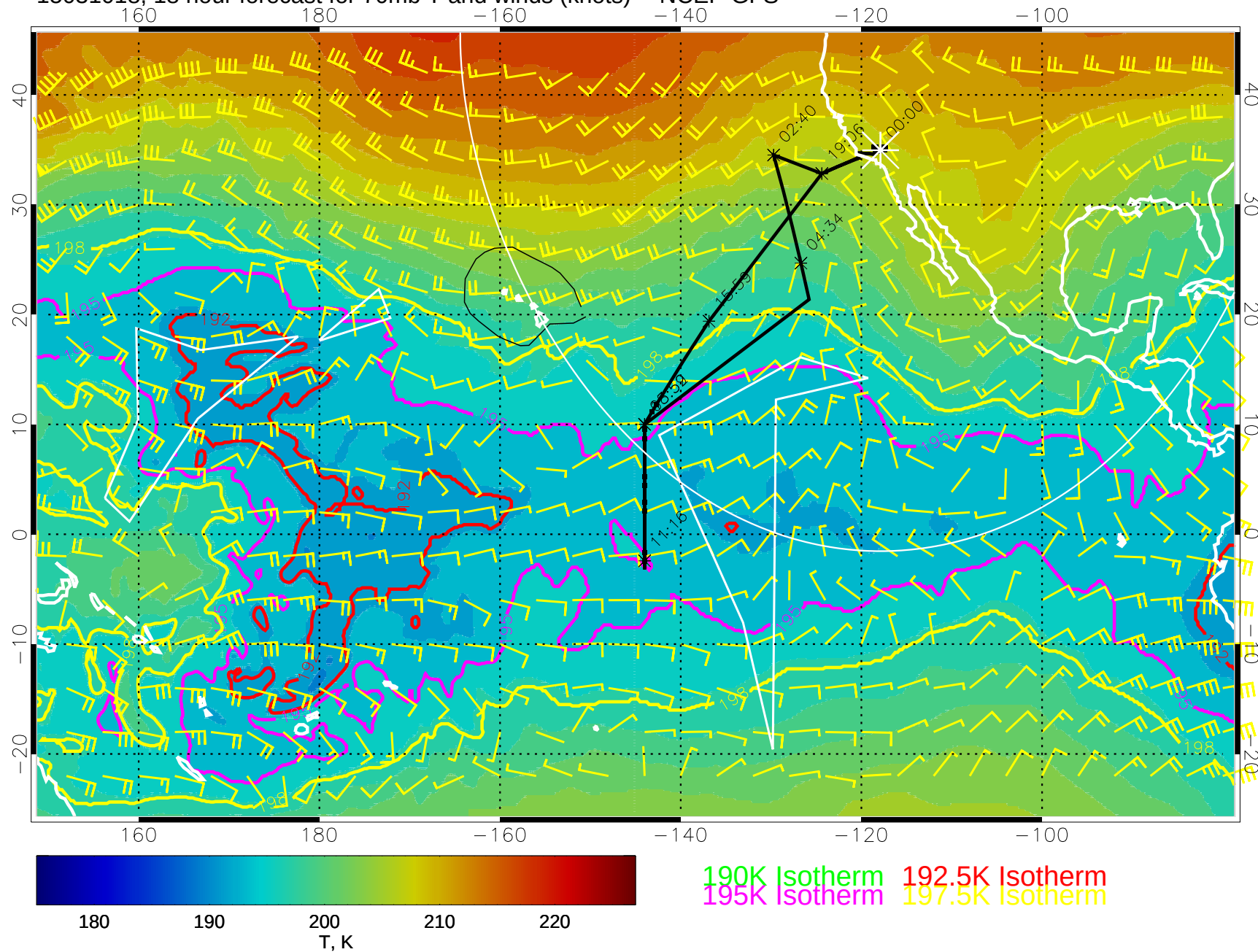
15031018, 18 hour forecast for 70mb T and winds (knots) -- NCEP GFS
