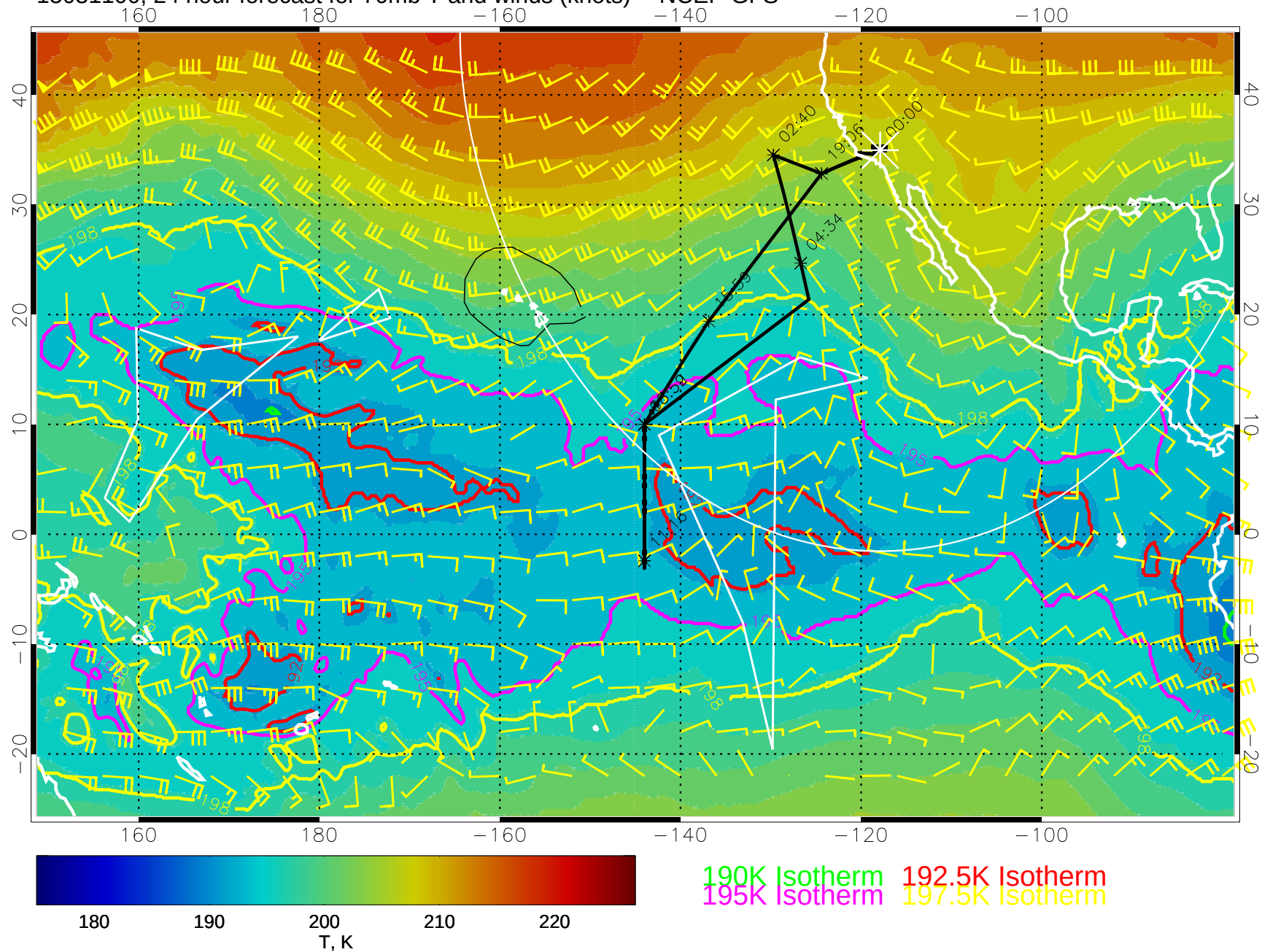
15031100, 24 hour forecast for 70mb T and winds (knots) -- NCEP GFS
