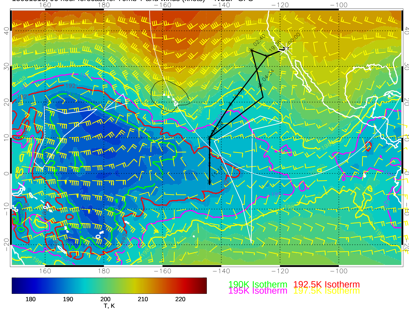
15031318, 90 hour forecast for 70mb T and winds (knots) -- NCEP GFS
