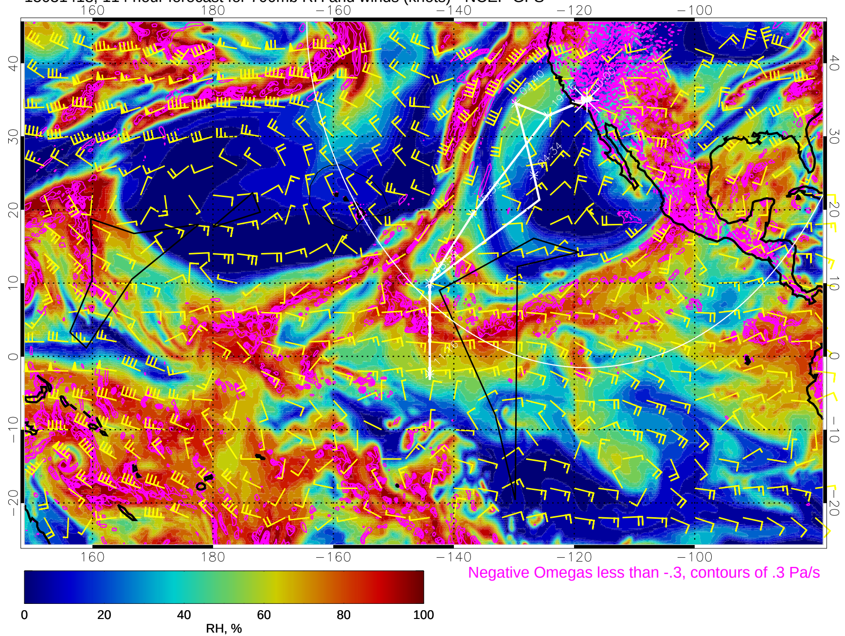
15031418, 114 hour forecast for 700mb RH and winds (knots) - NCEP GFS
