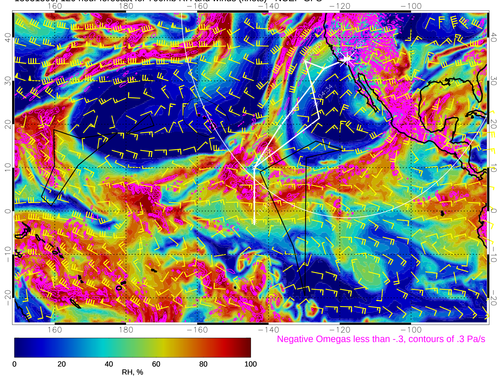
15031500, 120 hour forecast for 700mb RH and winds (knots) - NCEP GFS
