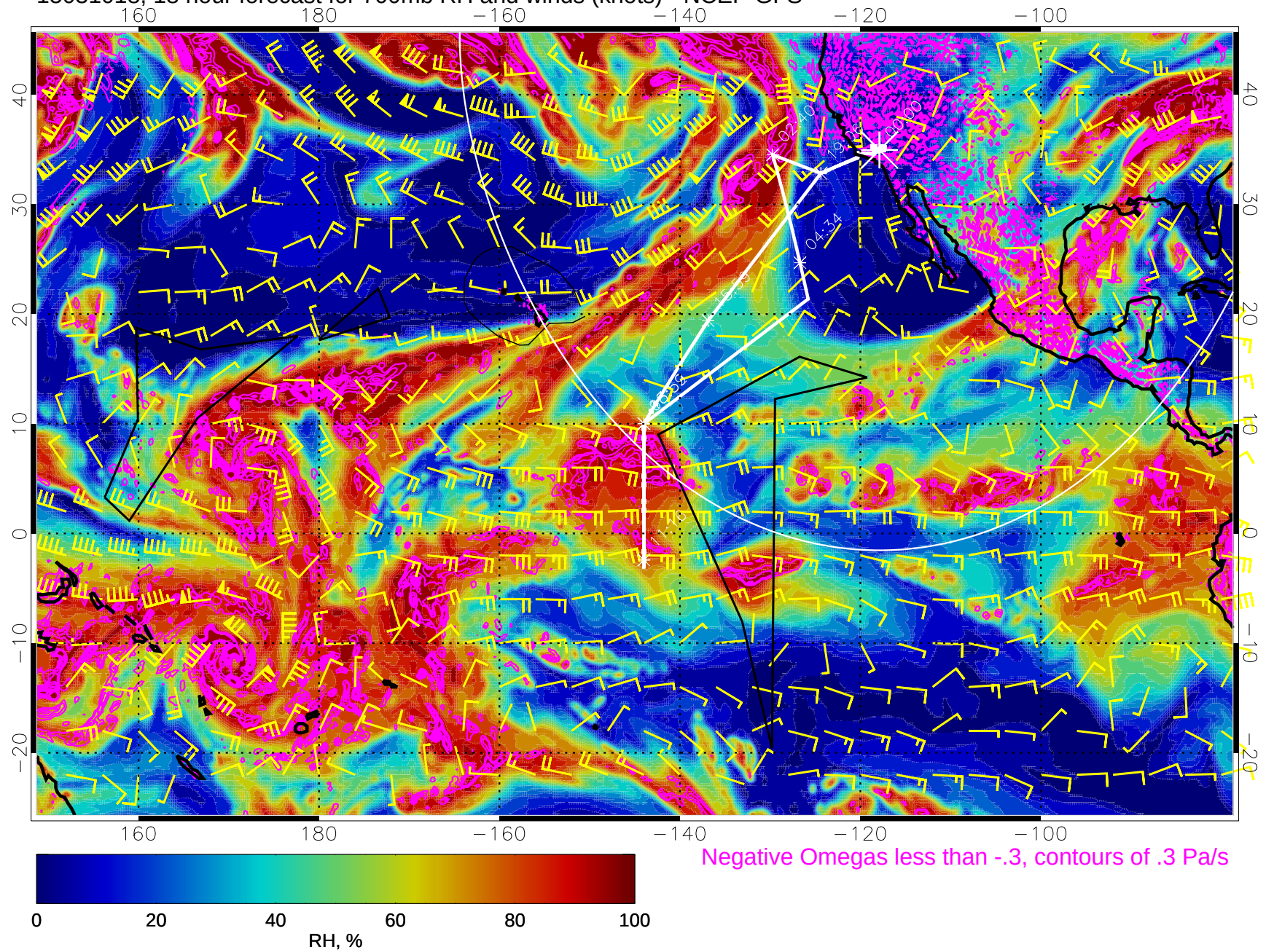
15031018, 18 hour forecast for 700mb RH and winds (knots) - NCEP GFS
