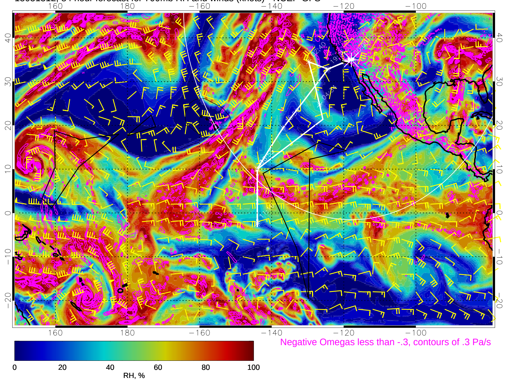
15031312, 84 hour forecast for 700mb RH and winds (knots) - NCEP GFS
