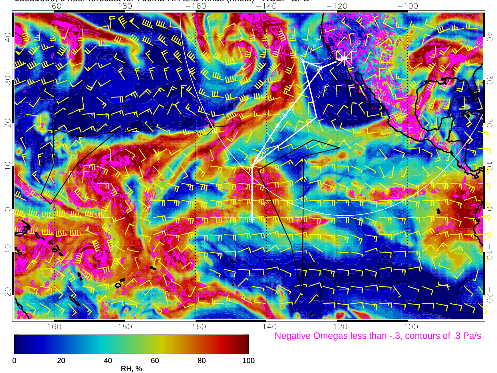
15031006, 6 hour forecast for 700mb RH and winds (knots) - NCEP GFS
