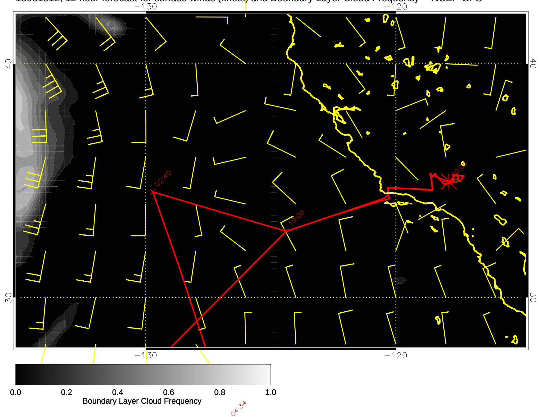
15031012, 12 hour forecast for surface winds (knots) and Boundary Layer Cloud Frequency -- NCEP GFS
