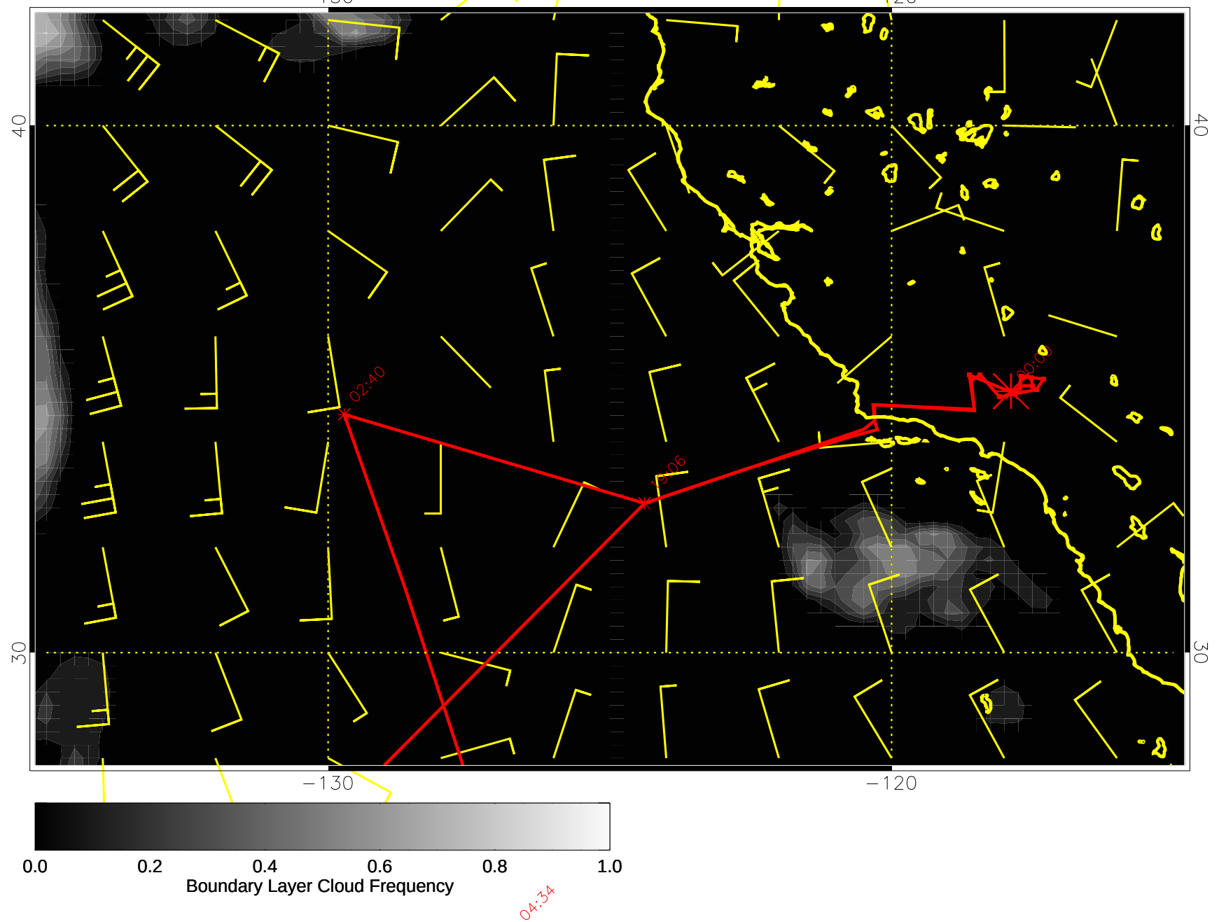
15031006, 6 hour forecast for surface winds (knots) and Boundary Layer Cloud Frequency -- NCEP GFS
