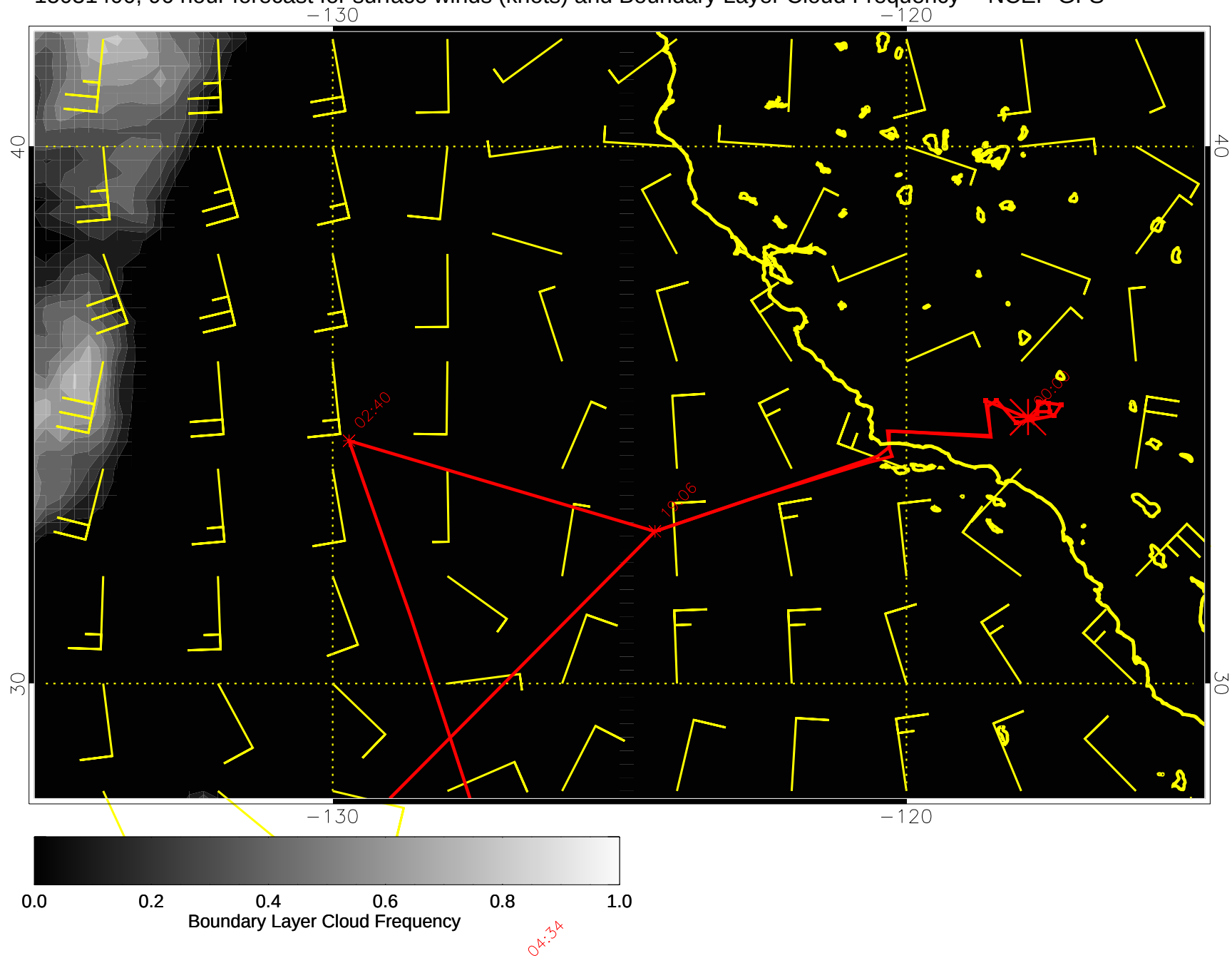
15031400, 96 hour forecast for surface winds (knots) and Boundary Layer Cloud Frequency -- NCEP GFS
