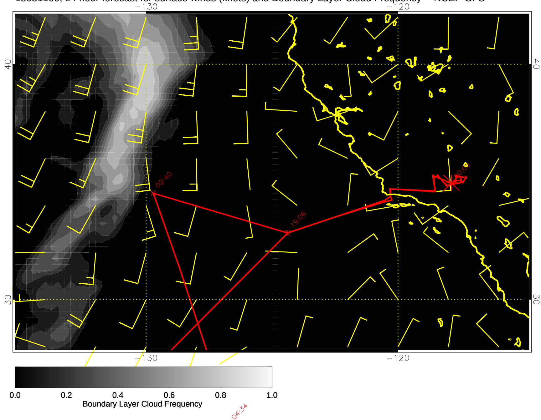
15031100, 24 hour forecast for surface winds (knots) and Boundary Layer Cloud Frequency -- NCEP GFS
