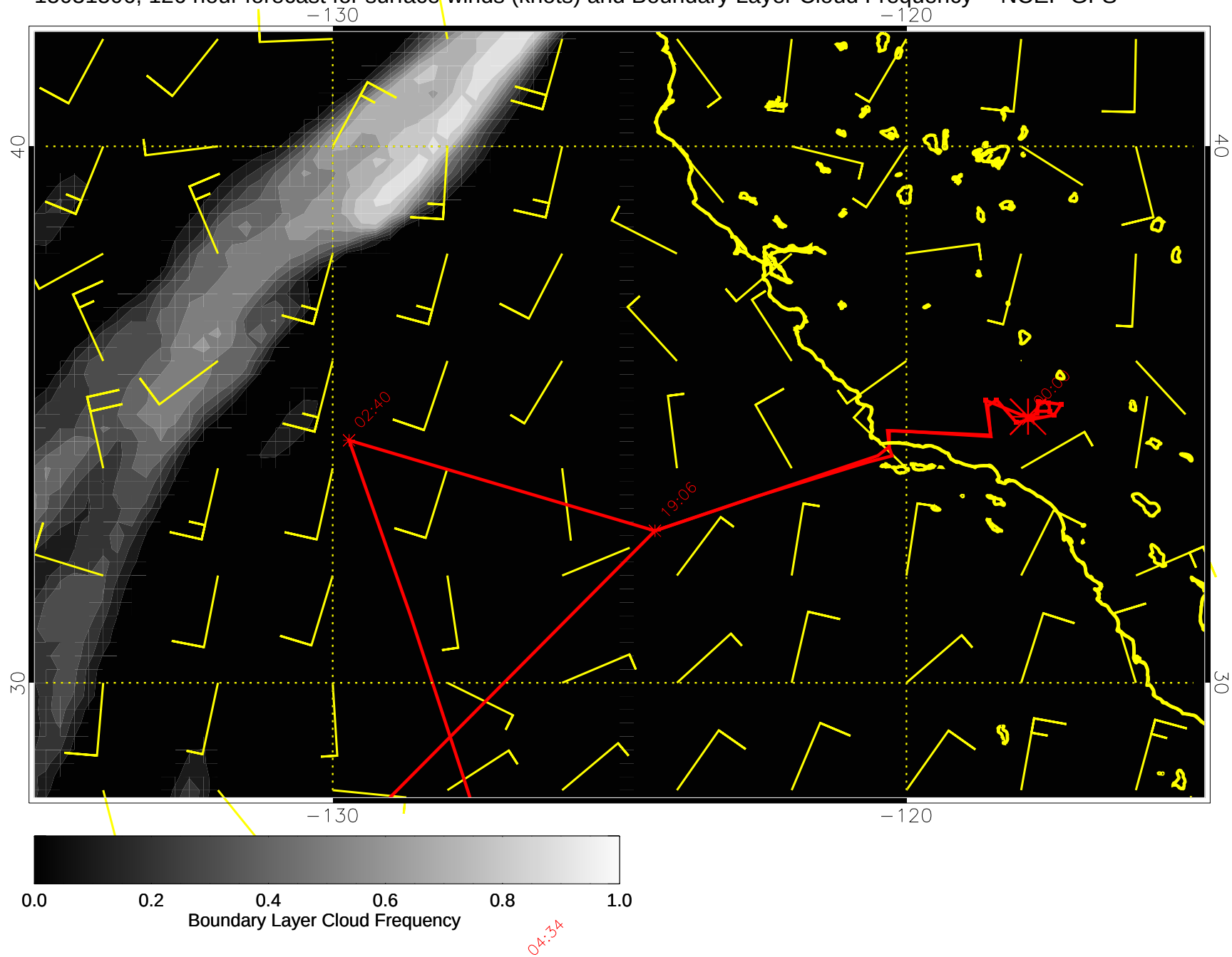
15031506, 126 hour forecast for surface winds (knots) and Boundary Layer Cloud Frequency -- NCEP GFS
