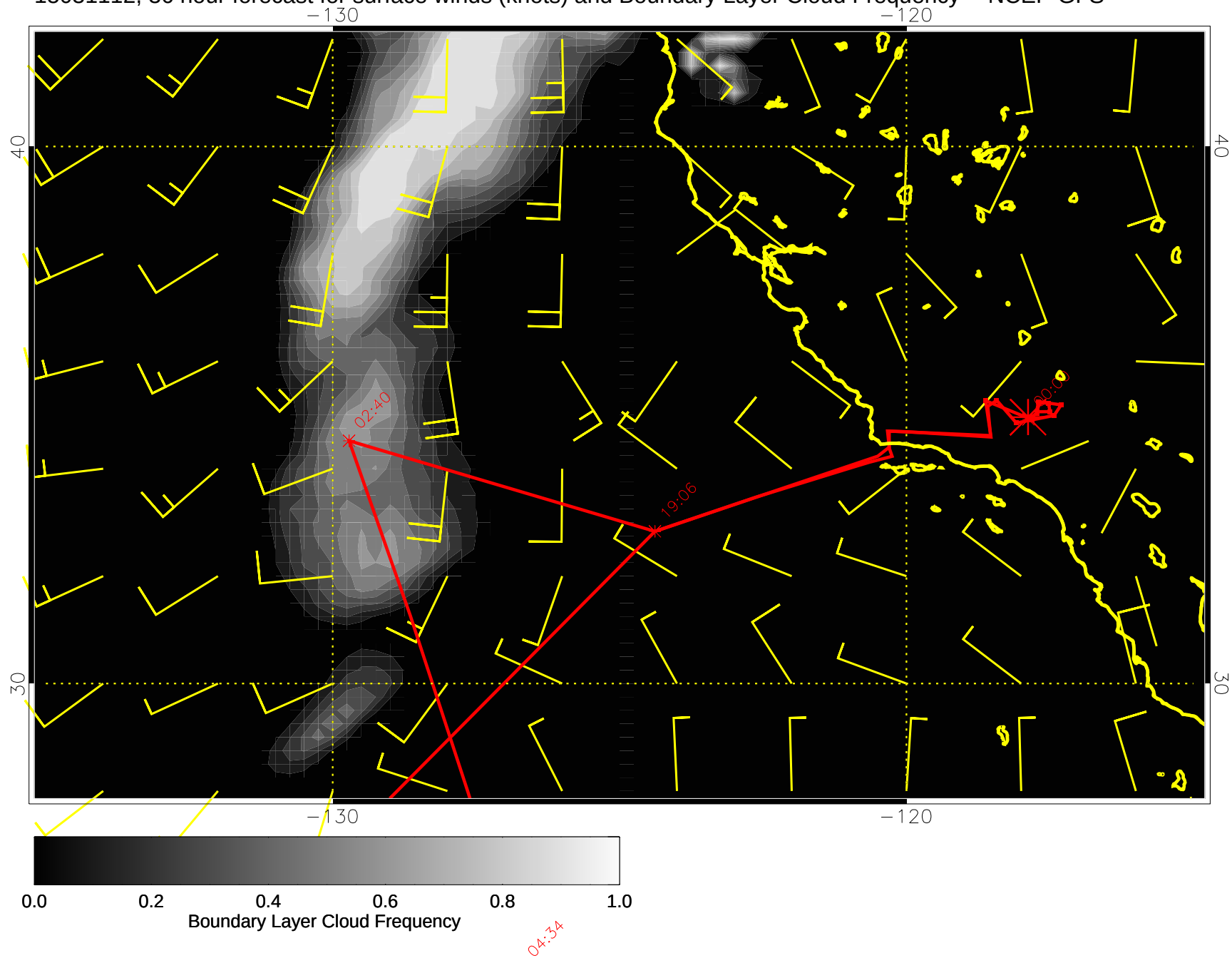
15031112, 36 hour forecast for surface winds (knots) and Boundary Layer Cloud Frequency -- NCEP GFS
