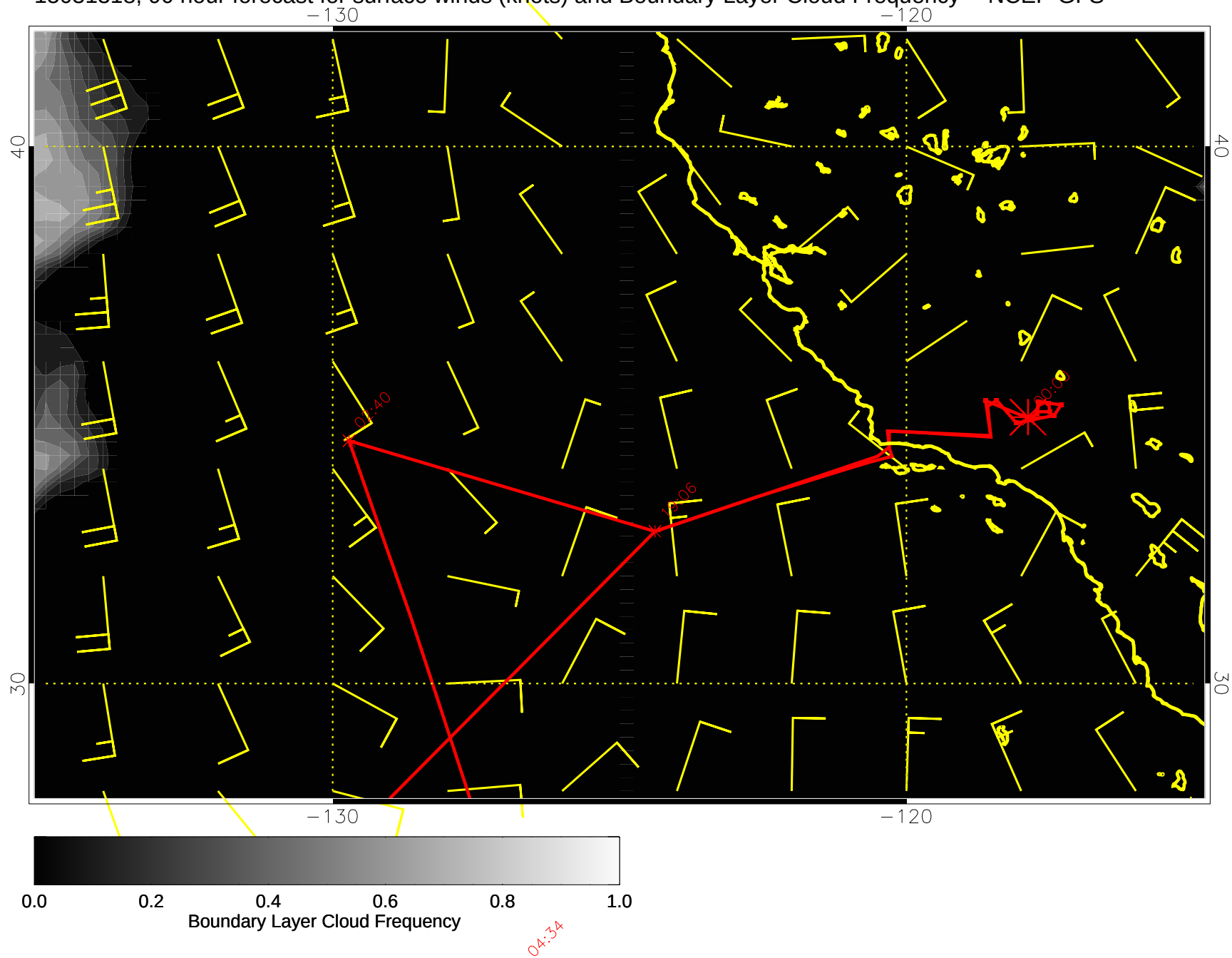
15031318, 90 hour forecast for surface winds (knots) and Boundary Layer Cloud Frequency -- NCEP GFS
