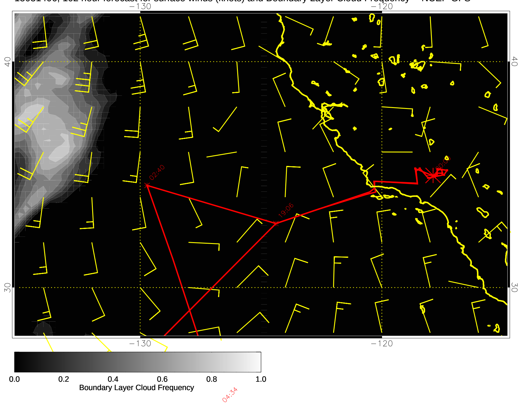
15031406, 102 hour forecast for surface winds (knots) and Boundary Layer Cloud Frequency -- NCEP GFS
