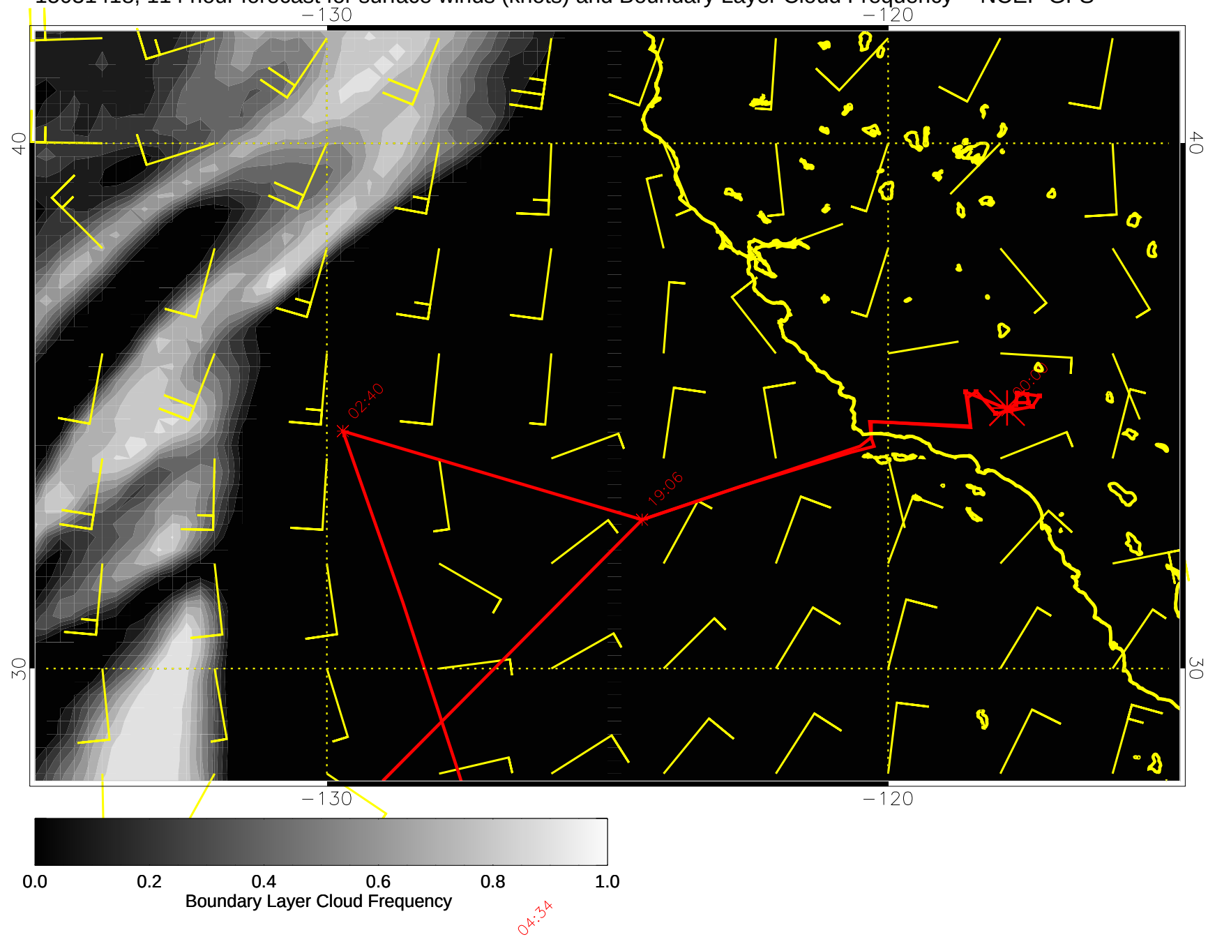
15031418, 114 hour forecast for surface winds (knots) and Boundary Layer Cloud Frequency -- NCEP GFS
