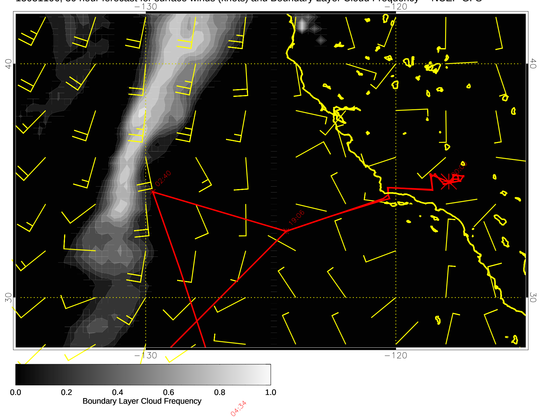
15031106, 30 hour forecast for surface winds (knots) and Boundary Layer Cloud Frequency -- NCEP GFS
