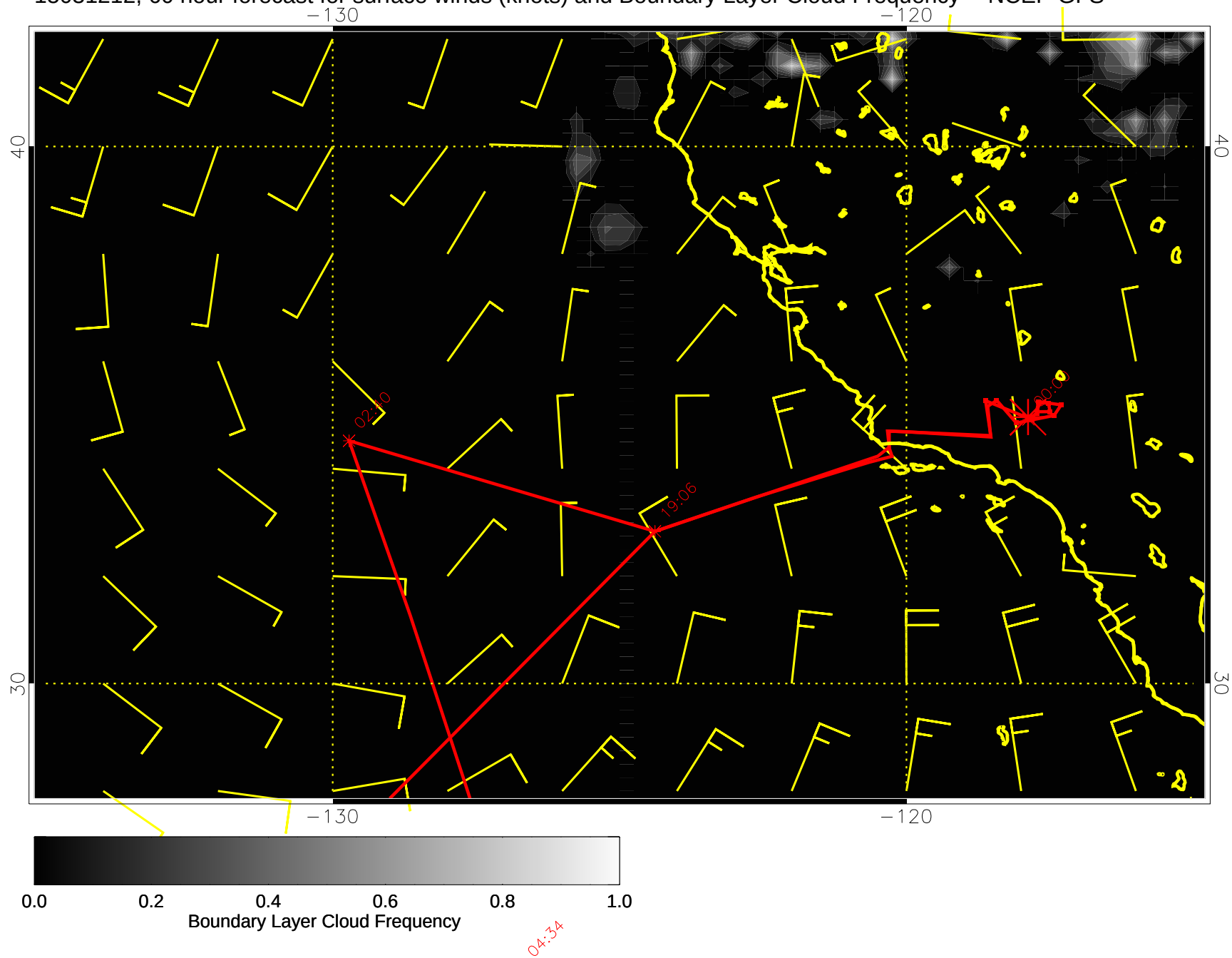
15031212, 60 hour forecast for surface winds (knots) and Boundary Layer Cloud Frequency -- NCEP GFS
