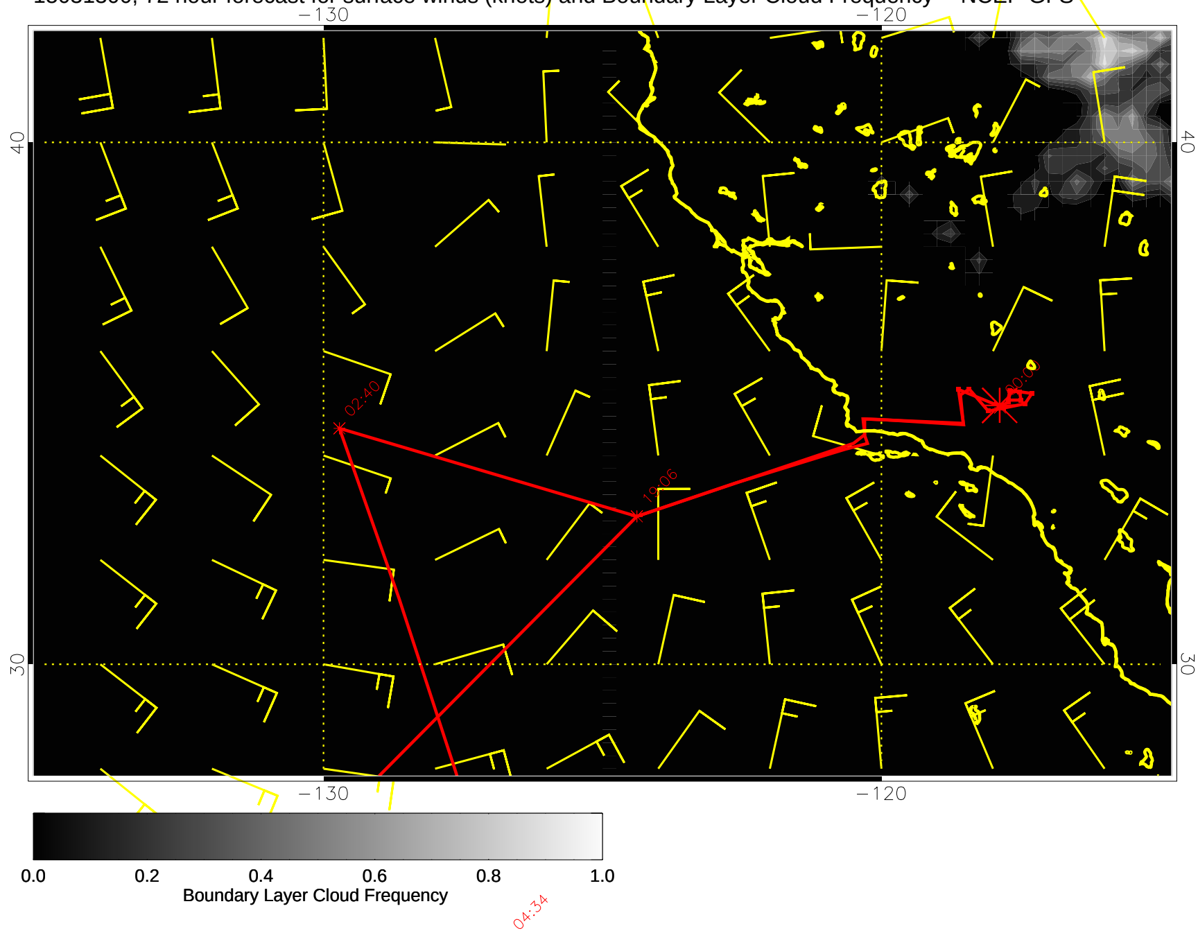
15031300, 72 hour forecast for surface winds (knots) and Boundary Layer Cloud Frequency -- NCEP GFS
