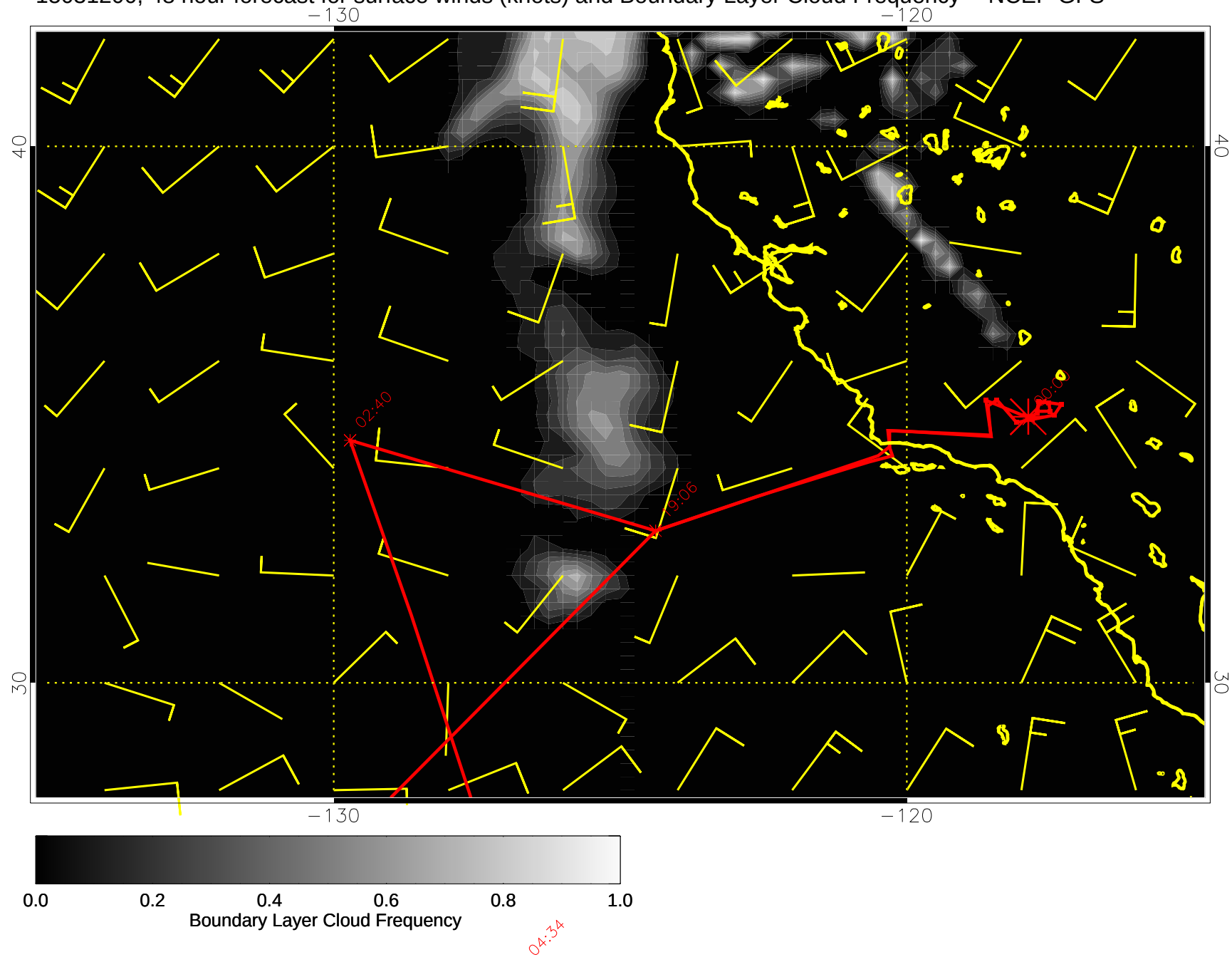
15031200, 48 hour forecast for surface winds (knots) and Boundary Layer Cloud Frequency -- NCEP GFS
