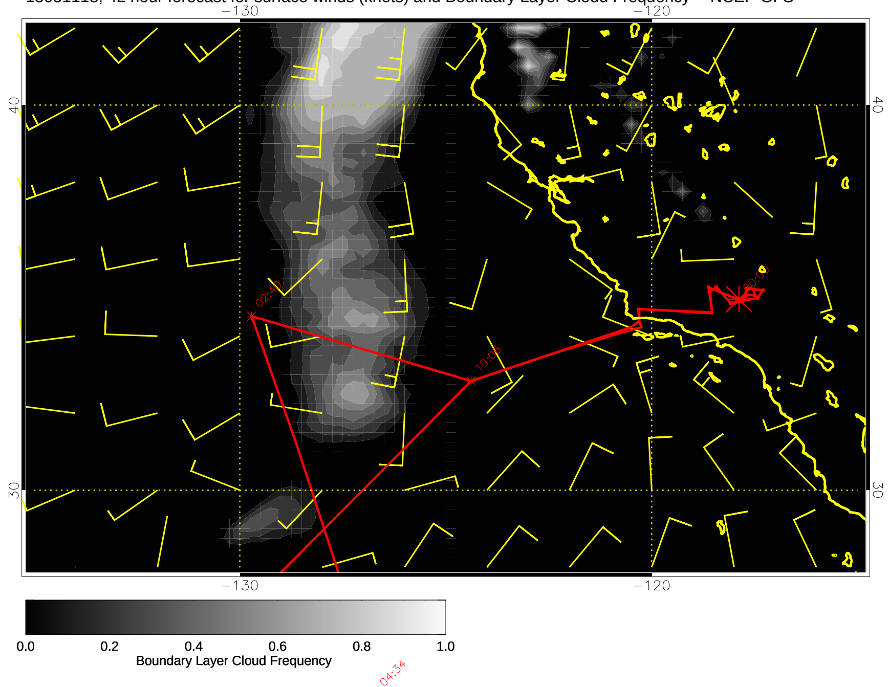
15031118, 42 hour forecast for surface winds (knots) and Boundary Layer Cloud Frequency -- NCEP GFS
