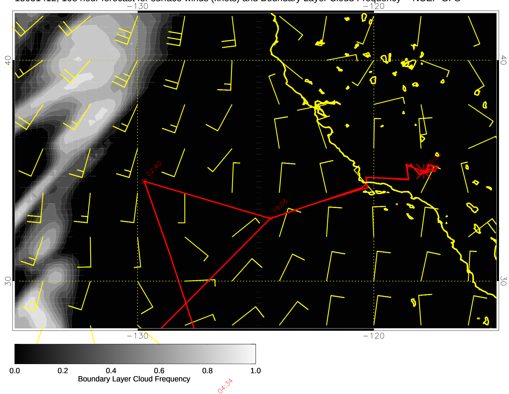
15031412, 108 hour forecast for surface winds (knots) and Boundary Layer Cloud Frequency -- NCEP GFS
