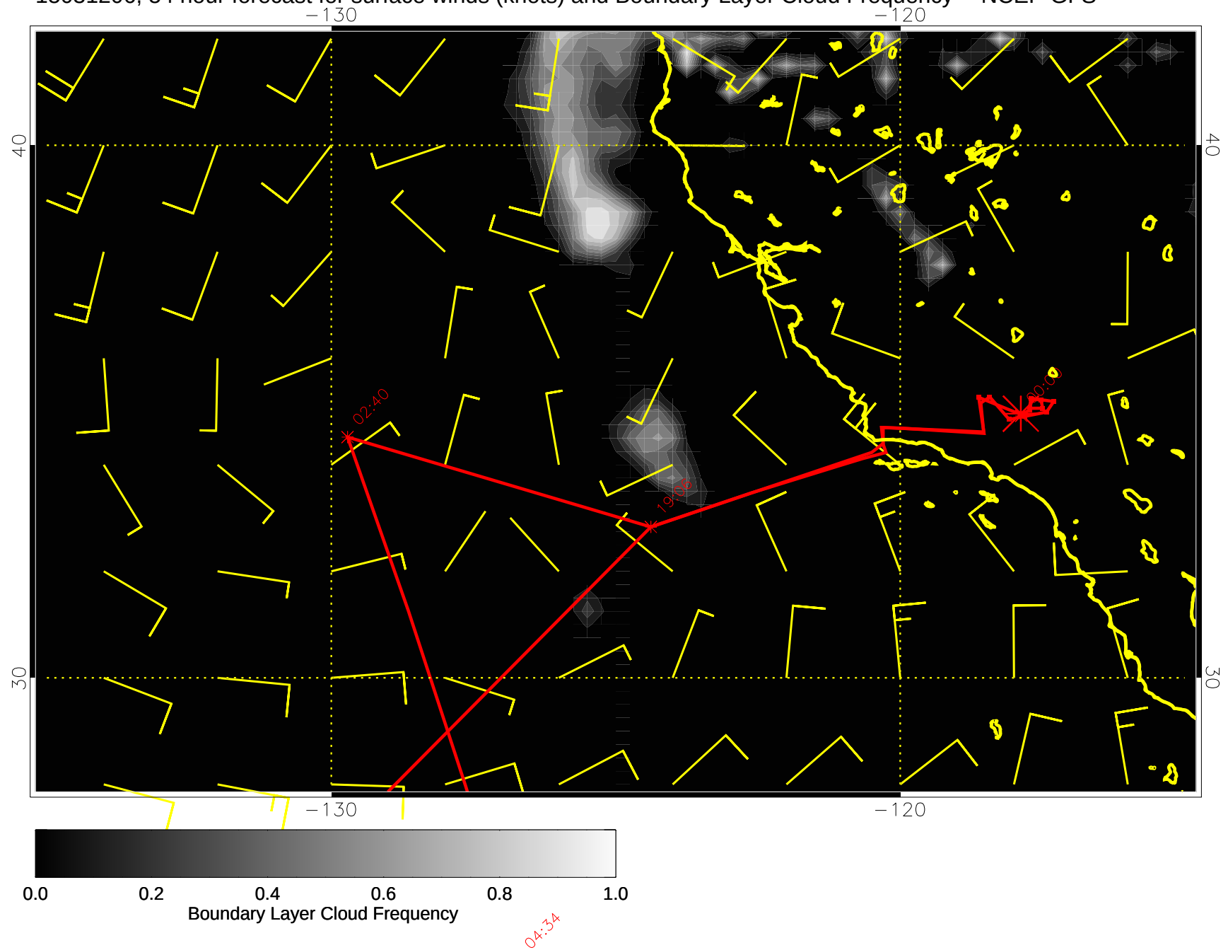
15031206, 54 hour forecast for surface winds (knots) and Boundary Layer Cloud Frequency -- NCEP GFS
