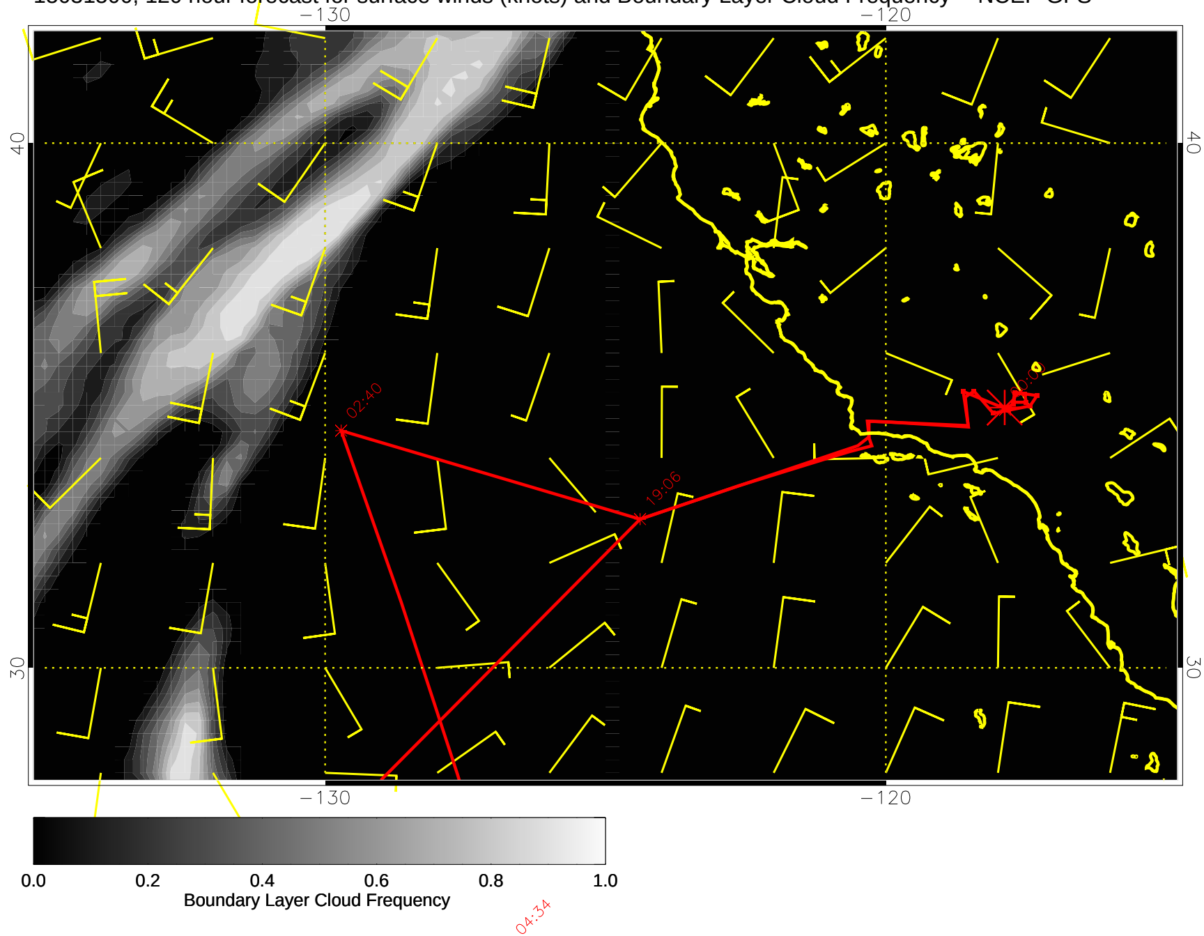
15031500, 120 hour forecast for surface winds (knots) and Boundary Layer Cloud Frequency -- NCEP GFS
