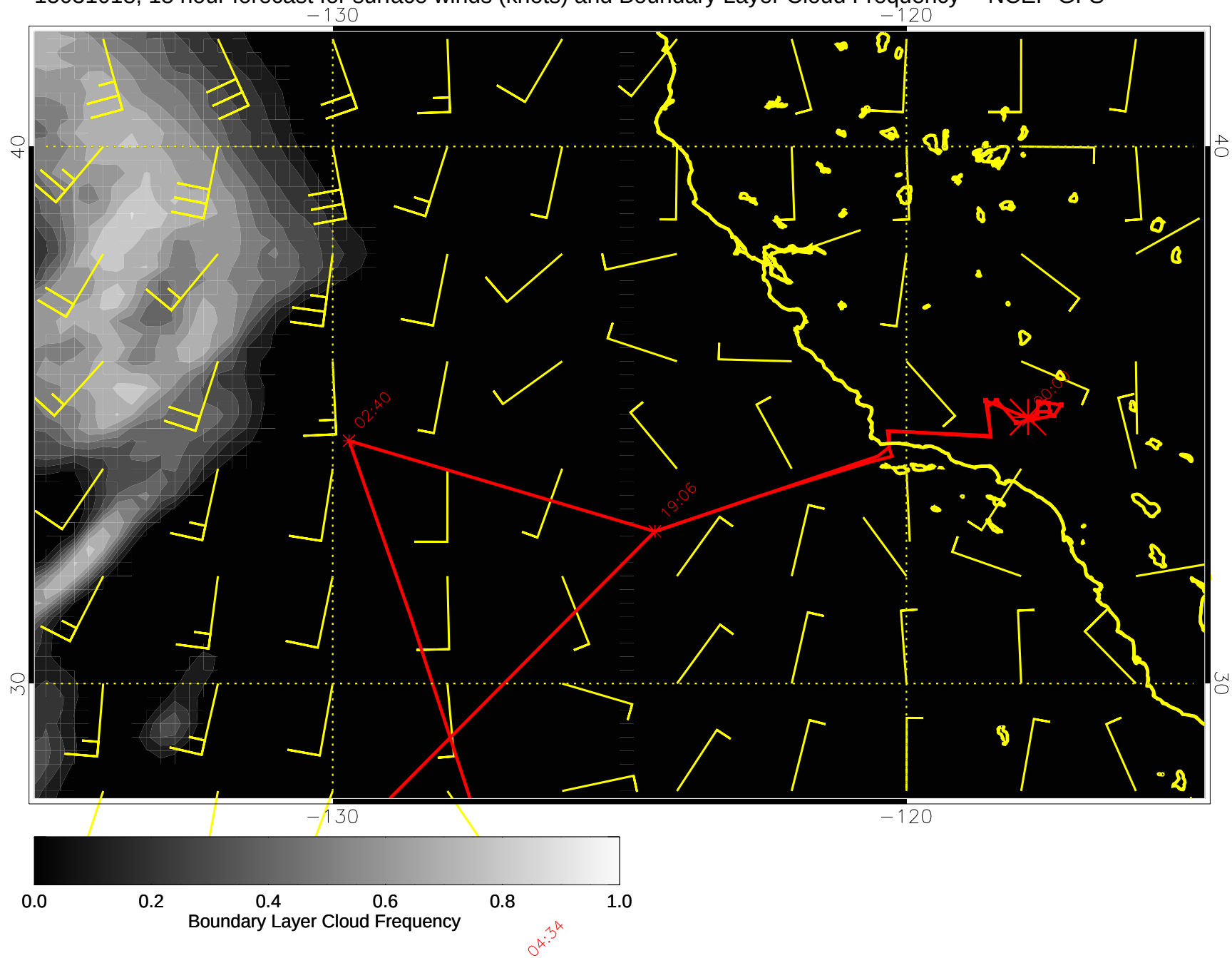
15031018, 18 hour forecast for surface winds (knots) and Boundary Layer Cloud Frequency -- NCEP GFS
