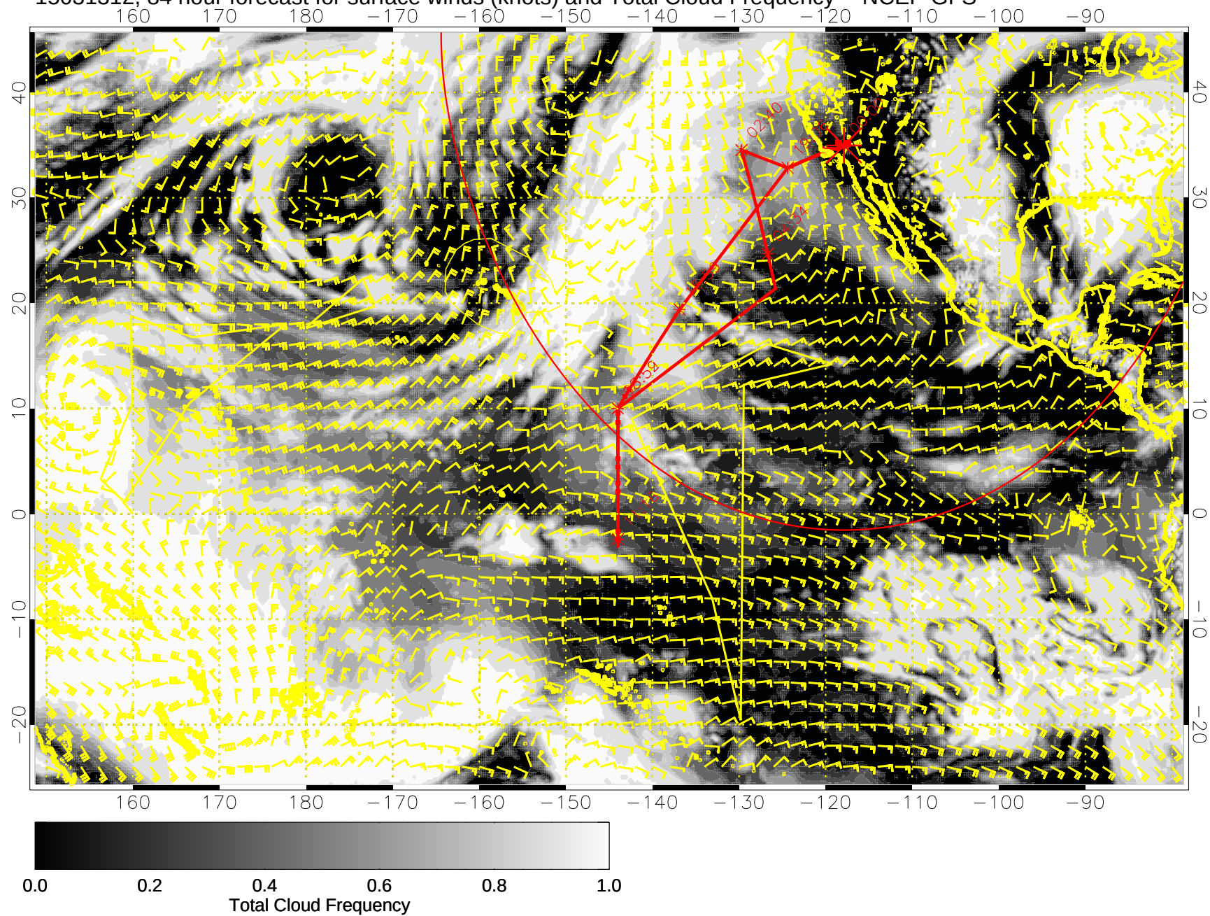
15031312, 84 hour forecast for surface winds (knots) and Total Cloud Frequency -- NCEP GFS
