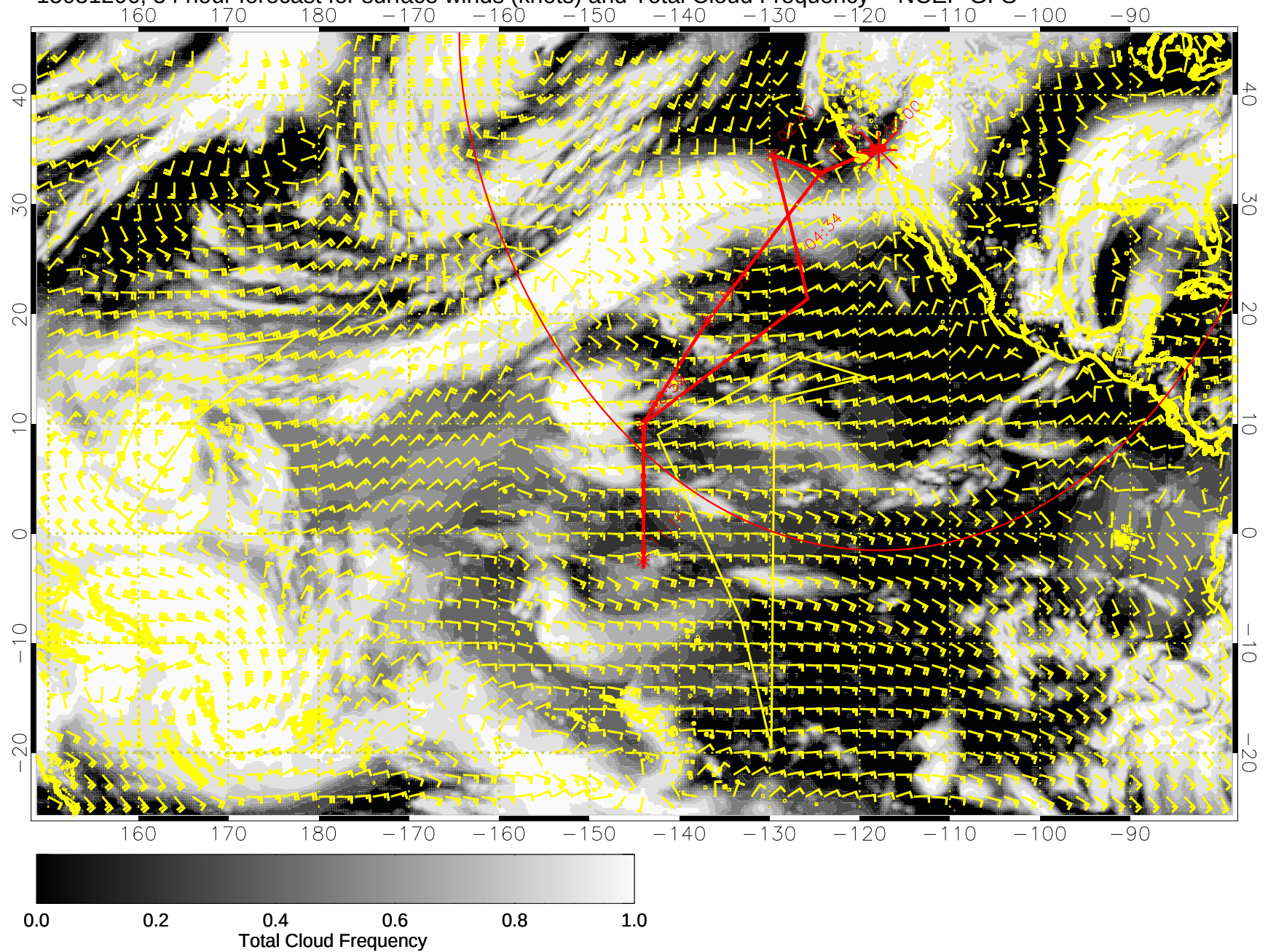
15031206, 54 hour forecast for surface winds (knots) and Total Cloud Frequency -- NCEP GFS
