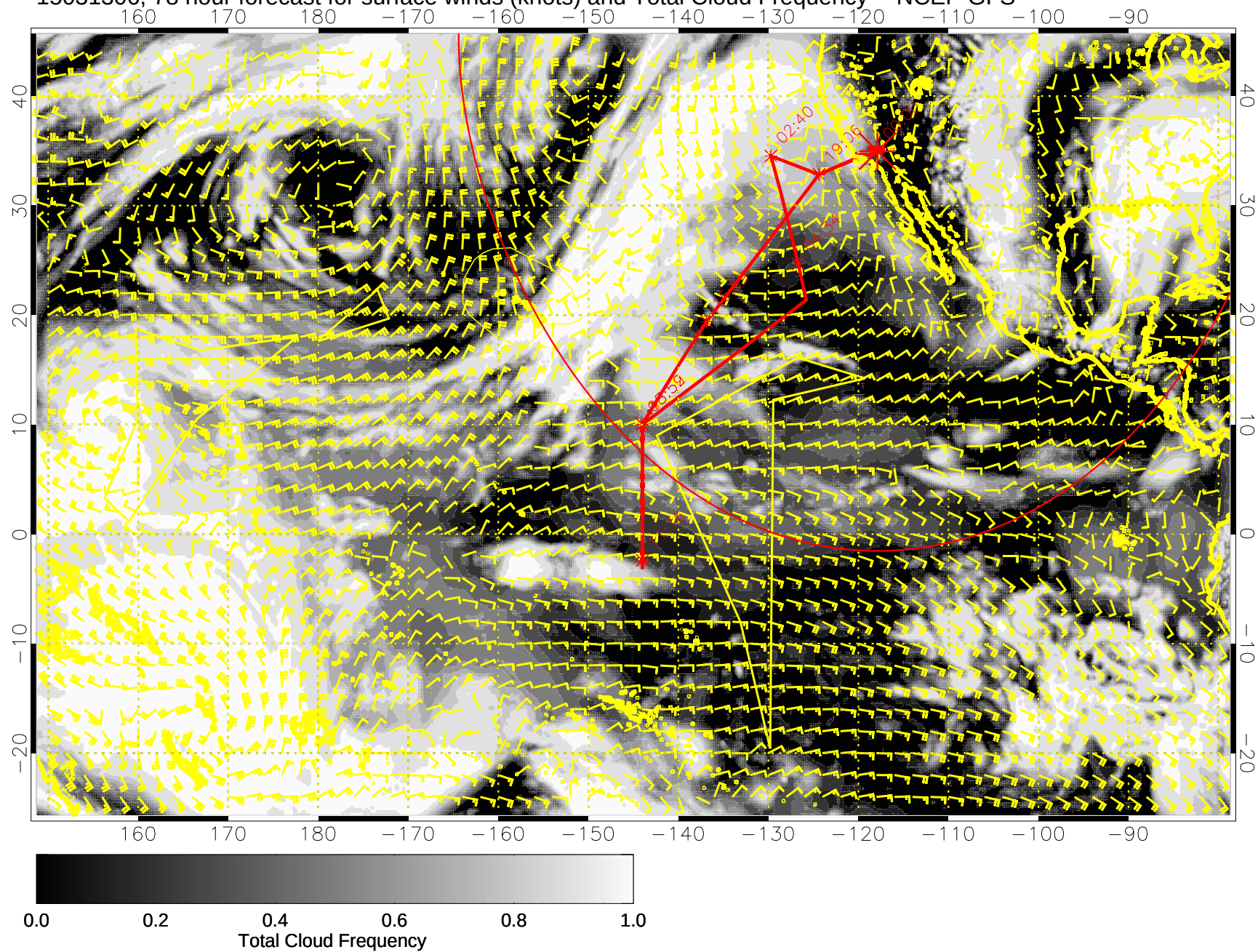
15031306, 78 hour forecast for surface winds (knots) and Total Cloud Frequency -- NCEP GFS
