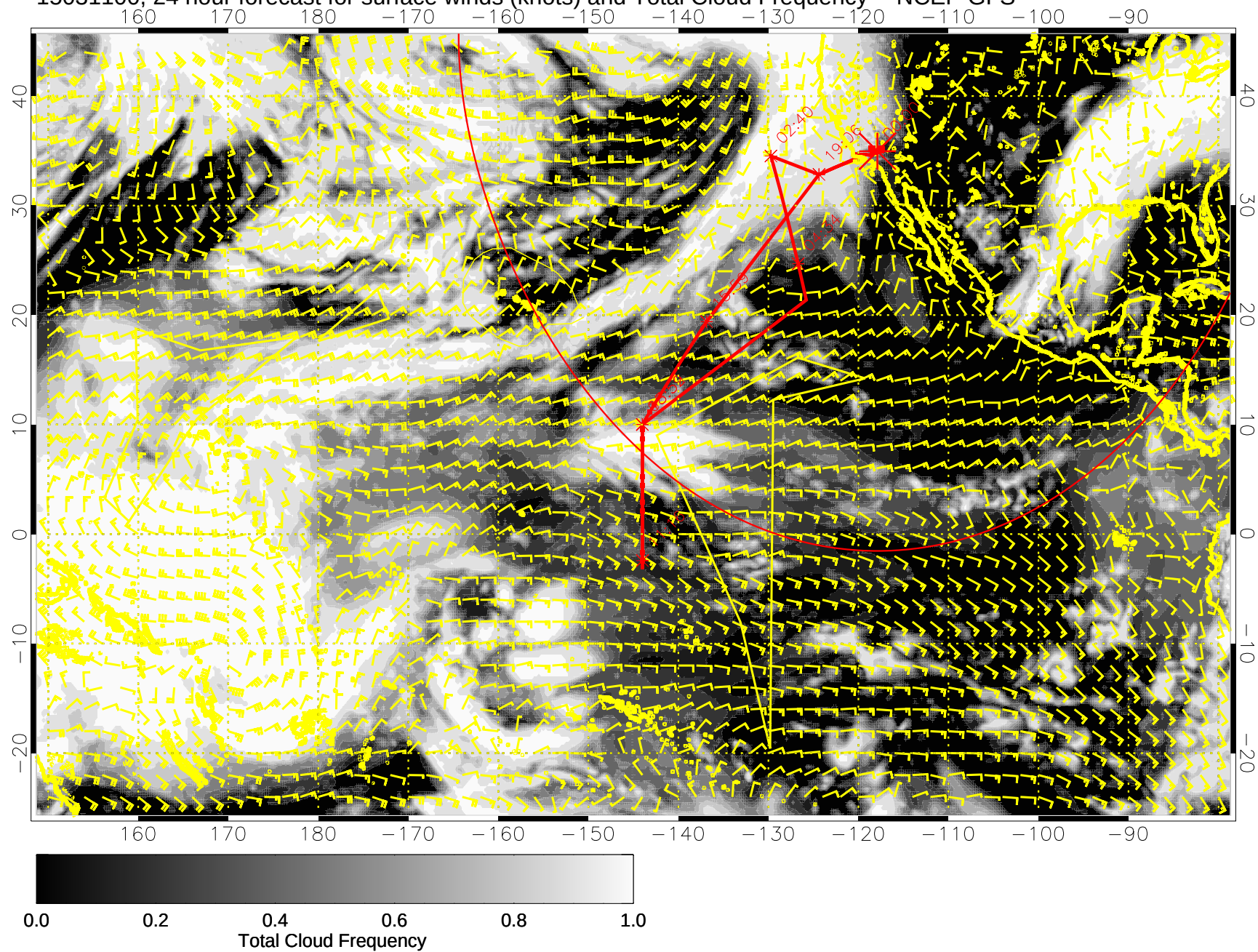
15031100, 24 hour forecast for surface winds (knots) and Total Cloud Frequency -- NCEP GFS
