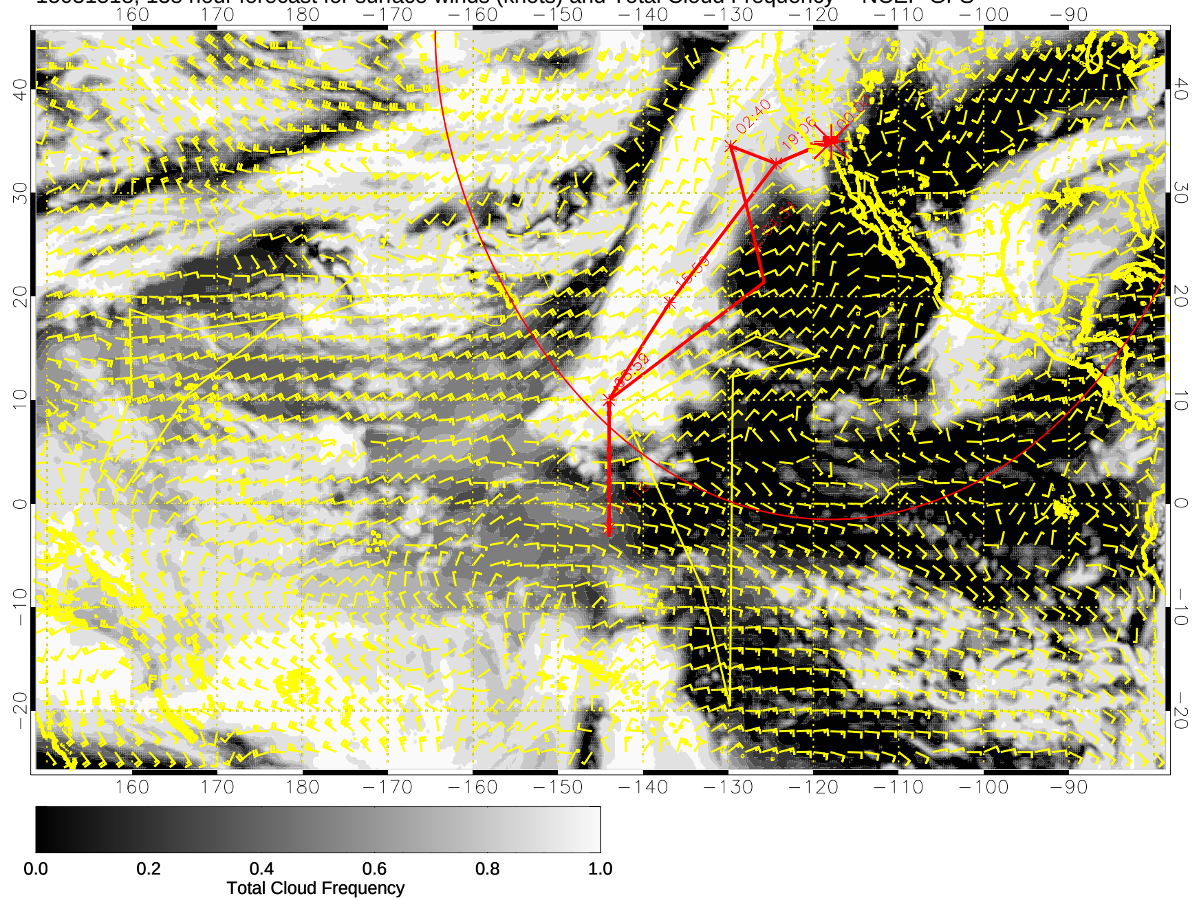
15031518, 138 hour forecast for surface winds (knots) and Total Cloud Frequency -- NCEP GFS
