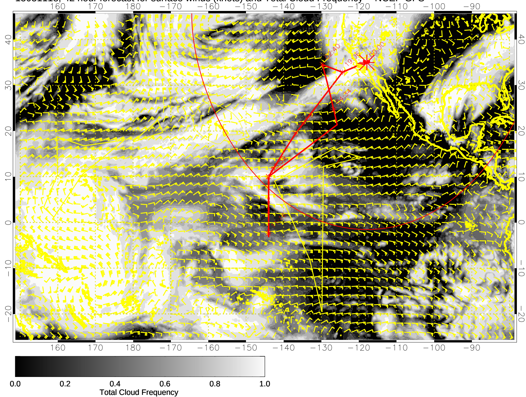
15031118, 42 hour forecast for surface winds (knots) and Total Cloud Frequency -- NCEP GFS
