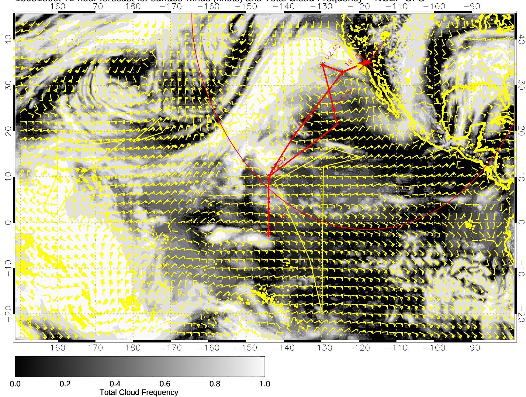
15031300, 72 hour forecast for surface winds (knots) and Total Cloud Frequency -- NCEP GFS
