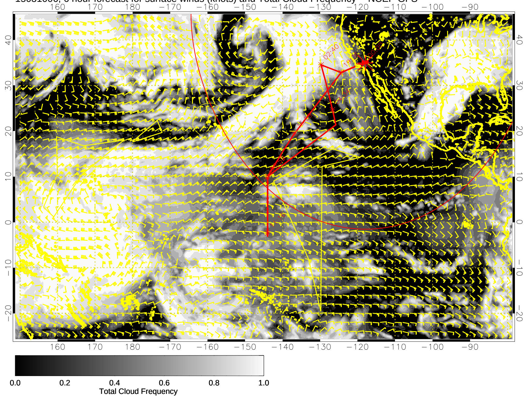
15031006, 6 hour forecast for surface winds (knots) and Total Cloud Frequency -- NCEP GFS
