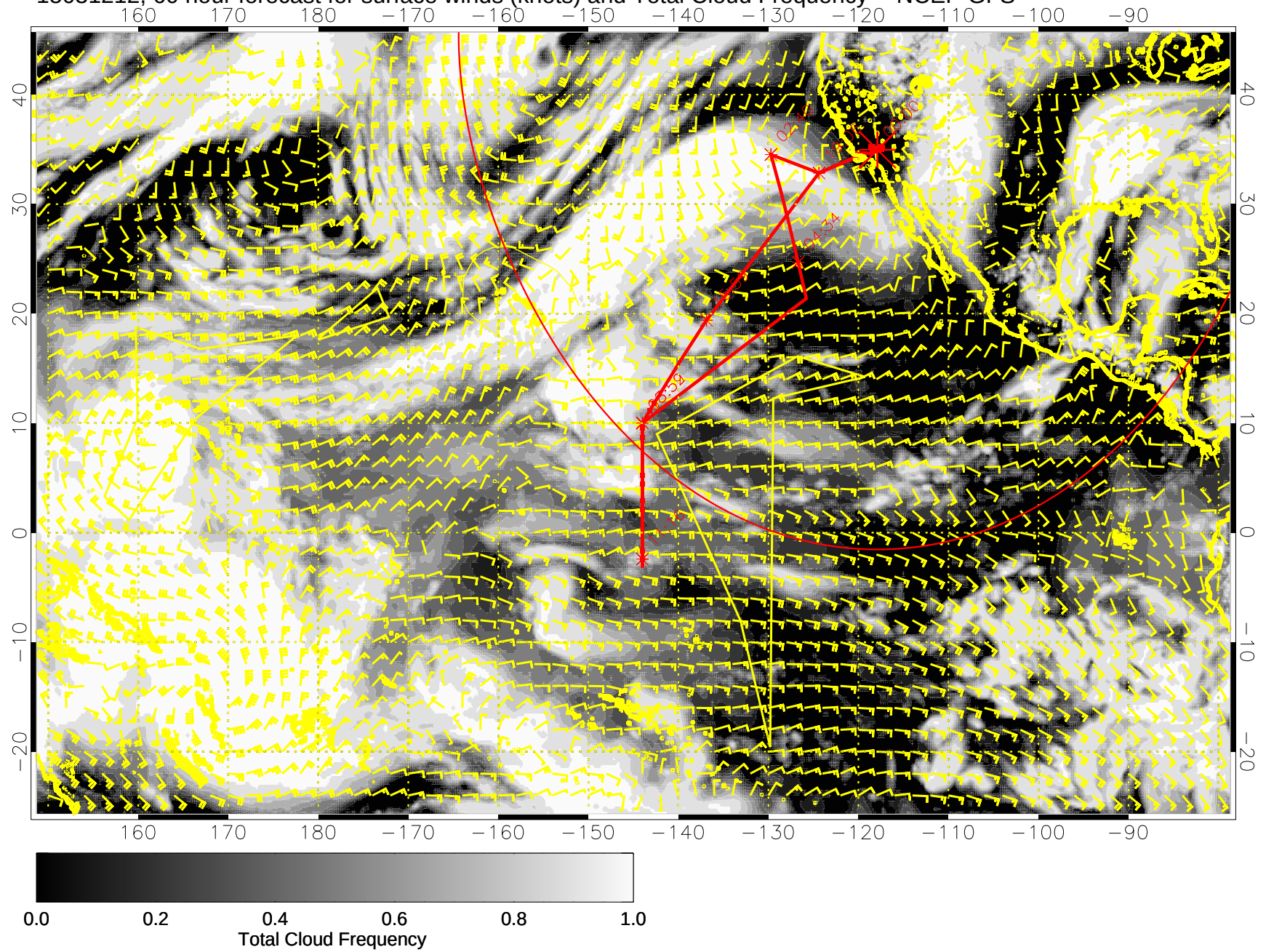
15031212, 60 hour forecast for surface winds (knots) and Total Cloud Frequency -- NCEP GFS
