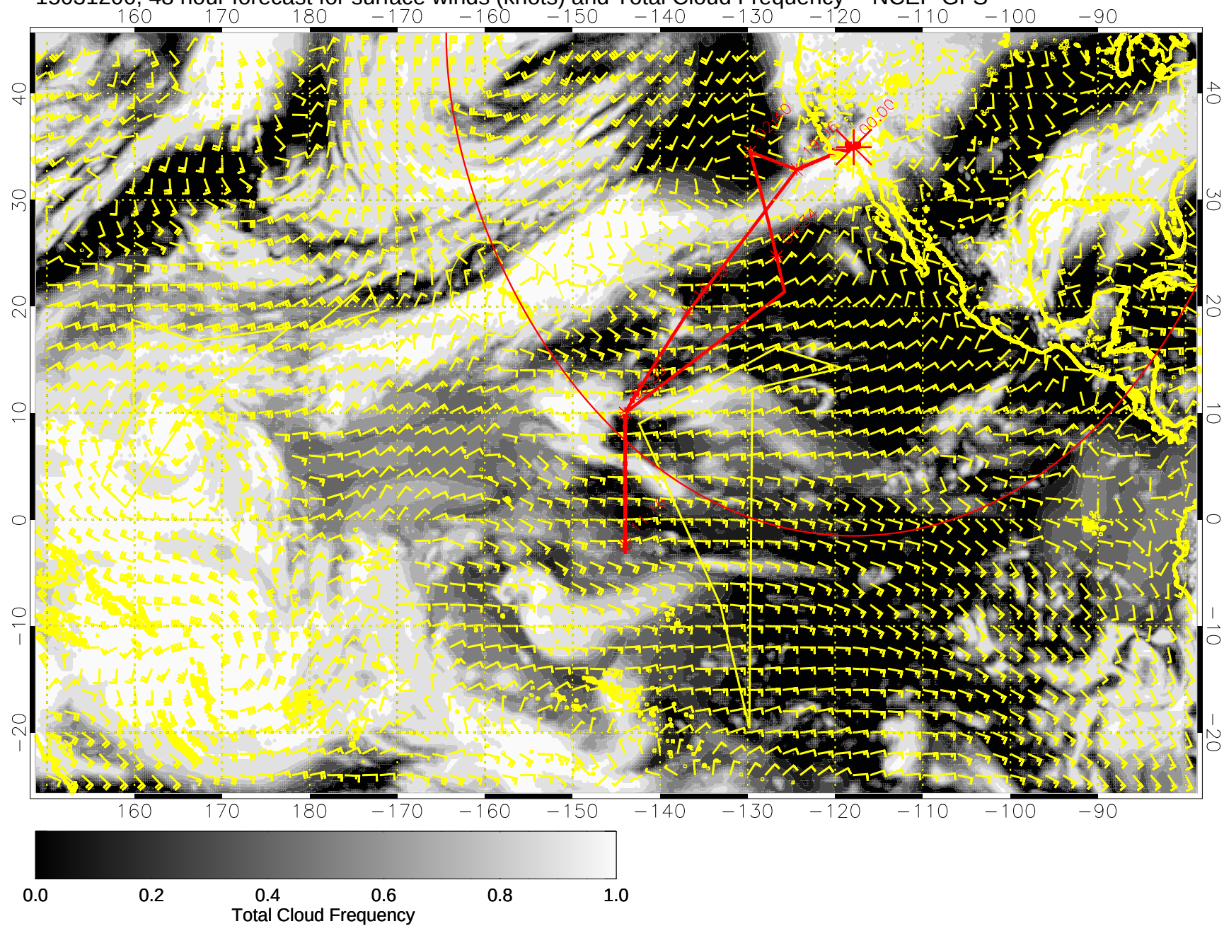
15031200, 48 hour forecast for surface winds (knots) and Total Cloud Frequency -- NCEP GFS
