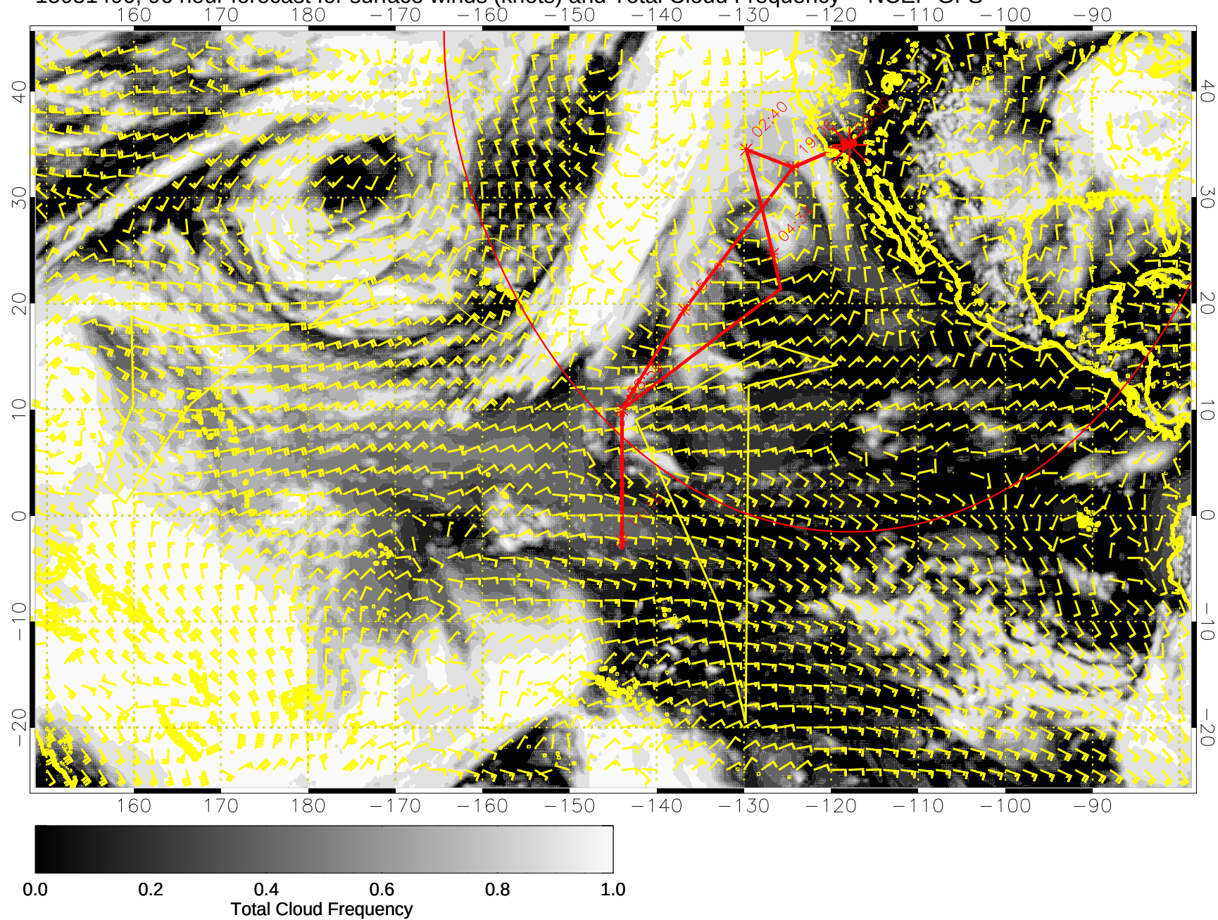
15031400, 96 hour forecast for surface winds (knots) and Total Cloud Frequency -- NCEP GFS
