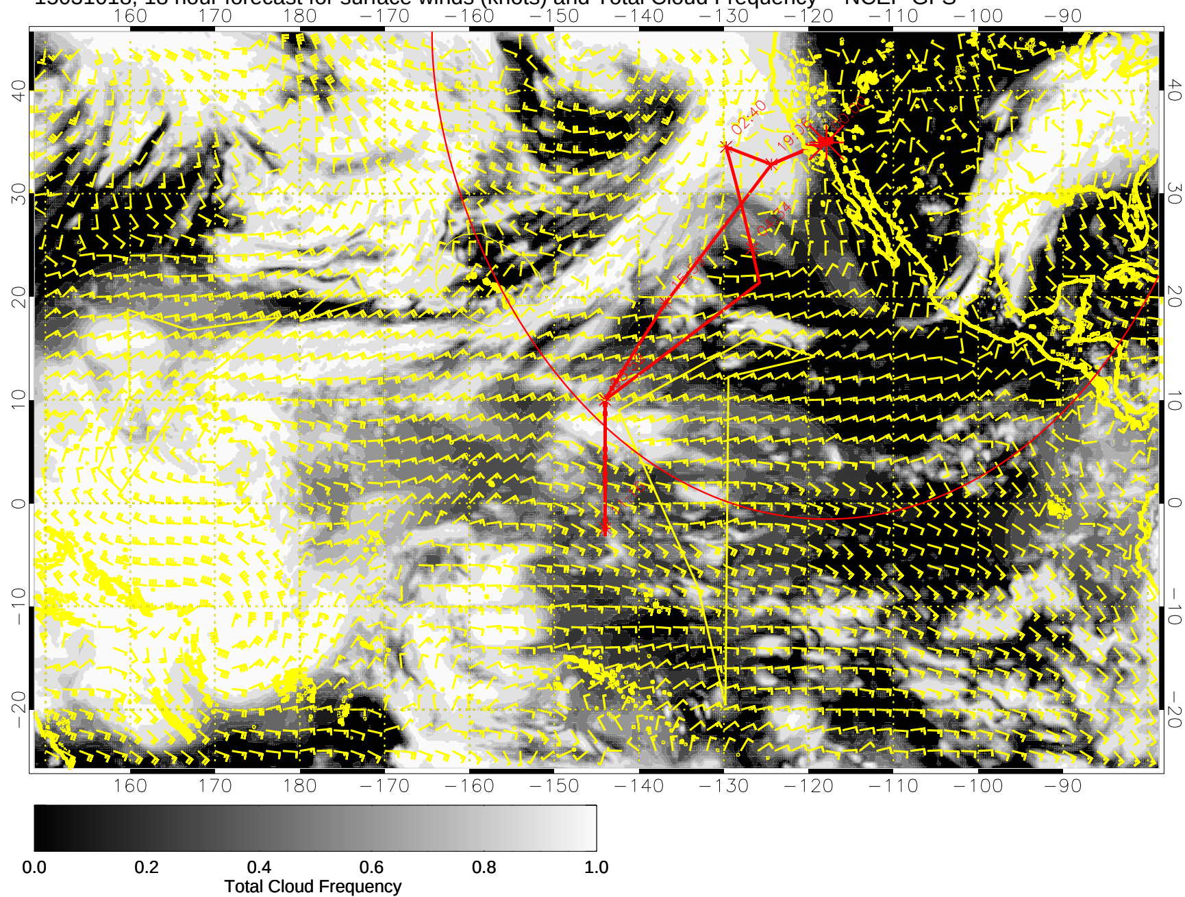
15031018, 18 hour forecast for surface winds (knots) and Total Cloud Frequency -- NCEP GFS
