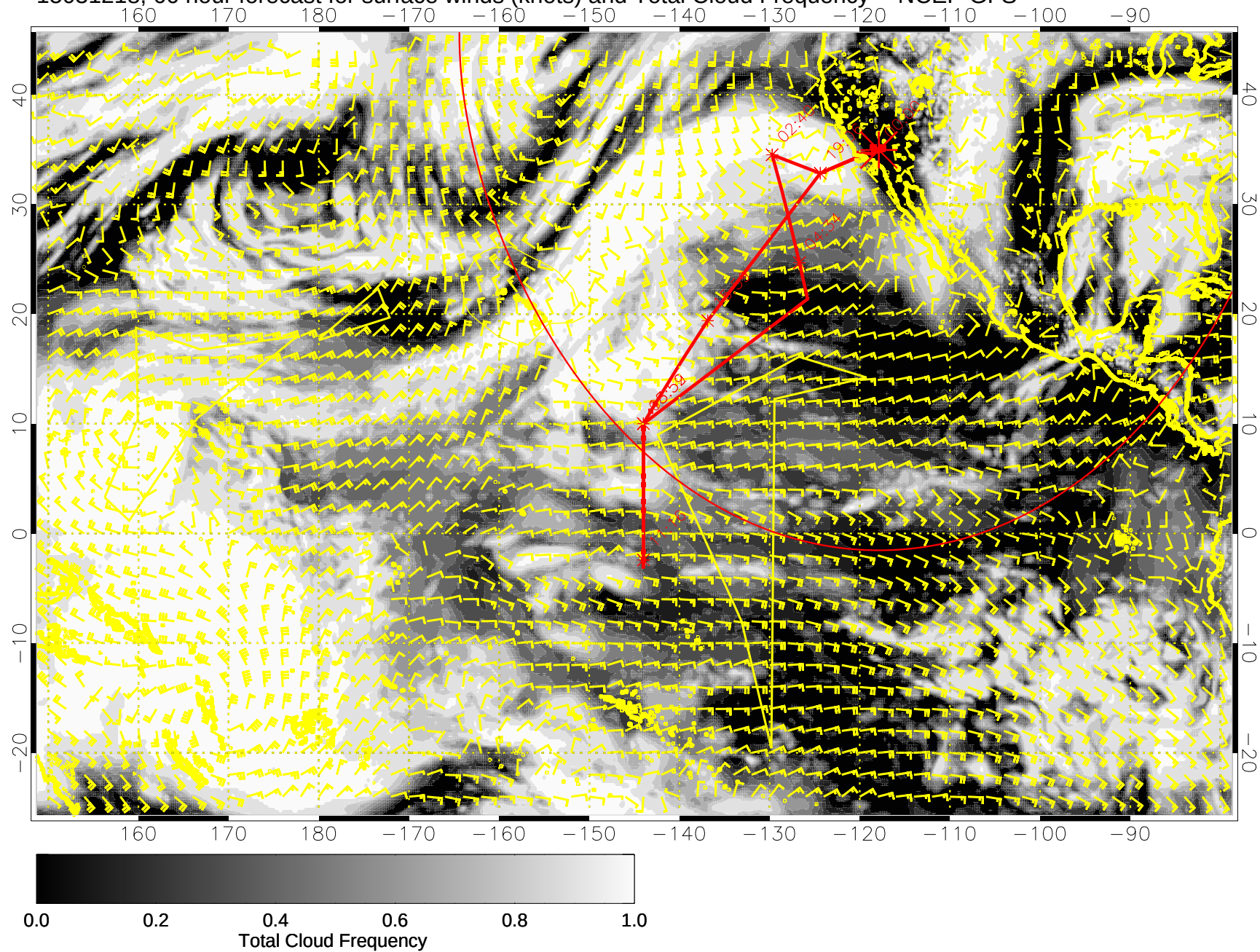
15031218, 66 hour forecast for surface winds (knots) and Total Cloud Frequency -- NCEP GFS
