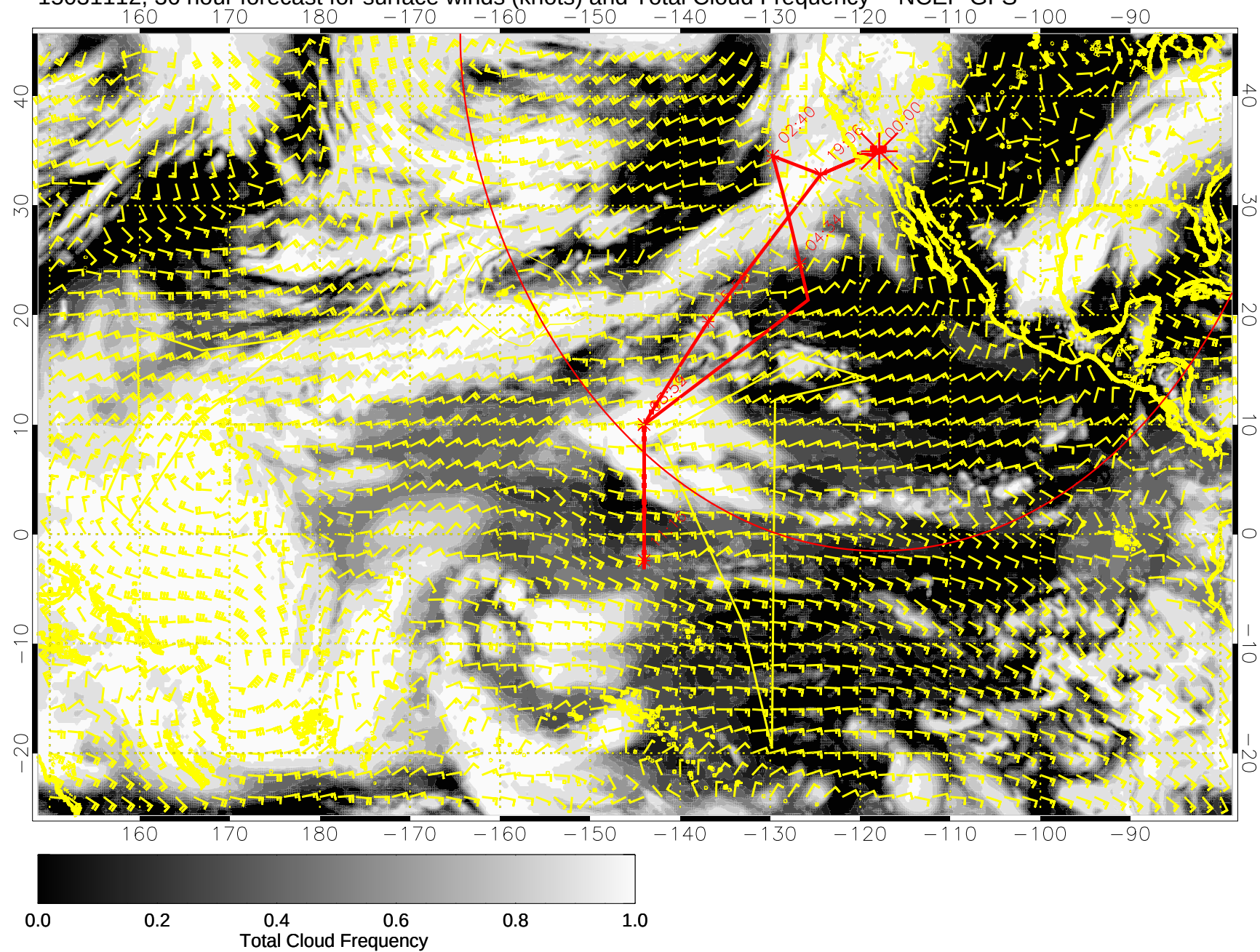
15031112, 36 hour forecast for surface winds (knots) and Total Cloud Frequency -- NCEP GFS
