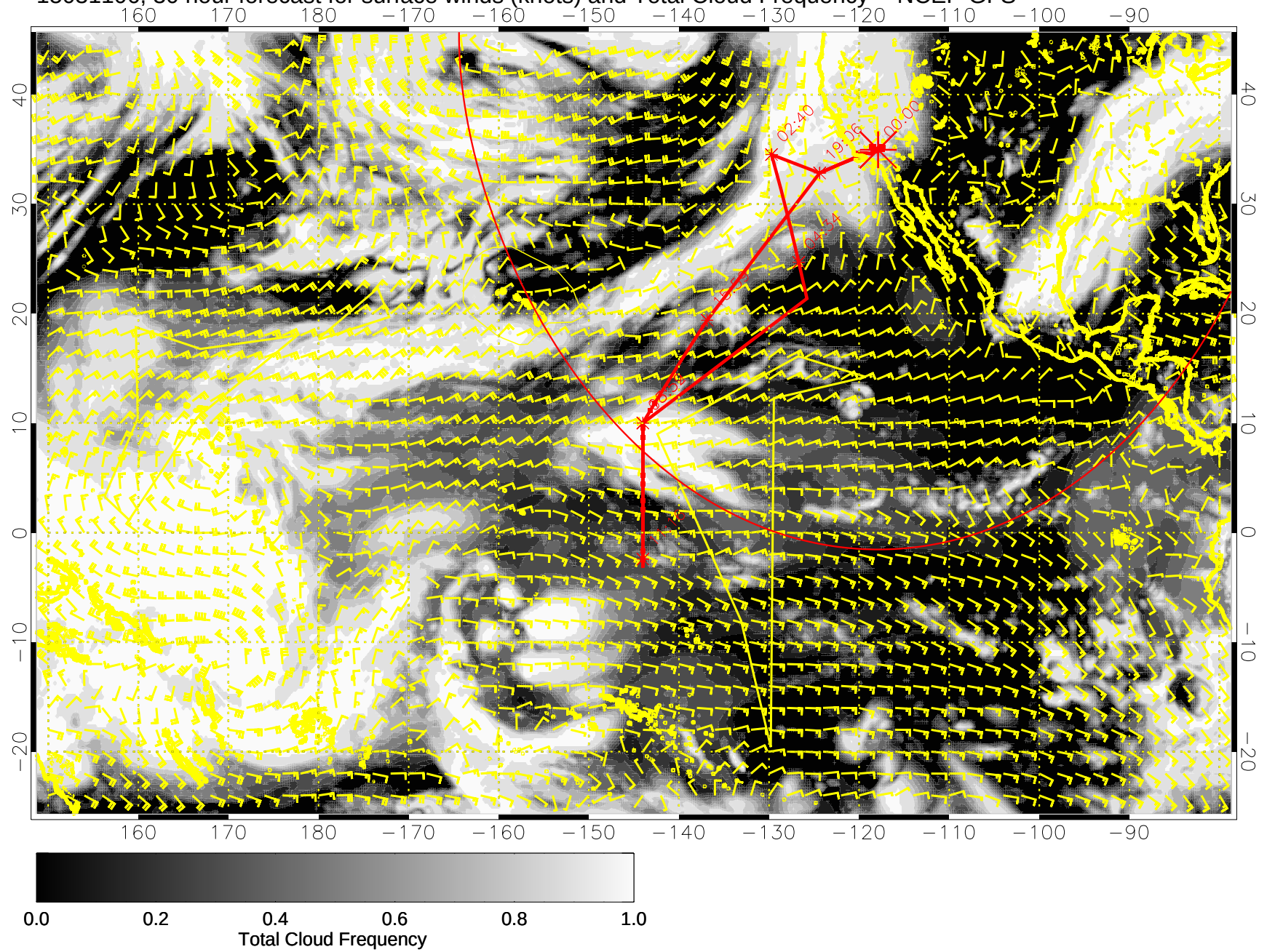
15031106, 30 hour forecast for surface winds (knots) and Total Cloud Frequency -- NCEP GFS
