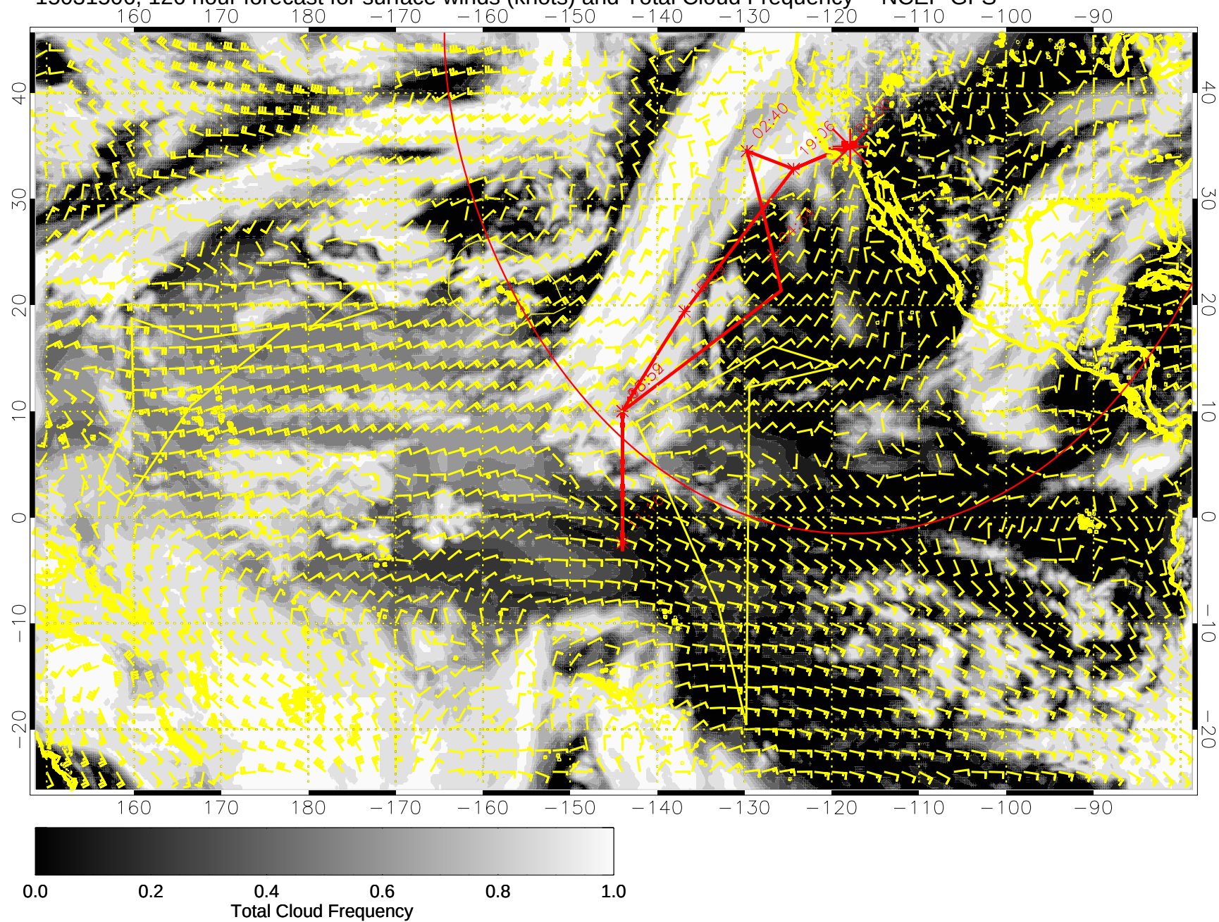
15031506, 126 hour forecast for surface winds (knots) and Total Cloud Frequency -- NCEP GFS
