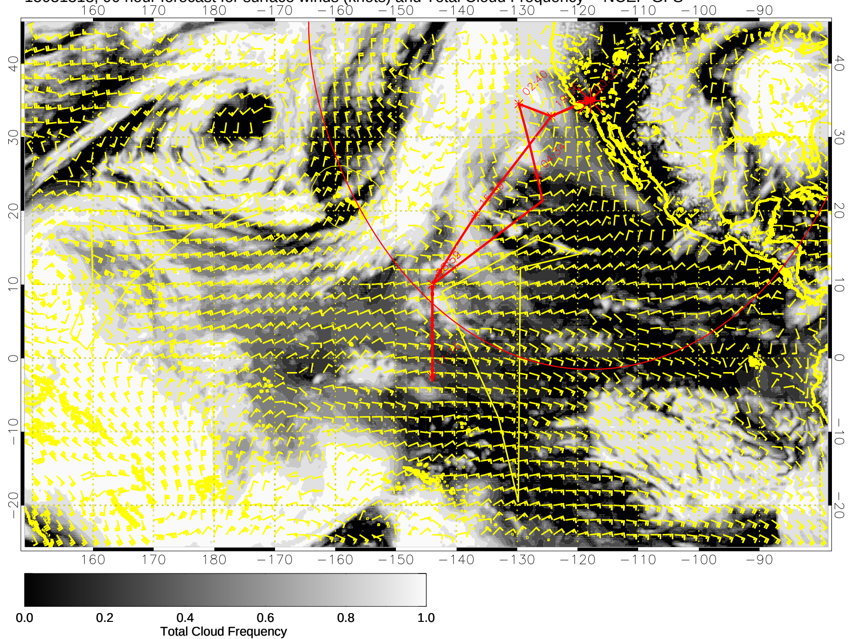
15031318, 90 hour forecast for surface winds (knots) and Total Cloud Frequency -- NCEP GFS
