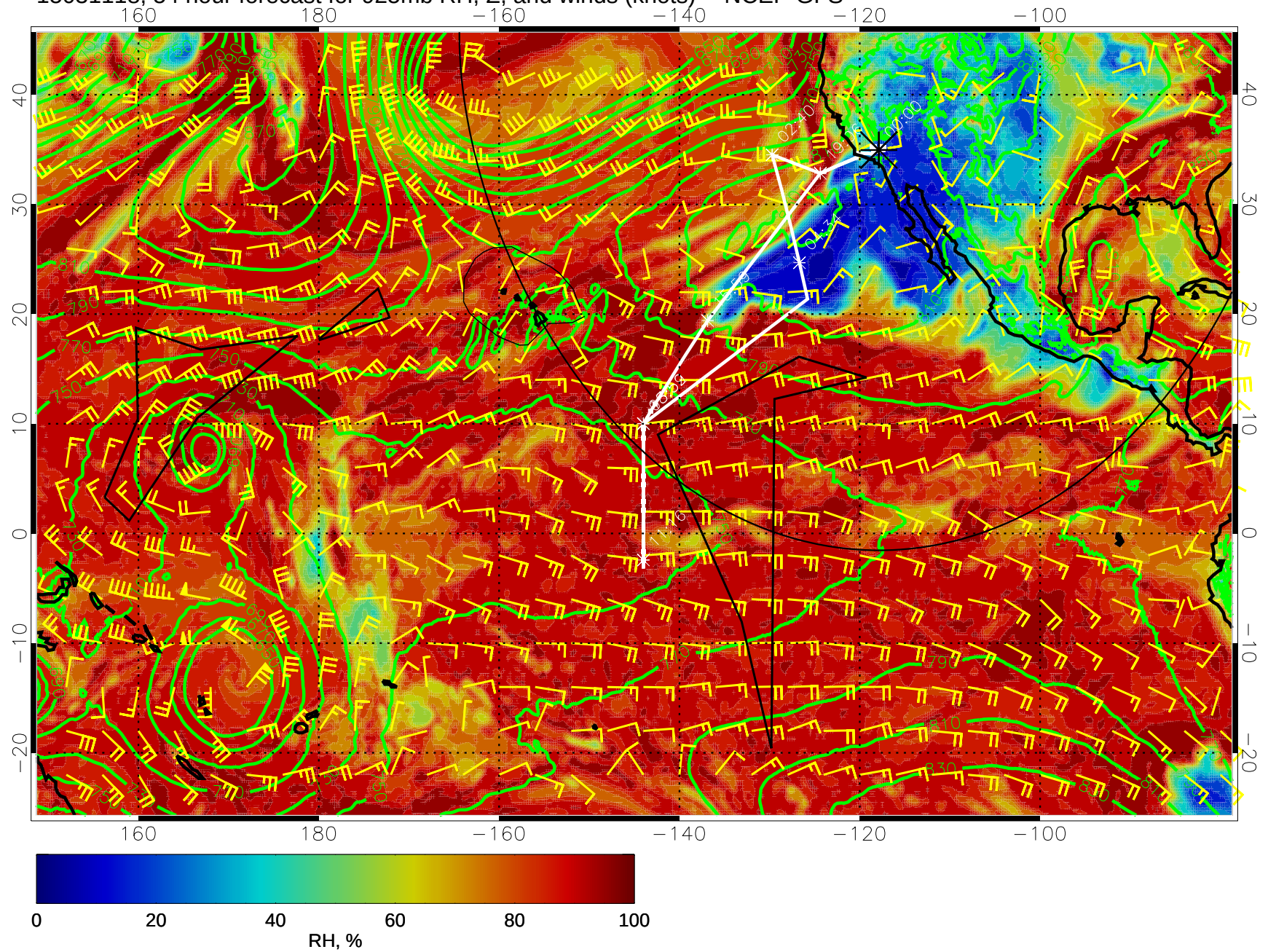
15031118, 54 hour forecast for 925mb RH, Z, and winds (knots) -- NCEP GFS
