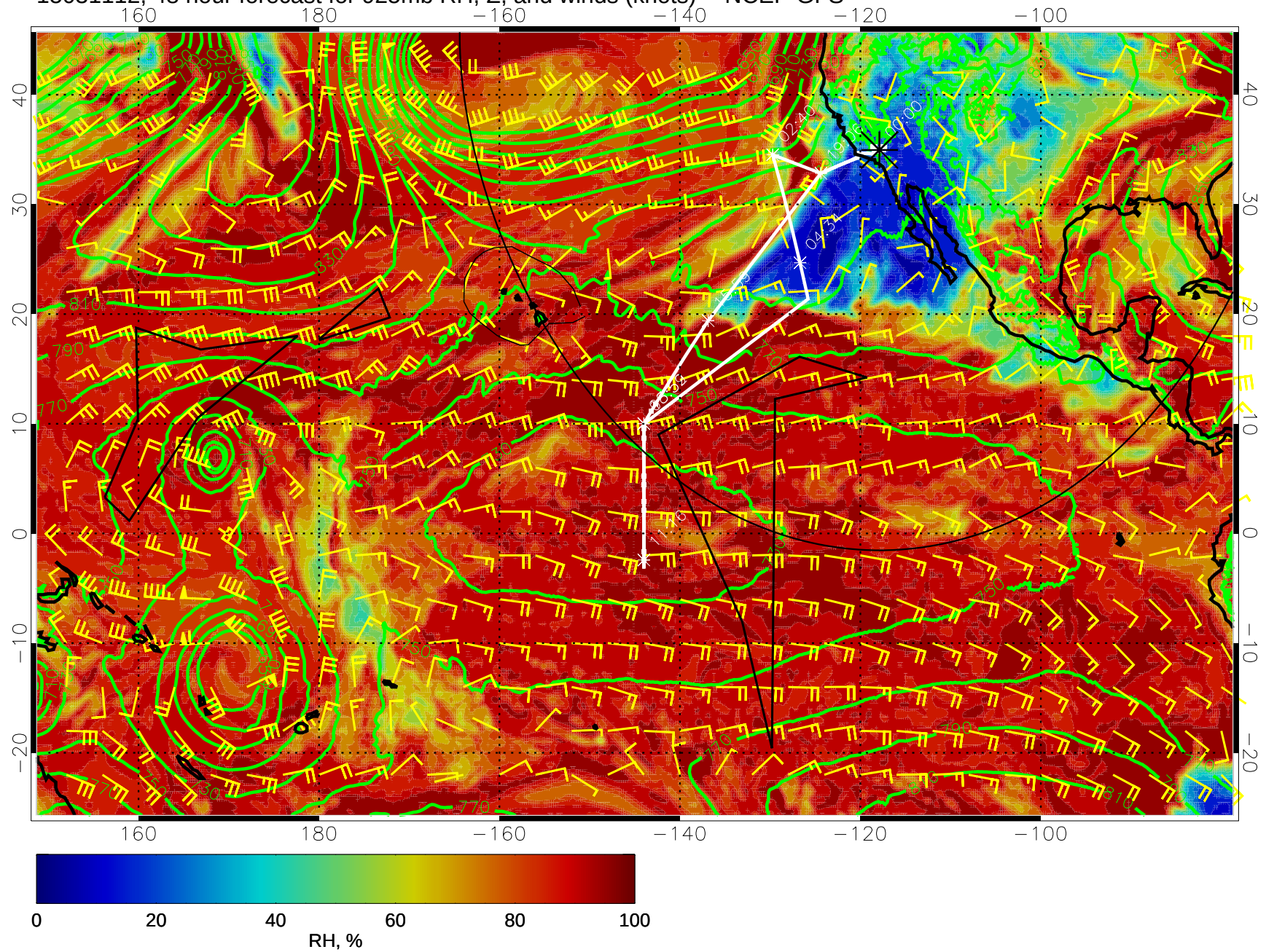
15031112, 48 hour forecast for 925mb RH, Z, and winds (knots) -- NCEP GFS
