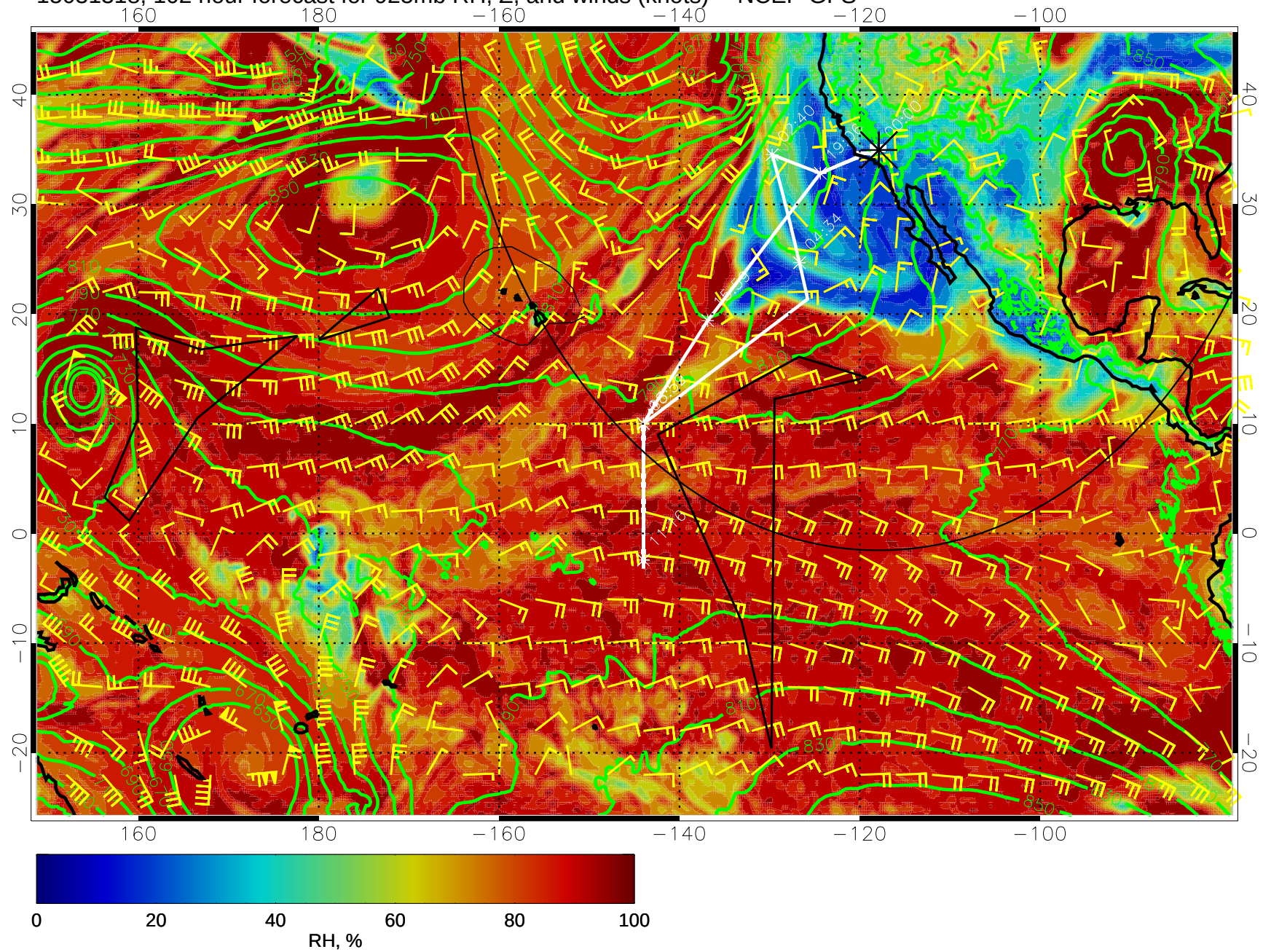
15031318, 102 hour forecast for 925mb RH, Z, and winds (knots) -- NCEP GFS
