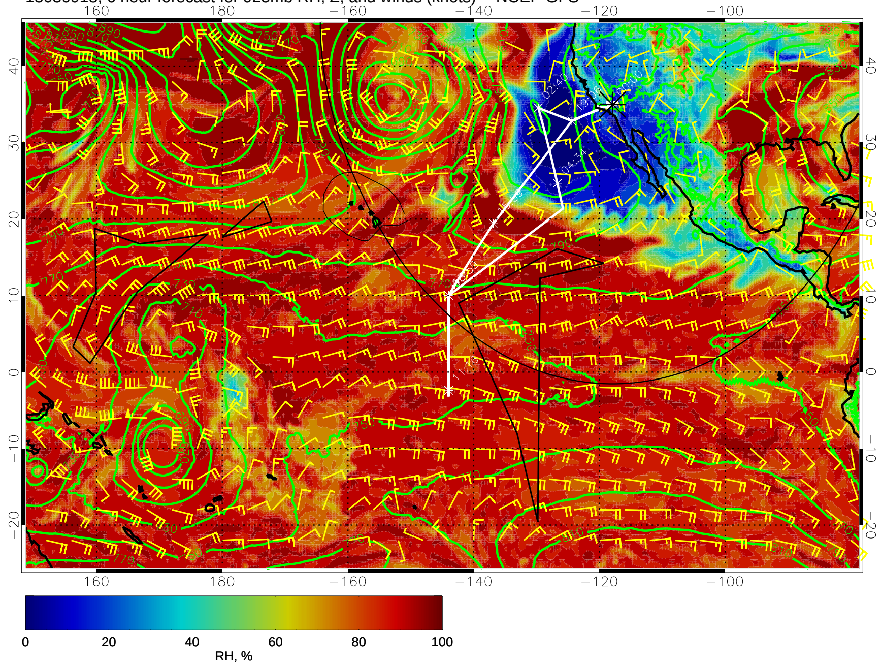
15030918, 6 hour forecast for 925mb RH, Z, and winds (knots) -- NCEP GFS
