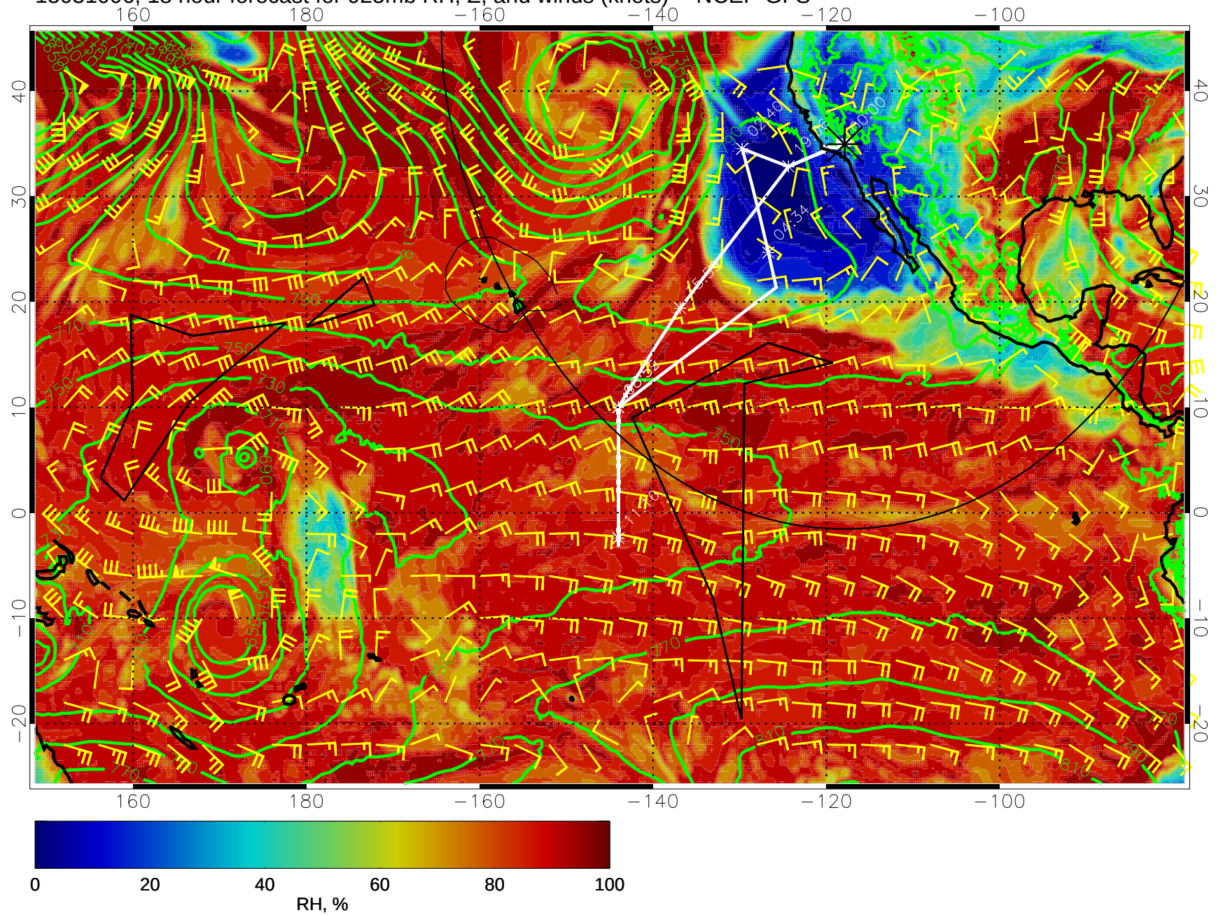
15031006, 18 hour forecast for 925mb RH, Z, and winds (knots) -- NCEP GFS
