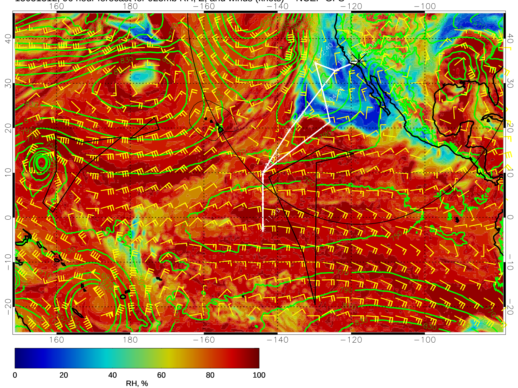
15031312, 96 hour forecast for 925mb RH, Z, and winds (knots) -- NCEP GFS
