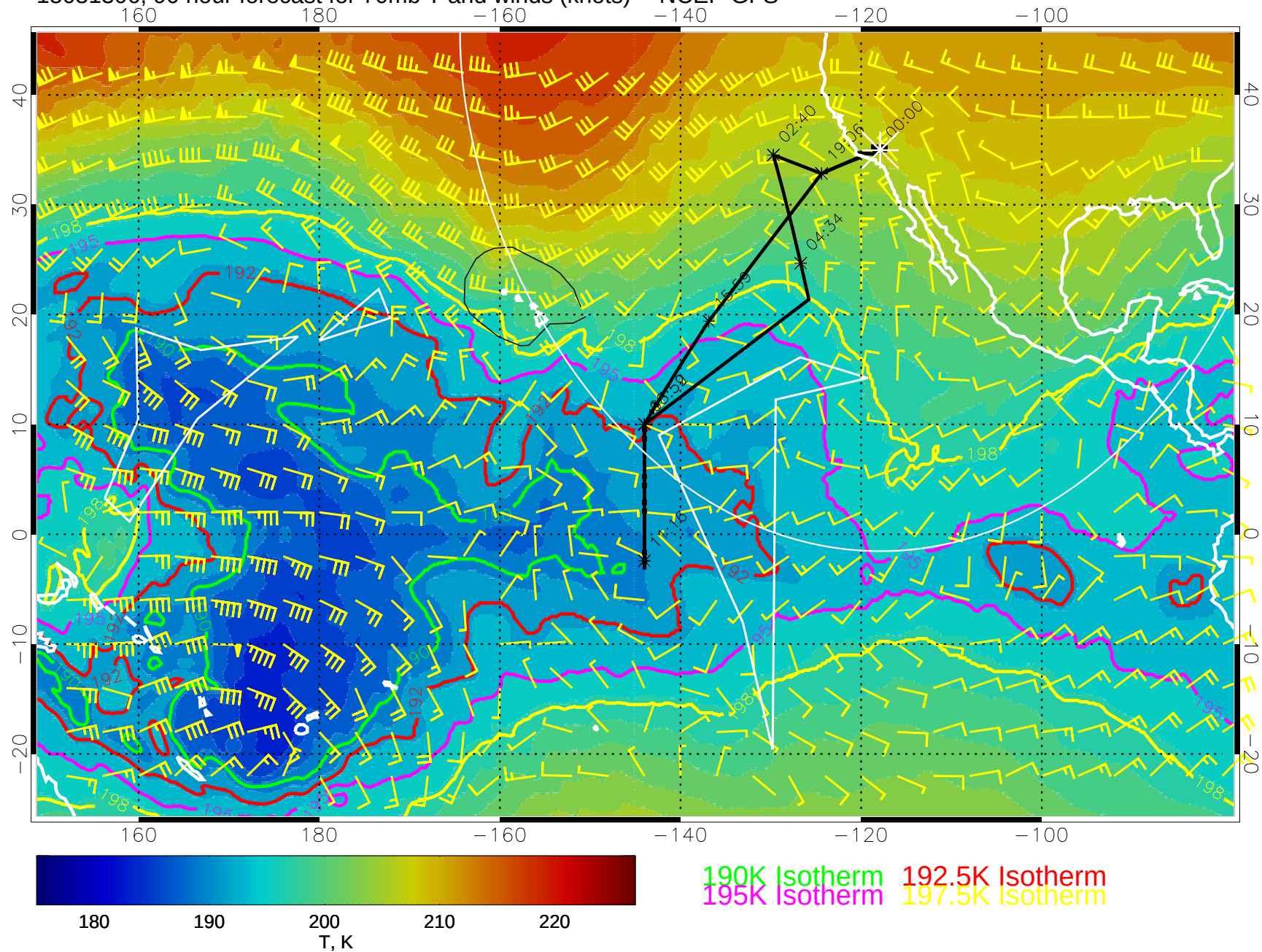
15031306, 90 hour forecast for 70mb T and winds (knots) -- NCEP GFS
