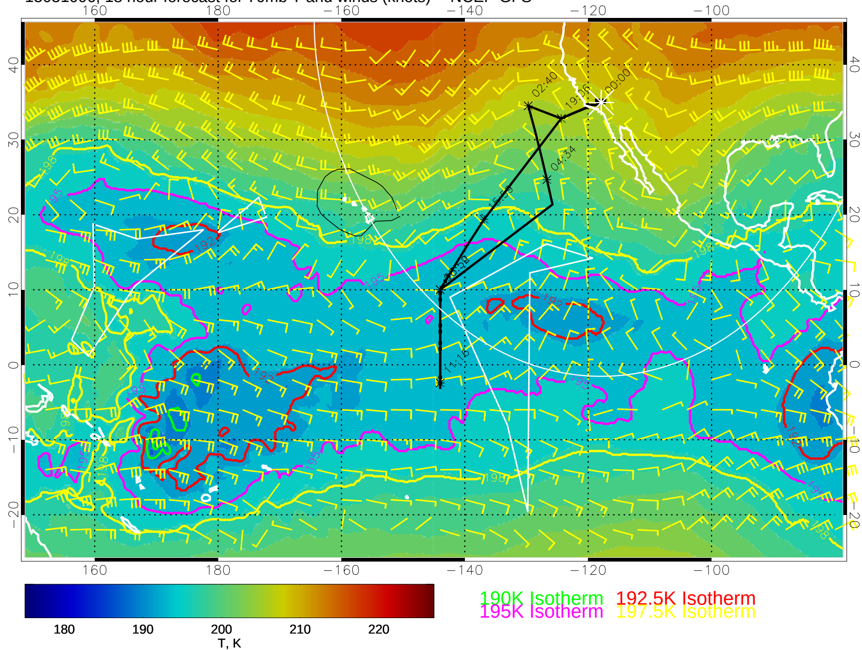
15031006, 18 hour forecast for 70mb T and winds (knots) -- NCEP GFS
