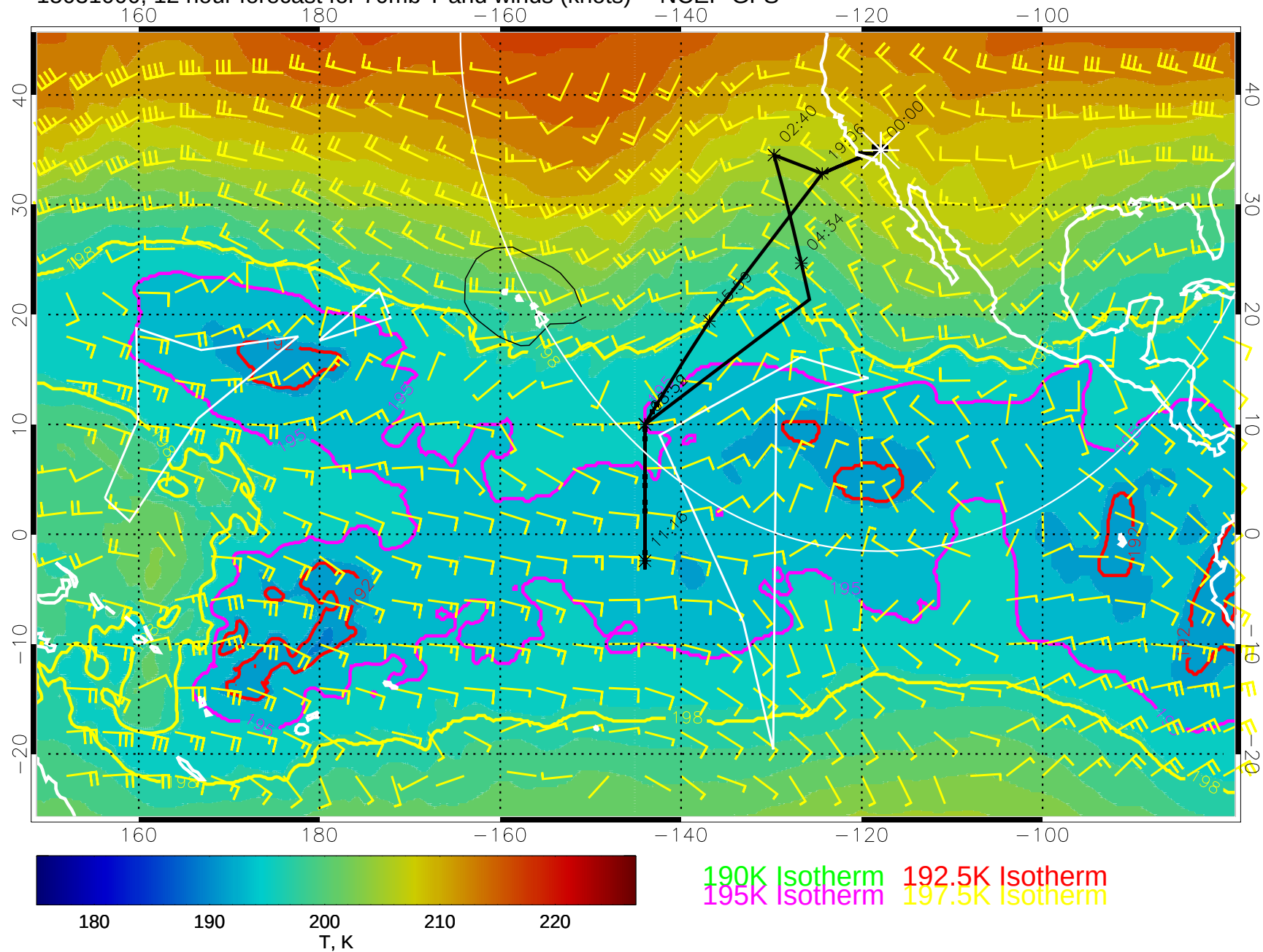
15031000, 12 hour forecast for 70mb T and winds (knots) -- NCEP GFS
