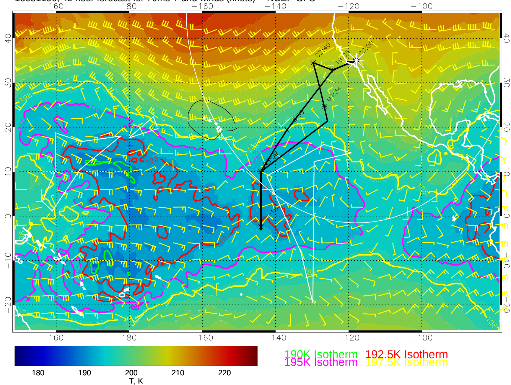
15031106, 42 hour forecast for 70mb T and winds (knots) -- NCEP GFS
