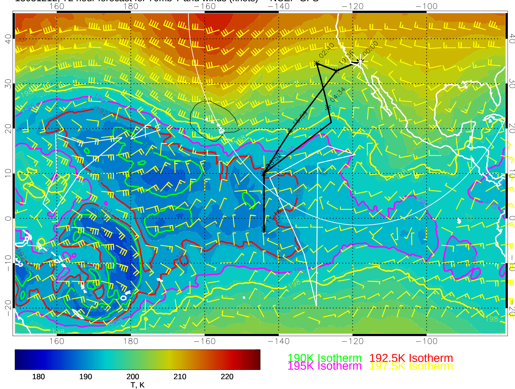
15031212, 72 hour forecast for 70mb T and winds (knots) -- NCEP GFS
