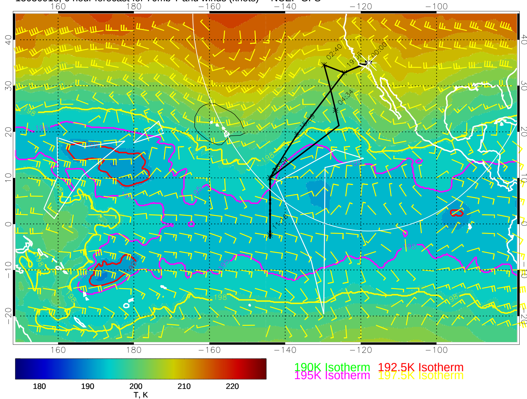
15030918, 6 hour forecast for 70mb T and winds (knots) -- NCEP GFS
