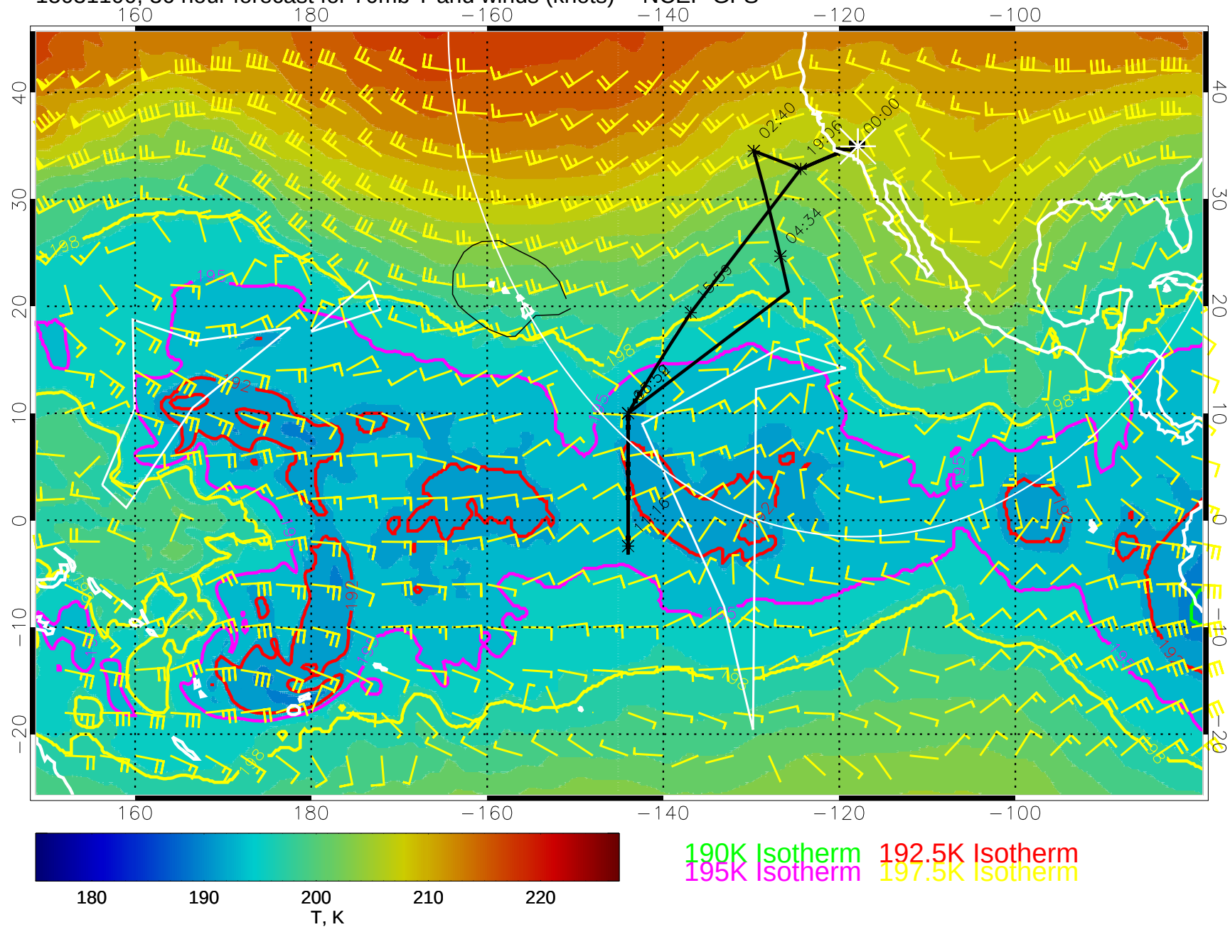
15031100, 36 hour forecast for 70mb T and winds (knots) -- NCEP GFS
