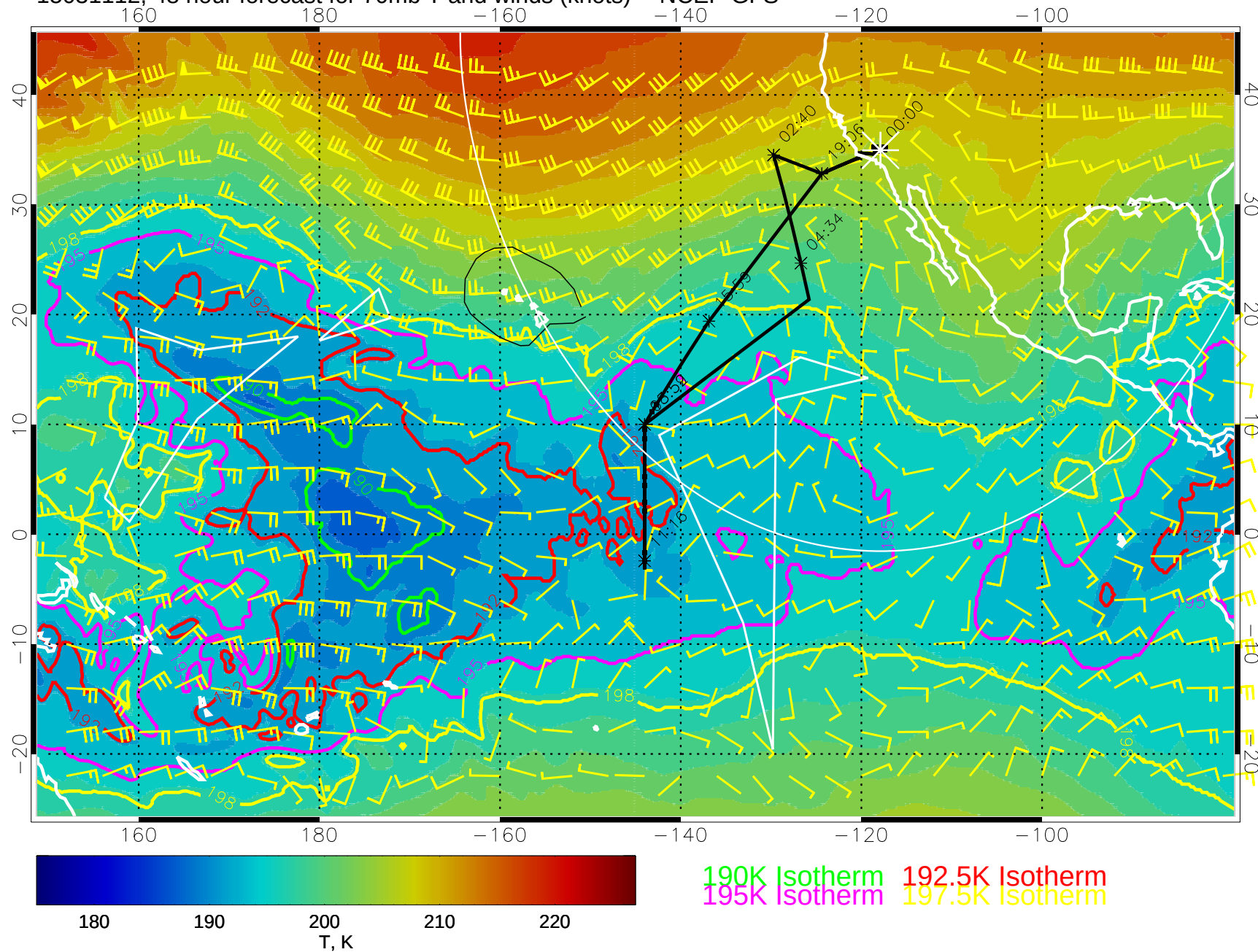
15031112, 48 hour forecast for 70mb T and winds (knots) -- NCEP GFS
