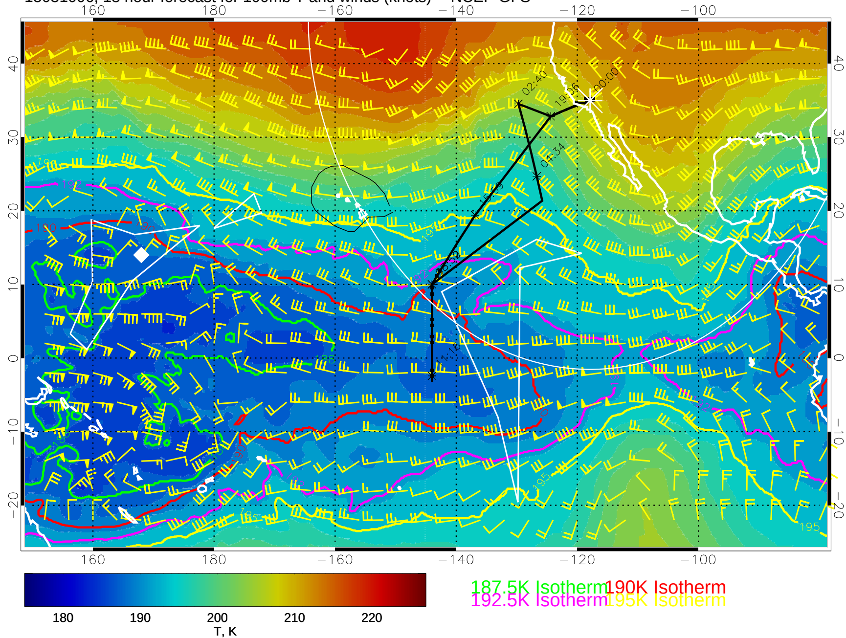
15031006, 18 hour forecast for 100mb T and winds (knots) -- NCEP GFS
