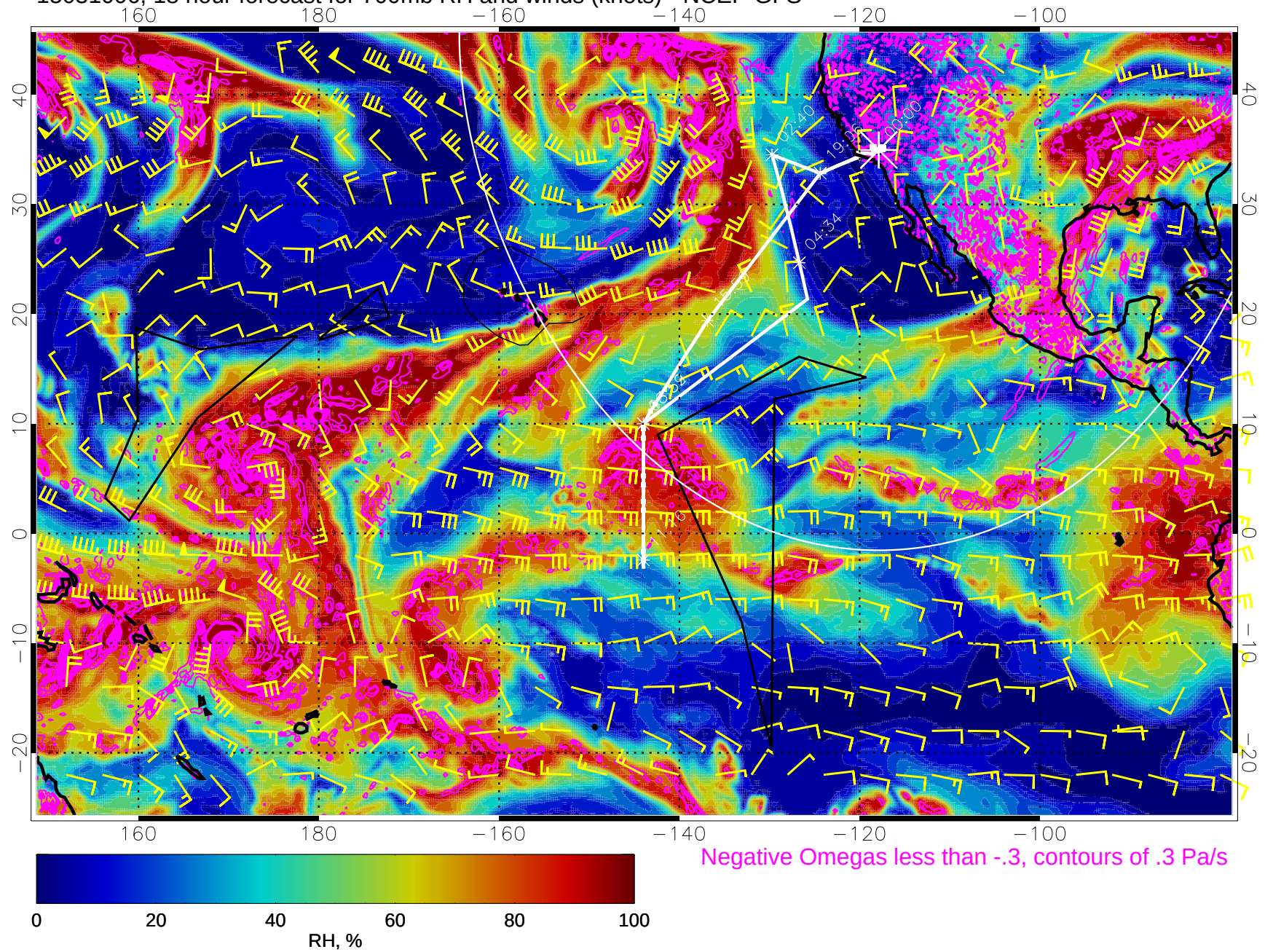
15031006, 18 hour forecast for 700mb RH and winds (knots) - NCEP GFS
