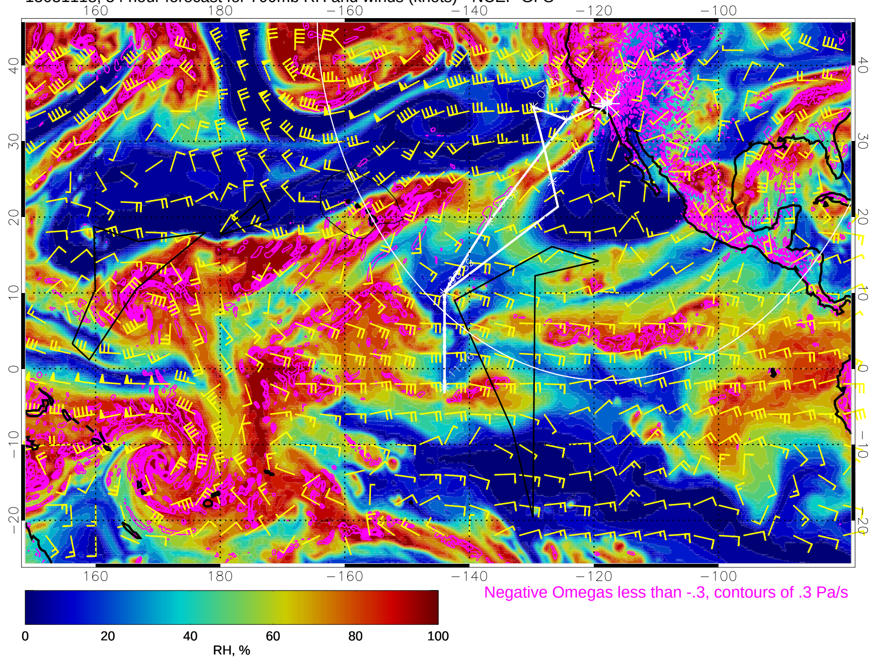
15031118, 54 hour forecast for 700mb RH and winds (knots) - NCEP GFS
