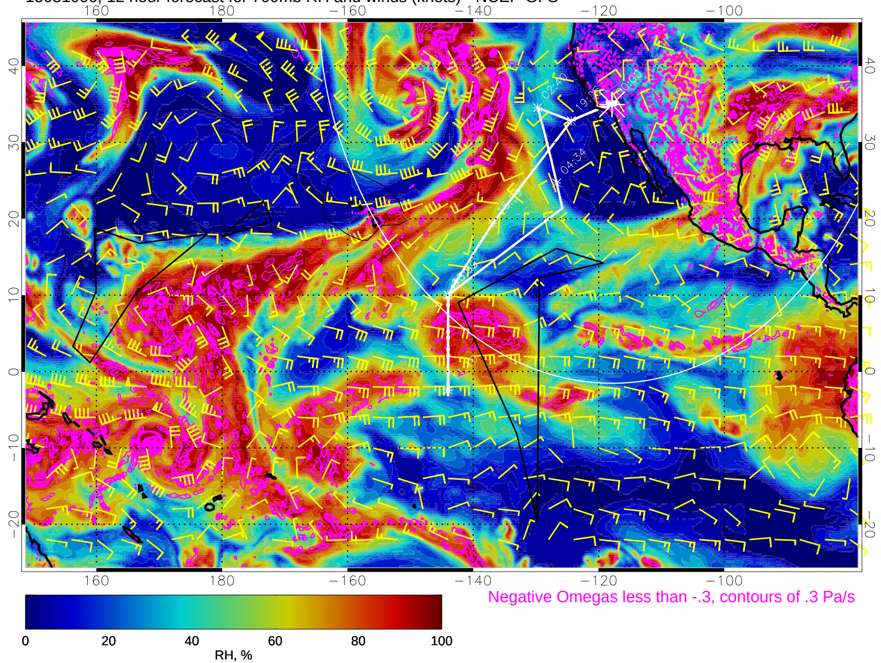
15031000, 12 hour forecast for 700mb RH and winds (knots) - NCEP GFS
