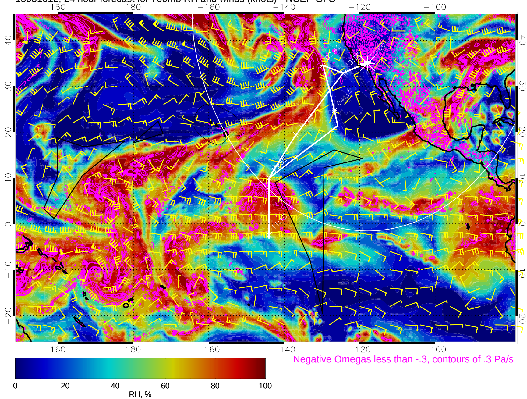
15031012, 24 hour forecast for 700mb RH and winds (knots) - NCEP GFS
