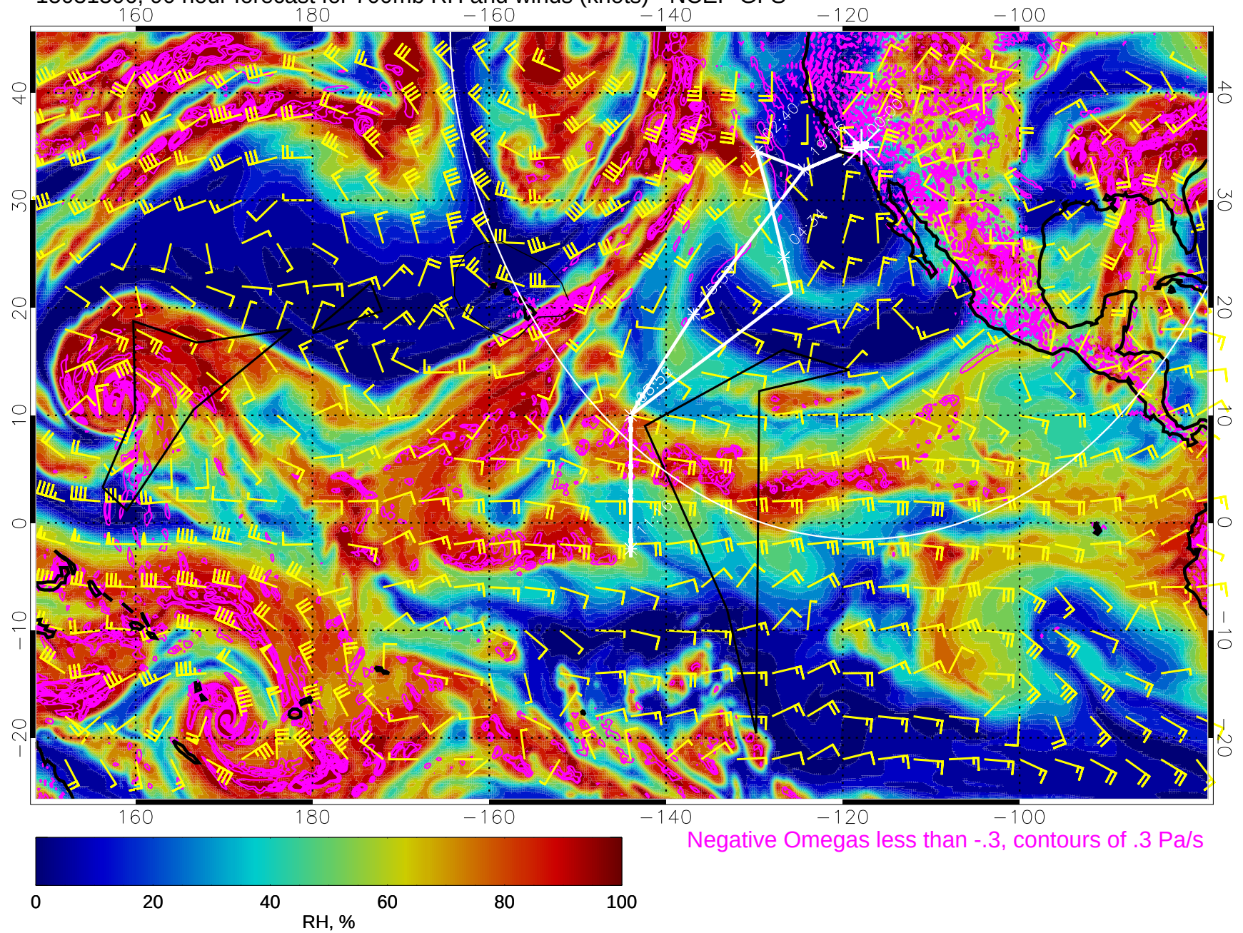
15031306, 90 hour forecast for 700mb RH and winds (knots) - NCEP GFS
