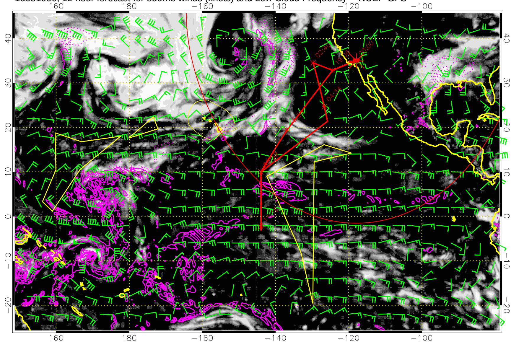
15031000, 12 hour forecast for 850mb winds (knots) and Low Cloud Frequency -- NCEP GFS
