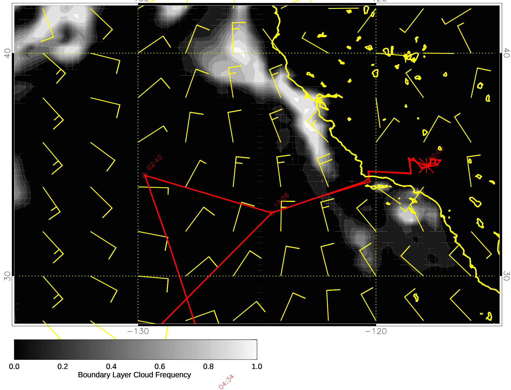
15030918, 6 hour forecast for surface winds (knots) and Boundary Layer Cloud Frequency -- NCEP GFS
