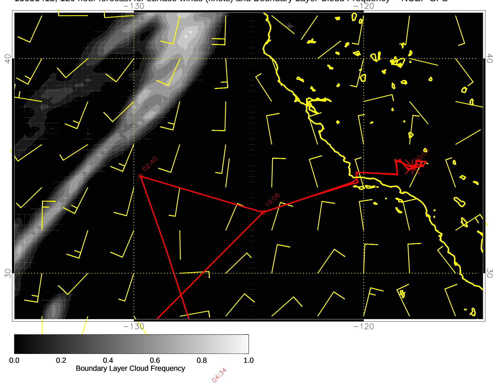
15031412, 120 hour forecast for surface winds (knots) and Boundary Layer Cloud Frequency -- NCEP GFS
