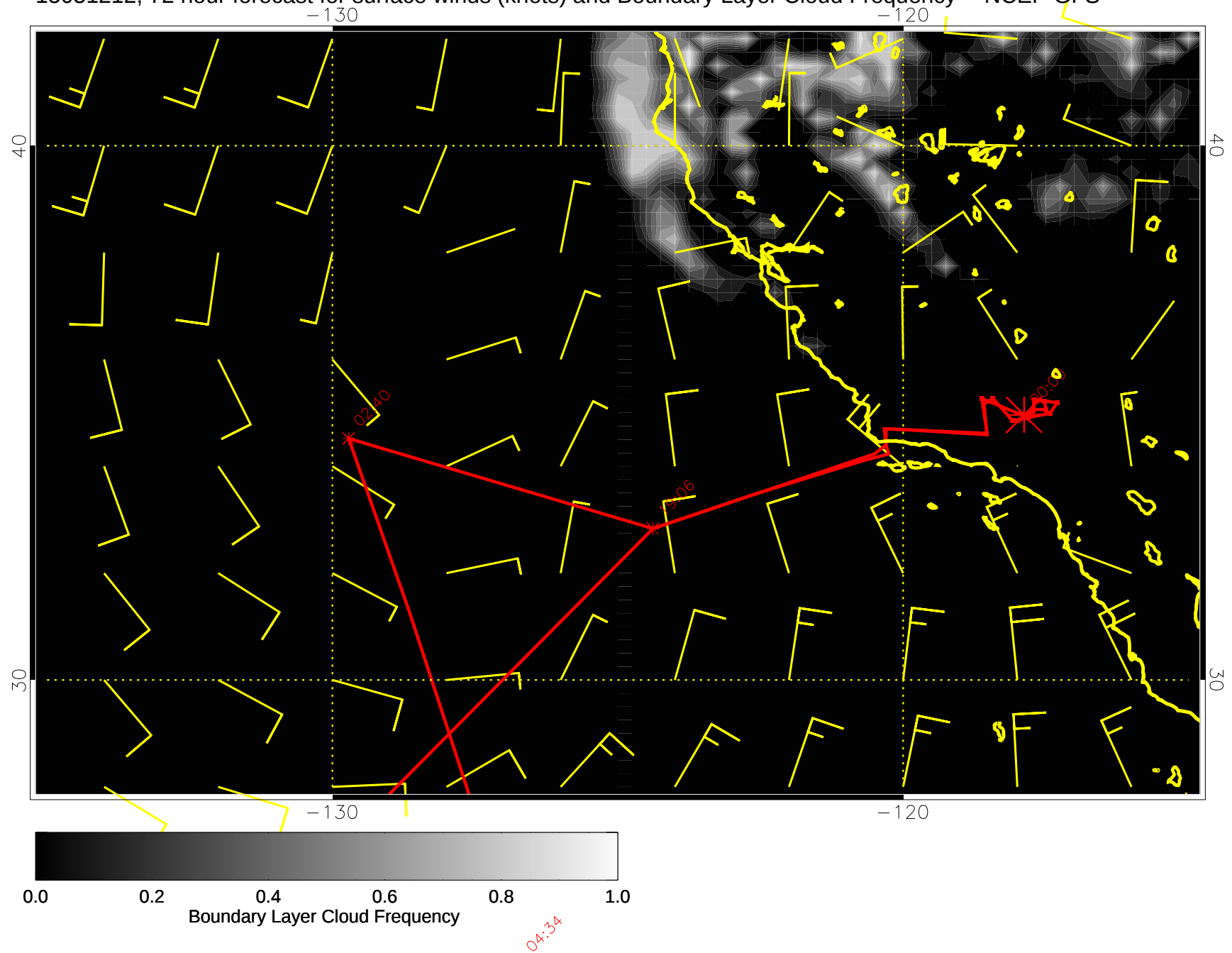
15031212, 72 hour forecast for surface winds (knots) and Boundary Layer Cloud Frequency -- NCEP GFS
