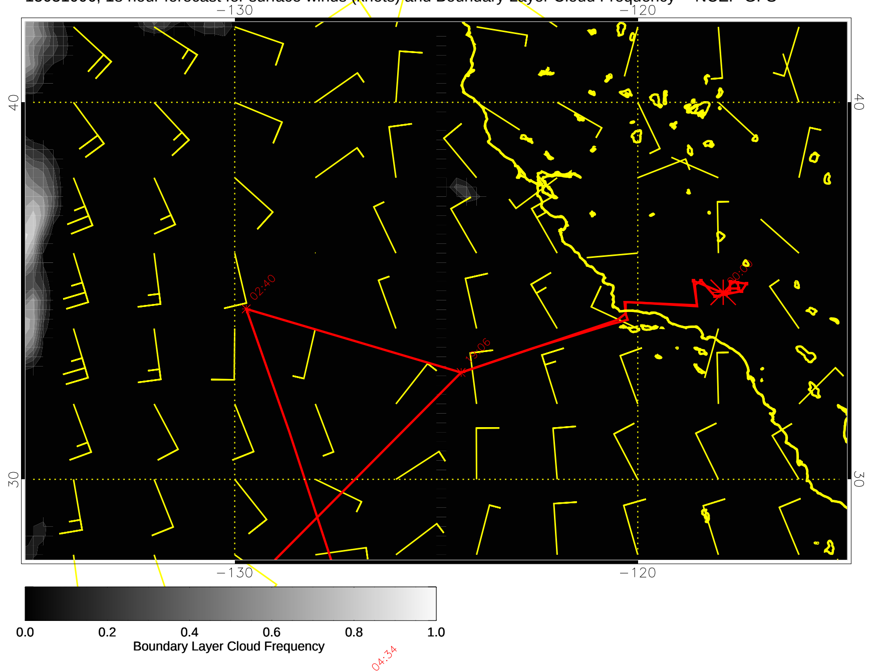
15031006, 18 hour forecast for surface winds (knots) and Boundary Layer Cloud Frequency -- NCEP GFS
