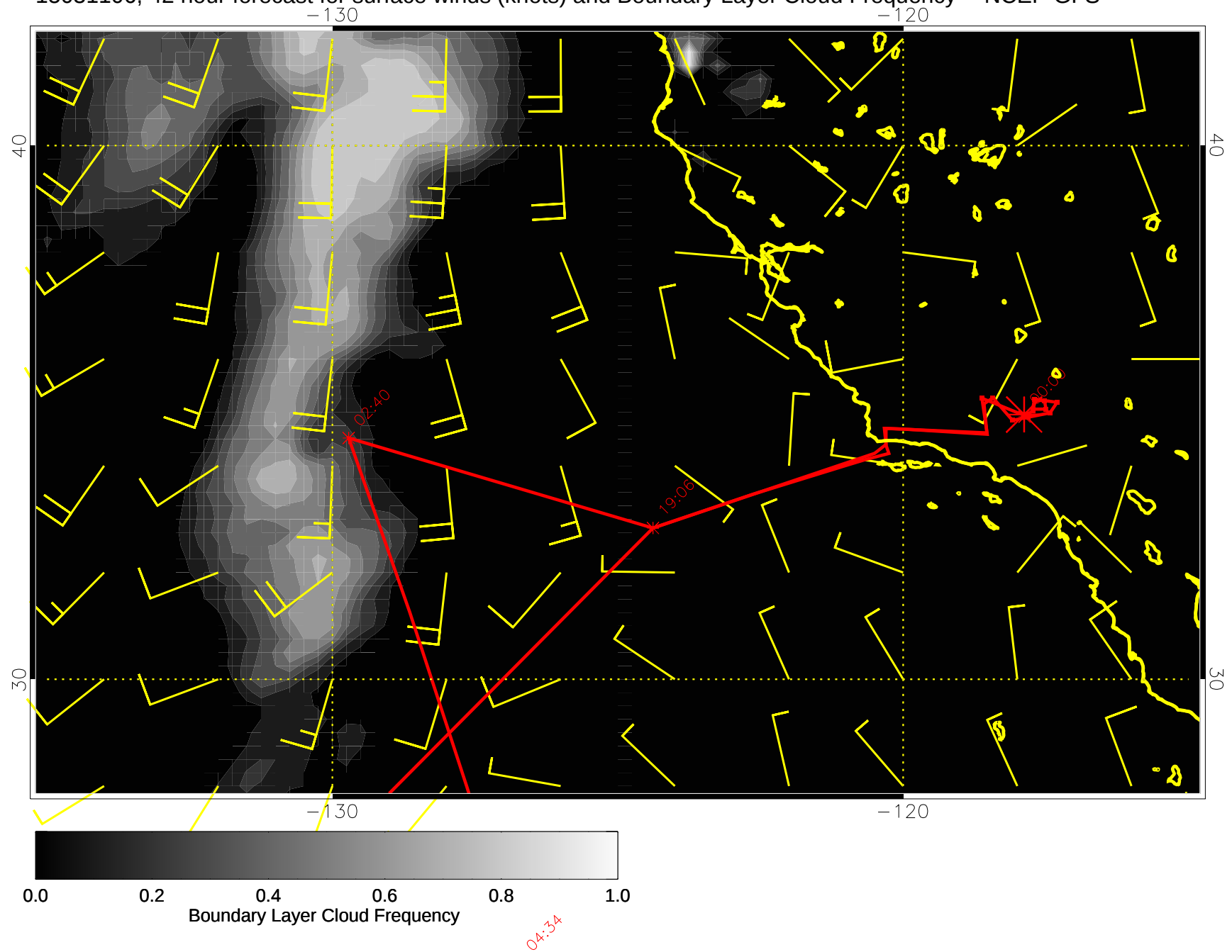
15031106, 42 hour forecast for surface winds (knots) and Boundary Layer Cloud Frequency -- NCEP GFS
