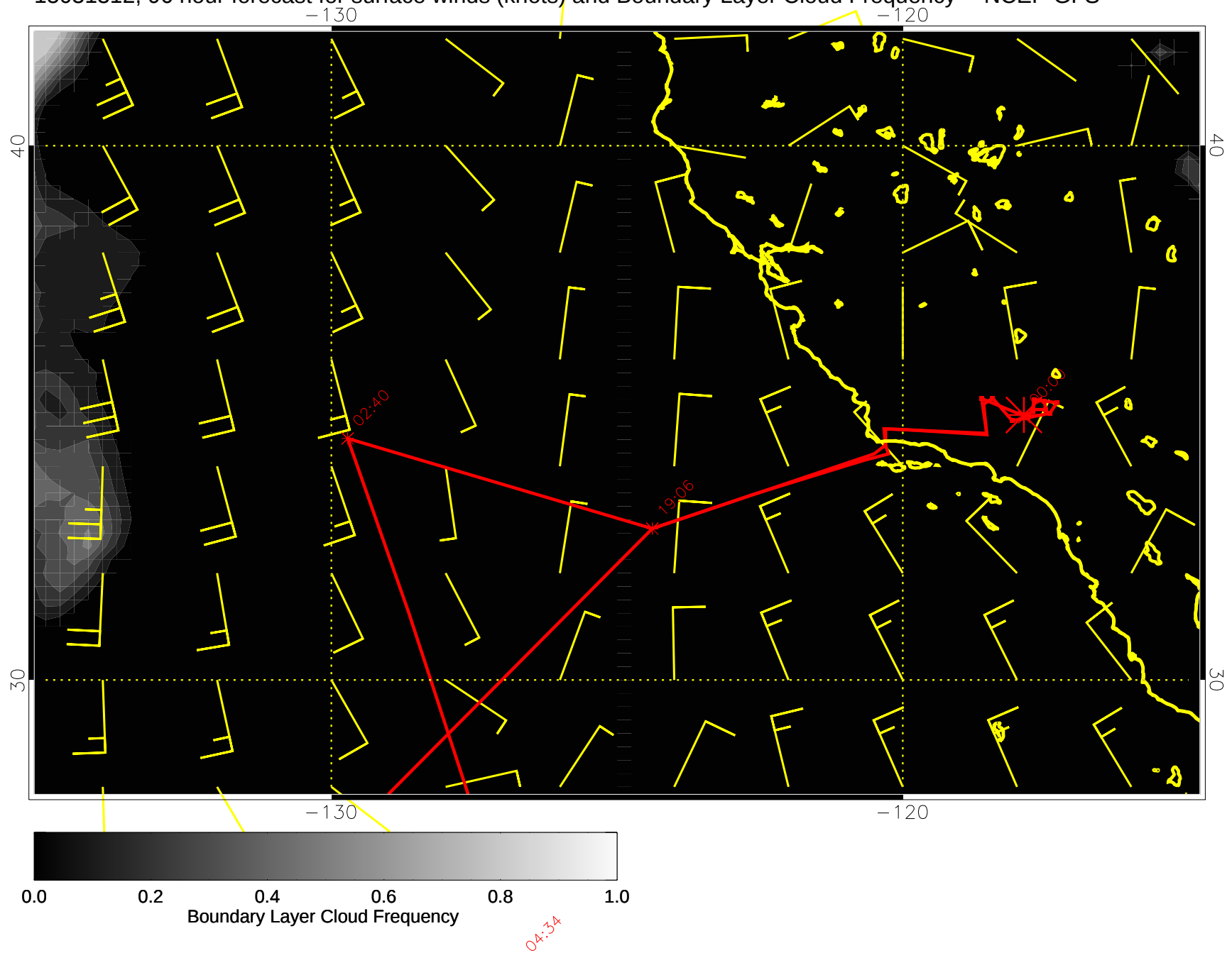
15031312, 96 hour forecast for surface winds (knots) and Boundary Layer Cloud Frequency -- NCEP GFS
