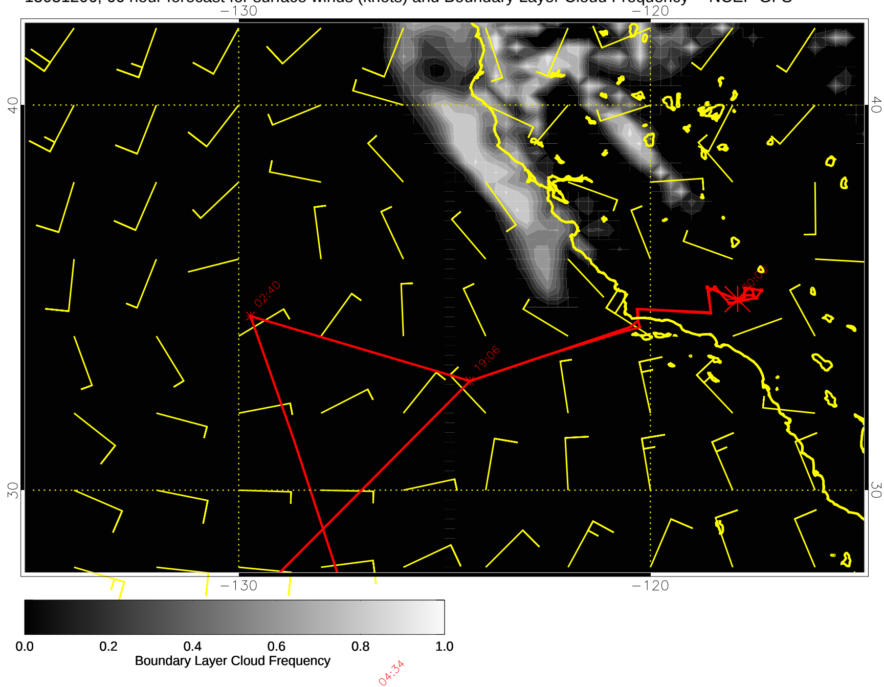
15031206, 66 hour forecast for surface winds (knots) and Boundary Layer Cloud Frequency -- NCEP GFS
