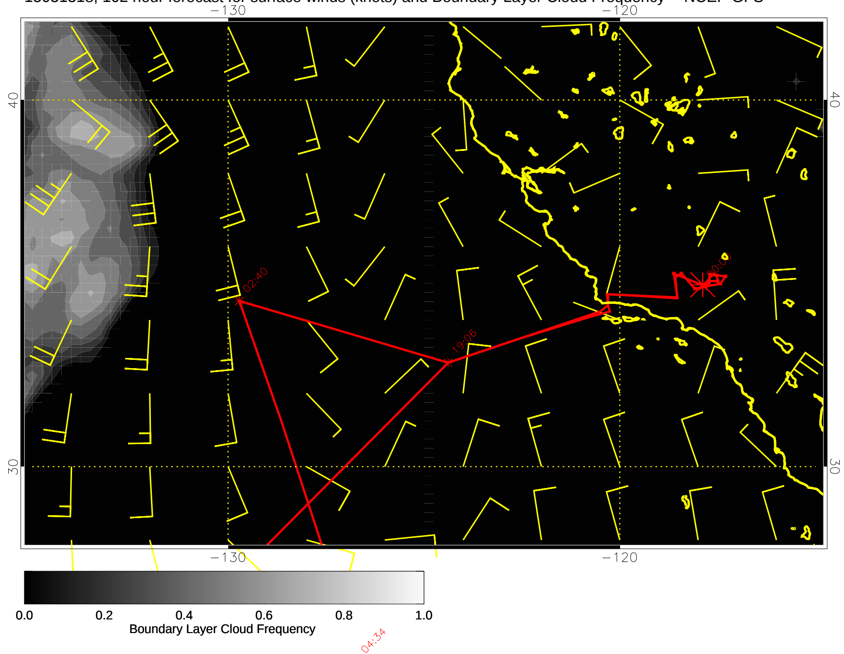
15031318, 102 hour forecast for surface winds (knots) and Boundary Layer Cloud Frequency -- NCEP GFS
