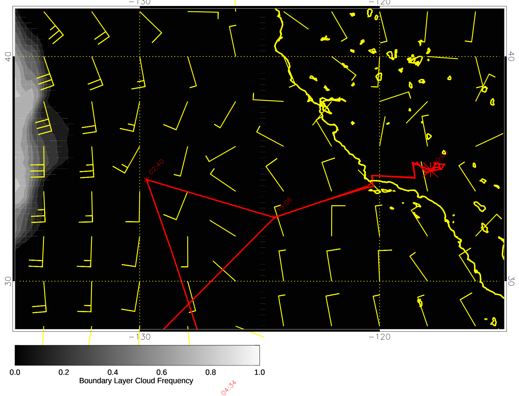
15031012, 24 hour forecast for surface winds (knots) and Boundary Layer Cloud Frequency -- NCEP GFS
