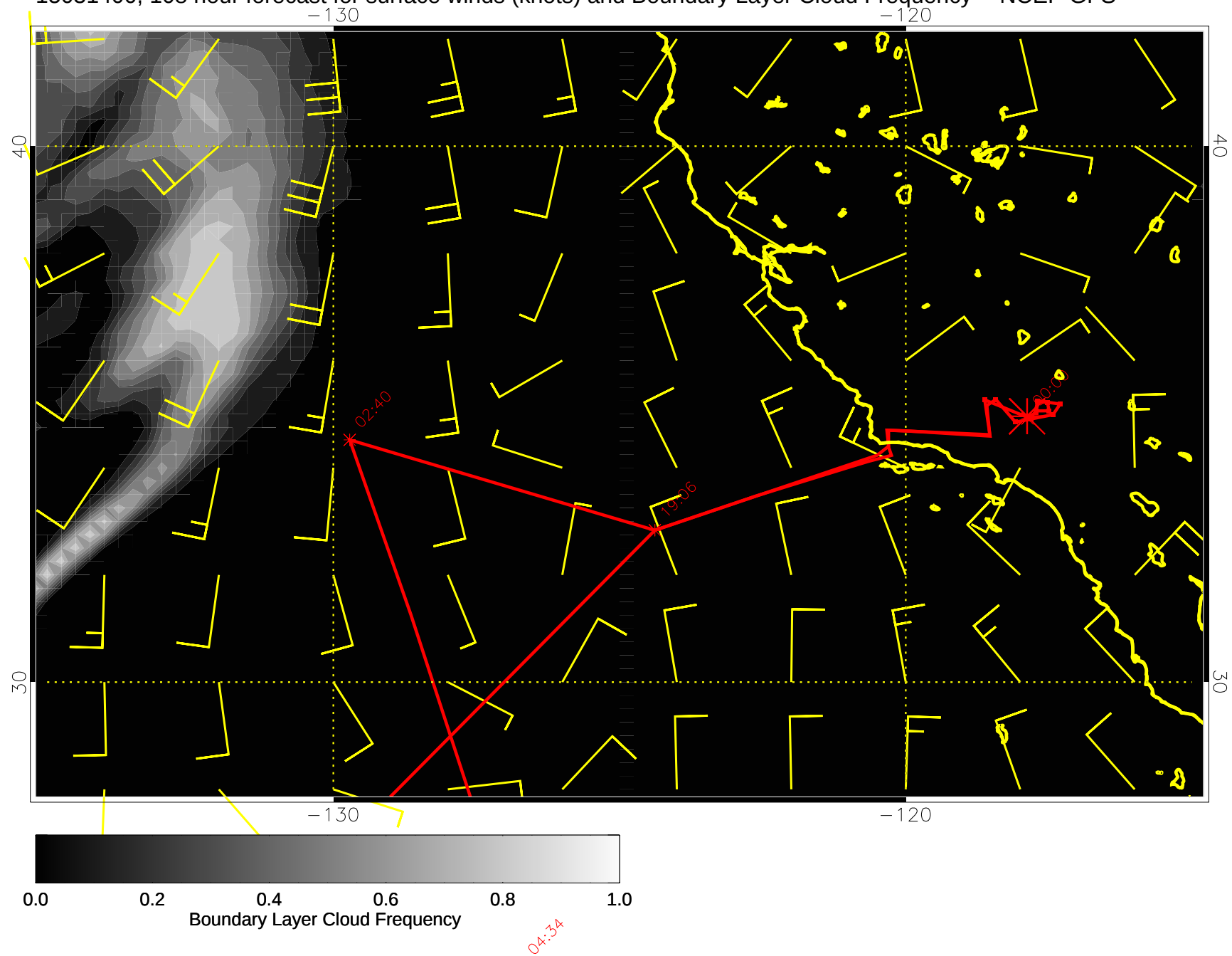
15031400, 108 hour forecast for surface winds (knots) and Boundary Layer Cloud Frequency -- NCEP GFS
