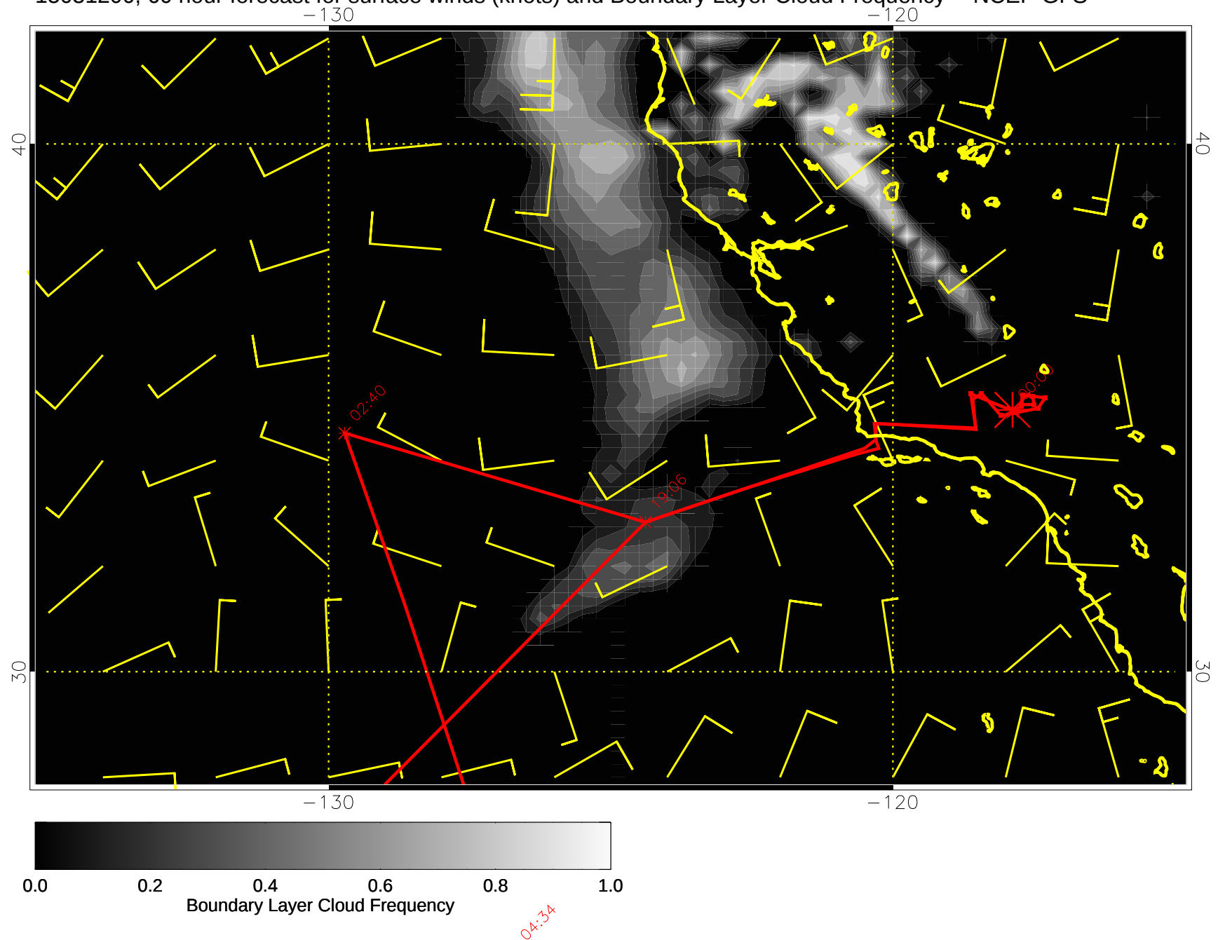
15031200, 60 hour forecast for surface winds (knots) and Boundary Layer Cloud Frequency -- NCEP GFS
