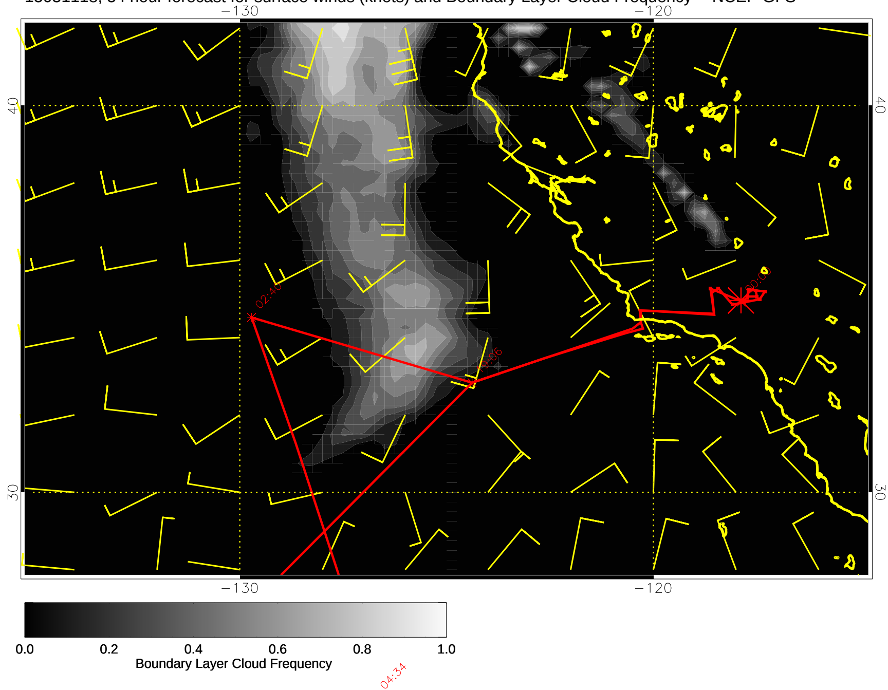
15031118, 54 hour forecast for surface winds (knots) and Boundary Layer Cloud Frequency -- NCEP GFS
