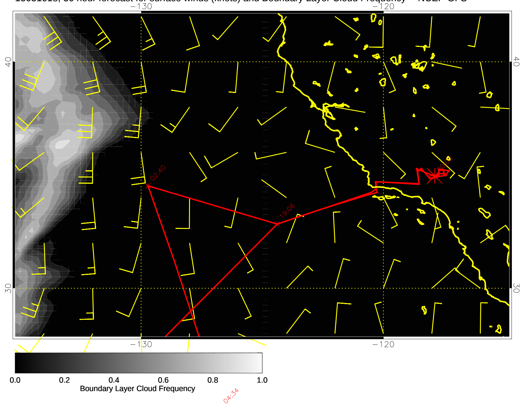
15031018, 30 hour forecast for surface winds (knots) and Boundary Layer Cloud Frequency -- NCEP GFS
