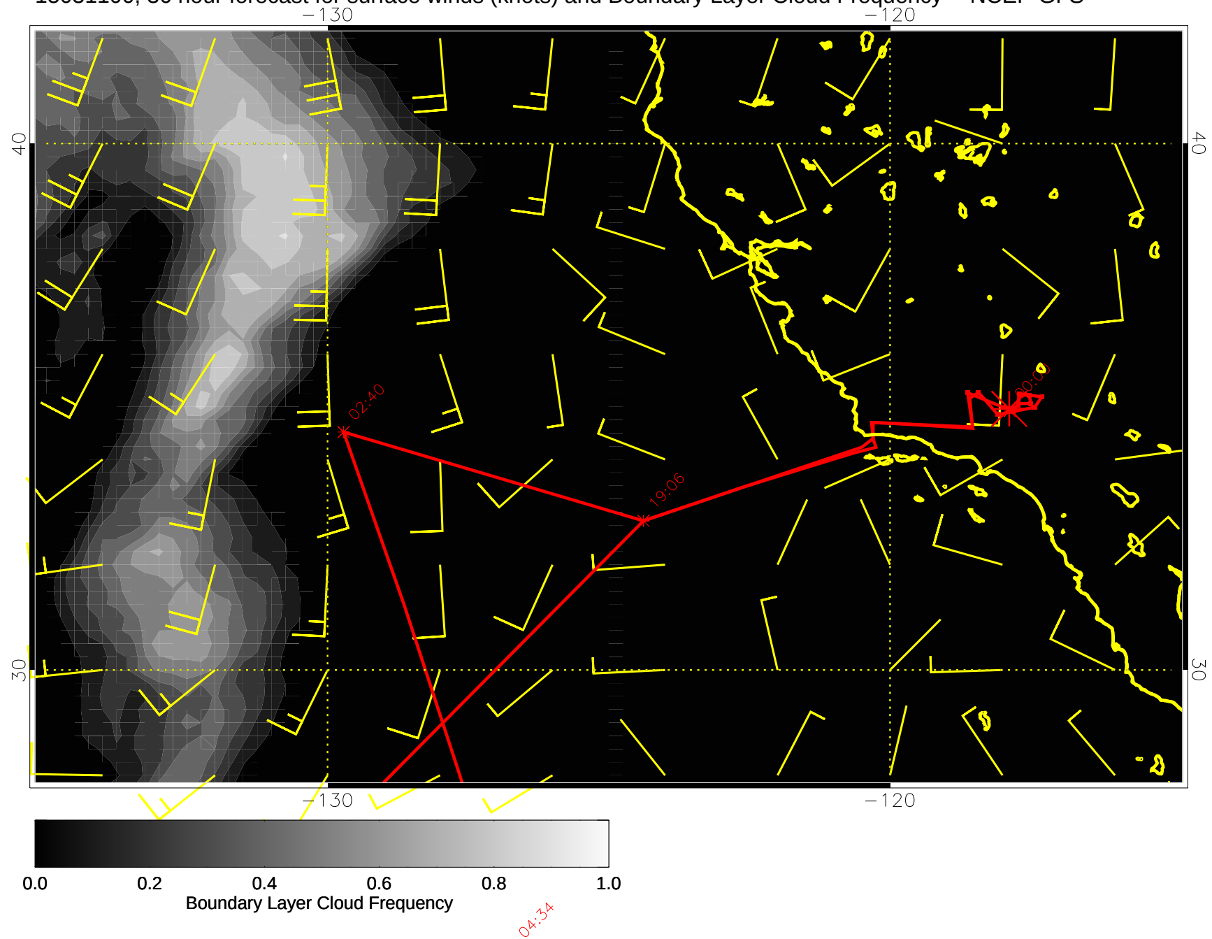
15031100, 36 hour forecast for surface winds (knots) and Boundary Layer Cloud Frequency -- NCEP GFS
