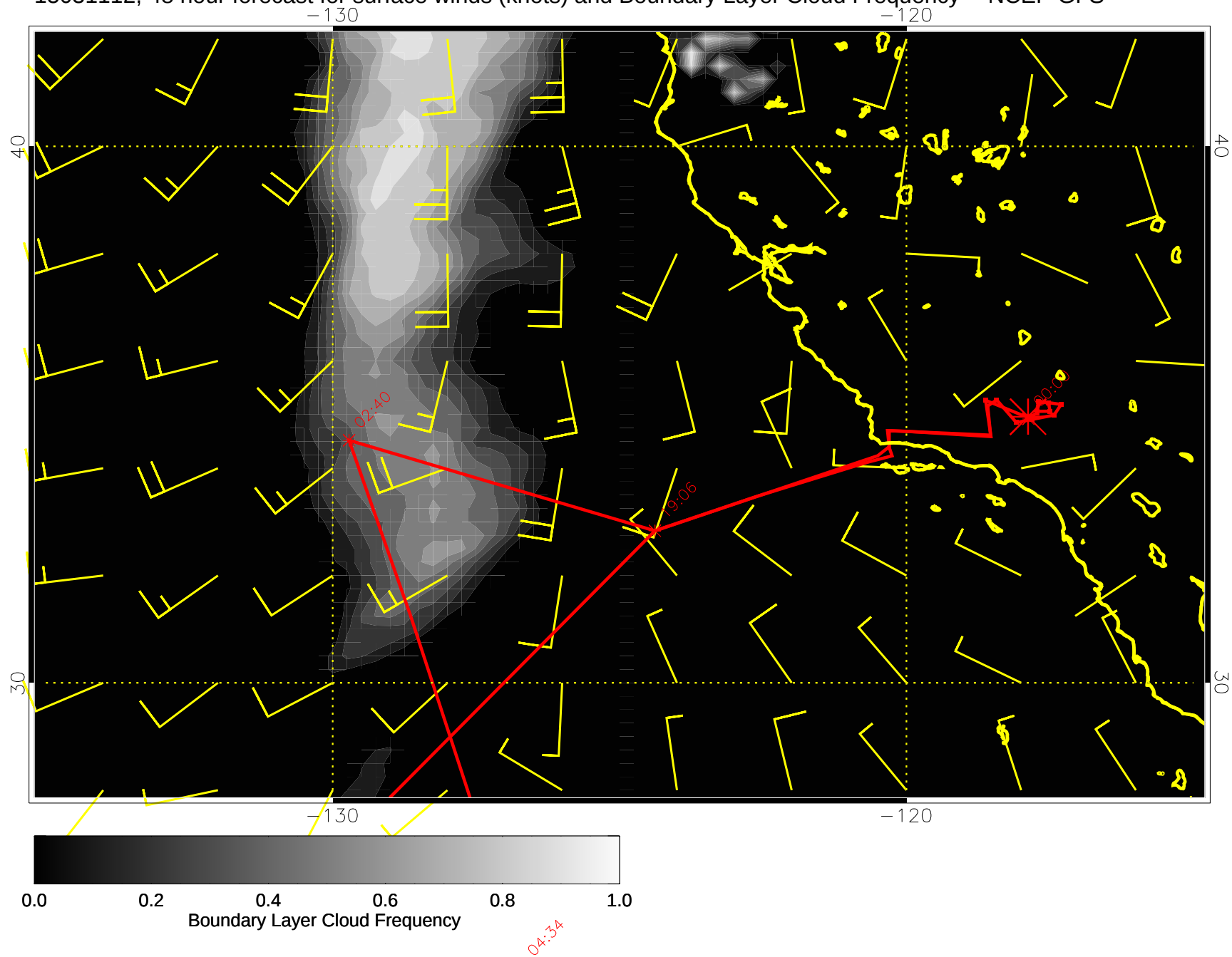
15031112, 48 hour forecast for surface winds (knots) and Boundary Layer Cloud Frequency -- NCEP GFS
