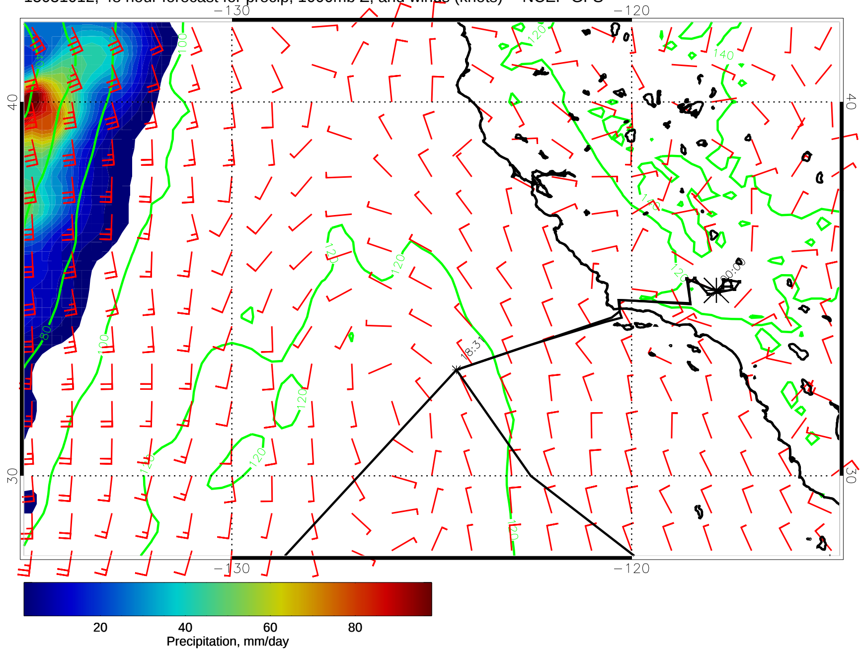
15031012, 48 hour forecast for precip, 1000mb Z, and winds (knots) -- NCEP GFS
