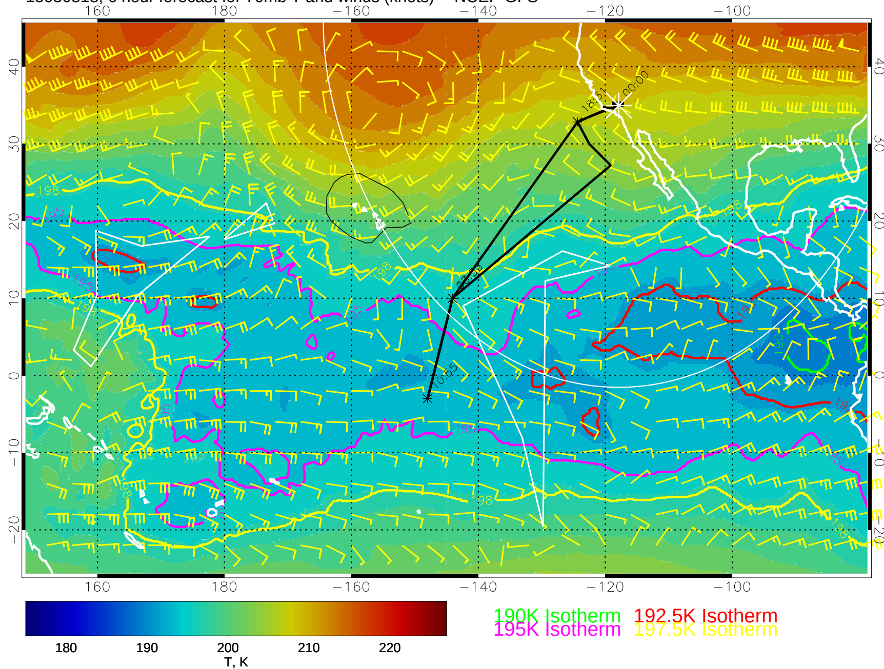
15030818, 6 hour forecast for 70mb T and winds (knots) -- NCEP GFS
