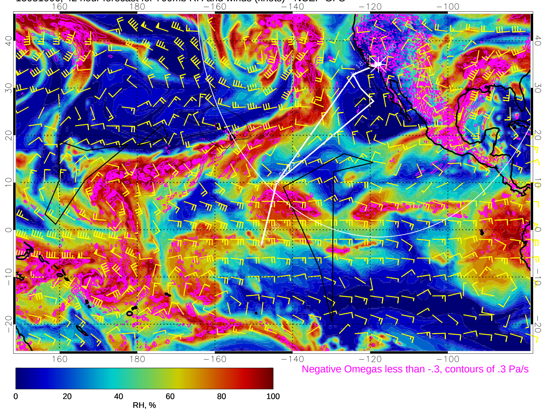
15031006, 42 hour forecast for 700mb RH and winds (knots) - NCEP GFS
