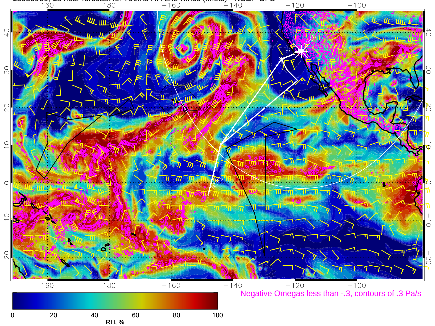
15030906, 18 hour forecast for 700mb RH and winds (knots) - NCEP GFS
