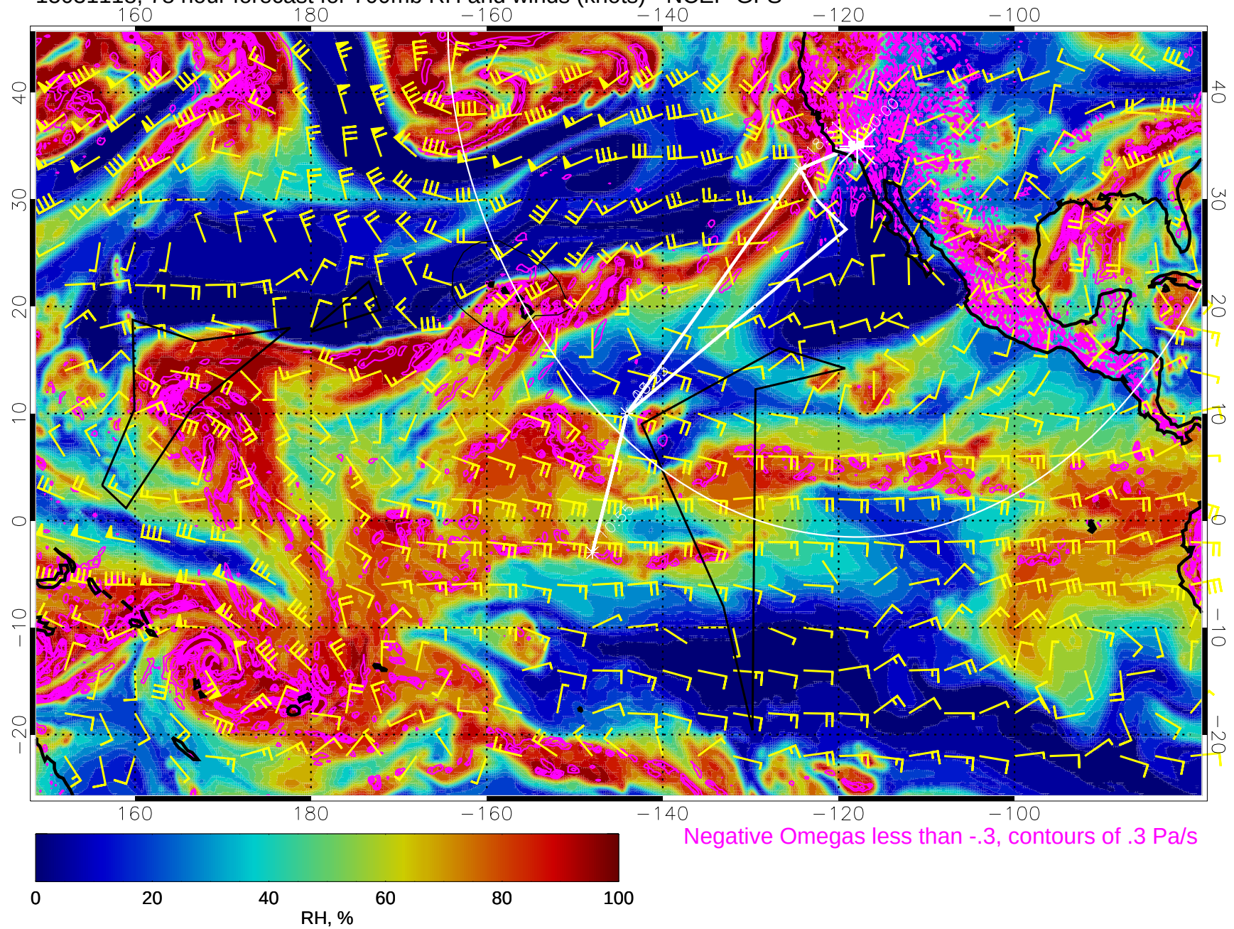
15031118, 78 hour forecast for 700mb RH and winds (knots) - NCEP GFS
