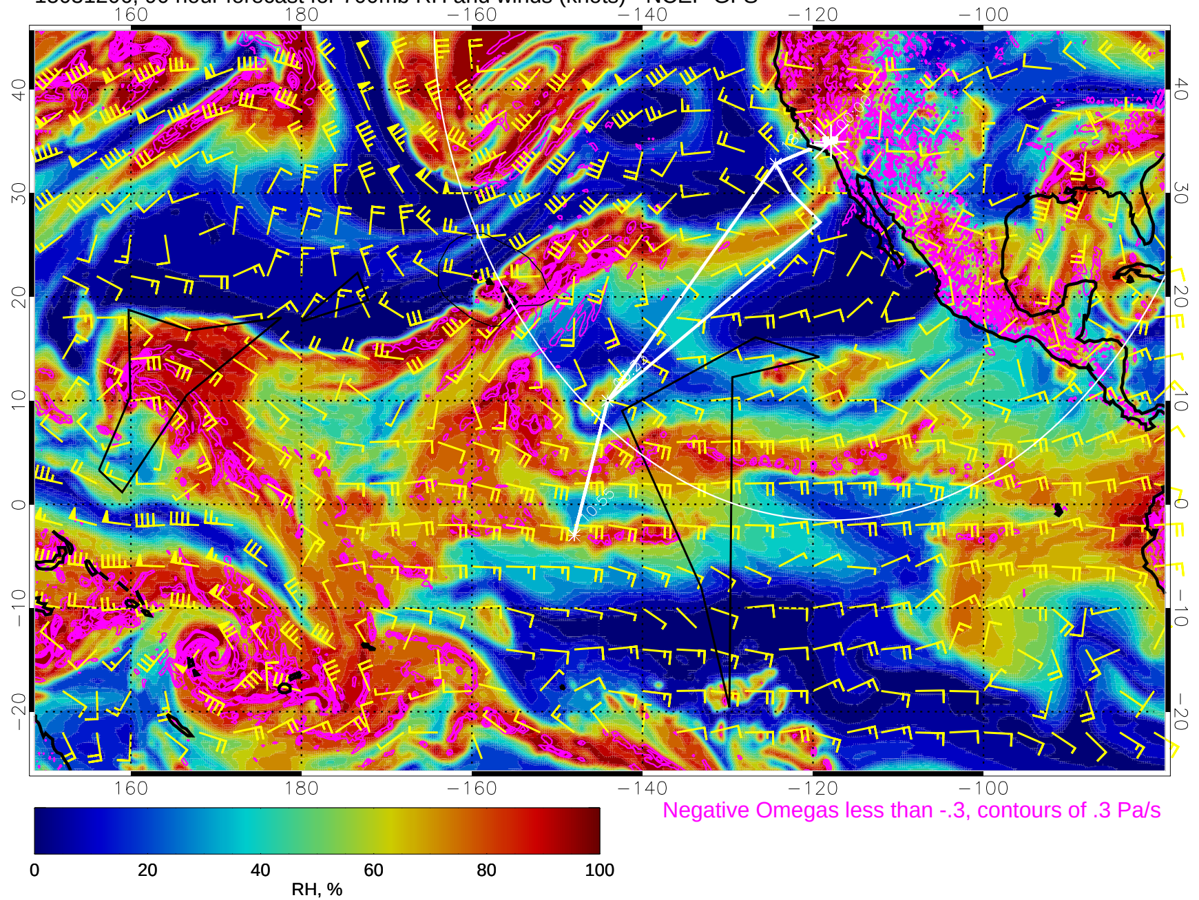
15031206, 90 hour forecast for 700mb RH and winds (knots) - NCEP GFS
