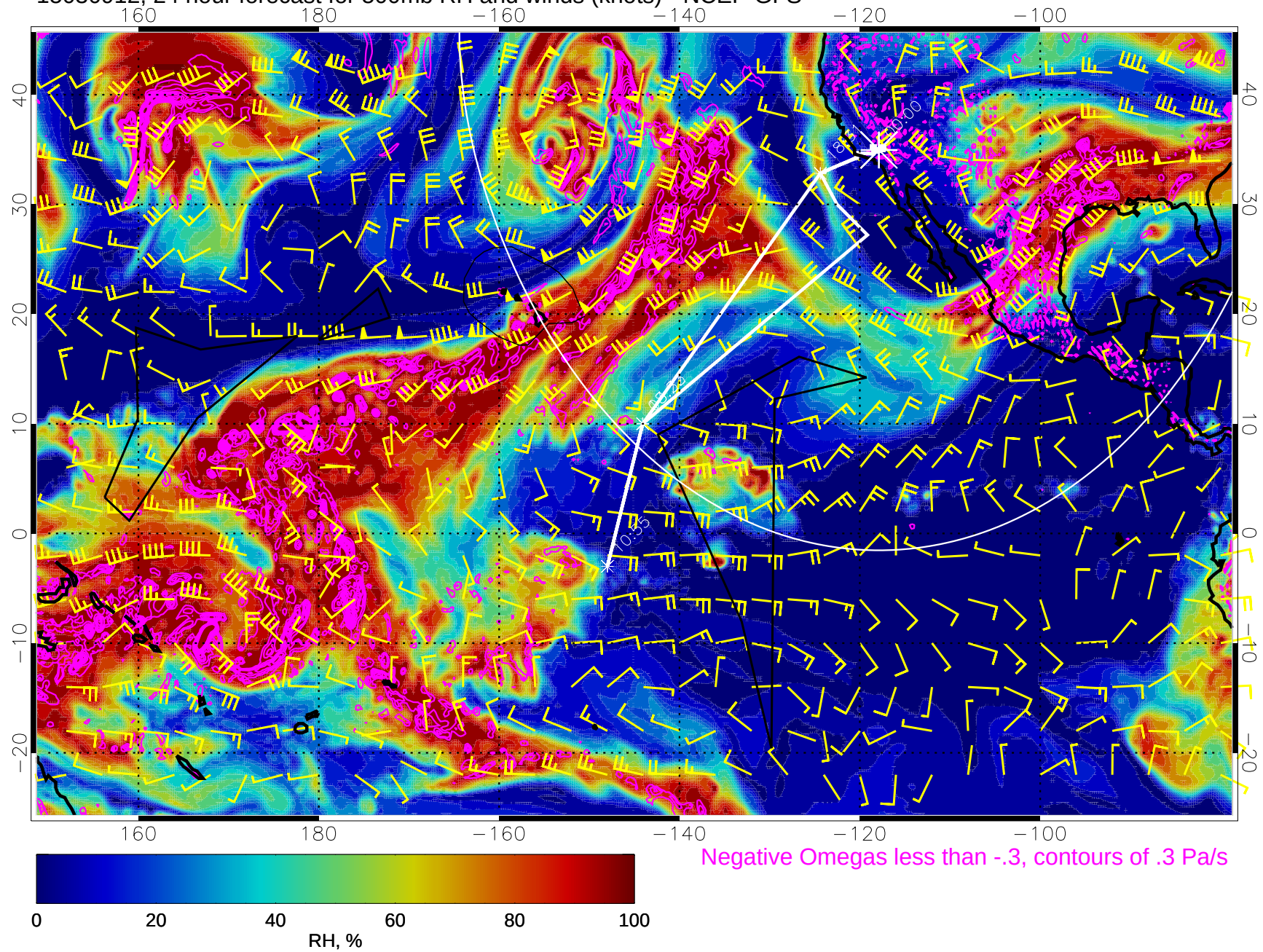
15030912, 24 hour forecast for 500mb RH and winds (knots) - NCEP GFS
