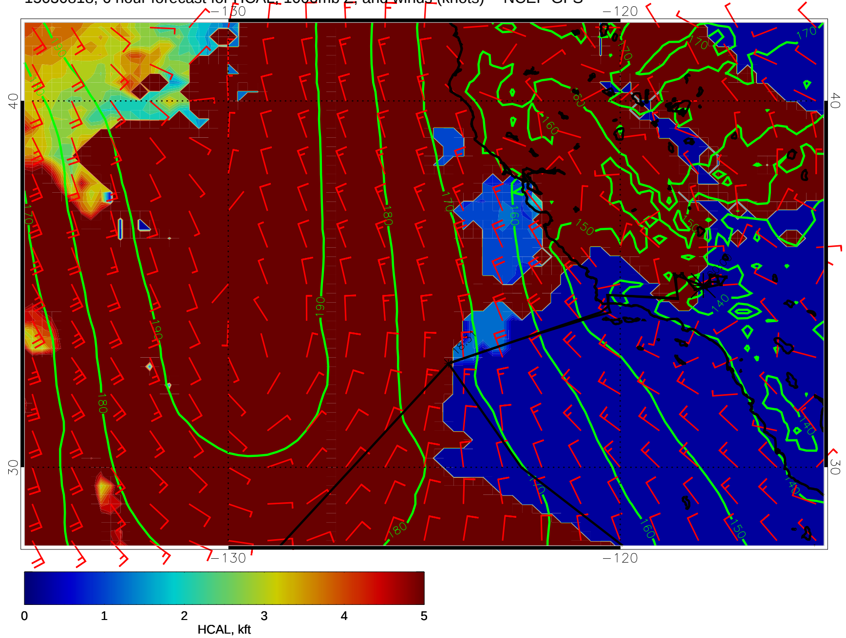
15030818, 6 hour forecast for HCAL, 1000mb Z, and winds (knots) -- NCEP GFS
