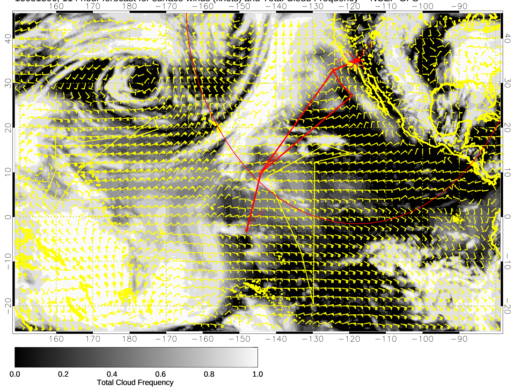
15031306, 114 hour forecast for surface winds (knots) and Total Cloud Frequency -- NCEP GFS
