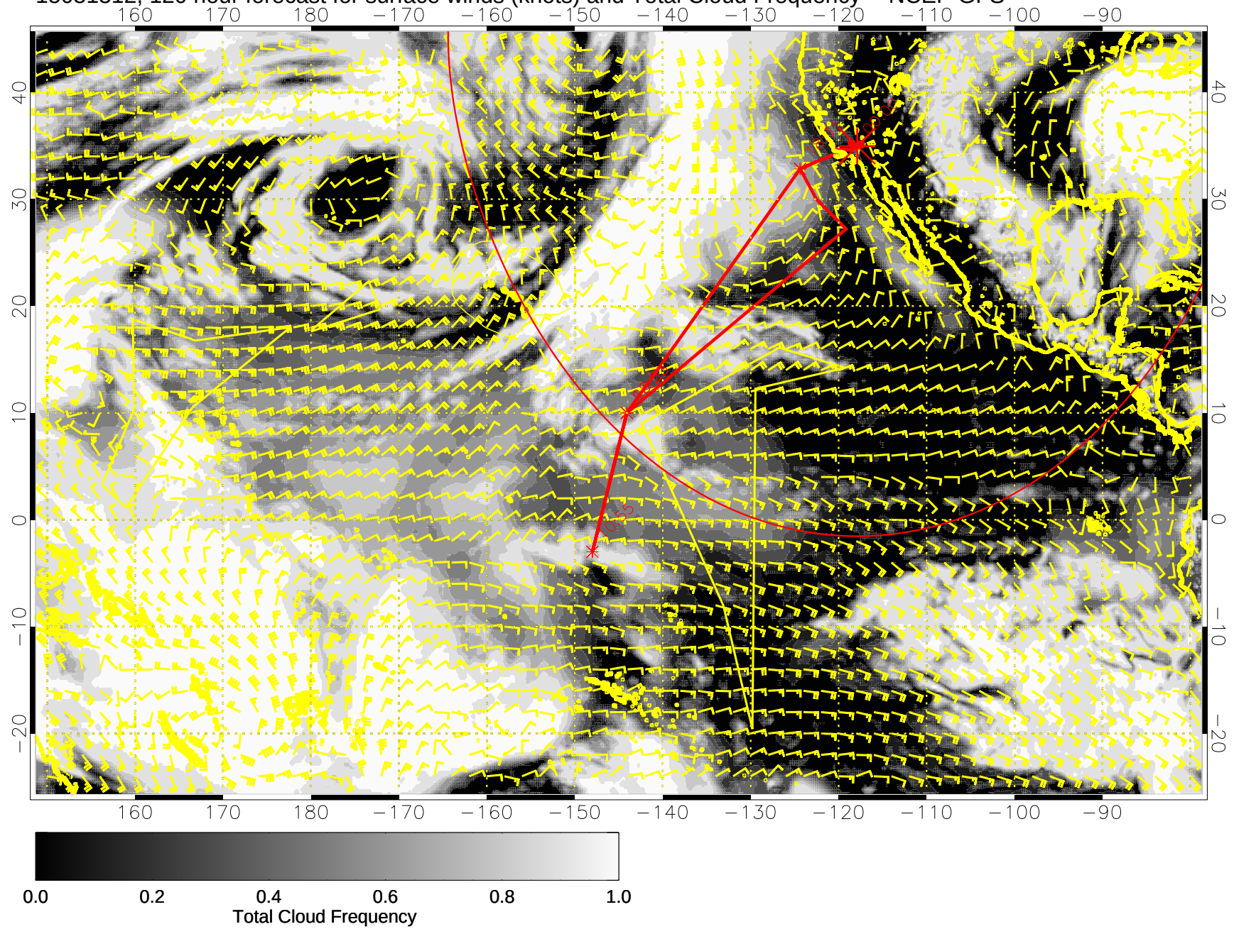
15031312, 120 hour forecast for surface winds (knots) and Total Cloud Frequency -- NCEP GFS
