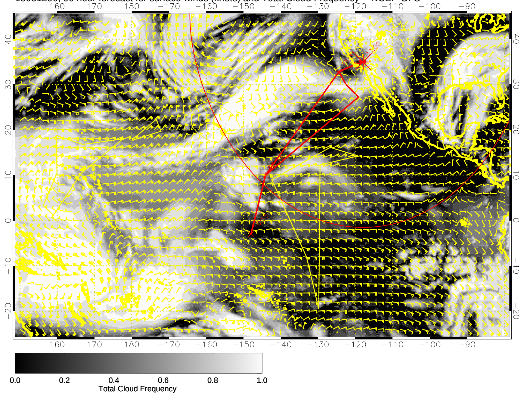
15031206, 90 hour forecast for surface winds (knots) and Total Cloud Frequency -- NCEP GFS
