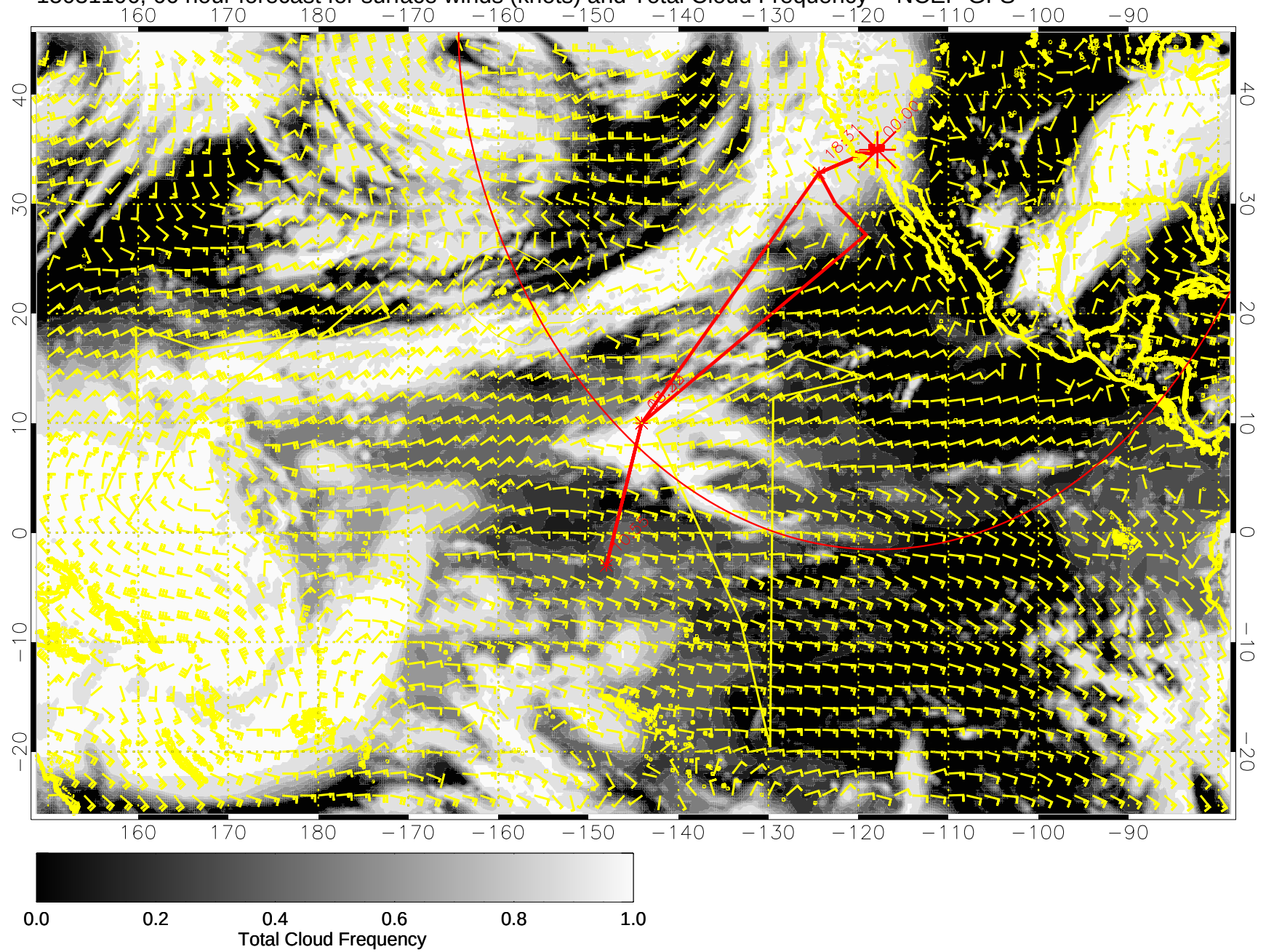
15031106, 66 hour forecast for surface winds (knots) and Total Cloud Frequency -- NCEP GFS
