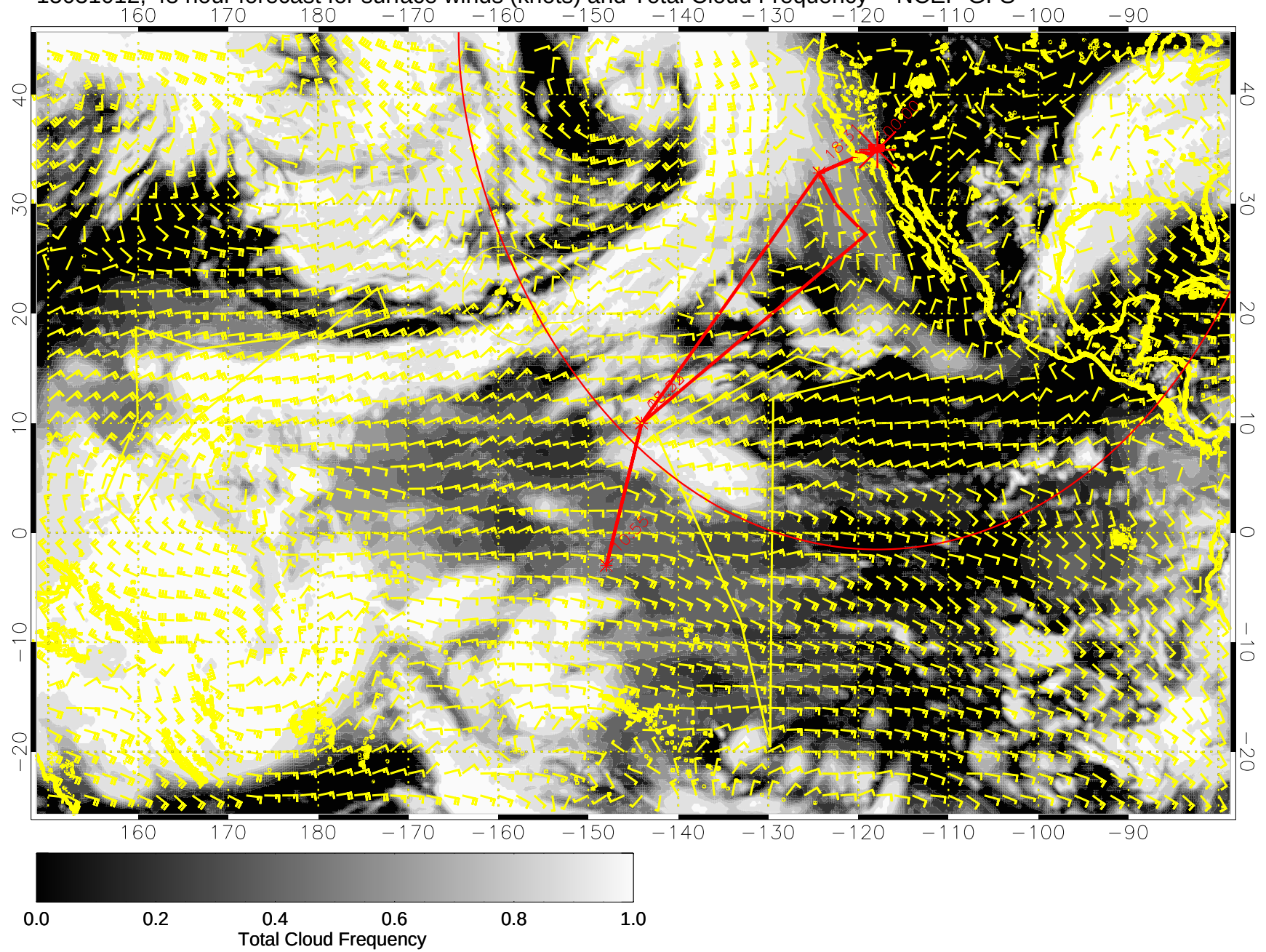
15031012, 48 hour forecast for surface winds (knots) and Total Cloud Frequency -- NCEP GFS
