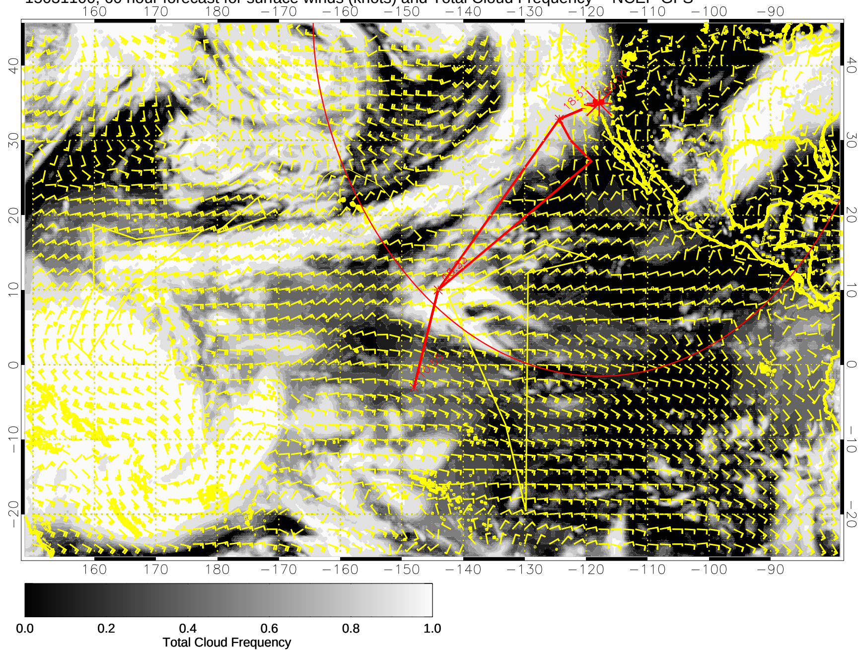
15031100, 60 hour forecast for surface winds (knots) and Total Cloud Frequency -- NCEP GFS
