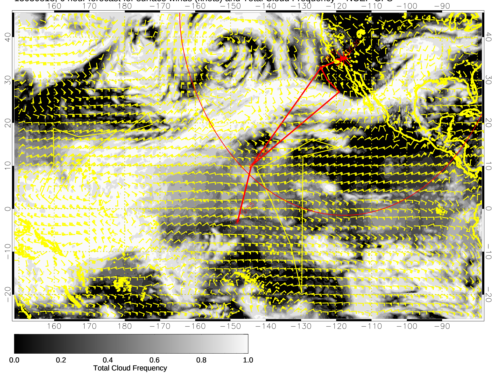
15030818, 6 hour forecast for surface winds (knots) and Total Cloud Frequency -- NCEP GFS
