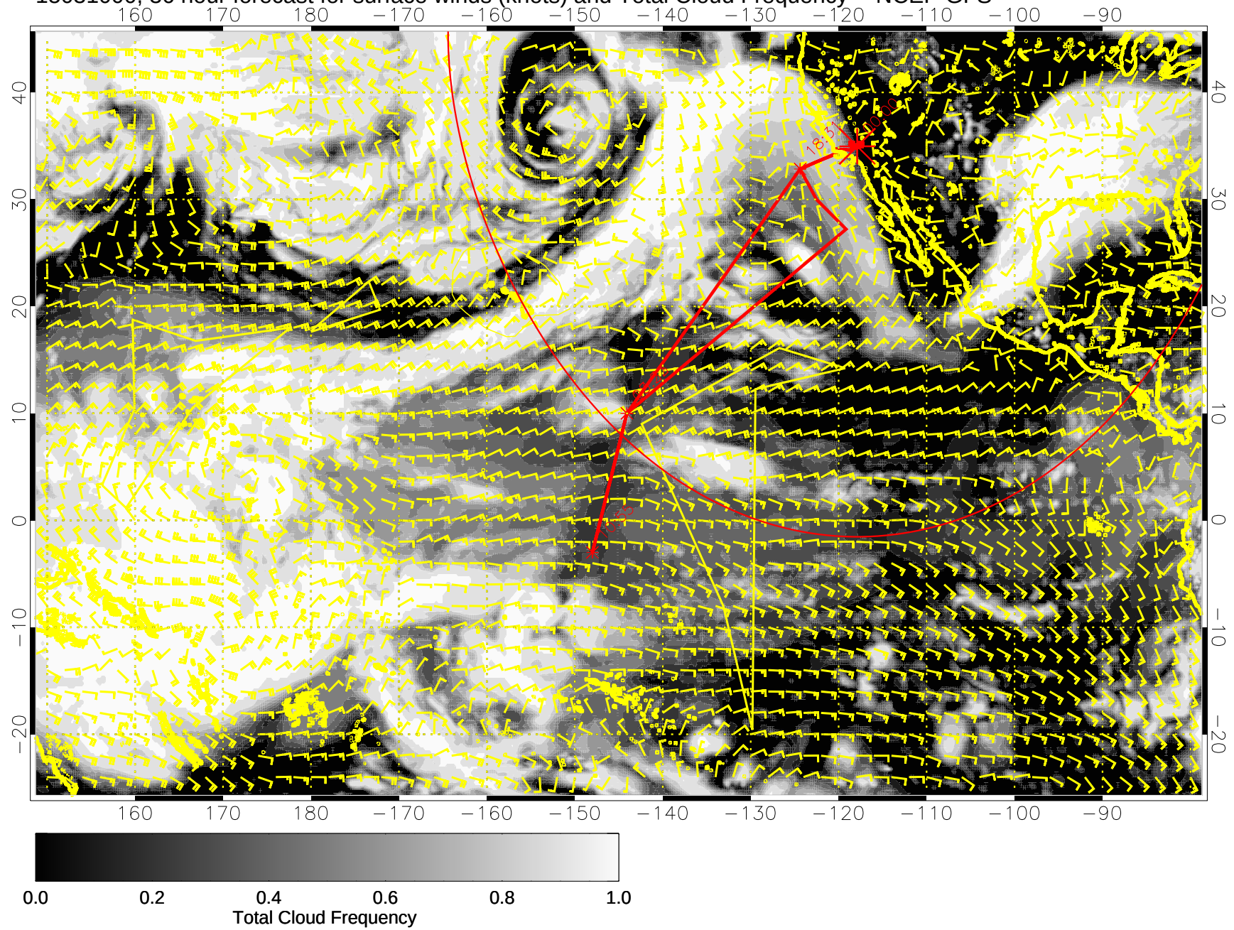
15031000, 36 hour forecast for surface winds (knots) and Total Cloud Frequency -- NCEP GFS
