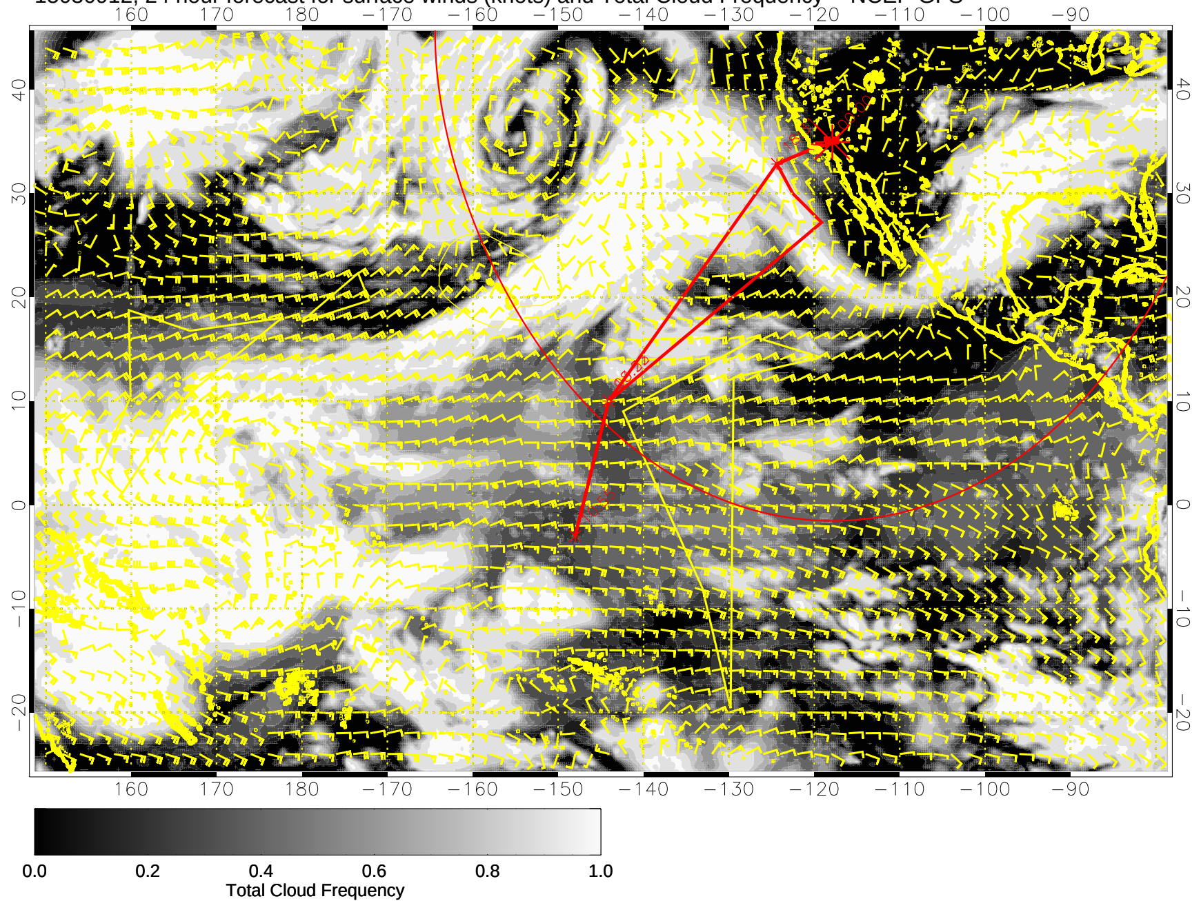
15030912, 24 hour forecast for surface winds (knots) and Total Cloud Frequency -- NCEP GFS
