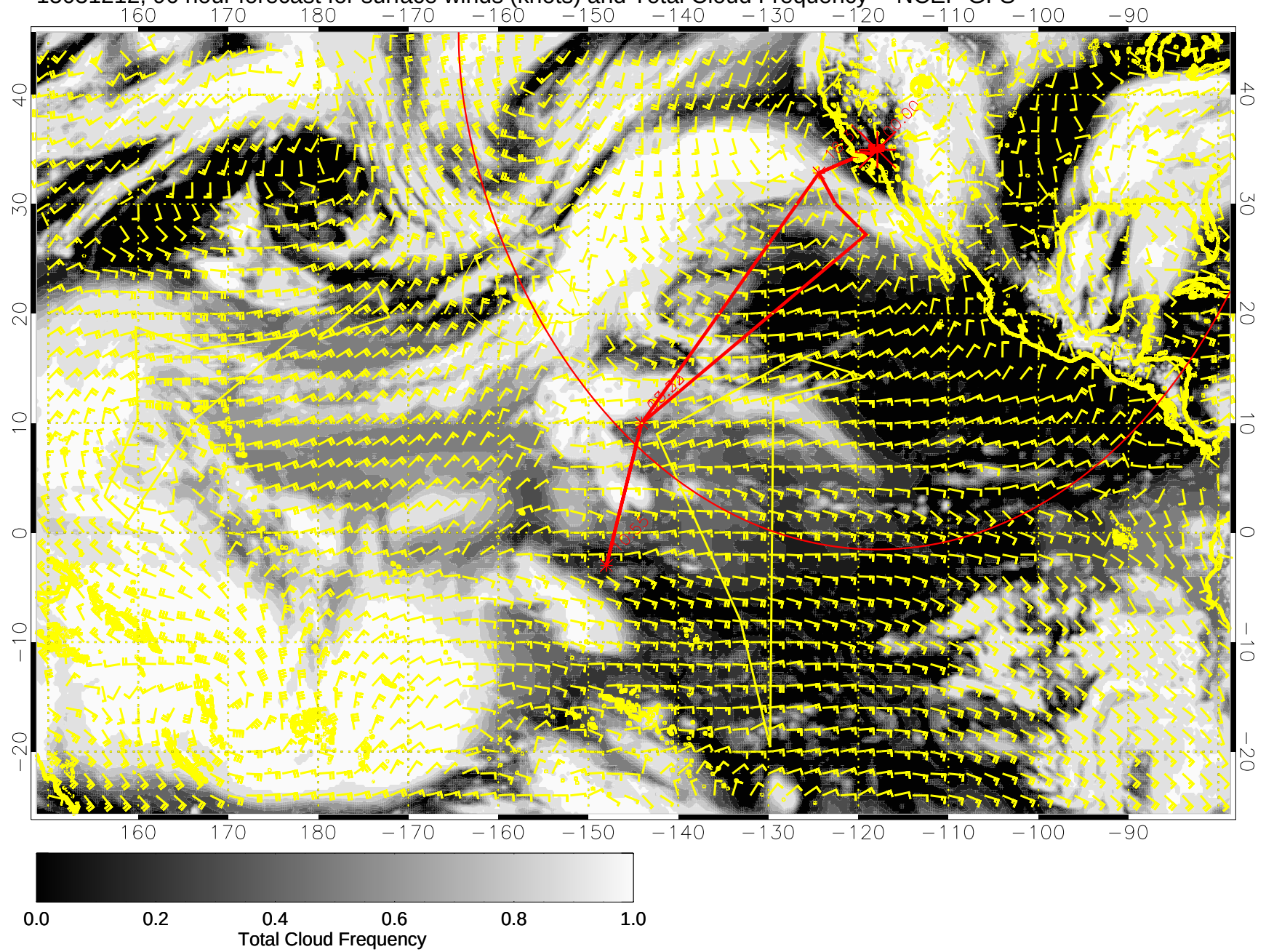
15031212, 96 hour forecast for surface winds (knots) and Total Cloud Frequency -- NCEP GFS
