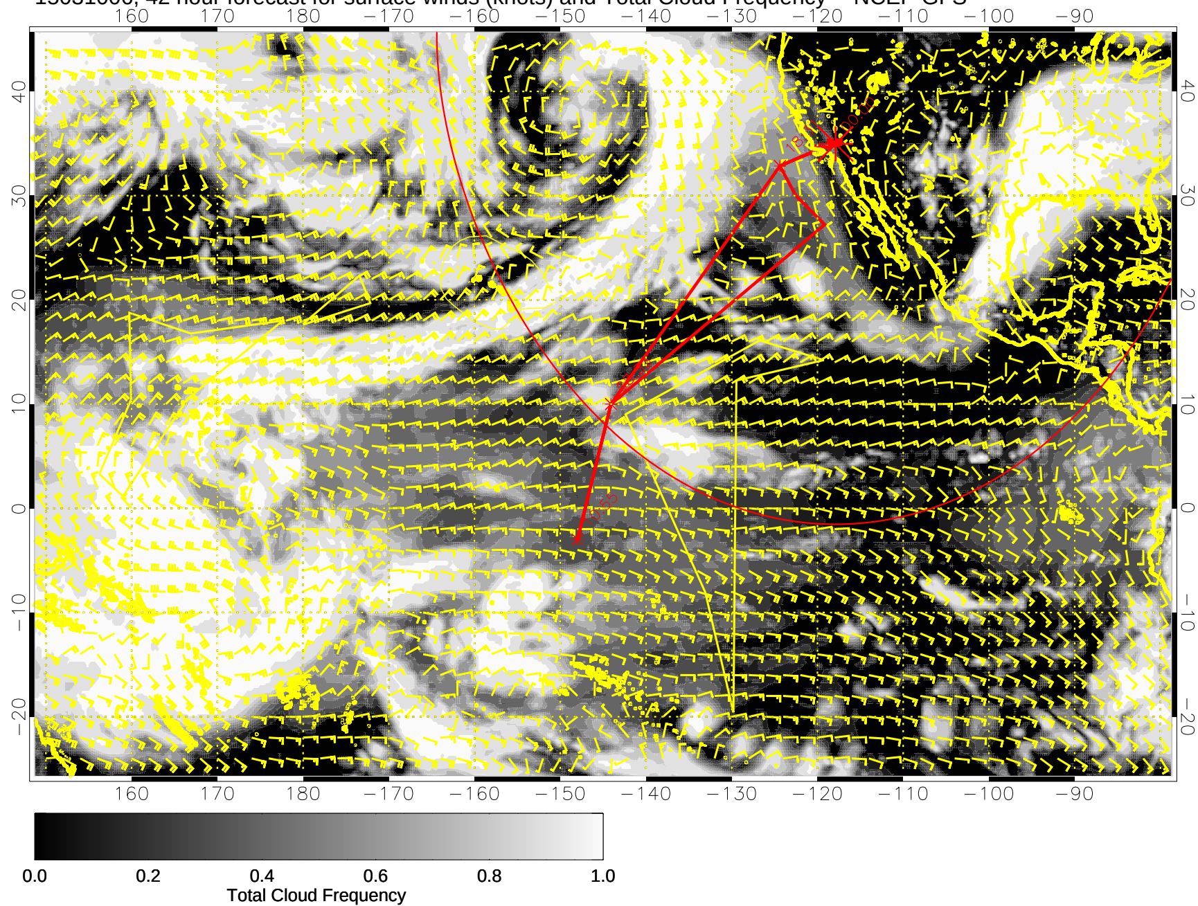
15031006, 42 hour forecast for surface winds (knots) and Total Cloud Frequency -- NCEP GFS
