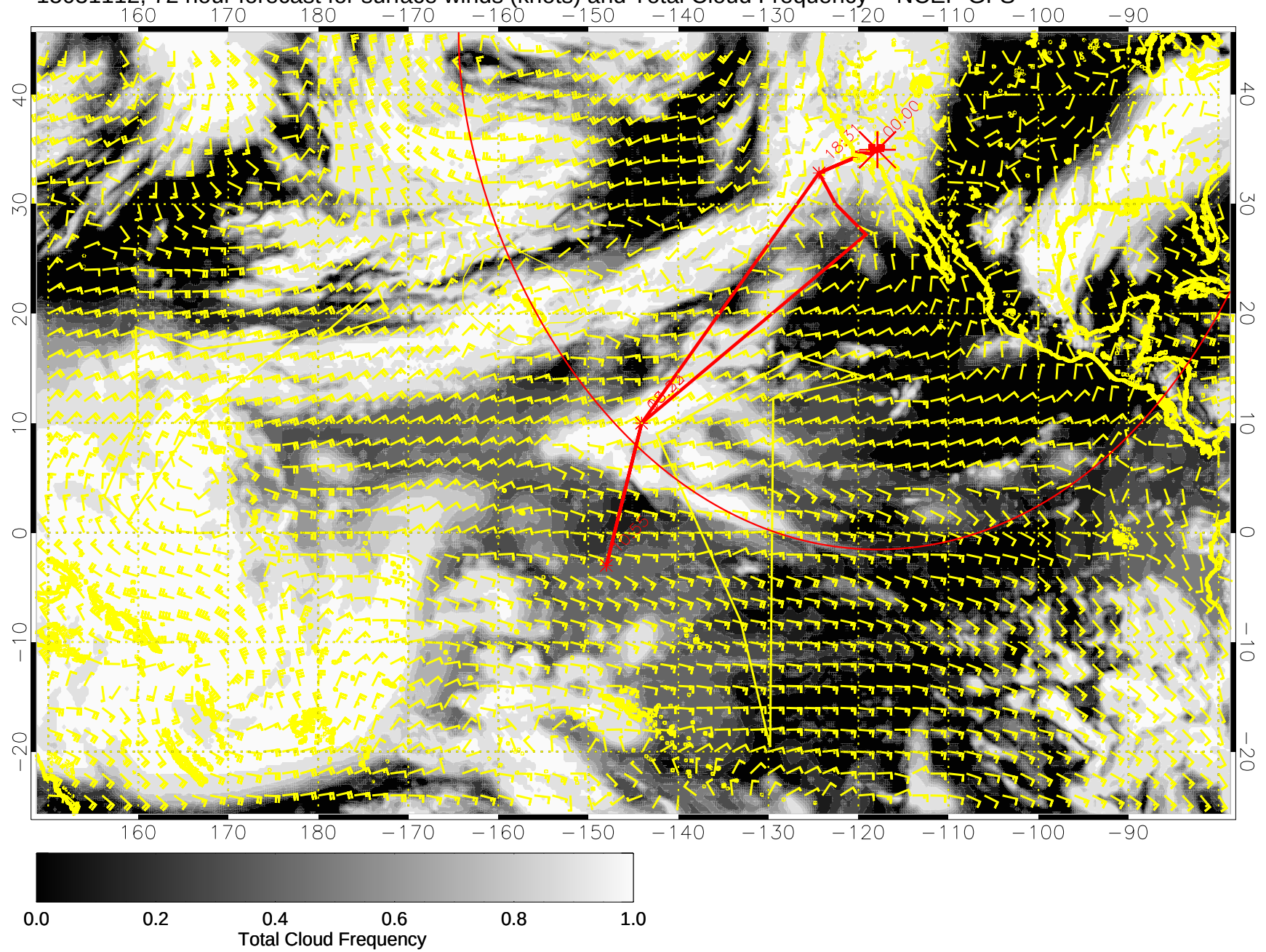
15031112, 72 hour forecast for surface winds (knots) and Total Cloud Frequency -- NCEP GFS
