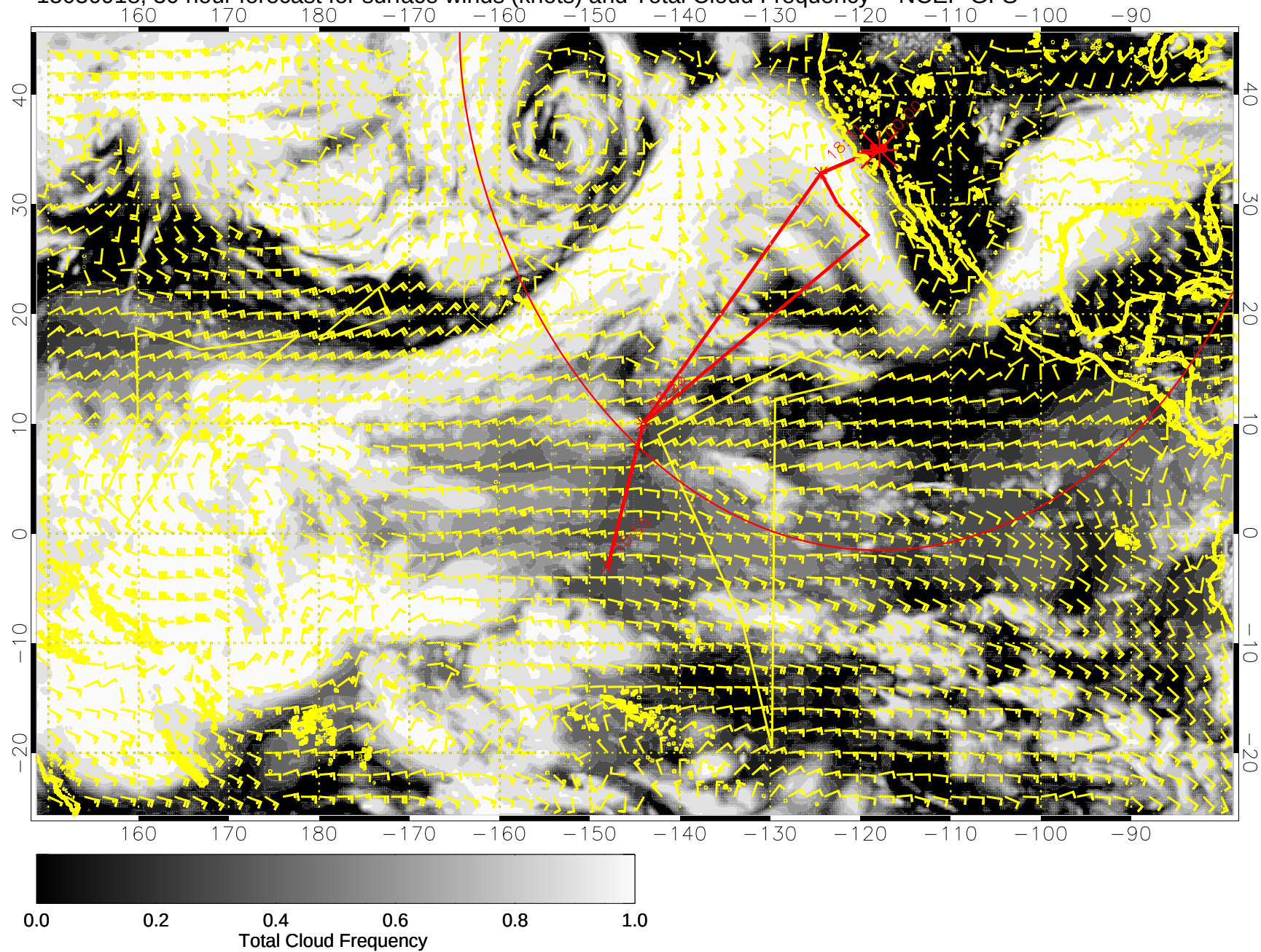
15030918, 30 hour forecast for surface winds (knots) and Total Cloud Frequency -- NCEP GFS
