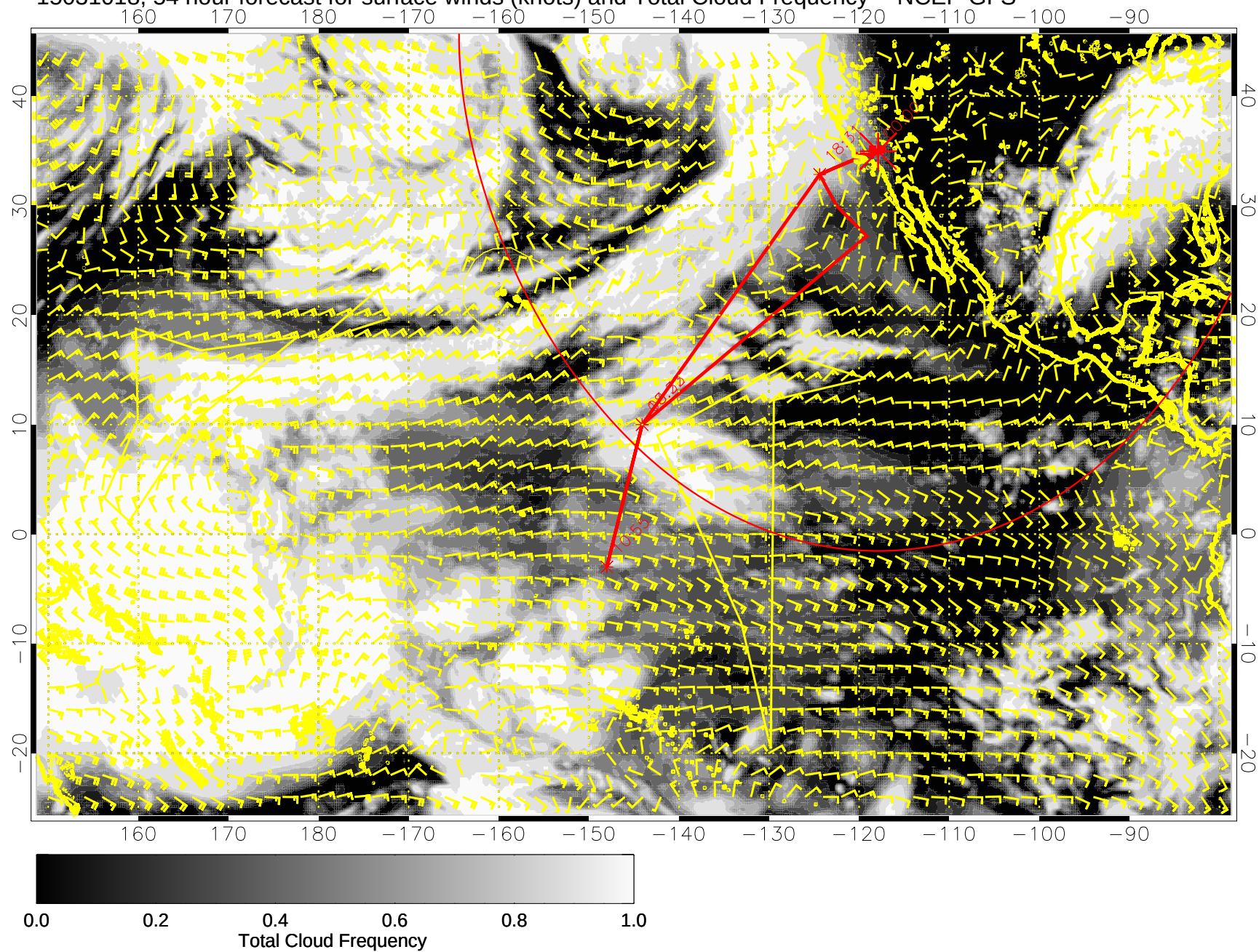
15031018, 54 hour forecast for surface winds (knots) and Total Cloud Frequency -- NCEP GFS
