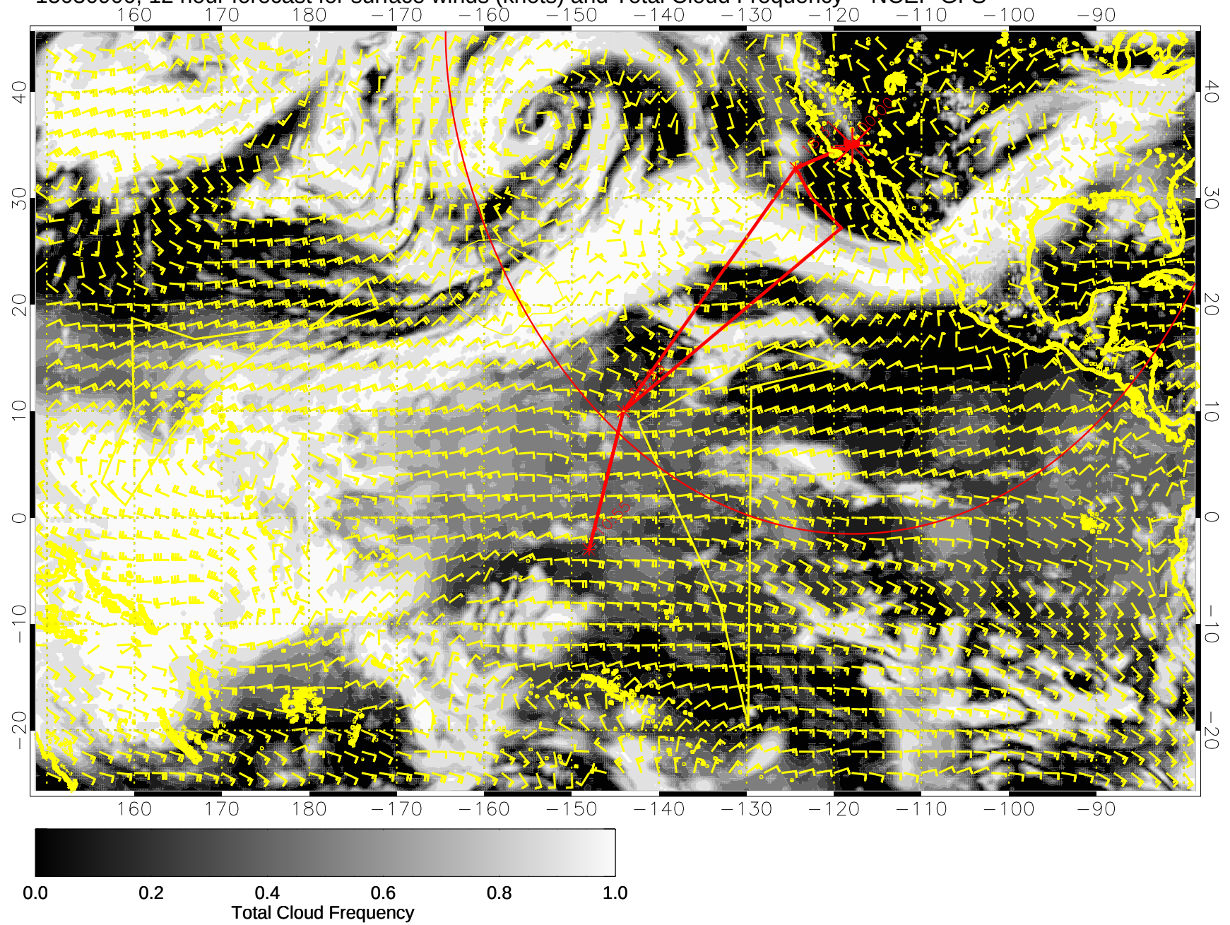
15030900, 12 hour forecast for surface winds (knots) and Total Cloud Frequency -- NCEP GFS
