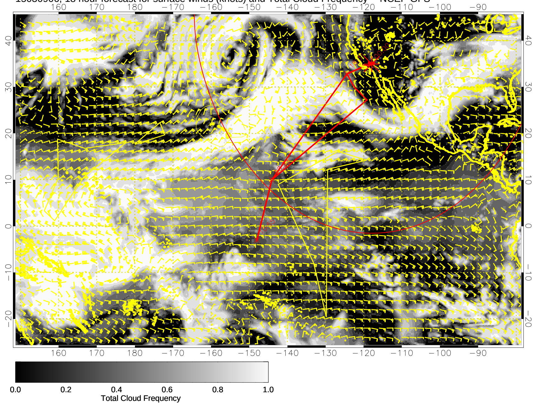
15030906, 18 hour forecast for surface winds (knots) and Total Cloud Frequency -- NCEP GFS
