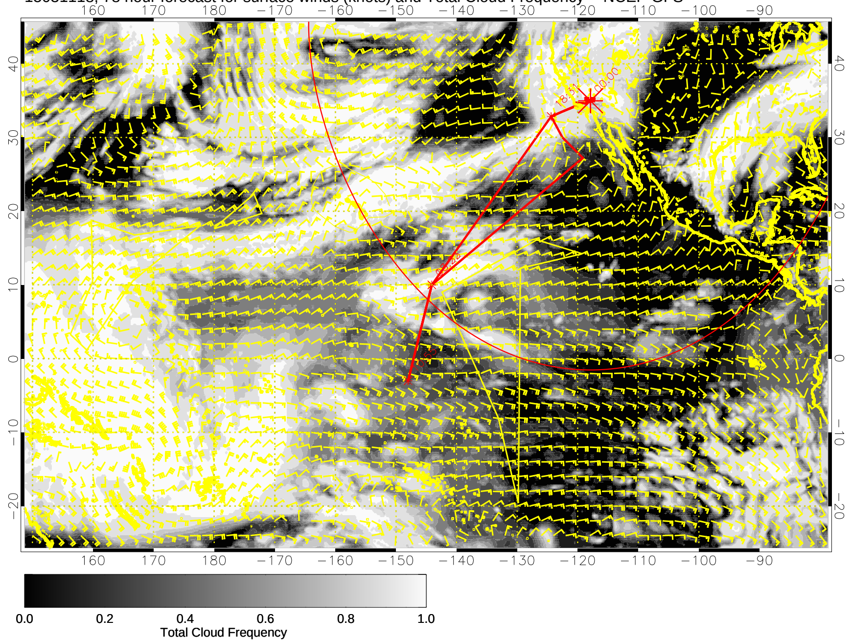
15031118, 78 hour forecast for surface winds (knots) and Total Cloud Frequency -- NCEP GFS
