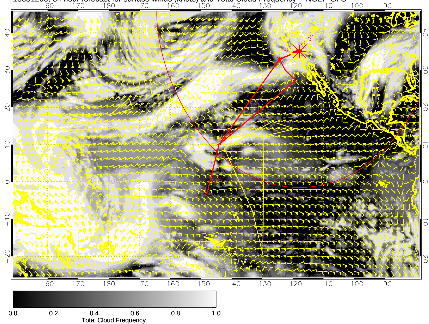
15031200, 84 hour forecast for surface winds (knots) and Total Cloud Frequency -- NCEP GFS
