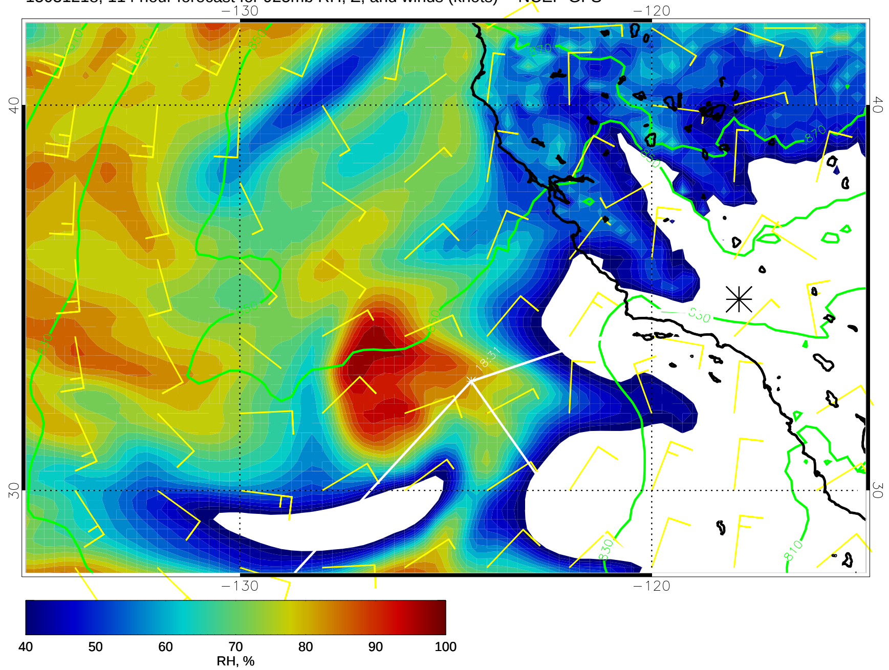
15031218, 114 hour forecast for 925mb RH, Z, and winds (knots) -- NCEP GFS
