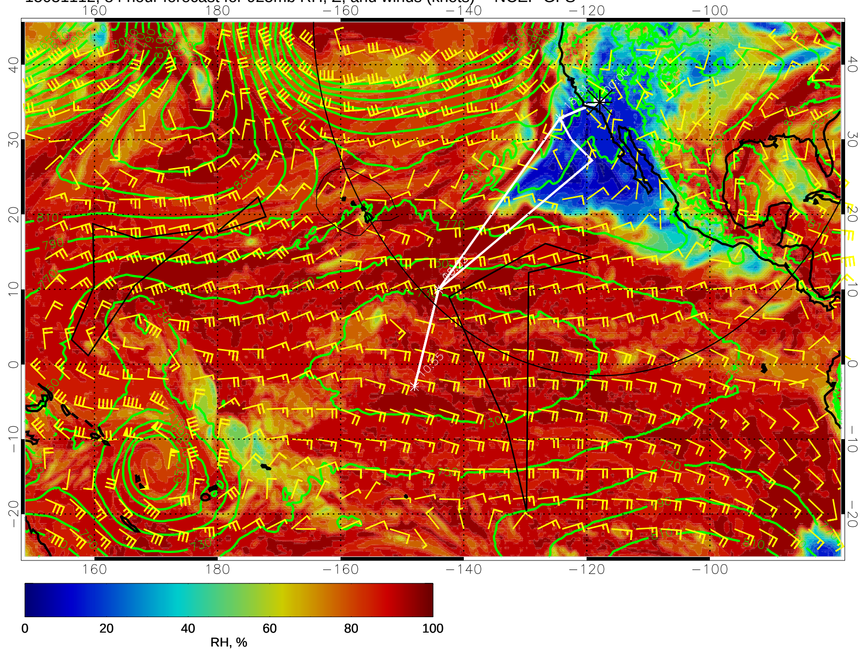
15031112, 84 hour forecast for 925mb RH, Z, and winds (knots) -- NCEP GFS
