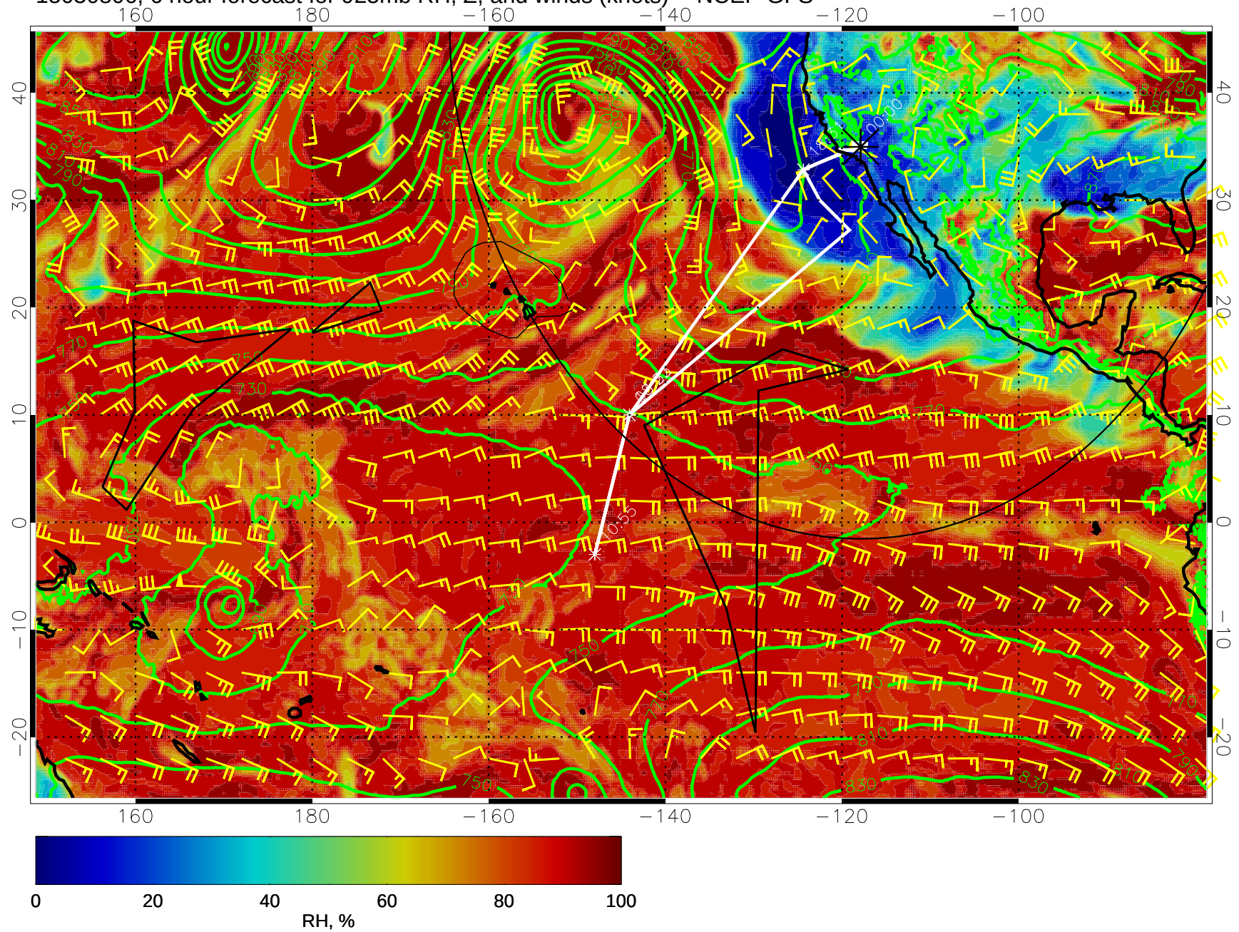
15030806, 6 hour forecast for 925mb RH, Z, and winds (knots) -- NCEP GFS
