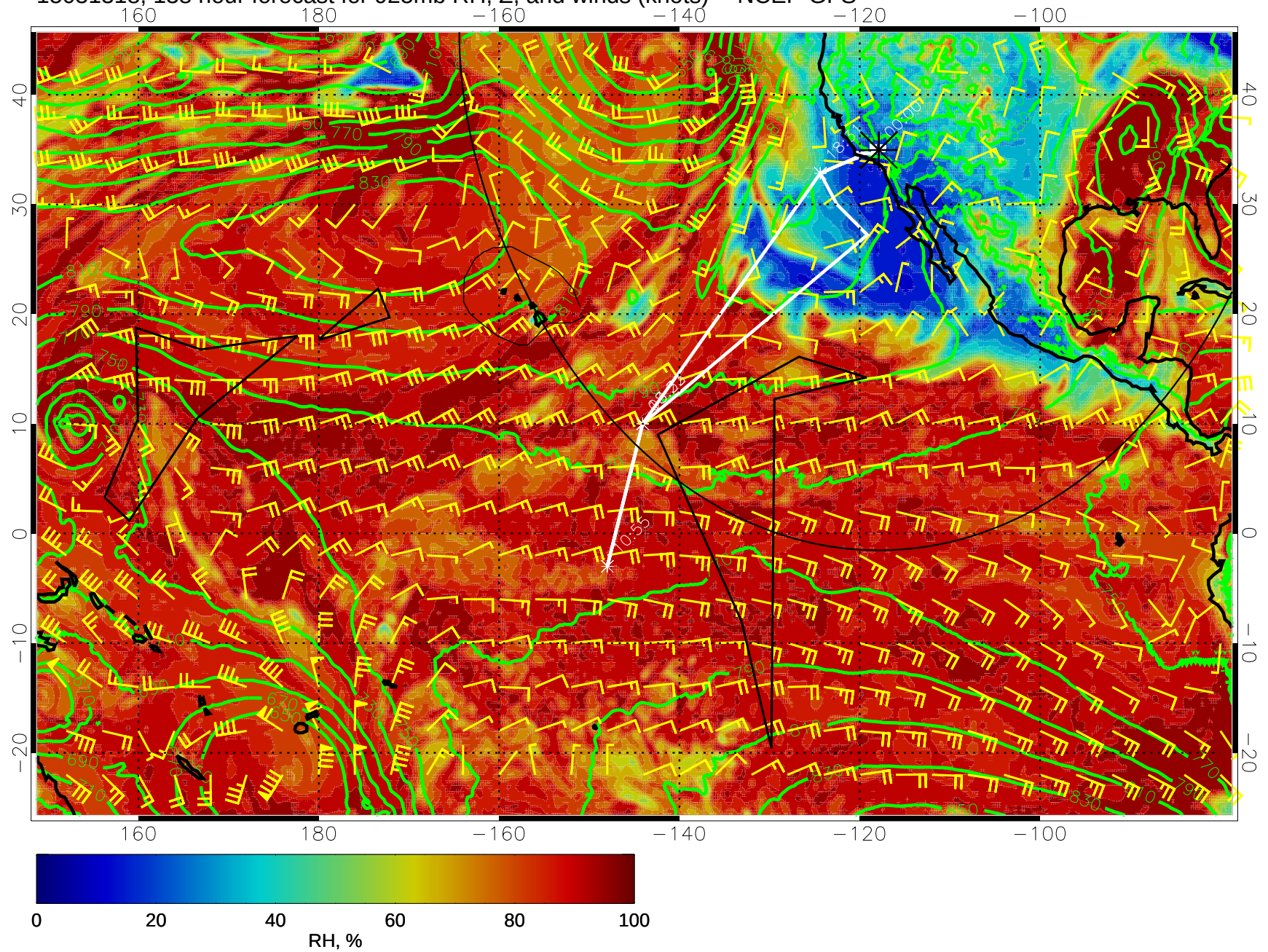
15031318, 138 hour forecast for 925mb RH, Z, and winds (knots) -- NCEP GFS
