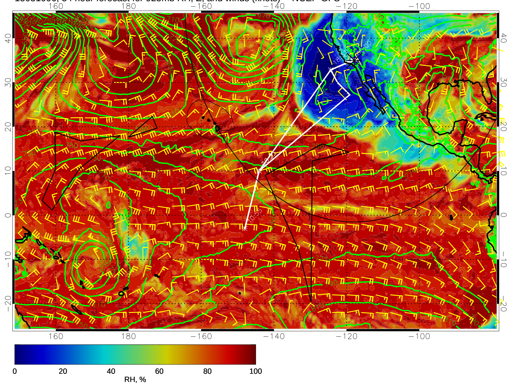
15031006, 54 hour forecast for 925mb RH, Z, and winds (knots) -- NCEP GFS
