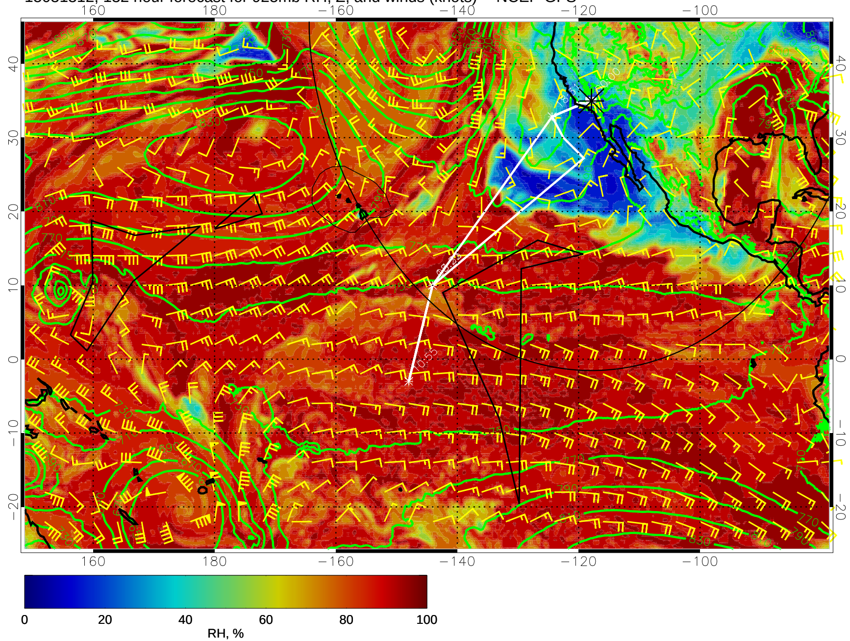
15031312, 132 hour forecast for 925mb RH, Z, and winds (knots) -- NCEP GFS
