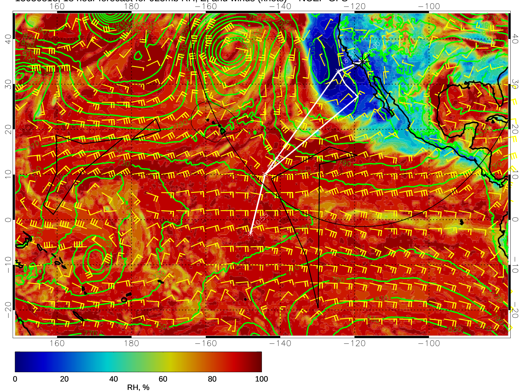
15030818, 18 hour forecast for 925mb RH, Z, and winds (knots) -- NCEP GFS
