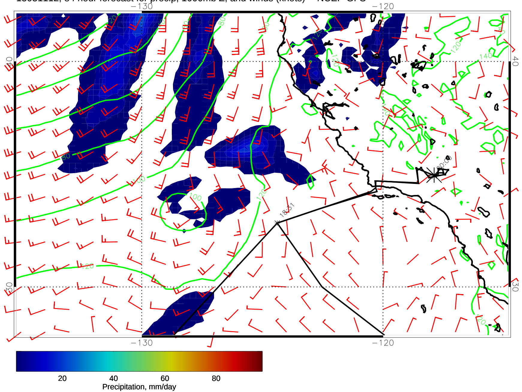
15031112, 84 hour forecast for precip, 1000mb Z, and winds (knots) -- NCEP GFS
