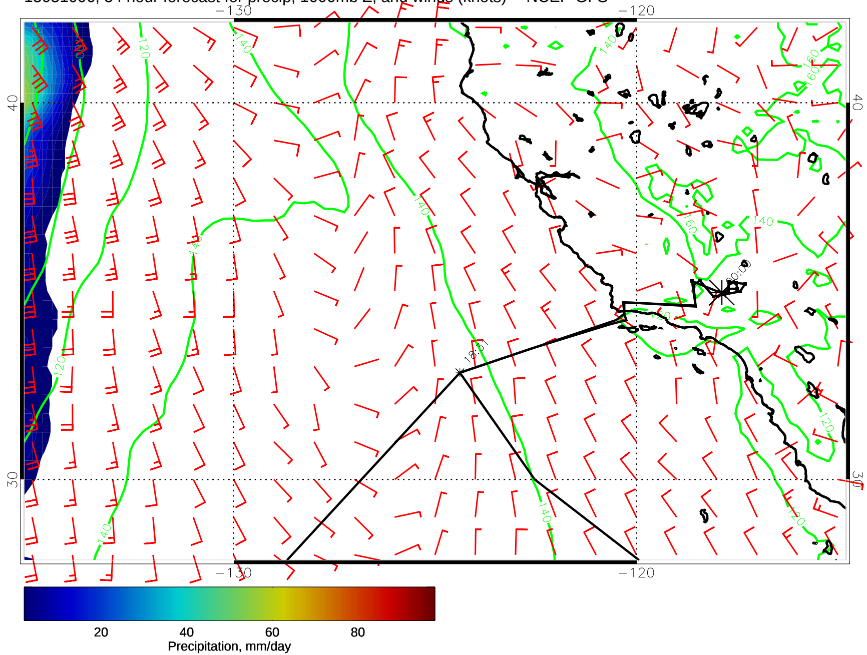
15031006, 54 hour forecast for precip, 1000mb Z, and winds (knots) -- NCEP GFS
