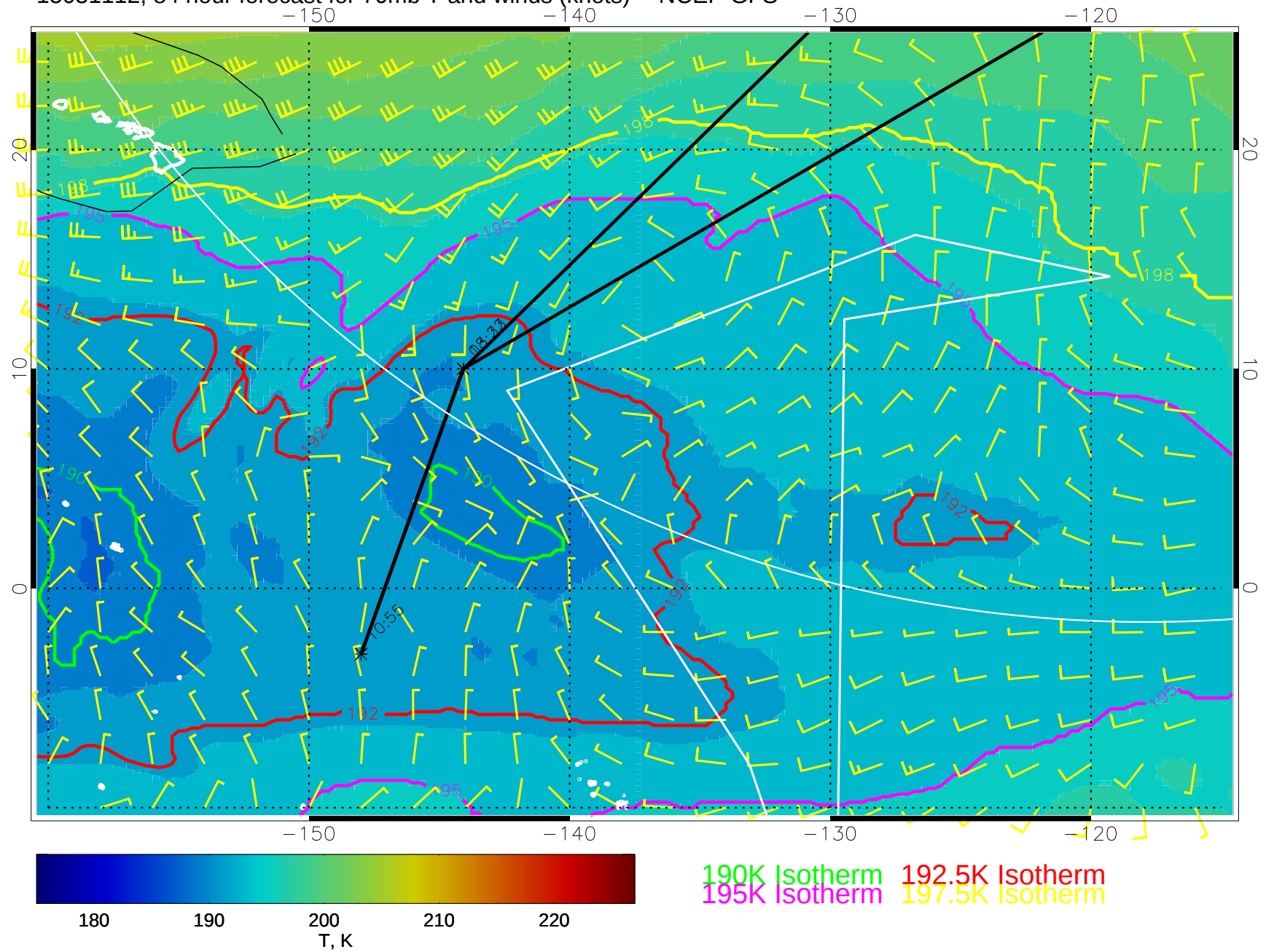
15031112, 84 hour forecast for 70mb T and winds (knots) -- NCEP GFS
