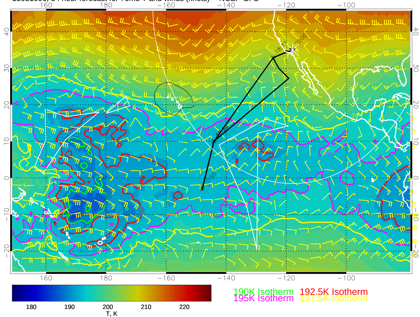
15031006, 54 hour forecast for 70mb T and winds (knots) -- NCEP GFS
