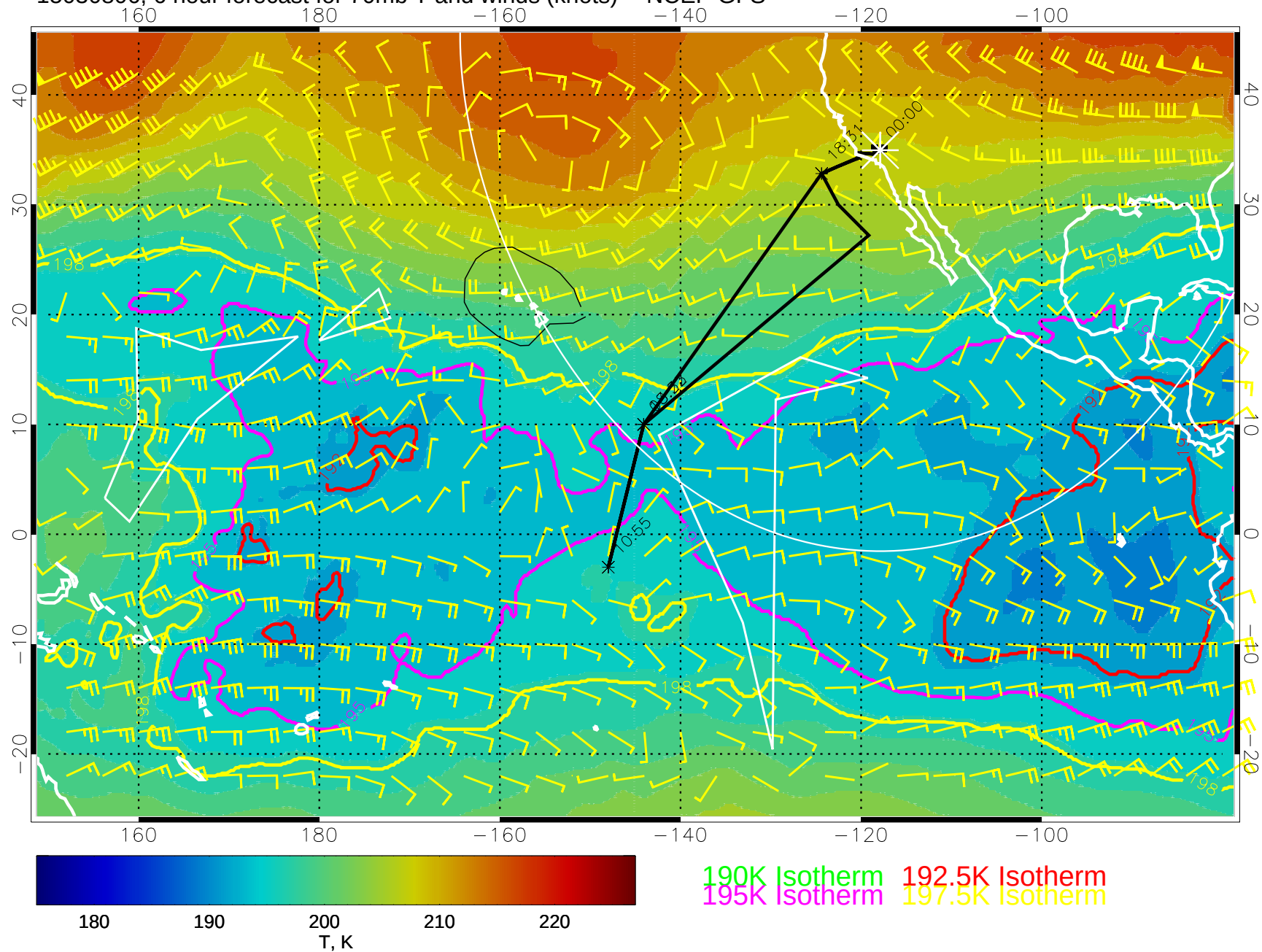
15030806, 6 hour forecast for 70mb T and winds (knots) -- NCEP GFS
