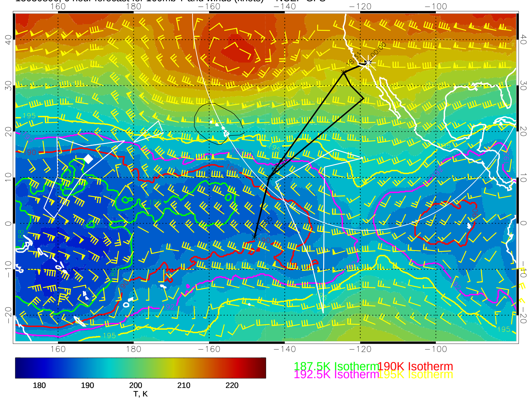
15030806, 6 hour forecast for 100mb T and winds (knots) -- NCEP GFS
